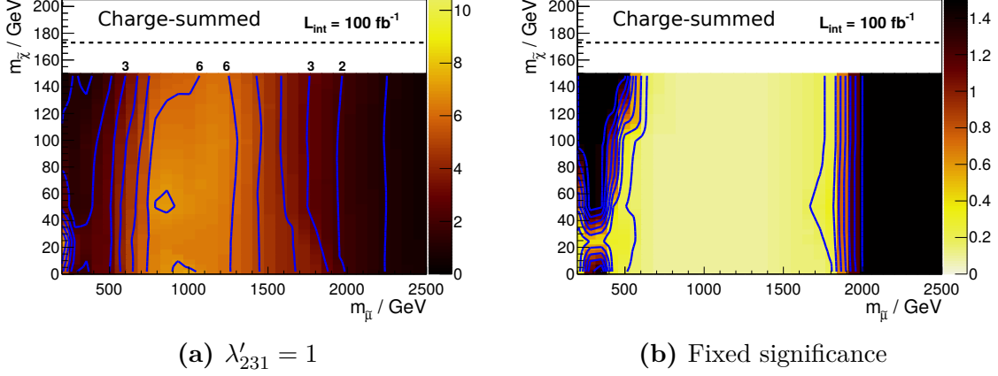
Figure 7.8: The left-hand plot shows the median significance of the charge-summed analysis, as quantified by the Z_A variable of Reference [143]. A constant 15% uncertainty in the background prediction is assumed. For each point on the grid, the significance is evaluated for events with \sum m_T greater than a model-dependent threshold. Contour lines show integer values of sensitivity. The right-hand plot shows the minimal value of the coupling strength \lambda'_{231} for which 2\sigma significance is achieved. Contour lines are drawn at intervals of 0.1 in the coupling strength.
