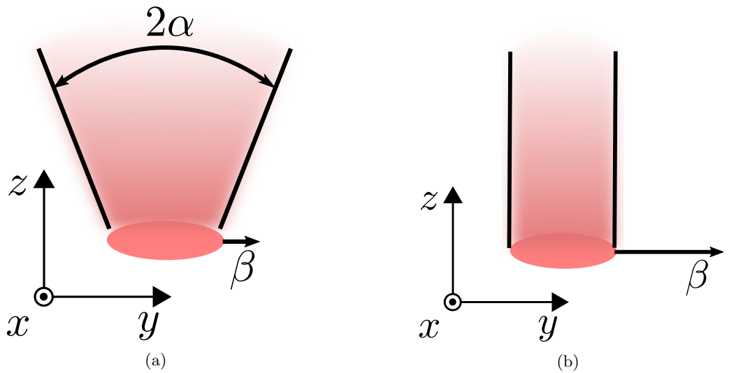
Figure 3.3: Propagating Coulomb field for (a) \beta \ll 1 and (b) \beta \simeq 1 .
