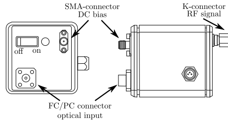
Figure 5.10: Technical drawing of the fast detector.
