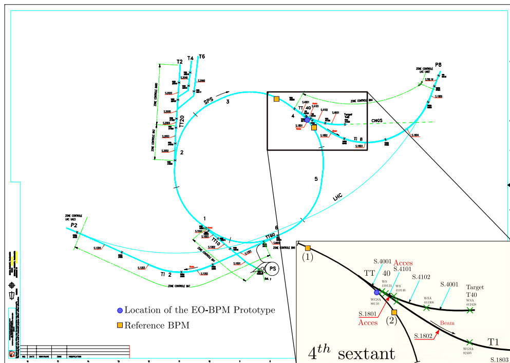
Figure 1.4: Layout of the SPS ring with a detail of the zoomed section that shows where the EO-BPM prototype was installed, and also the position of a pair of reference BPM (about 50 m upstream (1) and 14 m downstream (2)) employed to track the transverse beam offset in some experiments of this thesis [17].
