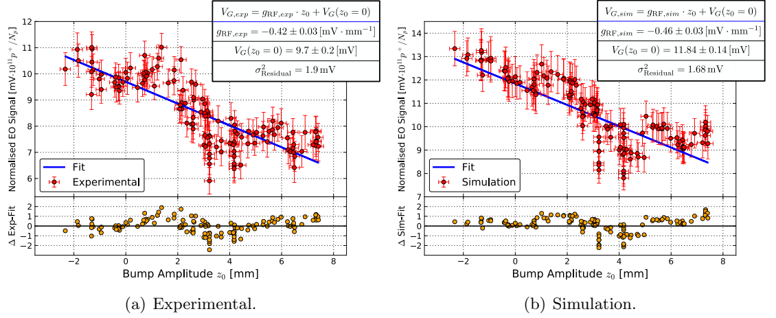
Figure 6.16: Experimental EO modulation peak V_G (a) compared to the expected simulation (b).
