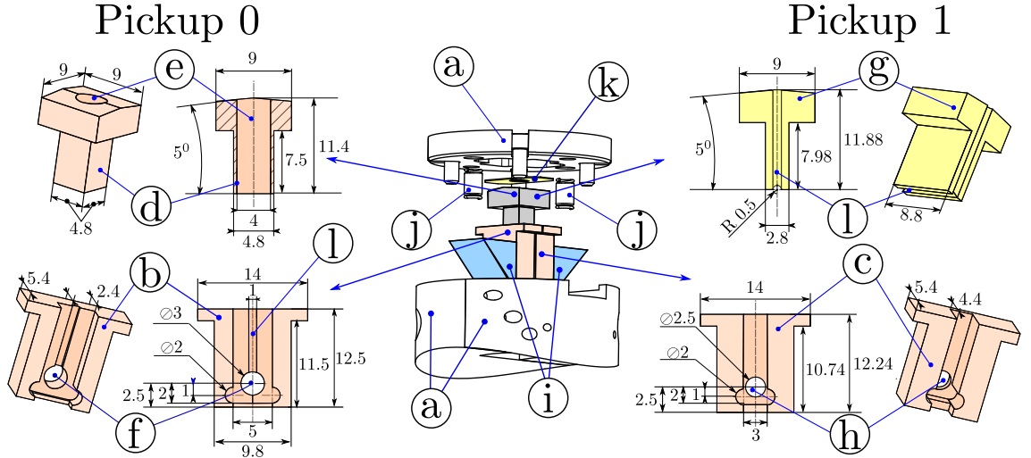
Figure 4.8: Assembly drawing of the ceramic holder and the button [56, 57].
