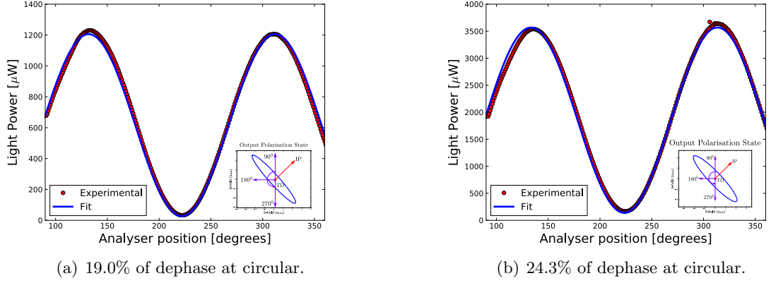
Figure 6.13: Polarisation output scan prior to the power increase by a factor 3 done just before the data-taking (a); after the experiment (b).
