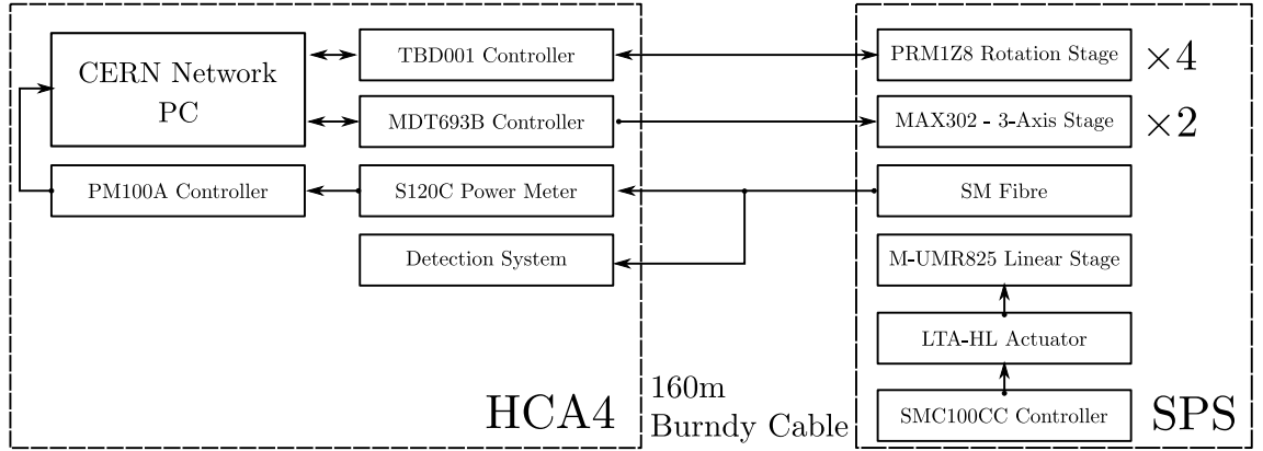
Figure 5.4: Flux diagram of the control instrumentation.
