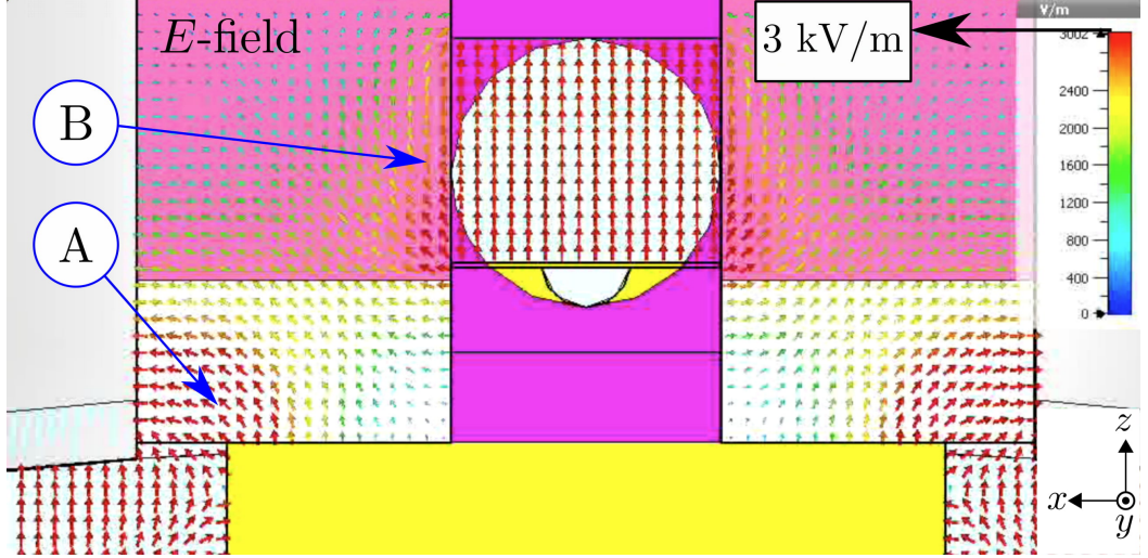
Figure 4.20: Vector field map produced by CST over the crystal section XZ at y = 0 for pickup one. The instant corresponds to the peak field at r_0 = 68.5 mm. The field goes through a shorter path A towards the grounded pipe and through B due to the lower dielectric constant of Macor.
