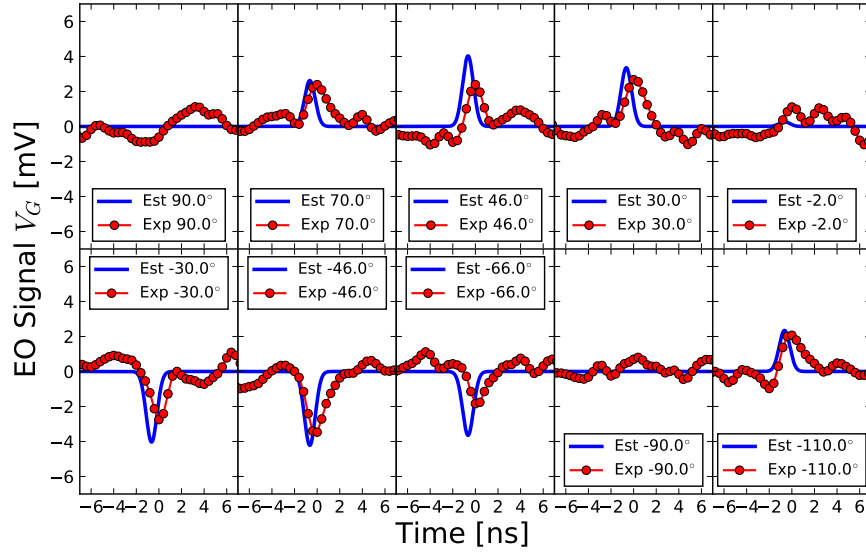
(c) EO Signal acquisition at different relevant analyser positions.
