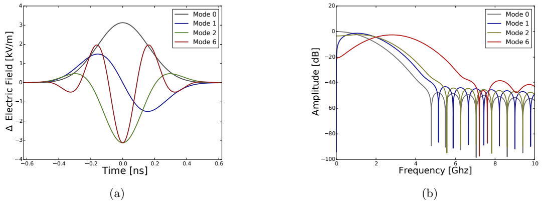
Figure 1.3: Typical HT signals for modes 0, 1, 2, and 6 in the time-domain (a) and the corresponding frequency bandwidth (b).
