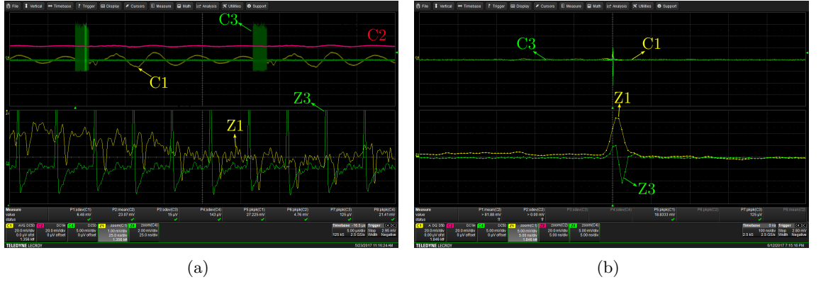
Figure 6.10: Oscilloscope display of the EO signal (C1 and amplified Z1) with a button reference signal (C3 and amplified Z3) for a bunch of trains (a) and AWAKE beam (b).
