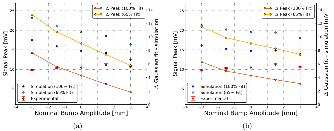
Figure 6.24: (a) Experimental and simulated signal maximum as a function of the bump amplitude, and the difference between them both for the perfect Gaussian fit (100%) and the 65% reduction in bunch length; (b) Peak signal scaled accordingly assuming a constant bunch length of 2.88 ns.
