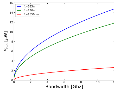
Figure 5.12: Noise Equivalent Power (NEP) against frequency bandwidth.
