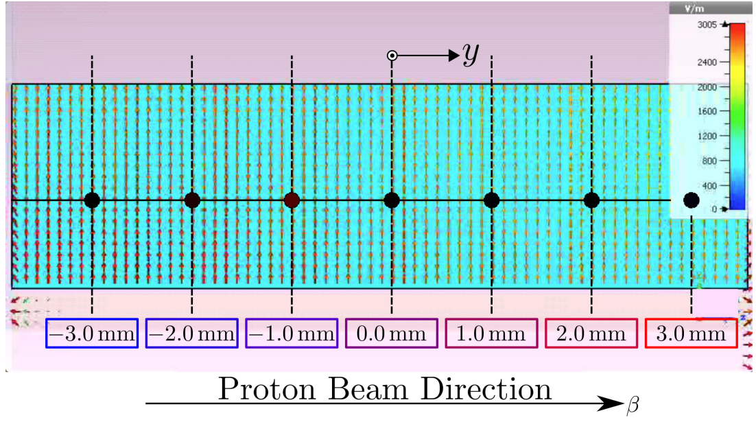
Figure 4.28: Vector map of the modulating field over the longitudinal section of the crystal for HT mode 8.
