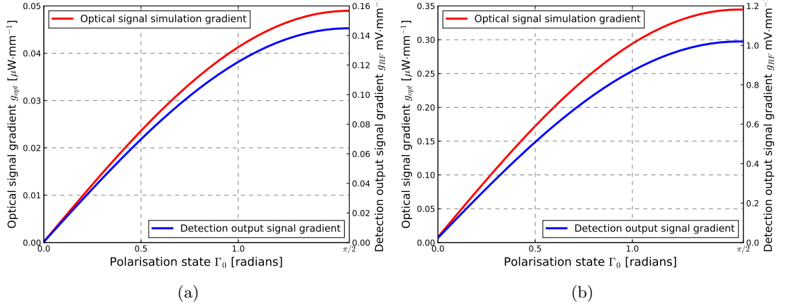
Figure 5.19: Gradients of the optical signal g_{opt} and the output detection system g_G as a function of the polarisation estate \Gamma_0 for pickup variants zero (a) and one (b).
