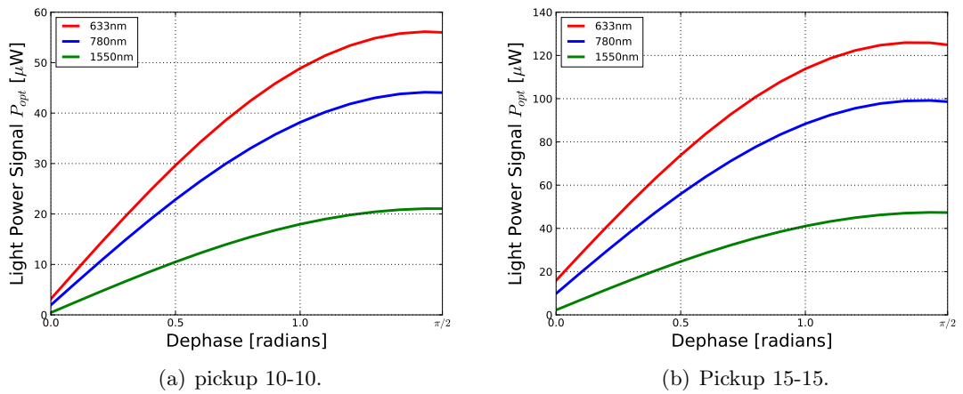
Figure 7.1: Optical signal as a function of the output polarisation for pickups 10-10 (a) and 15-15 (b).
