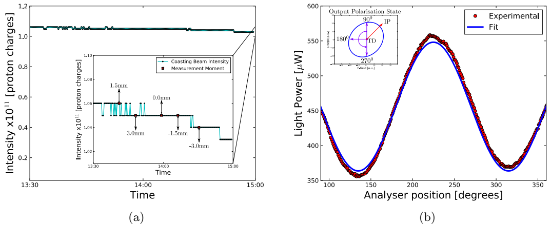
Figure 6.22: Beam intensity drift with time (a) and polarisation scan (b) for the high intensity coast beam measurements.
