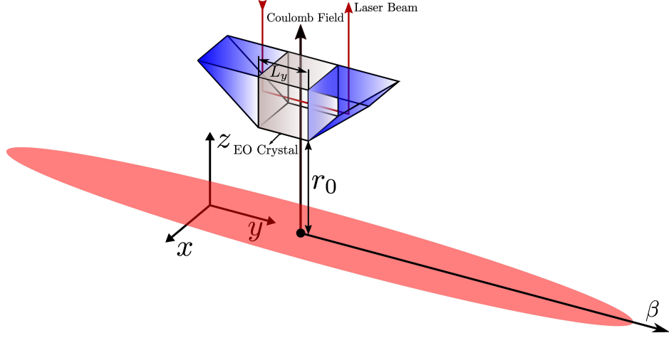
Figure 3.7: Interaction between the Coulomb field of the passing bunch and the conceptual EO pickup.
