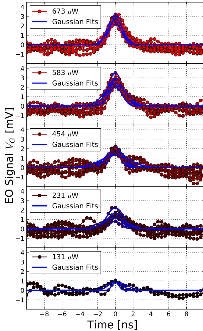
Figure 6.8: Experimental signal at different laser input power values with the baseline subtracted.
