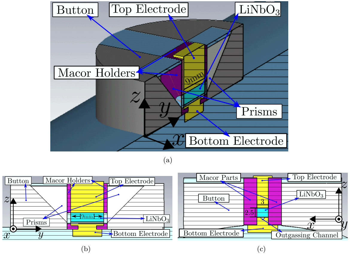
Figure 4.18: Screenshots of different views of pickup one in the CST user interface.
