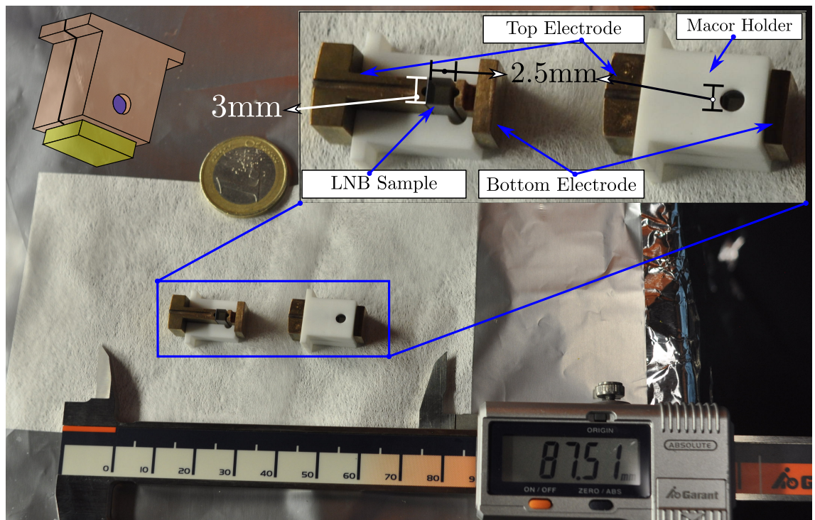
(b) Detail of the electrodes, ceramic holder and crystal for pickup one.
