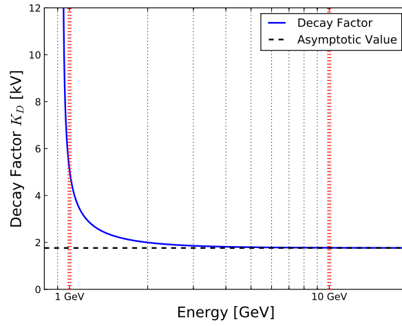
Figure 3.5: Decay factor K_D as a function of energy for a nominal SPS bunch.
