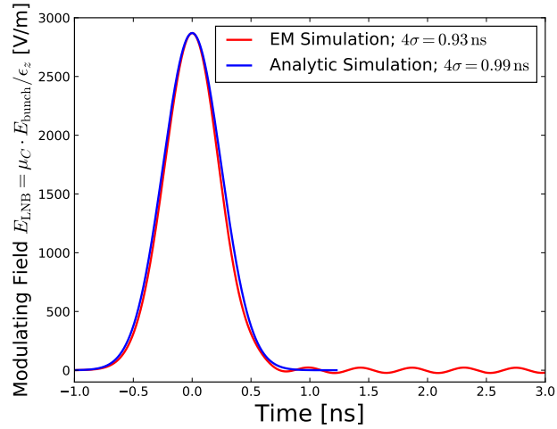
Figure 4.21: Modulating field time-profile curve inside the LNB sample for pickup one.
