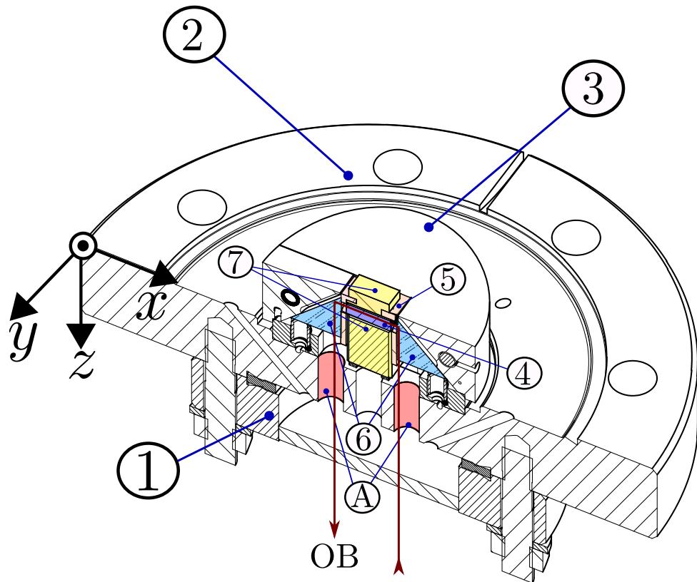
Figure 4.7: Assembly drawing of the pickup one (all the units are in millimetres) [55].
