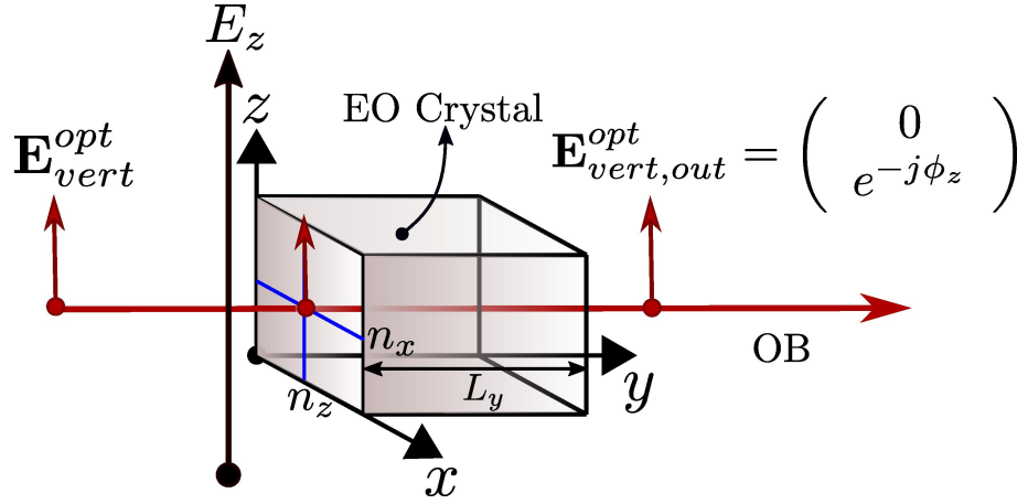
Figure 2.8: Phase modulator configuration where the input and output polarisation states are parallel to the z direction.
