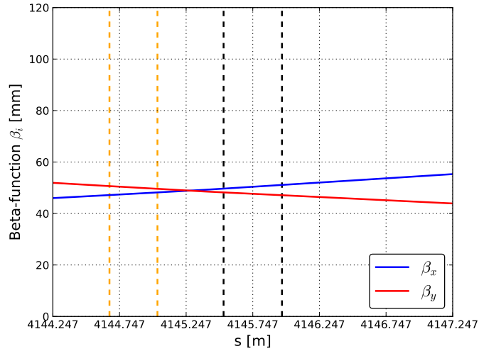
Figure 1.7: Zoomed in section of the lattice around the position of the EO-BPM and HT monitor.
