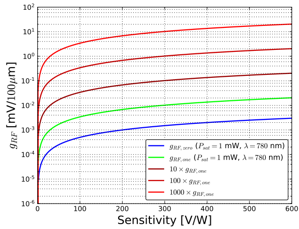
Figure 7.3: Isogradient curve for g_{RF} = 1 \text{ mV}/100\mu\text{m} at 780 nm, with P_{sat} = 1 \text{ mW} .
