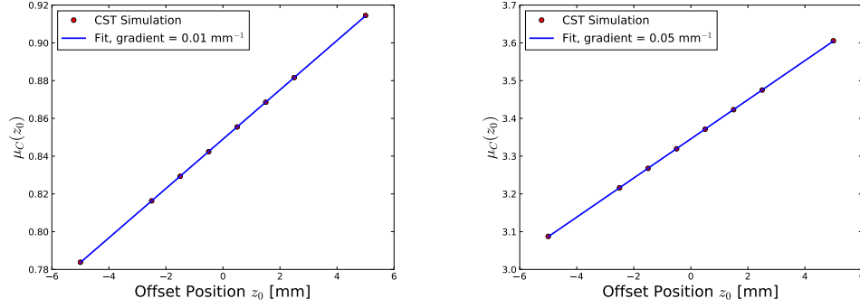
(a) \mu_C(z_0) at r_{\text{centre}} = 68.0 mm for pickup zero. (b) \mu_C(z_0) at r_{\text{centre}} = 68.5 mm for pickup one.
