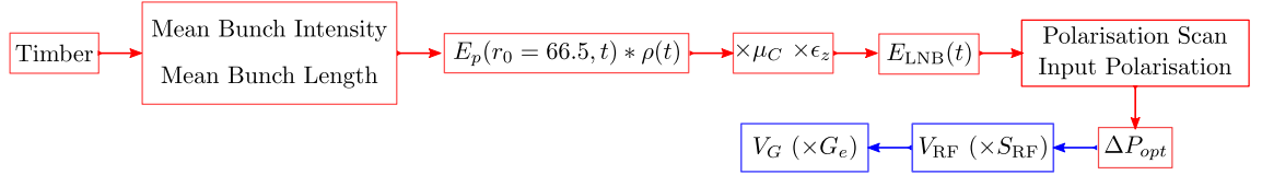
Figure 6.2: Flow diagram of the algorithm to calculate the EO signal estimation.
