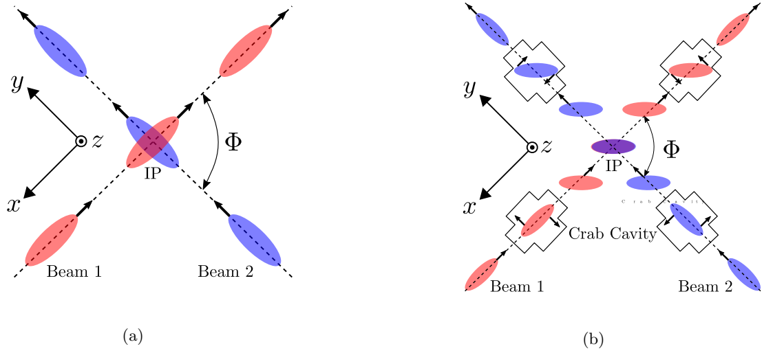
Figure 1.2: Diagrams of the current collision geometry (a), and the crab cavity mechanism (b): the bunch is rotated before the Interaction Point IP to orient the bunches head-on and is kicked back to the original position afterwards.
