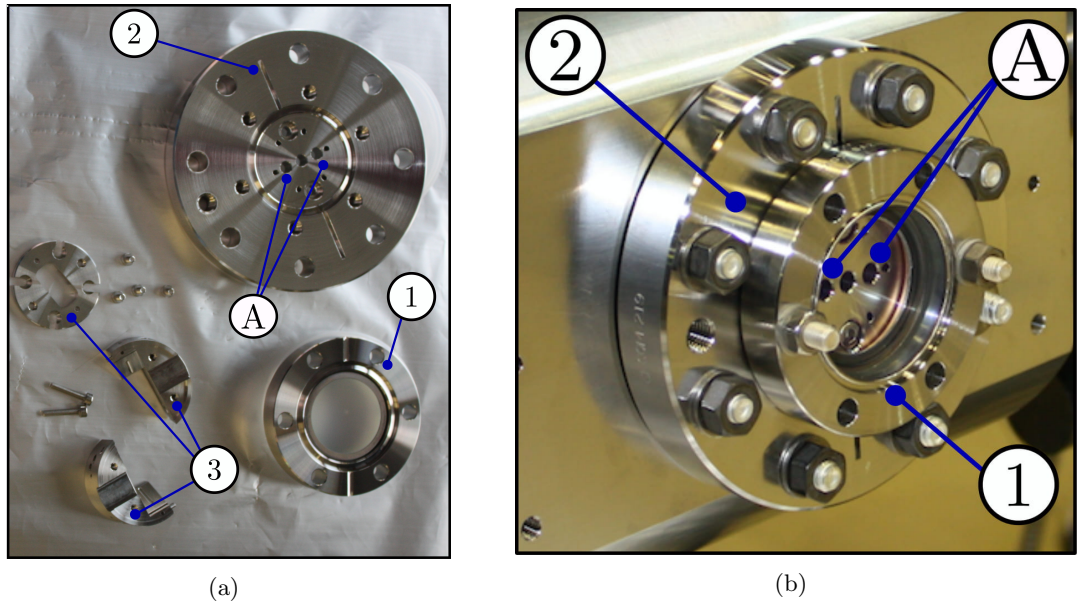
Figure 4.3: (a) Button pieces, central flange and viewport; (b) EO pickup mounted in the horizontal plane of the SPS pipe.
