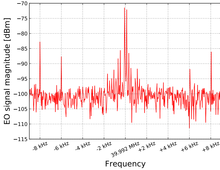
Figure 6.21: Frequency spectrum of the EO pickup signal around the 922^{\text{nd}} harmonic of the SPS revolution frequency.
