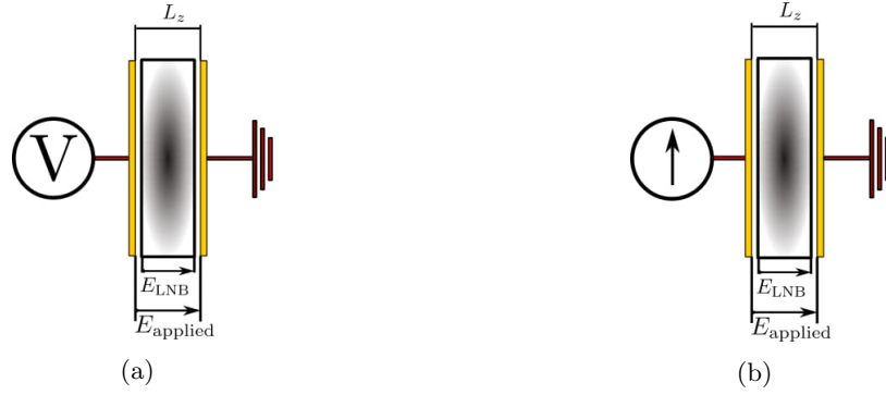
Figure 4.2: Equivalent circuits for (a) an optical modulator and (b) a EO pickup.
