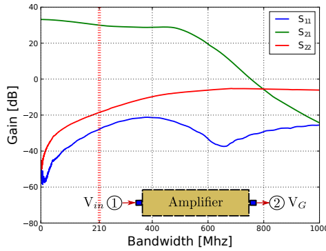
Figure 5.13: S-parameters against frequency for the external amplifier [67].
