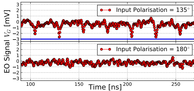
Figure 6.11: The train of signals disappears when the input polarisation is at 180^\circ .
