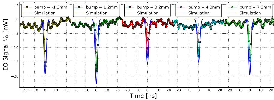
Figure 6.15: Set of experimental EO signals compared to the expected simulation for different orbit bump amplitudes. The offset bump value does not follow the signal amplitude as the beam conditions were different in each measurement.
