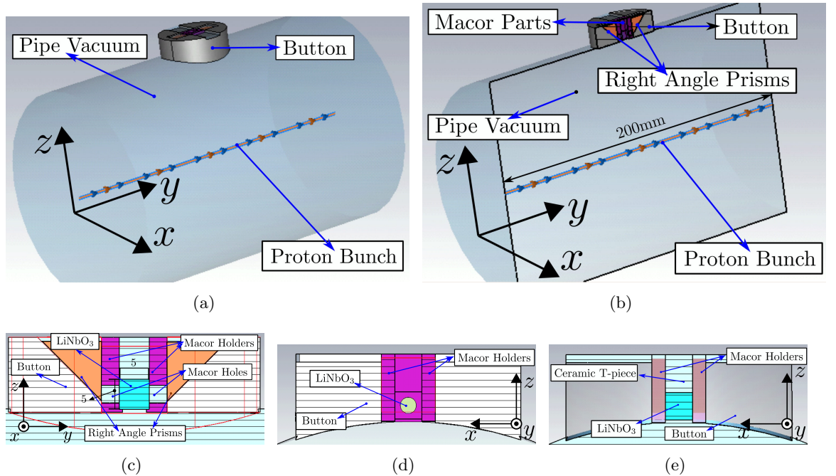
Figure 4.14: Screenshots of different views of pickup zero in the CST user interface.
