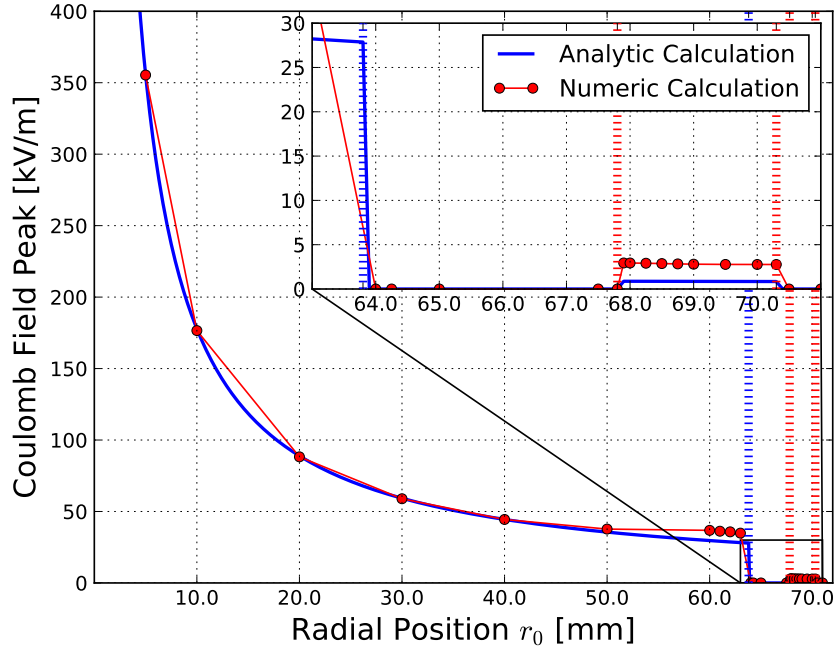
Figure 4.19: Numerical electromagnetic and analytic simulations of the peak Coulomb field along the radial transverse position r_0 over the pipe section for pickup one.
