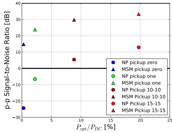
Figure 7.2: SNR_{p-p} comparison between the prototype acquisition system (NP) and MSM detector.
