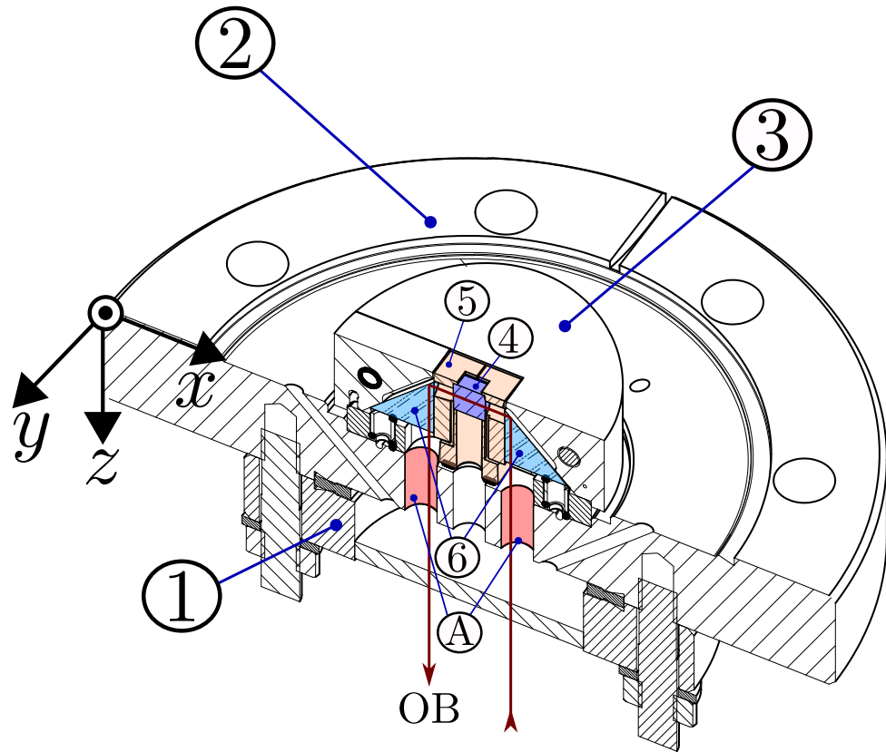
Figure 4.6: Assembly drawing of the pickup zero (all the units are in millimetres) [54].
