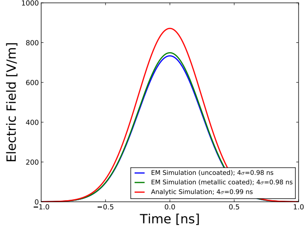
Figure 4.17: Coulomb field time-profile curve inside the LNB sample for pickup zero ( r_0 = 68.0 mm).
