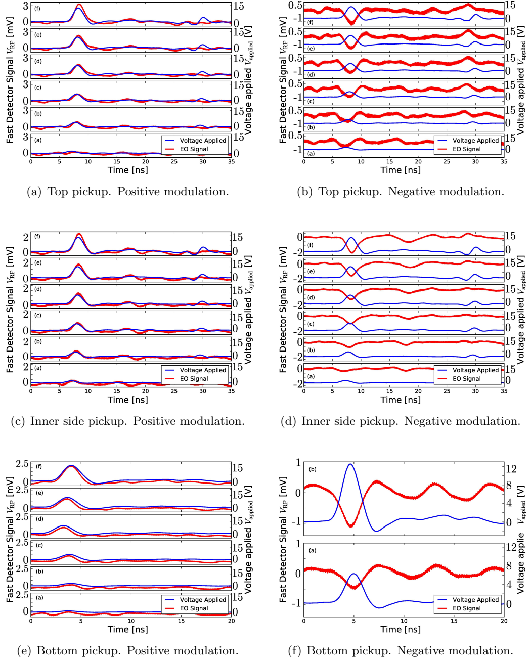
Figure 5.21: Averaged EO modulation when a fast voltage signal is applied on the electrodes of pickup one. The data recorded for Figure (f) only covered to 20 ns scope.
