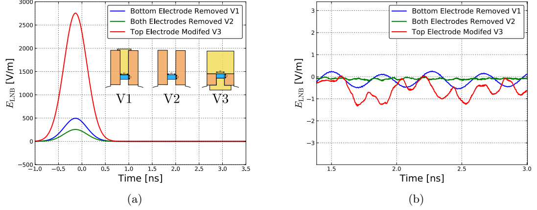
Figure 4.27: Modulating field for different modifications of pickup one: (a) standard single pickup signal; (b) zoomed in depiction of the resonance.
