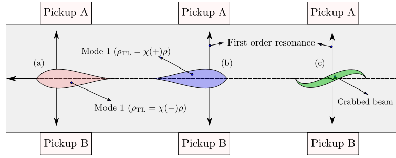
Figure 4.23: Diagram of the resonance mechanism.
