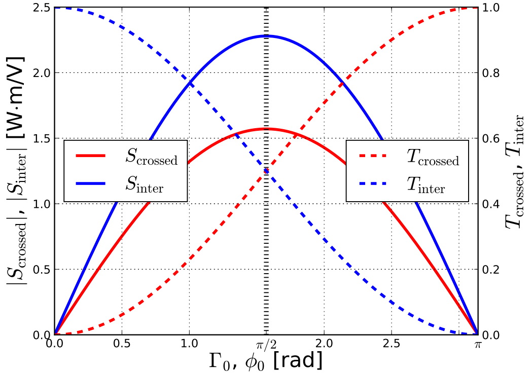
Figure 2.11: Sensitivity and transfer function versus the initial offset phase differences \Gamma_0 and \phi_0 for the amplitude and interferometric modulator.
