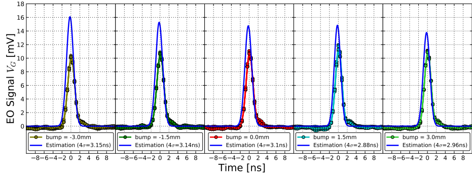
(a) Experimental measurements for each nominal bump amplitude in comparison with the prediction when assuming the bunch length obtained directly from the signal fit.
