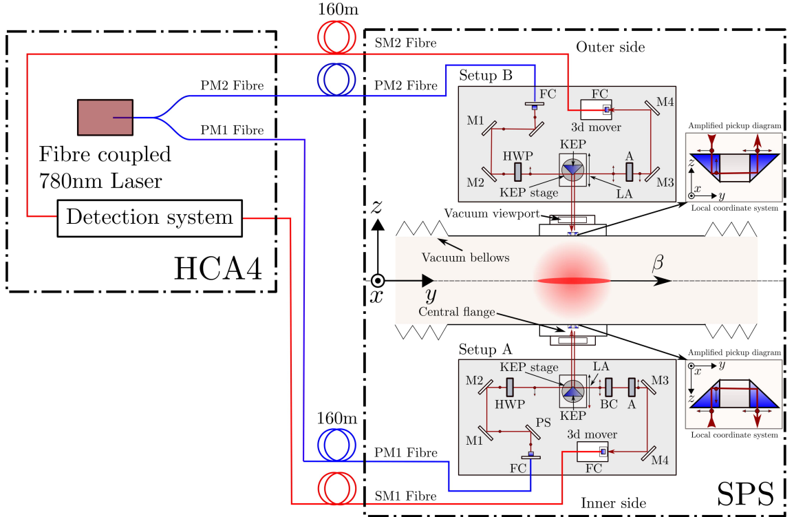
Figure 5.1: Layout of the optical setup for the EO-BPM experiment.
