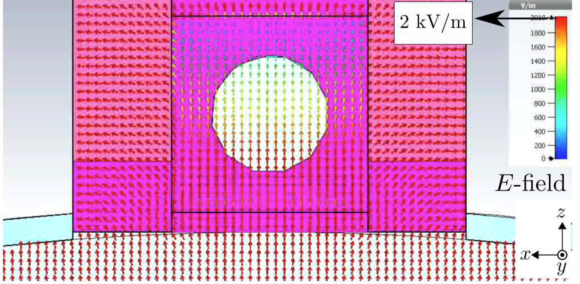
Figure 4.16: Vector field map produced by CST over the crystal section XZ at y = 0 for pickup zero. The instant corresponds to the peak field at r_0 = 68.0 mm.
