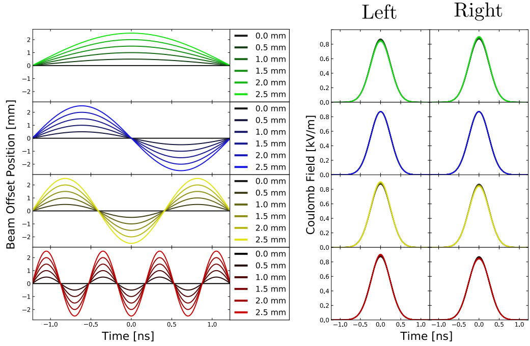
(a) Representation of the HT instabilities of modes 0, 1, 2 and 6. (b) Modulating field inside a LNB crystal located at 30 mm from the beam.
