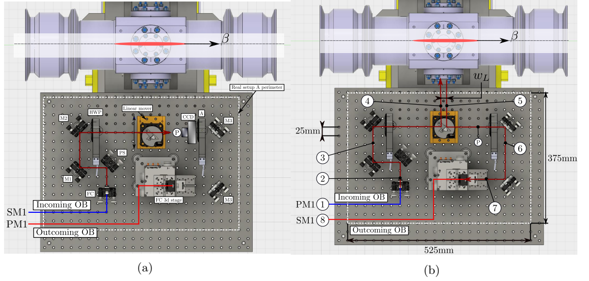
Figure 5.3: Example of the OB trajectory when the knife-edge prism is retracted (a) and placed in the final position (b) for setup A.
