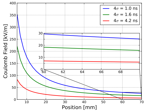
Figure 3.6: Coulomb field peak as a function of the transverse radial distance r_0 .
