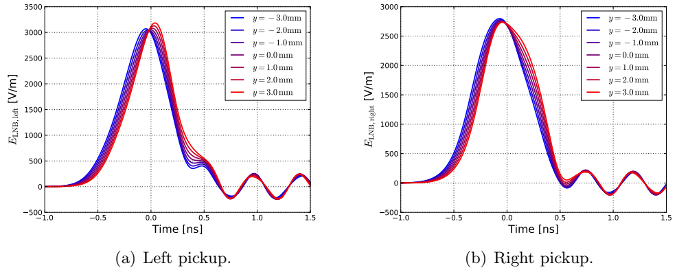
Figure 4.29: Modulating field in opposing pickups for mode 8 at different positions over the y axis for pickup one.
