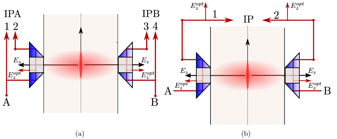
Figure 3.10: Concept of the optical layout for the interferometric design with (a) two different IP in the same plane and (b) with a single interferometric IP per plane outside the pipe.
