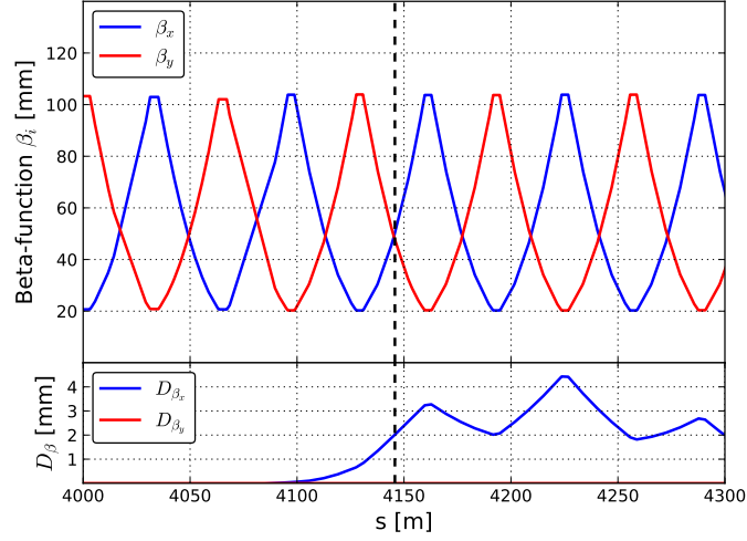
Figure 1.6: SPS lattice represented by the beta function projections \beta_x and \beta_y against s , and their dispersion values D_{\beta_x} and D_{\beta_y} , respectively.
