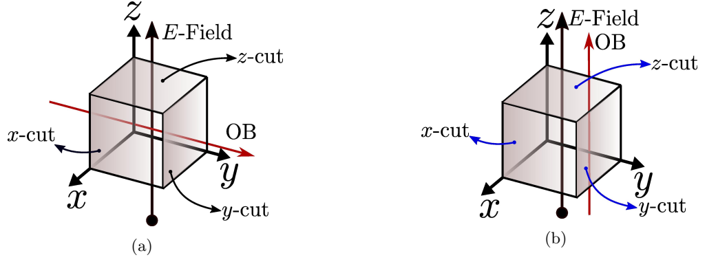
Figure 2.3: (a) Transverse modulation and (b) Longitudinal modulation geometries.
