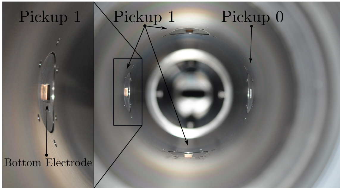
Figure 4.13: Buttons one and zero from inside the pipe.
