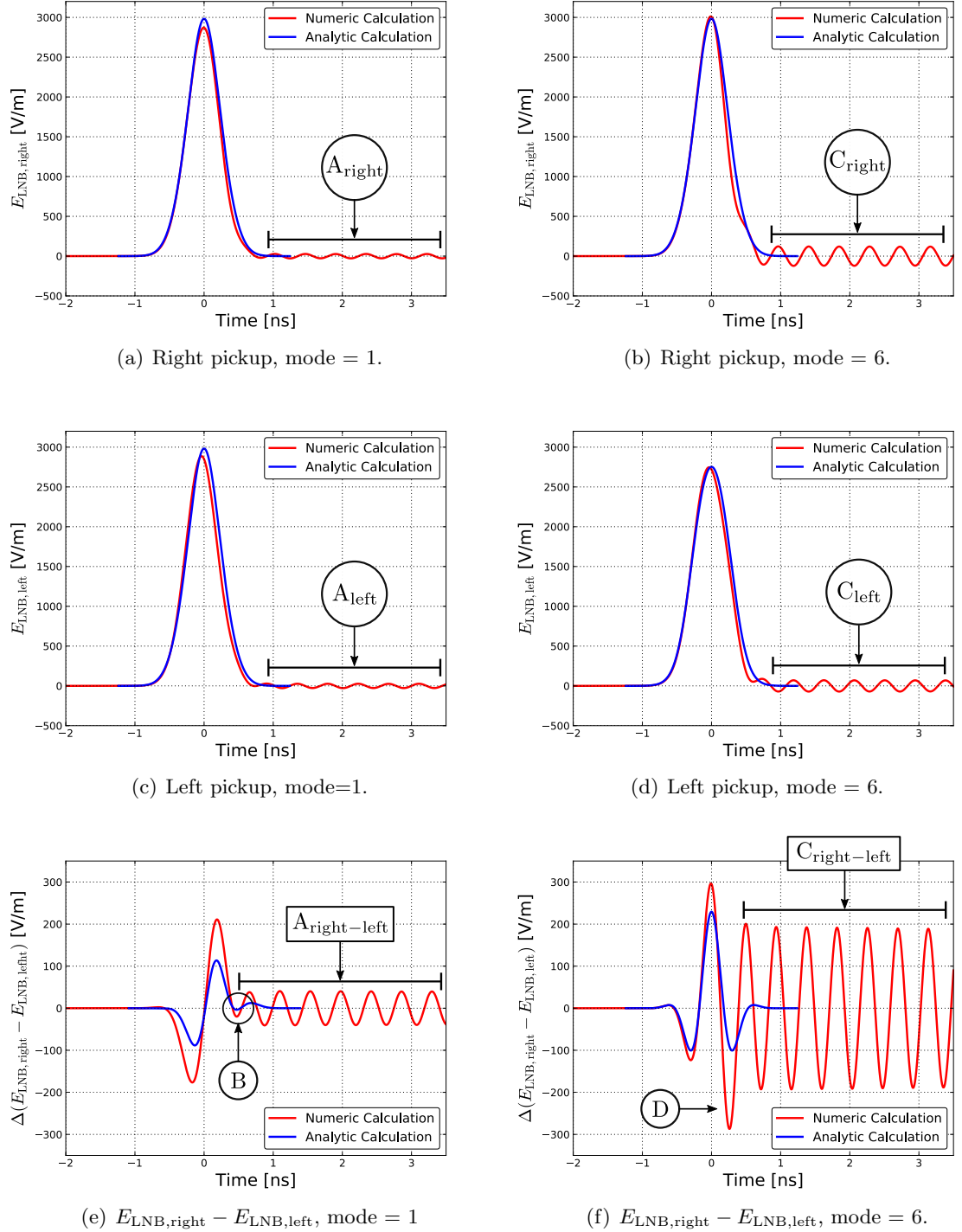
Figure 4.22: Comparison between the numeric and analytic simulations of HT instability modes 1 and 6, both of 3 mm amplitude.
