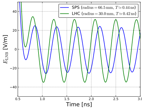
Figure 4.25: Resonances of the rigid mode for a pickup one installed in the LHC (30 mm) and the SPS (66.5 mm).
