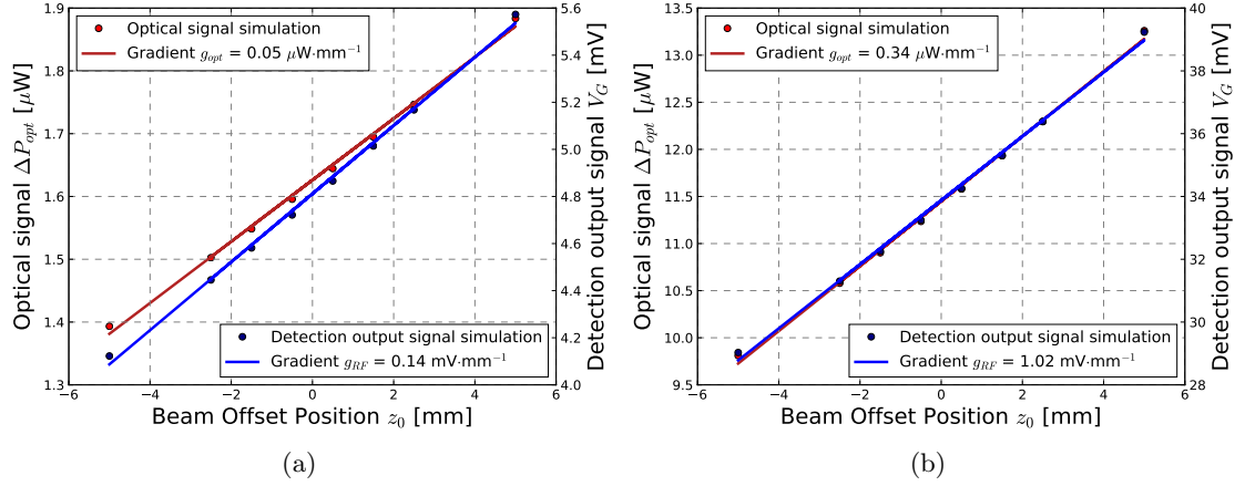
Figure 5.18: Gradients of the optical signal g_{opt} and the output detection system g_G as a function of the position for (a) pickup zero and (b) pickup one when the output polarisation estate is circular ( \Gamma_0 = \pi/2 ).
