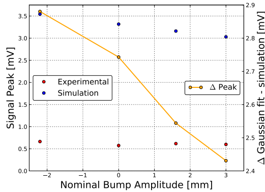
Figure 6.20: Analysis of the experimental and simulated peak signals related to the low intensity coast beam acquisition.
