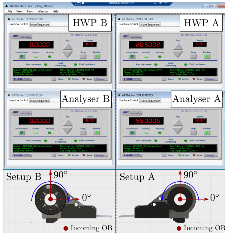
(a) Panel interface of the APT software associated with the remote stages controlling the HWP and analyser; on the left, for setup B, the rotation stage is depicted with the incoming beam direction and the corresponding control panels; on the right, equivalently, for setup A.
