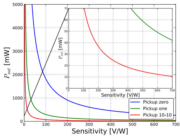
Figure 7.4: Isogradient curves for g_{RF} = 1 \text{ mV}/100\mu\text{m} at 780 nm.
