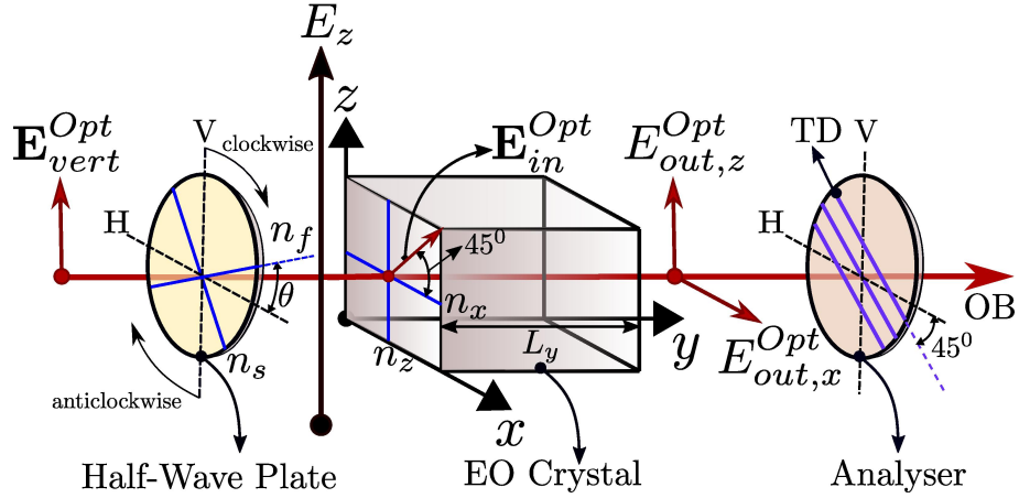
Figure 2.5: Amplitude modulation diagram.
