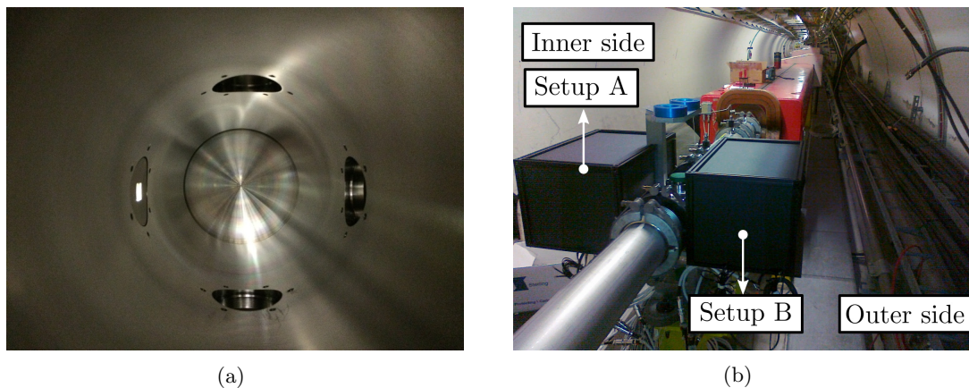
Figure 5.8: Picture inside the pipe with a single button installed next to setup A (a); the whole arrangement with the enclosed setups on the horizontal plane (b).
