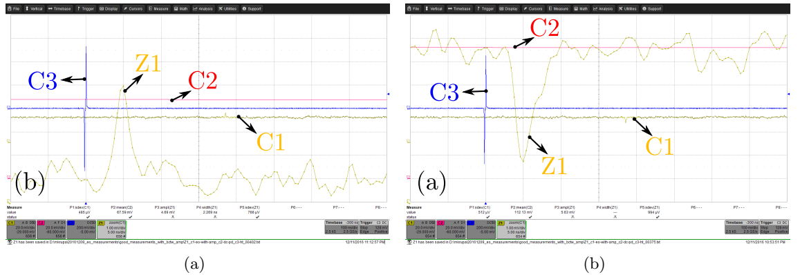
Figure 6.3: Example of the oscilloscope display appearance for a negative (a) and a positive (b) bunch-induced EO signal.
