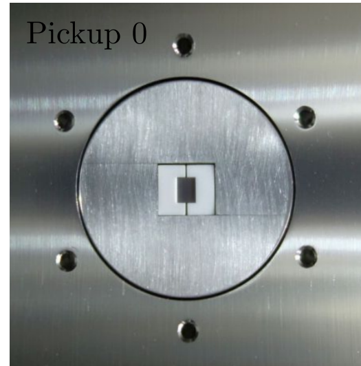
Figure 4.12: Button zero from inside the pipe.
