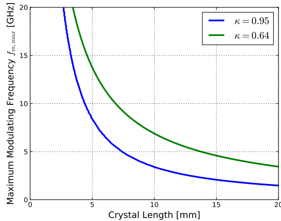
Figure 2.21: Maximum modulating frequency as a function of the crystal length L_y in the linear ( \kappa = 0.95 ) and maximum modulation ( \kappa = 0.64 ) regimes for LNB with n_e = 2.18 .
