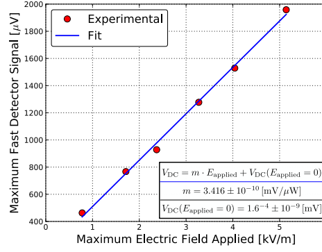
Figure 5.23: Maximum EO signal as a function of the field applied resulted from the characterisation of the inner side EO pickup one for positive signals.
