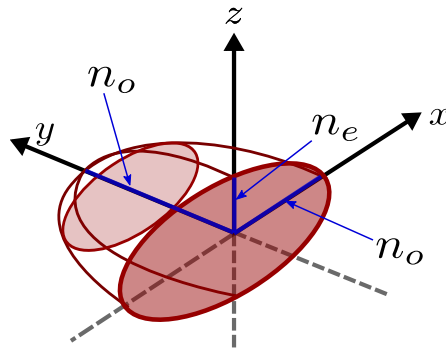
Figure 2.1: Section of the index ellipsoid on the y -cut (shaded) plane when the optical beam is propagating along the y axis. The ellipsoid axes are shown in blue: n_o is the refractive index along x and y , and n_e along z .
