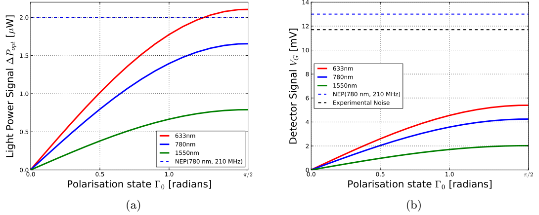
Figure 5.16: Optical power signal \Delta P_{opt} (a) and detection signal voltage (b) as a function of the output polarisation, for the 5 mm cubic crystal in pickup zero modulated by 750 V/m electric field that corresponds to the SPS nominal bunch. The NEP at 780 nm and the experimental noise are also calculated.
