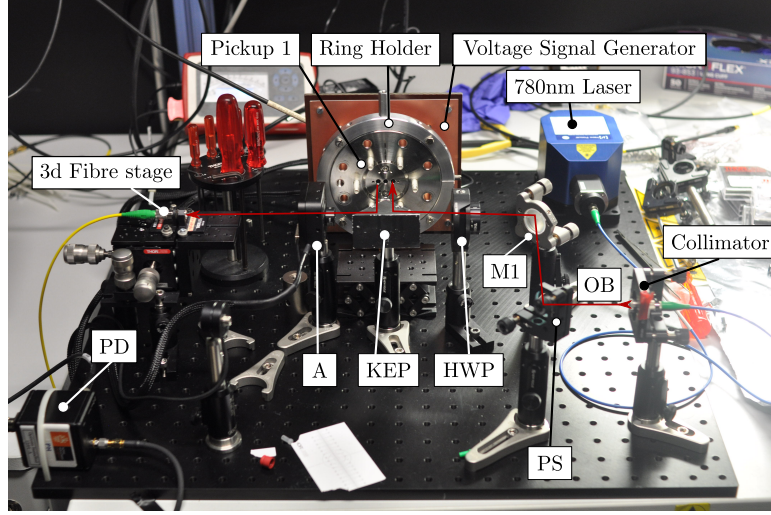
Figure 5.20: Pickup one characterisation setup.
