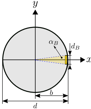
Figure D.1: Diagram illustrating the coverage angle \alpha_B for a traditional button pickup.
