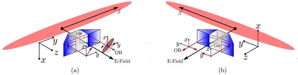
Figure 3.9: Conceptual designs for (a) a crossed polarisers pickup and (b) a phase modulator pickup.
