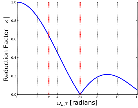
Figure 2.18: Reduction factor \kappa as a function of \omega_m\tau .
