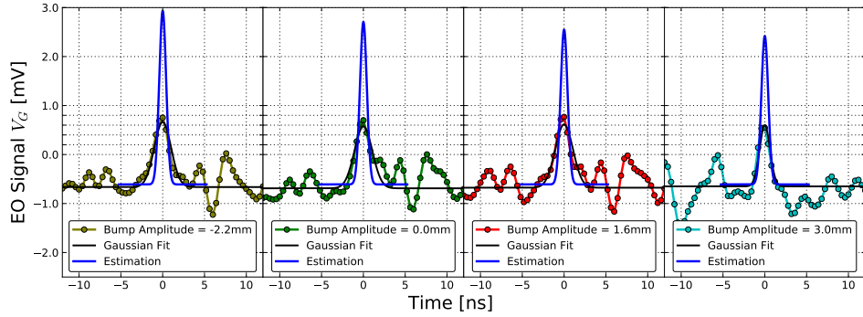
Figure 6.19: Set of experimental EO signals compared to the expected simulation for the low-intensity coast beam conditions.
