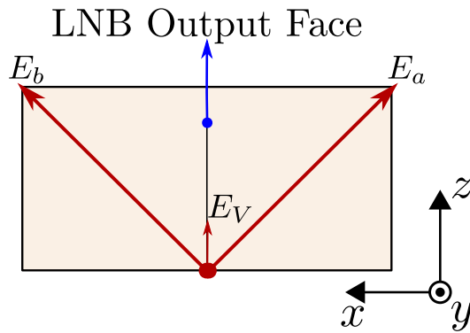
Figure 2.17: Diagram of the output face of lithium niobate along with the elliptical axes projections of the polarisation state oriented at 45^\circ and -45^\circ .
