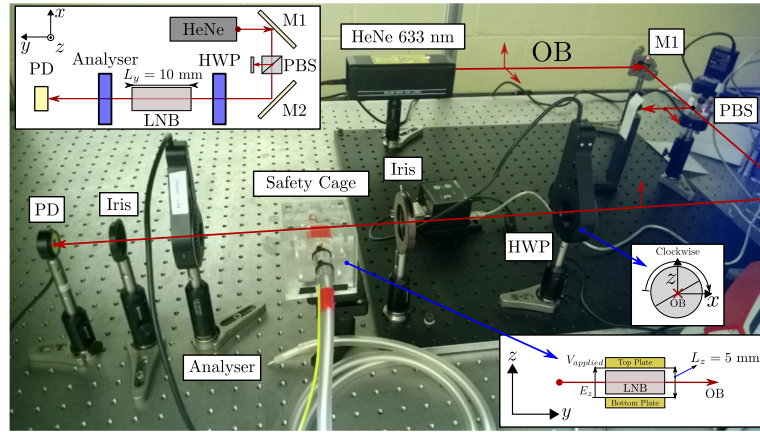
Figure 2.13: Experimental electro-optic characterisation setup.
