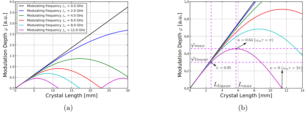
Figure 2.20: (a) Modulation depth against crystal length for the extraordinary refractive index n_e ; (b) zoomed in amplification until 14 mm with labels to mark the linear and maximum modulation regimes for the case f_m = 12 GHz.
