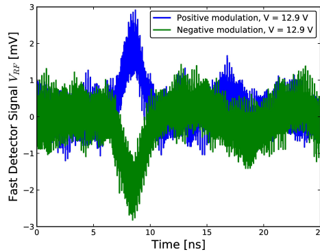
Figure 5.24: EO modulation acquisition at single shot taken during the characterisation for pickup one installed on the inner side adjacent to the setup A.
