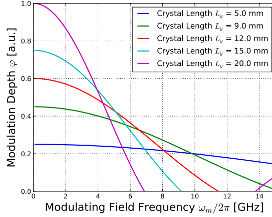
Figure 2.19: Modulation depth against frequency of the modulating field for the extraordinary refractive index n_e .
