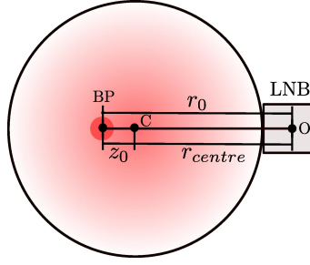
Figure 4.32: Diagram with the main geometrical parameters in the gradient calculation: BP is the beam position; C is the centre of the pipe; O is the crystal position.
