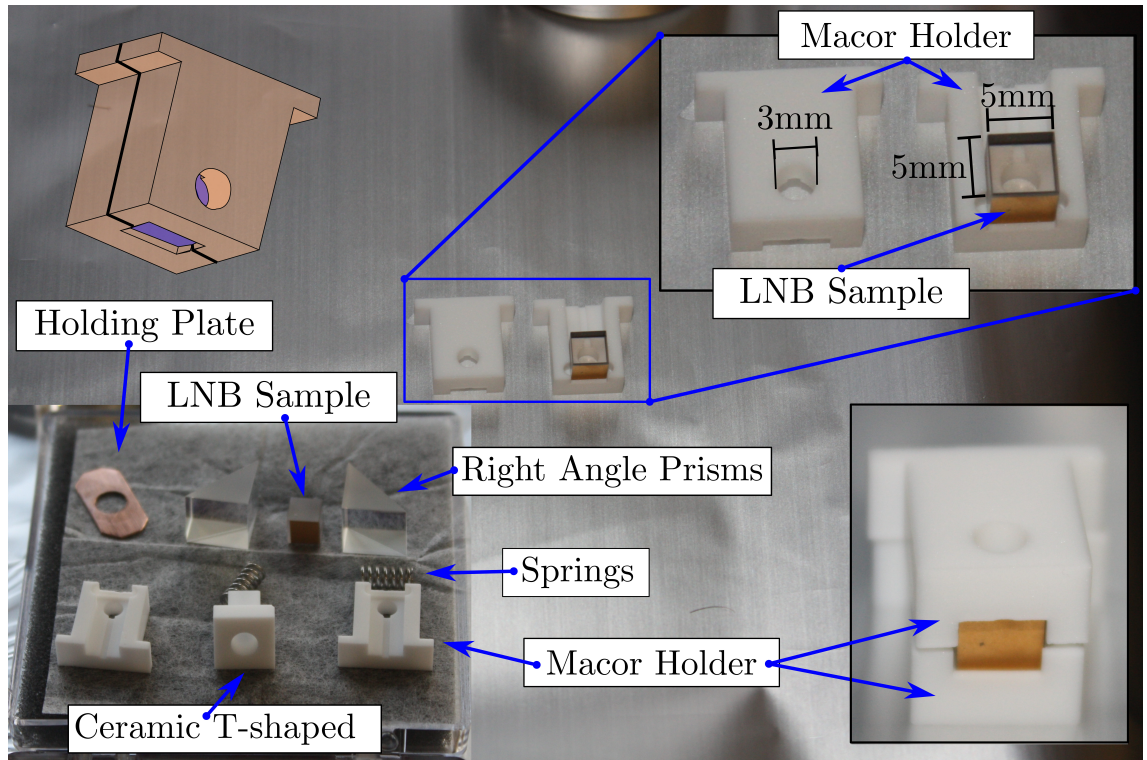
(a) Detail of the ceramic pieces, prisms, springs and crystal for pickup zero.
