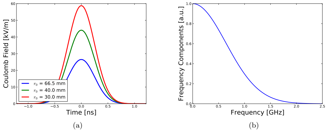
Figure 3.2: (a) Time profile and (b) frequency spectrum for a rigid mode bunch with the nominal SPS parameters.
