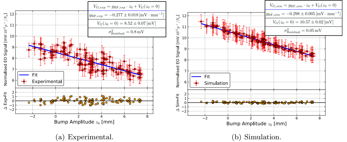
Figure 6.17: Experimental EO modulation peak V_G (a) compared to the expected simulation (b) when the sensitivity drift has been removed.
