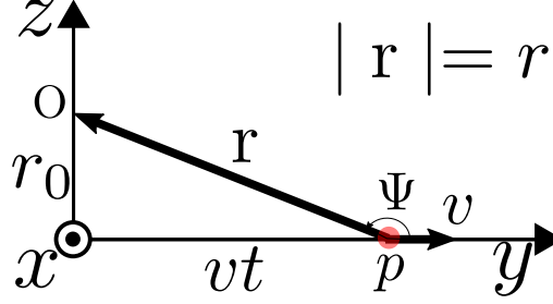
Figure 3.1: Relativistic proton diagram.
