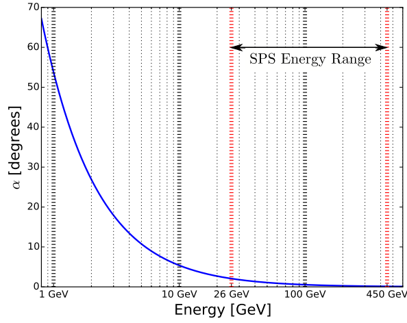
Figure 3.4: The angle \alpha subtended by the bunch Coulomb field as a function of proton energy. The SPS energy range covers from injection at 26 GeV up to 450 GeV.
