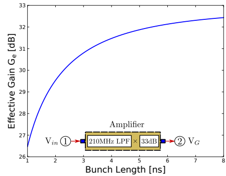
Figure 5.14: Effective gain for a simulated Gaussian bunch length signal.
