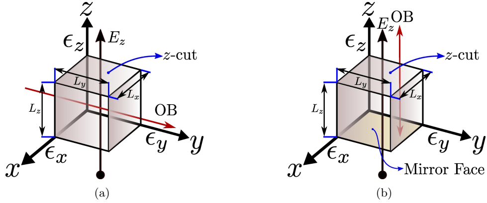
Figure 4.1: Orientation diagram of the LNB sample in the (a) transverse and (b) longitudinal configurations.
