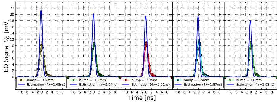
(b) Experimental measurements for each nominal bump amplitude in comparison with the prediction when the bunch length is shortened by 65% with respect the signal fit.
