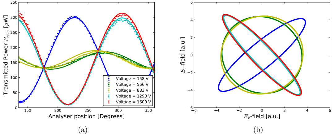
Figure 2.16: Experimental polarisation scans from 135^\circ (points) and fits (continuous curve) (a) of the different polarisation states (b).
