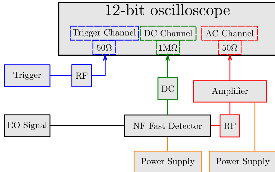
Figure 5.9: Detection scheme diagram.
