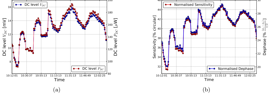
Figure 6.14: Optical P_{DC} and detector DC output V_{DC} drift during the data taking (a) and how that translates into the detection sensitivity as a function of the maximum point at circular polarisation (b).
