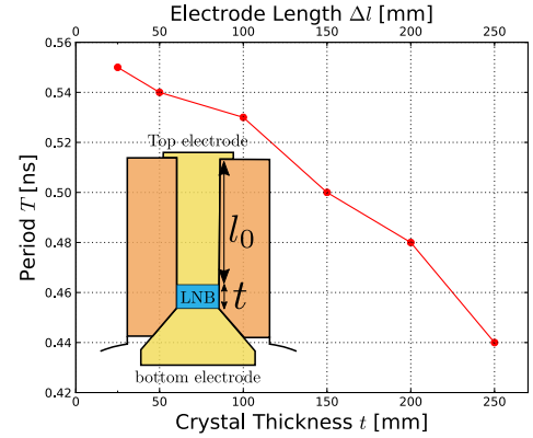
Figure 4.26: Period of the resonance at rigid mode against the crystal thickness.
