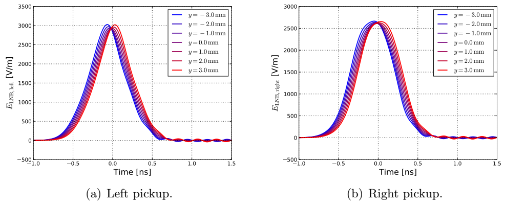
Figure 4.30: Modulating field in opposing pickups for mode 8 at different positions over the y axis for the modified pickup one, V3.
