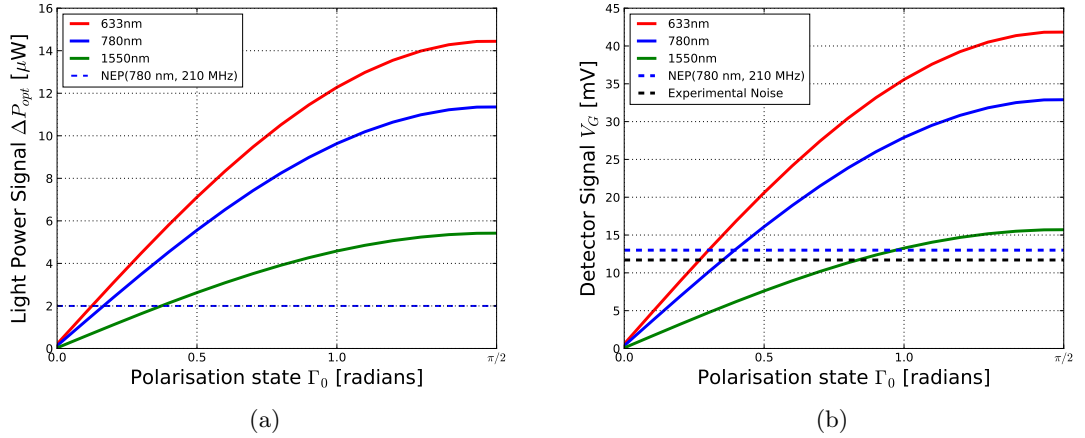
Figure 5.17: Optical power signal \Delta P_{opt} (a) and detection signal voltage (b) as a function of the output polarisation, for the 9 mm long crystal in pickup one modulated by 2.86 kV/m electric field that corresponds to the SPS nominal bunch. The NEP at 780 nm and the experimental noise are also calculated.
