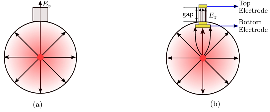
Figure 3.8: Concept designs for (a) the EO pickup with no electrode and (b) with electrode.
