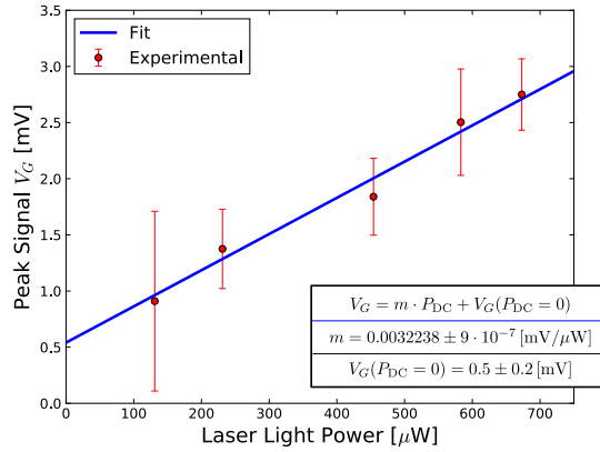
Figure 6.9: Linear relation between the EO peak signal against the input laser power.
