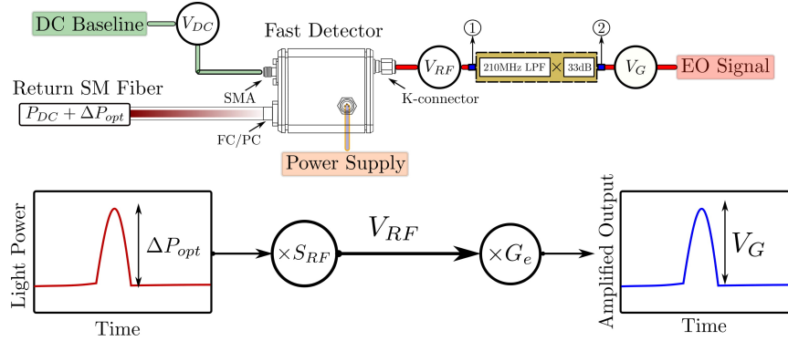
Figure 5.15: Detection chain diagram.
