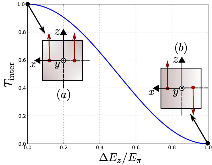
Figure 2.10: Transfer function (eqn. 2.37) for an interferometer phase modulation system from polarisation in phase (a) to anti-phase (b).
