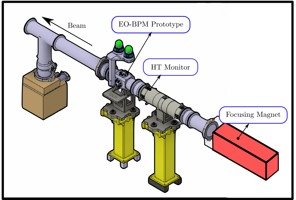
Figure 1.5: Representation of the section of the SPS ring where the EO-BPM was installed.
