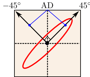
Figure 5.22: Diagram of the output face of the crystal sample with the possible positions of the analyser that lead to opposite sign modulations.
