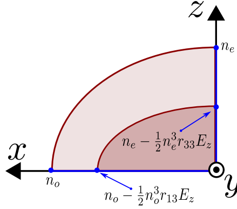
Figure 2.2: The index ellipsoid section with E = 0 occupies more surface (clearer) than when E \neq 0 (darker).
