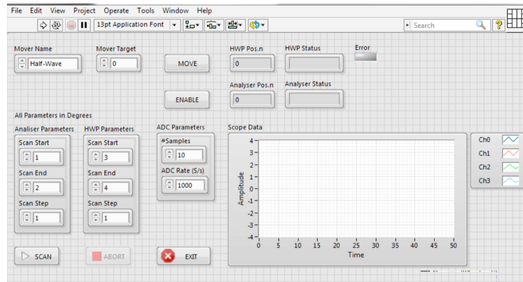
(b) LabVIEW control panel for measuring the crystal birefringence by acquiring polarisation scans.
