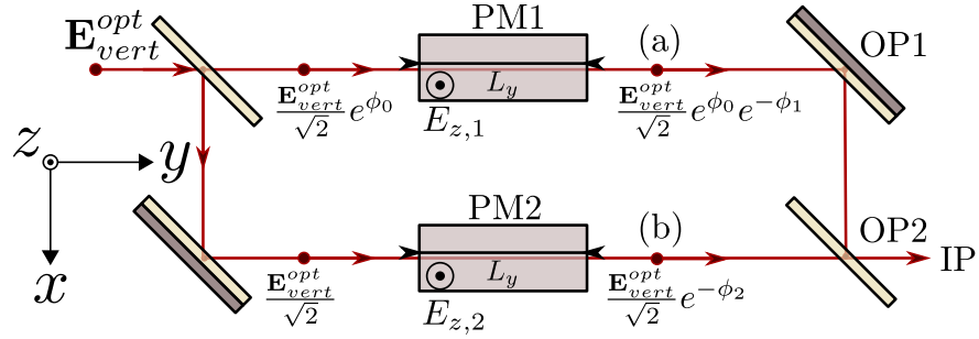
Figure 2.8: Phase modulator configuration where the input and output polarisation states are parallel to the z direction.
