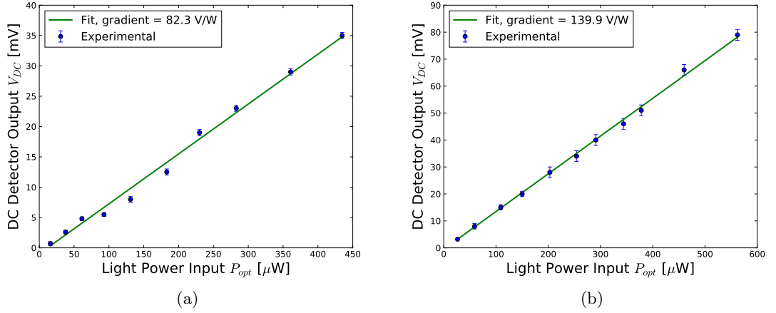
Figure 5.11: Fast detector DC calibration curve when the input fibre connection APC/PC (a) and PC/PC (b) for 780 nm.
