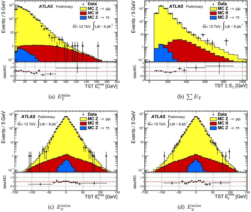
Figure 5.12: Distributions of TST E_T^{\text{miss}} (a), \sum E_T (b), E_x^{\text{miss}} (c), E_y^{\text{miss}} (d) in Z(\mu\mu) + \text{jets} events. The expectation from MC simulation is superimposed and normalized to data, after each MC sample is weighted with its corresponding cross-section.
