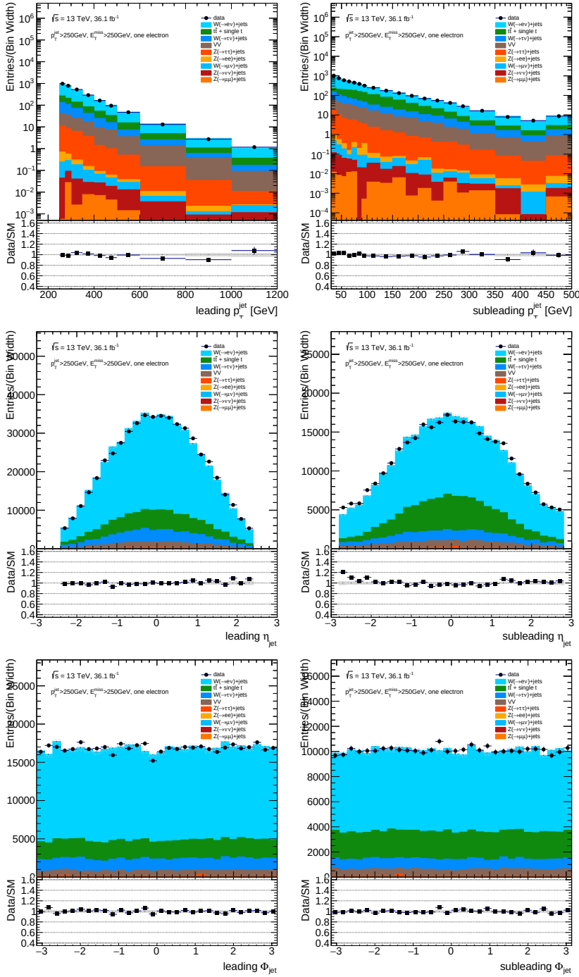
Figure 8.16: Pre-fit kinematic distributions in the CR1e. V + jets spectra are weighted to higher order corrections (see Section 8.2.3). The sum of the MC spectra are normalized to the total number of observed events in data. The error bands in the upper and lower panel include only the uncertainty due to limited MC statistics.
