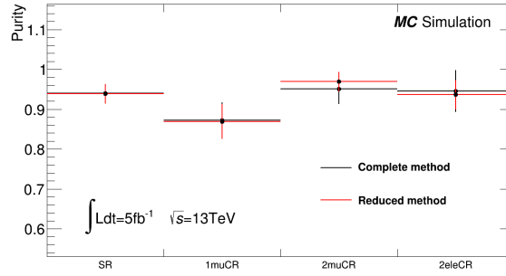
Figure 7.7: Photon purity evaluated with the complete and the reduced methods. For the reduced method, in the SR and in the \text{CR}\gamma\mu the r coefficient is obtained from the same regions; in the \text{CR}\gamma\mu\mu and \text{CR}\gamma ee the r coefficient is evaluated as the weighted mean from the SR and the \text{CR}\gamma\mu . Plot by collaborator.
