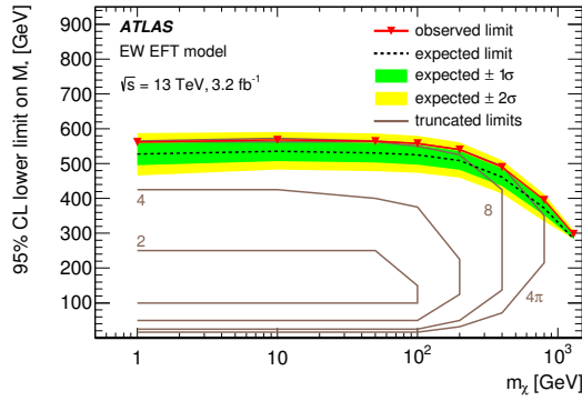
Figure 7.19: The observed and expected 95% CL limits on M_* for the EW EFT model with contact interaction of type \gamma\gamma\chi\chi as a function of dark matter mass m_\chi . Results where EFT truncation is applied are also shown, assuming representative coupling values of 2, 4, 8 and 4\pi .
