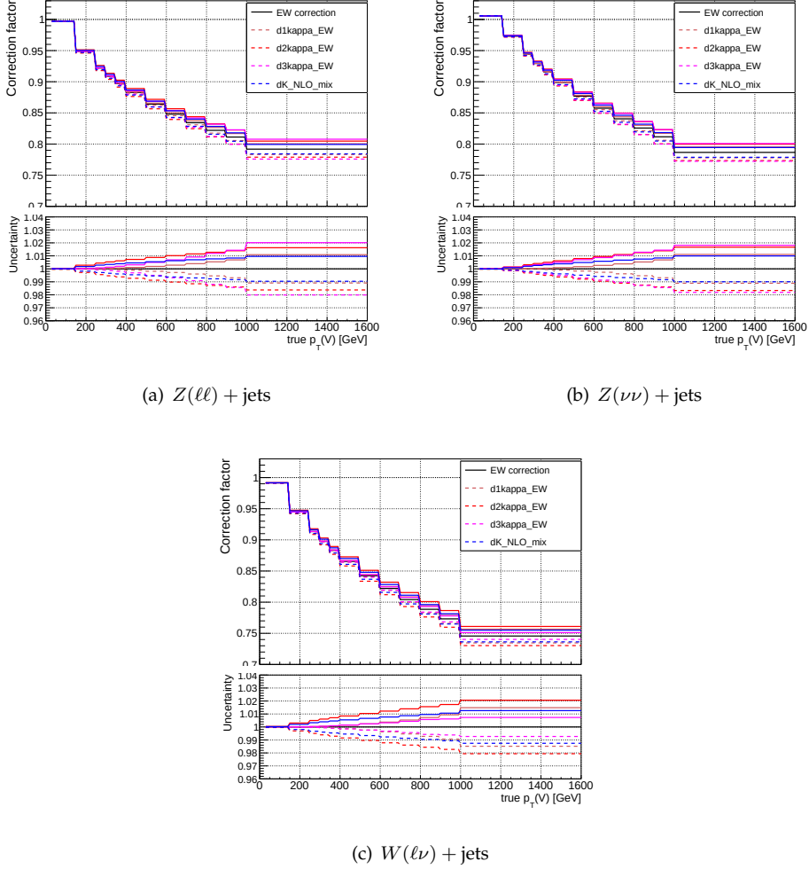
Figure 8.22: Electroweak correction for the Z(\ell\ell) + \text{jets} , Z(\nu\nu) + \text{jets} , W(\ell\nu) + \text{jets} processes with the corresponding uncertainties. For each variation, the ‘up’ effect is shown with a solid line, and the ‘down’ effect with a dashed line. The correction factor is shown on the top pad, while the ratios between the correction factor for any variation and the nominal one are shown in the bottom pad.
