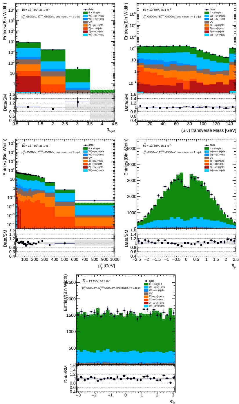
Figure 8.10: Pre-fit kinematic distributions in the CR1mulb. V + jets spectra are weighted to higher order corrections (see Section 8.2.3). The sum of the MC spectra are normalized to the total number of observed events in data. The error bands in the upper and lower panel include only the uncertainty due to limited MC statistics.
