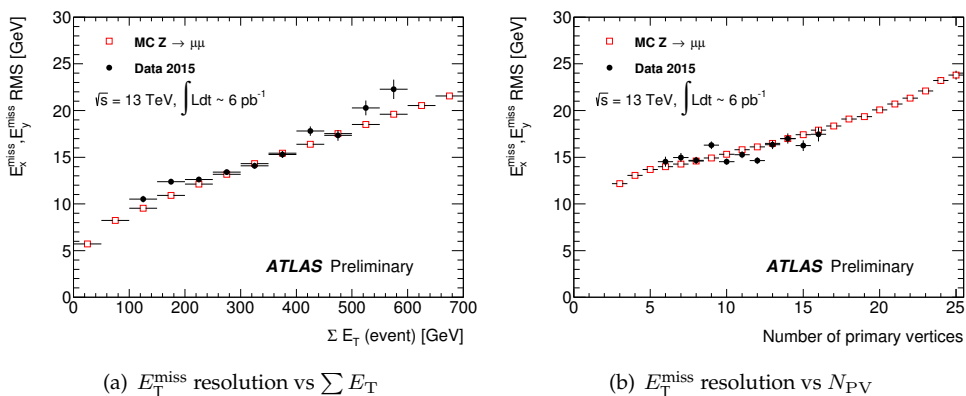
Figure 5.15: Distributions of TST E_x^{\text{miss}}, E_y^{\text{miss}} resolution as a function of \sum E_T and of the number of primary vertices in Z(\mu\mu) + jets events. The data (black circles) and MC simulation (red squares) are overlaid.
