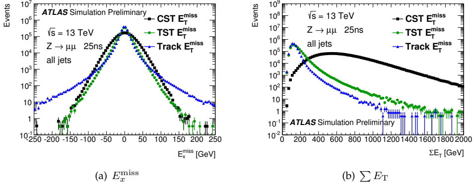
Figure 5.1: Distributions of (a) the x component of the total E_T^{\text{miss}} , and (b) the \Sigma E_T . These are shown for the TST E_T^{\text{miss}} , CST E_T^{\text{miss}} and Track E_T^{\text{miss}} definitions, using POWHEG+PYTHIA Z(\mu\mu) + jets simulated events.
