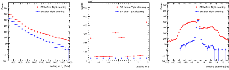
Figure 8.20: Leading jet p_T , \phi , and t_{\text{jet}} distributions in the signal region before and after tight jet cleaning. The distinctive \phi structure in the before-cleaning distribution is characteristic of NCB. Plots by collaborator.
