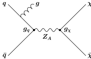
Figure 6.1: Leading order mono-jet process for the s – channel axial-vector model.
