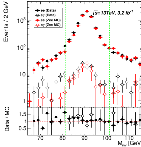
Figure 7.5: Invariant mass distribution of the tag-and-probe pair as measured in the data and in the Z(ee) + \text{jets} Monte Carlo samples, for electron and photon probes. A mass window of 10 GeV around the Z mass is used to evaluate the fake rate. Plot by collaborator.
