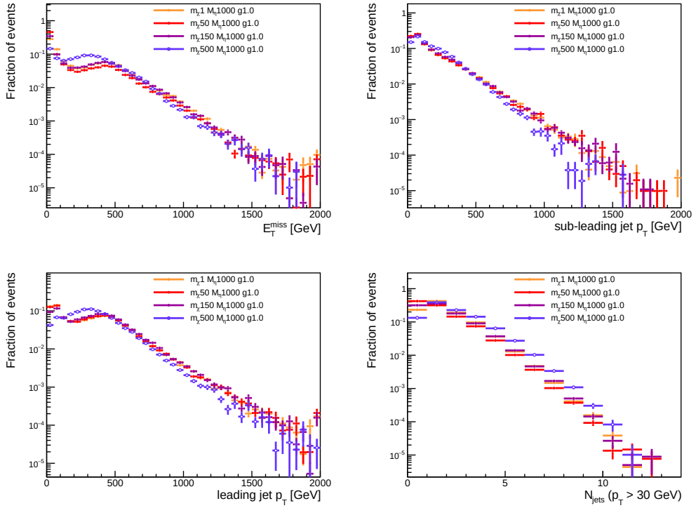
Figure 6.10: E_T^{\text{miss}} , leading jet p_T , sub-leading jet p_T , and jet multiplicity distributions of the combined sample for M_\eta = 1000 \text{ GeV} , g = 1 , and several values of m_\chi . Spectra are normalized to unity.
