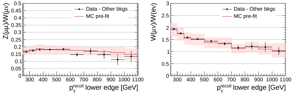
Figure 8.27: Comparison between data and reweighted MC simulation of Z(\mu\mu) + \text{jets} in CR2 \mu and W(\mu\nu) + \text{jets} in CR1 \mu 0b (left) and of W(\mu\nu) + \text{jets} in CR1 \mu 0b and W(e\nu) + \text{jets} in CR1e (right) before the simultaneous fit. Uncertainty bands on the MC distributions include statistical and systematic components.
