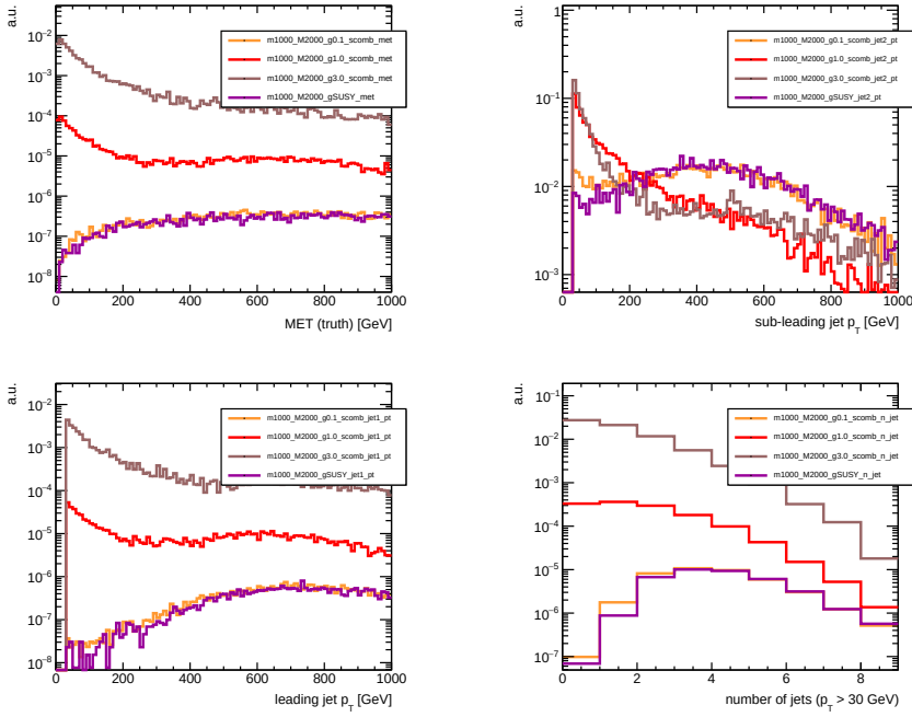
Figure A.11: E_T^{\text{miss}} , leading jet p_T , sub-leading jet p_T , and jet multiplicity distributions for m_\chi = 1000 GeV, M_\eta = 2000 GeV. The distributions for the t – channel model with several couplings ( g = 0.1 in orange, g = 1.0 in red, g = 3.0 in grey) are compared to the distribution for the SUSY model (purple). Spectra are normalized to their cross-section.
