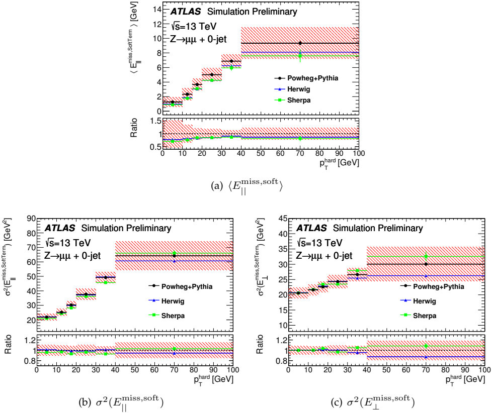
Figure 5.18: RMS and mean of the E_T^{\text{miss,soft}} projected into components longitudinal and transverse to \mathbf{p}_T^{\text{hard}} in Z(\mu\mu) + \text{jets } 0\text{-jet} events. Points are shown for POWHEG+PYTHIA (nominal), HERWIG and SHERPA generators. The shaded band shows the effect of the TST systematic uncertainties with contributions from the difference of generators, the change in detector geometry and the variation in bunch spacing.
