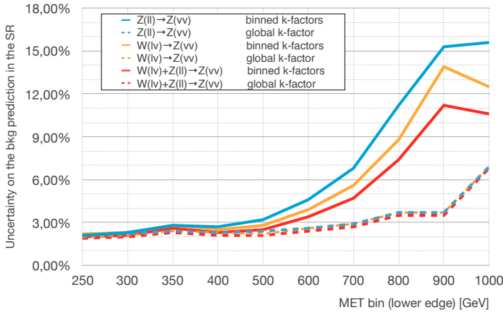
Figure 8.26: The relative estimated uncertainty on the background prediction in each E_T^{\text{miss}} bin of the SR as obtained from several fitting strategies. The fits are performed with Asimov datasets. The fit configurations are described in the text.
