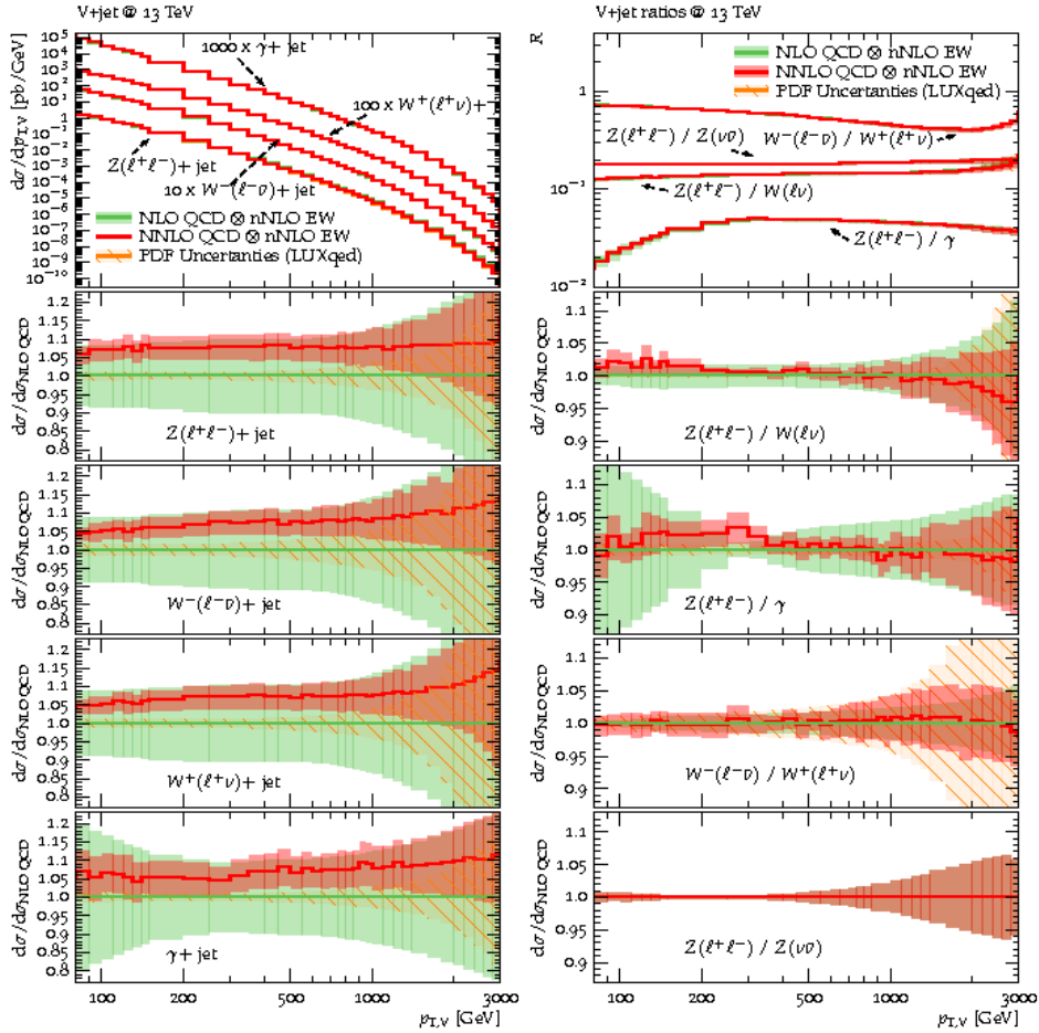
Figure 8.1: Predictions at NLO QCD⊗nNLO EW and NNLO QCD⊗nNLO EW for V + \text{jets} spectra (left) and ratios (right) at 13 TeV. The lower frames show the relative impact of NNLO corrections and theory uncertainties normalized to NLO QCD⊗nNLO EW. The green bands at NLO QCD⊗nNLO EW correspond to the combination (in quadrature) of the perturbative QCD, EW and mixed QCD-EW uncertainties, while the NNLO QCD⊗nNLO EW bands (red) display only QCD scale variations. PDF uncertainties are shown as separate hashed orange bands. From [140]. Note that the version of the calculations available for the mono-jet analysis does not include NNLO QCD predictions and PDF uncertainties, as they were not available.
