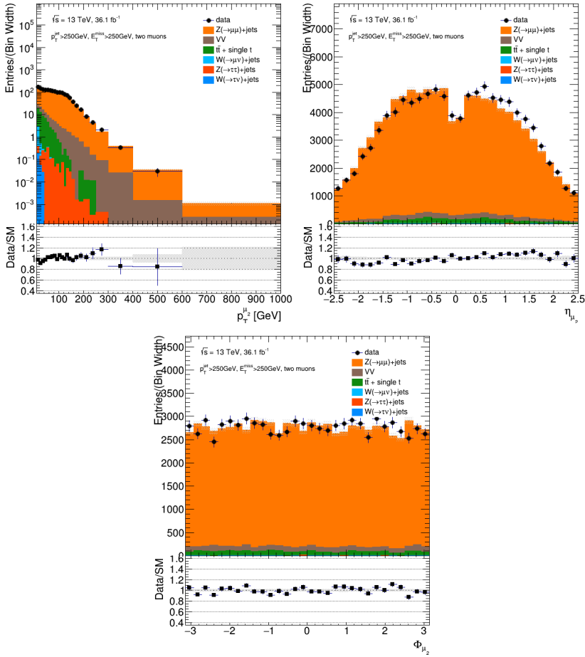
Figure 8.14: Pre-fit kinematic distributions in the CR2mu. V + jets spectra are weighted to higher order corrections (see Section 8.2.3). The sum of the MC spectra are normalized to the total number of observed events in data. The error bands in the upper and lower panel include only the uncertainty due to limited MC statistics.
