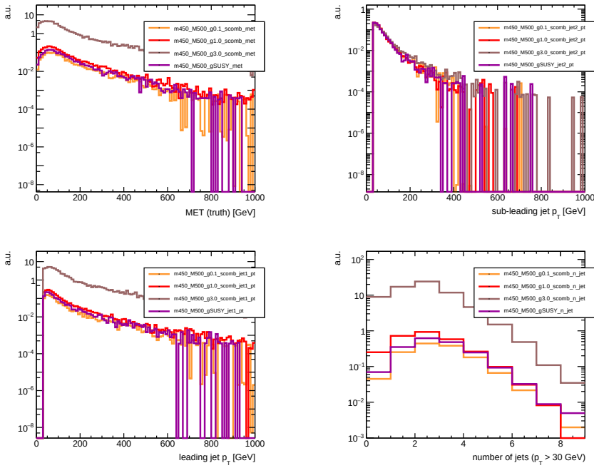
Figure A.10: E_T^{\text{miss}} , leading jet p_T , sub-leading jet p_T , and jet multiplicity distributions for m_\chi = 450 GeV, M_\eta = 500 GeV. The distributions for the t - \text{channel} model with several couplings ( g = 0.1 in orange, g = 1.0 in red, g = 3.0 in grey) are compared to the distribution for the SUSY model (purple). Spectra are normalized to their cross-section.
