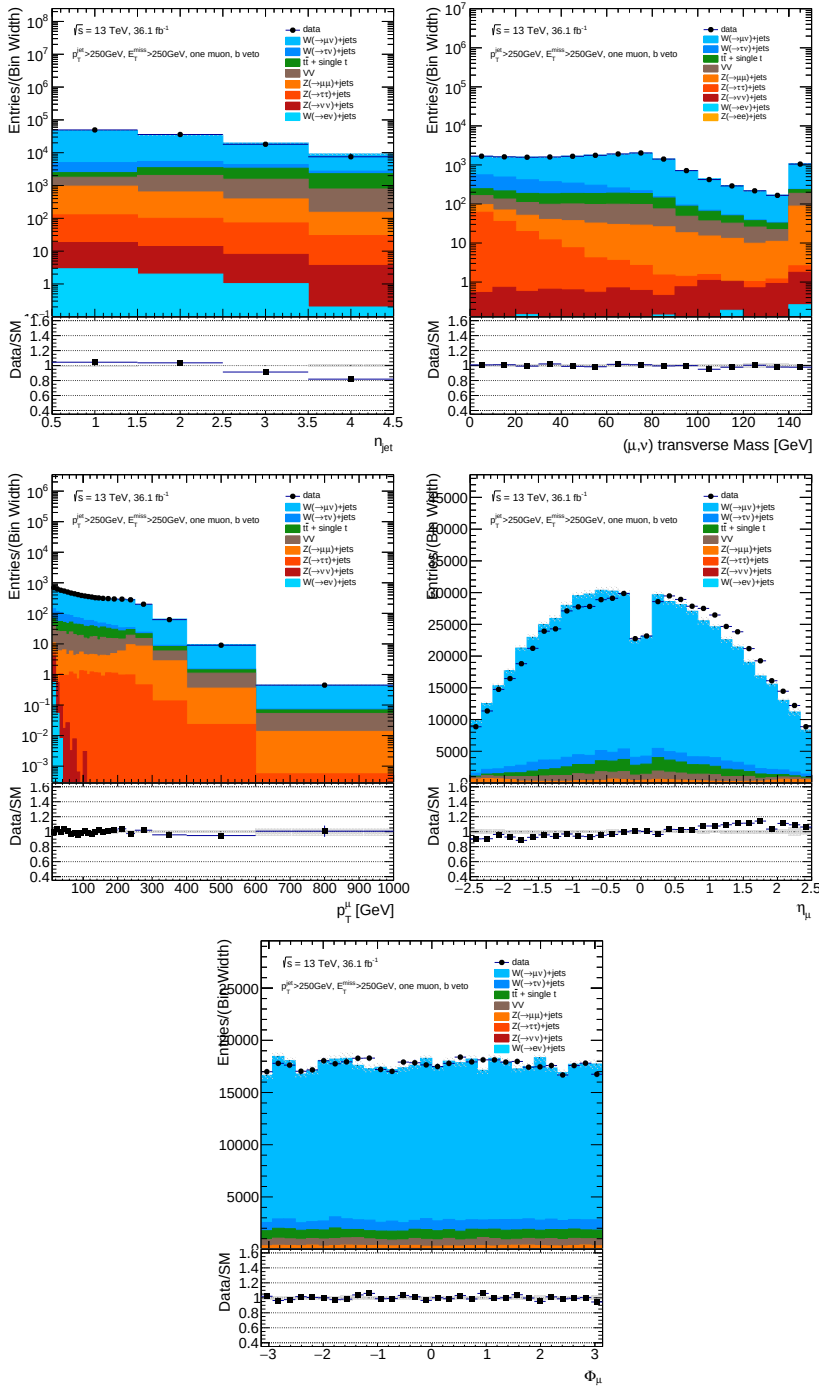
Figure 8.7: Pre-fit kinematic distributions in the CR1mu0b. V + \text{jets} spectra are weighted to higher order corrections (see Section 8.2.3). The sum of the MC spectra are normalized to the total number of observed events in data. The error bands in the upper and lower panel include only the uncertainty due to limited MC statistics.
