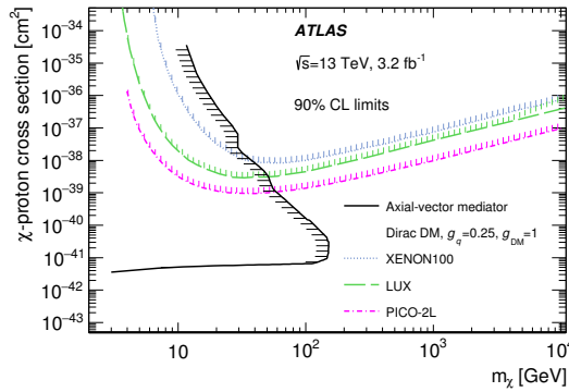
Figure 7.18: The 90% CL exclusion limit on the spin-dependent \chi -proton scattering cross section in a simplified model of DM production involving an axial-vector operator, Dirac DM and couplings g_q = 0.25 and g_\chi = 1 as a function of the dark matter mass m_\chi . Also shown are results from three direct DM search experiments [136, 137, 138].
