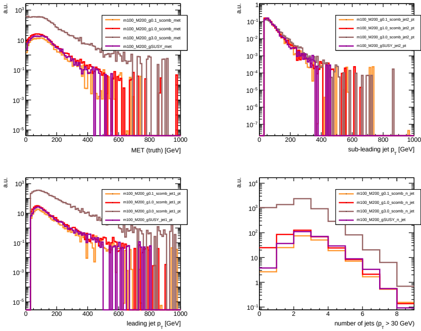
Figure A.9: E_T^{\text{miss}} , leading jet p_T , sub-leading jet p_T , and jet multiplicity distributions for m_\chi = 100 GeV, M_\eta = 200 GeV. The distributions for the t -channel model with several couplings ( g = 0.1 in orange, g = 1.0 in red, g = 3.0 in grey) are compared to the distribution for the SUSY model (purple). Spectra are normalized to their cross-section.
