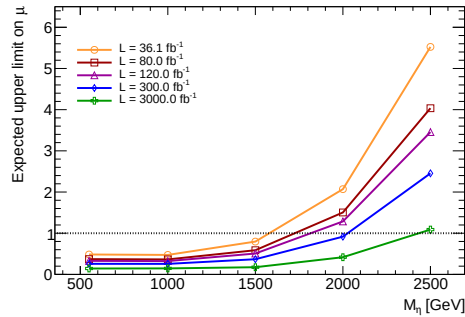
(c) Colored scalar mediator, m_\chi = 500 GeV
