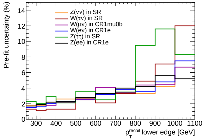
Figure 8.25: Relative PDF systematic uncertainty (in %) on the W + jets, Z + jets backgrounds as function of the p_T^{\text{recoil}} bins. Uncertainties on a given process are quoted in the region where that process is dominant. The uncertainty quoted on the Z(ee) + jets sample is used as a proxy for the Z(\mu\mu) + jets.
