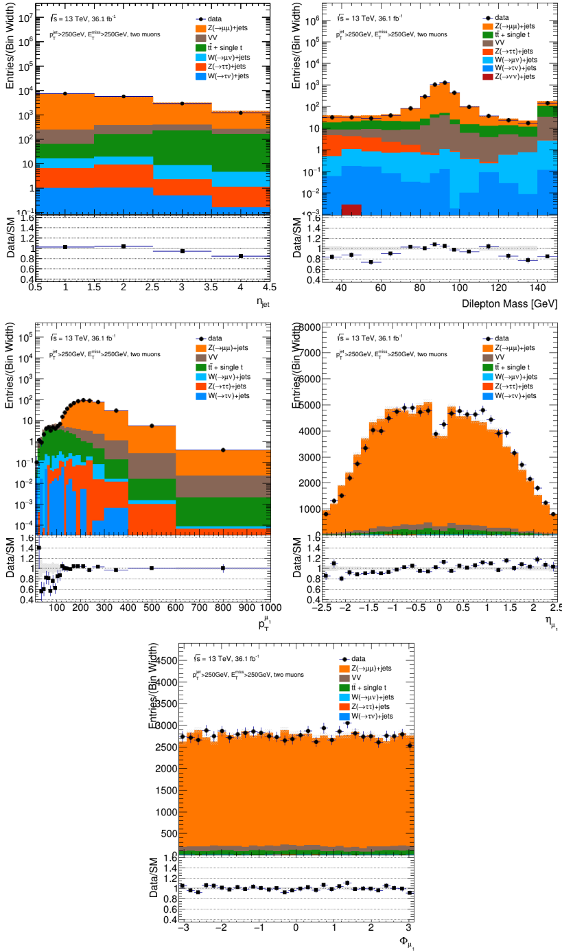
Figure 8.13: Pre-fit kinematic distributions in the CR2mu. V + \text{jets} spectra are weighted to higher order corrections (see Section 8.2.3). The sum of the MC spectra are normalized to the total number of observed events in data. The error bands in the upper and lower panel include only the uncertainty due to limited MC statistics. Note that for the distribution of the dimuon invariant mass, the full distribution is shown, but only events with 66 < m_{\mu\mu} < 116 GeV are retained in CR2mu.
