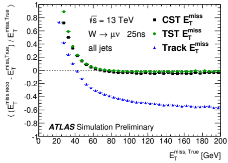
(b) \Delta^{\text{lin}}, \text{inclusive } N_{\text{jets}}
