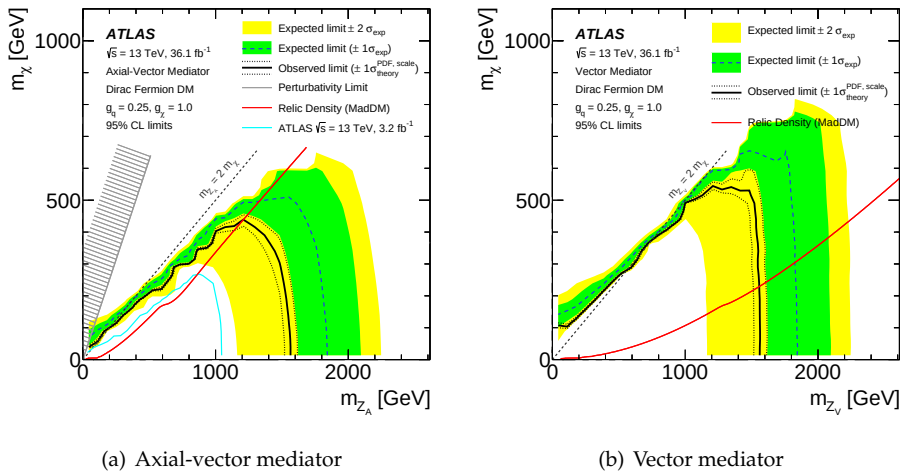
Figure 8.36: Axial-vector (left) and vector (right) 95% CL exclusion contours in the m_{Z_A} - m_\chi and m_{Z_V} - m_\chi parameter planes. The solid (dashed) curves show the observed (expected) limits, while the bands indicate the \pm 1\sigma theory uncertainties in the observed limit and \pm 1\sigma and \pm 2\sigma ranges of the expected limit in the absence of a signal. The red curve corresponds to the expected relic density, as computed with MADDM [98]. In the left lot the region excluded due to perturbativity, defined by m_\chi > \sqrt{\pi/2} m_{Z_A} , is indicated by the hatched area. The dotted line indicates the kinematic limit for on-shell production m_{Z_A} = 2 \times m_\chi . The cyan line indicates previous results at 13 TeV [141] using 3.2 fb ^{-1} .
