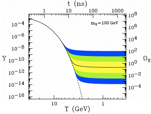
Figure 2.6: The comoving number density Y and resulting thermal relic density for a 100 GeV dark matter as a function of temperature or time. The solid line corresponds to the solution of the Boltzmann equation which yields the correct relic density and the colored regions correspond to a cross section that differ by 10,100,1000 from this value. The shaded line indicates the solution for a particle that remains in thermal equilibrium [22].
