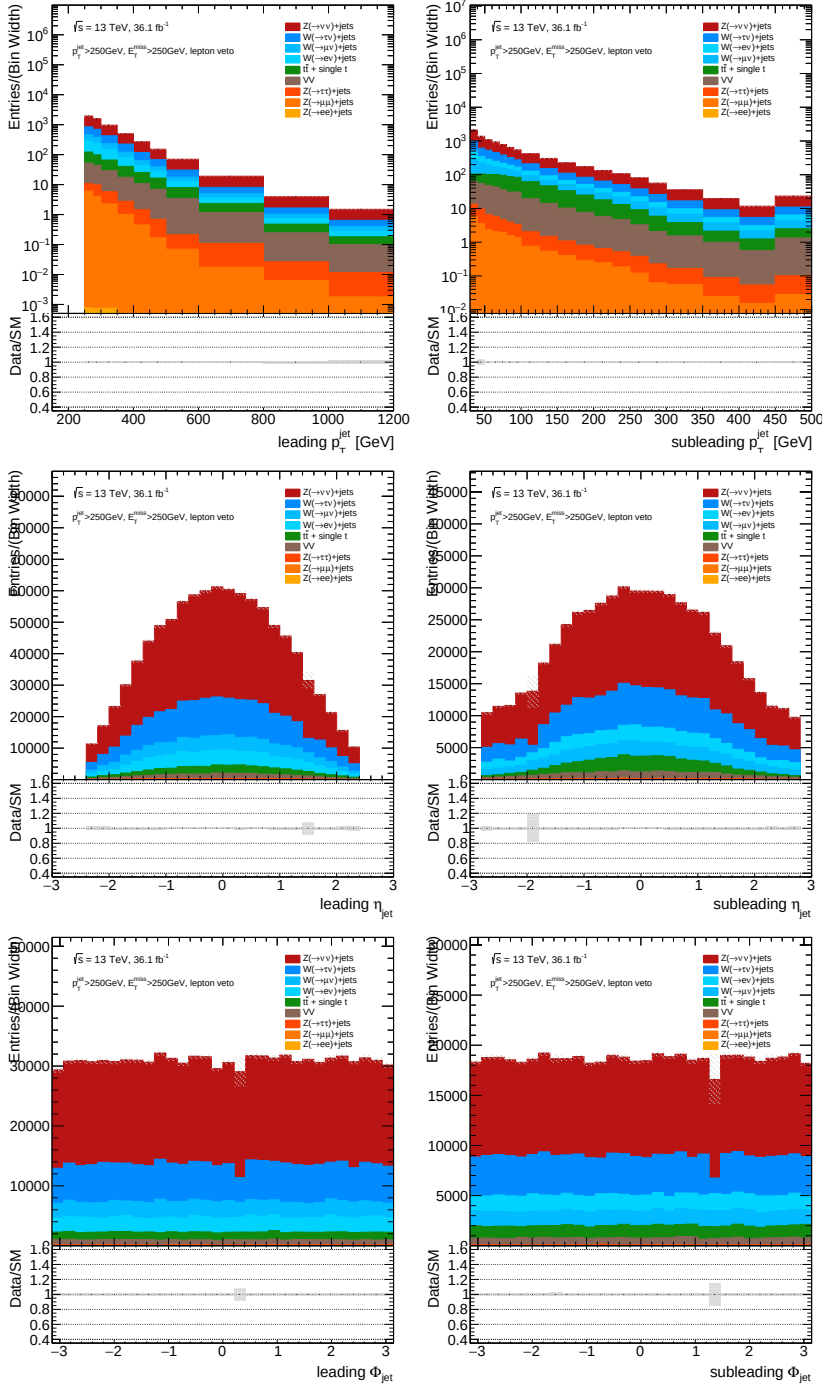
Figure 8.3: Pre-fit Pre-fit kinematic distributions in the SR corresponding to 36.1 \text{ fb}^{-1} . The error bands in the upper and lower panel include only the uncertainty due to limited MC statistics.
