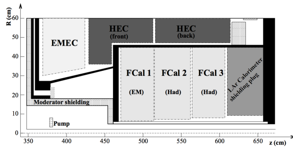
Figure 3.18: Diagram showing the placement of the three FCal modules with respect to the end-cap calorimeters. The shielding plug behind the FCal is also shown [61].
