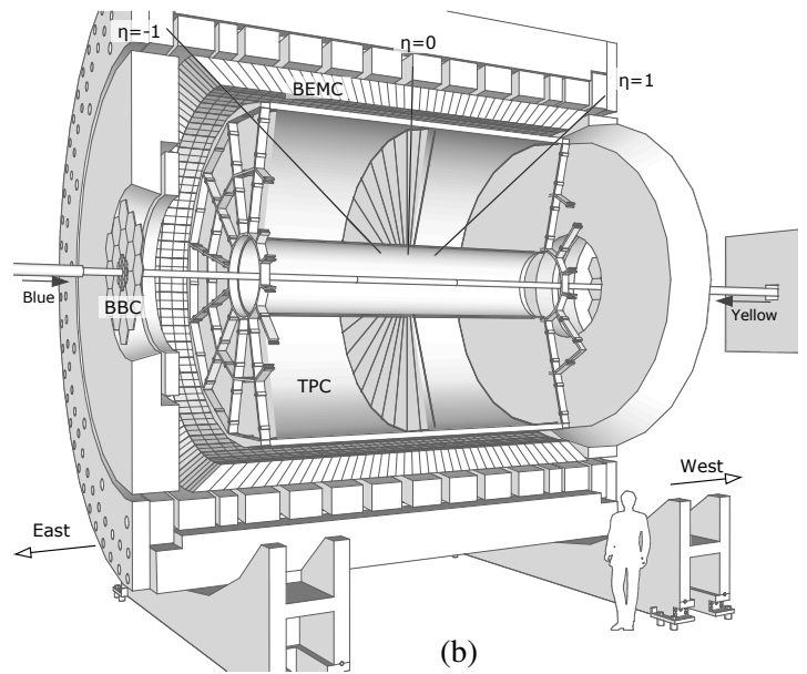
Figure 5.2: (a) Photograph [127] and (b) longitudinal section of the model of the STAR central detector [110].
