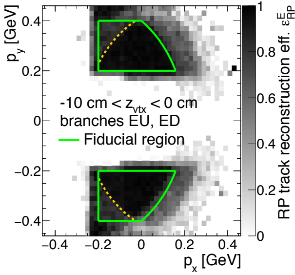
Figure 11.13: Sample RP track reconstruction efficiency in the single z -vertex bin on the East side. The efficiency was calculated using forward proton MC simulation embedded into the zero-bias data sample. Areas surrounded by green lines correspond to the fiducial region used in the measurement, while the dashed yellow lines mark the corner parts of the fiducial region where applying as additional data-driven efficiency correction was necessary needed.
