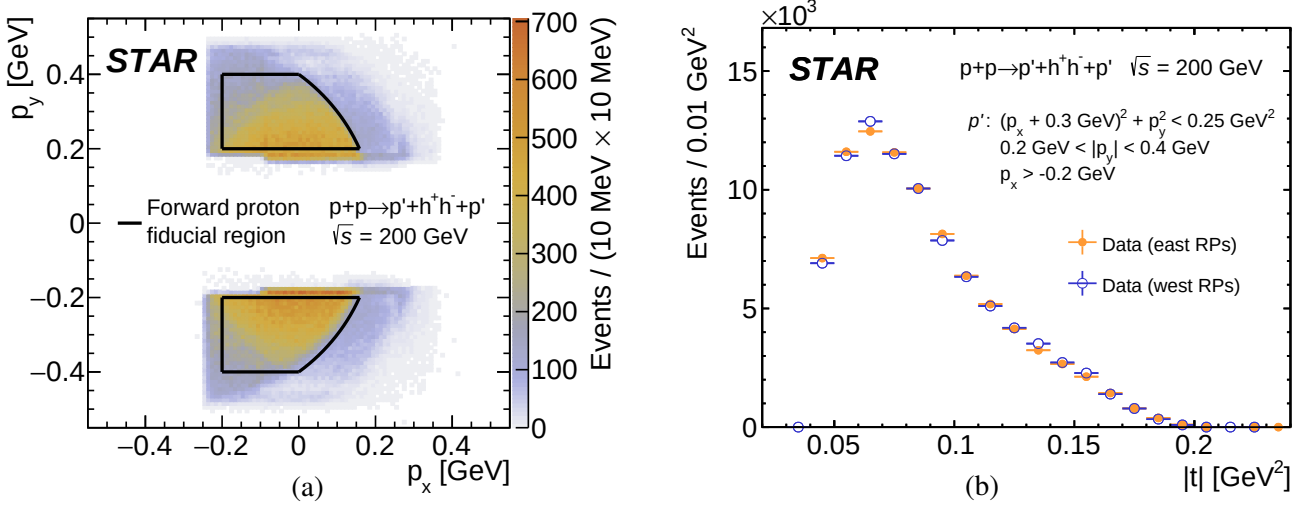
Figure 9.8: (a) Merged distributions of diffractively scattered protons momenta p_y vs. p_x in exclusive h^+h^- events reconstructed with the East and West RP stations, are shown together with the kinematic region used in the measurement marked with the black line. (b) Distributions of measured squared four momenta transfers at the proton vertices for exclusive h^+h^- events with all particles in the fiducial phase space are shown for East and West stations with yellow and blue colour, respectively.
