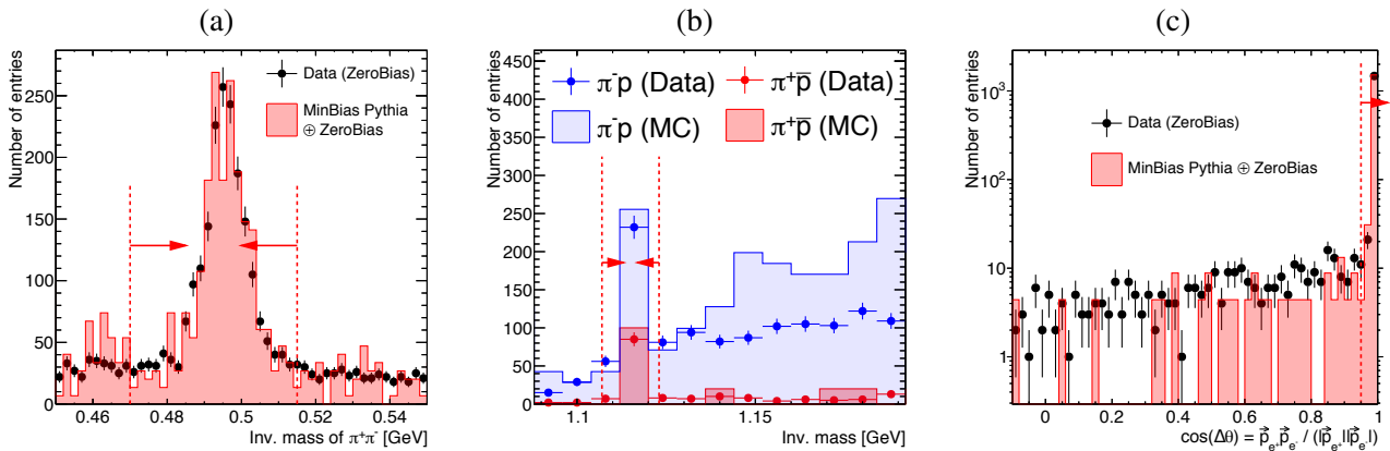
Figure 12.9: Invariant mass of two opposite-sign tracks forming a secondary vertex, recognised as (a) \pi^+ \pi^- , or (b) \pi^+ \bar{p}/\pi^- p pairs, and (c) cosine of the opening angle between two opposite-sign tracks recognised as e^+ e^- pair. Dashed red lines and red arrows indicate ranges of quantities which define particular nature of the secondary vertex (photoconversion/resonance decay/hadronic). Zero-bias data are shown as points, while embedded MB MC as filled histograms.
