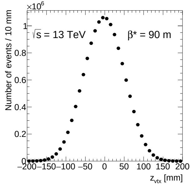
Figure 16.2: z -position of the single primary vertices.
