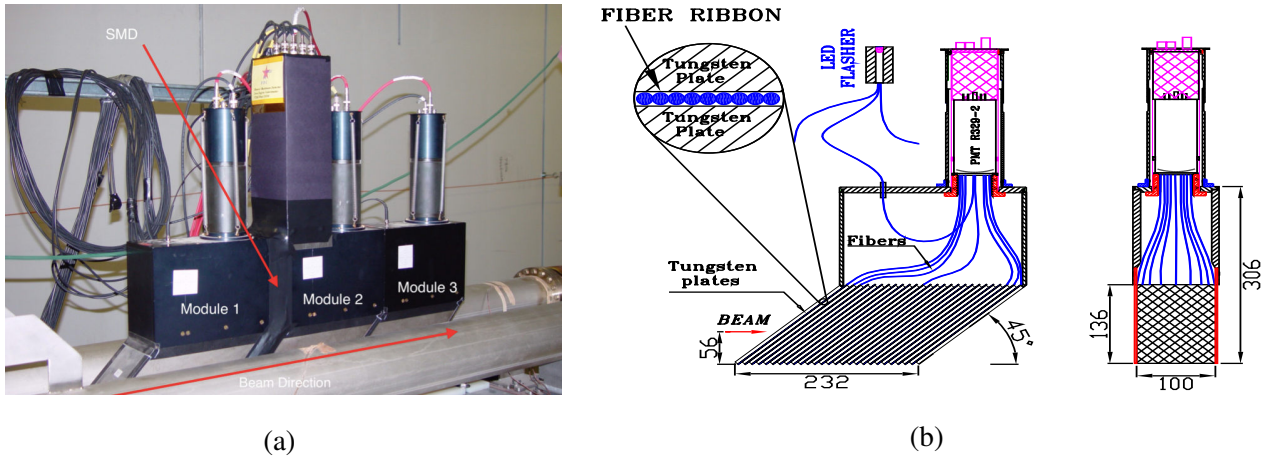
Figure 5.5: (a) Photograph of the ZDC detector and (b) schematic side (left) and front (right) view of a single module (length unit is mm). Figures taken from [139] (left) and from [133] (right).
