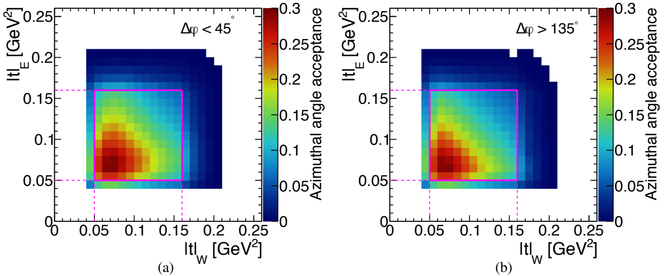
Figure 11.40: Geometrical acceptance for the forward-scattered protons measured in the fiducial region related to the extrapolation to the Lorentz invariant phase space region defined by |y(\pi^+\pi^-)| < 0.4 and 0.05 < -t_1, -t_2 < 0.16 \text{ GeV}^2 , separately for two intervals of \Delta\varphi : (a) \Delta\varphi < 45^\circ , and (b) \Delta\varphi > 135^\circ . Dashed red lines mark the region, in which the fits to corrected data were performed.
