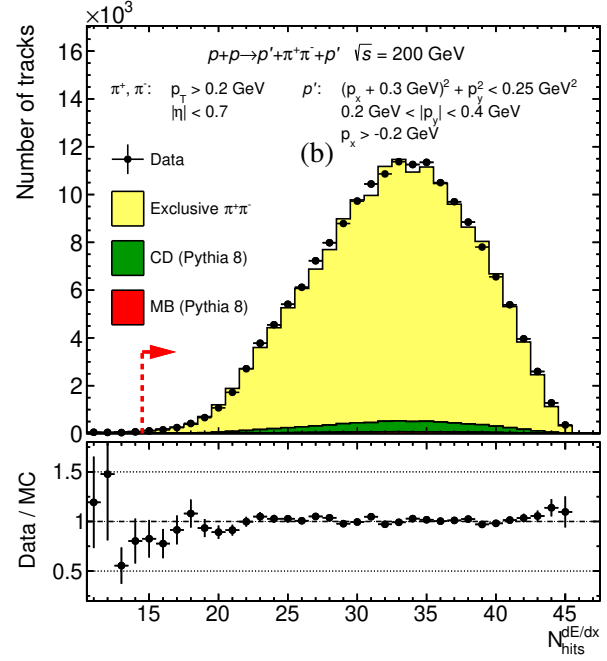
Figure 9.5: Comparison of (a) the number of hits used in TPC track reconstruction N_{\text{hits}}^{\text{fit}} , (b) the number of hits used in specific energy loss reconstruction N_{\text{hits}}^{\text{dE/dx}} and (c) the fraction of the number of hits potentially generated by a track and finally used in the reconstruction N_{\text{hits}}^{\text{fit}}/N_{\text{hits}}^{\text{poss}} in the data (black points) and embedded MC (stacked colour histograms). Normalisations of the signal and backgrounds were established according to description in Sec. 10.3. Predictions for MCs other than GenEx (yellow) were replaced by predictions for GenEx scaled to have the same integrals as replaced histograms - this was driven by the fact that only GenEx was embedded into zero-bias TPC data, which is required to describe the shape of distributions of presented quantities. Vertical error bars represent statistical uncertainties, horizontal bars represent bin sizes. Red dashed lines and red arrows indicate the range of each quantity, which is accepted in the analysis.
