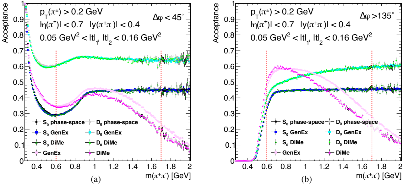
Figure 11.39: Geometrical acceptance for the CEP of \pi^+\pi^- pairs in the fiducial region related to the extrapolation to the Lorentz invariant phase space region defined by |y(\pi^+\pi^-)| < 0.4 and 0.05 < -t_1, -t_2 < 0.16 \text{ GeV}^2 , separately for two intervals of \Delta\varphi : (a) \Delta\varphi < 45^\circ , and (b) \Delta\varphi > 135^\circ . Dashed red lines mark the region, in which the fits to corrected data were performed.
