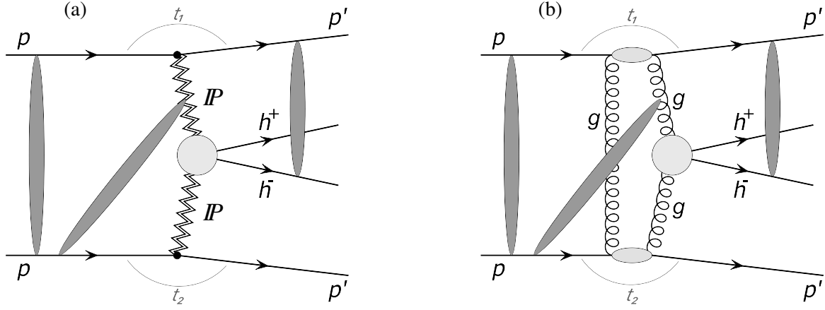
Figure 1.6: Diagrams of DIPE of two opposite-charge hadrons in proton-proton collision, with both protons staying intact. Figure a shows the Regge representation, whereas Fig. b depicts the same process in the leading order pQCD. The light grey circle denotes the non-resonant or resonant mechanism of production of h^+h^- . Dark grey ovals illustrate some possible absorption effects, described in some more detail in Sec. 1.4.2.
