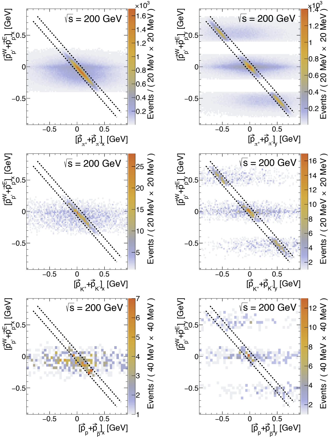
Figure 9.19: Two-dimensional distributions of sum of forward protons momenta (x-axis) and sum of central tracks momenta (y-axis) for exclusive \pi^+\pi^- (top row), K^+K^- (middle row) and p\bar{p} (bottom row) event candidates after full event selection, except the exclusivity cut SC9 . Left and right column shows correlation of respectively x- and y-component of tracks' momenta. Anti-diagonal representing perfect momentum balance of the central and forward system is limited with dashed lines extending by \pm 2.5\sigma ( \sigma \approx 30 MeV) around the anti-diagonal. Three distinct horizontal regions in plots on the right hand side correspond to different forward proton configurations: elastic-like (protons in branches EU&WD or ED&WU, |\vec{p}_{p'}^W + \vec{p}_{p'}^E|_y| < 0.2 GeV) and anti-elastic configuration (protons in branches ED&WD or EU&WU, |\vec{p}_{p'}^W + \vec{p}_{p'}^E|_y| > 0.4 GeV).
