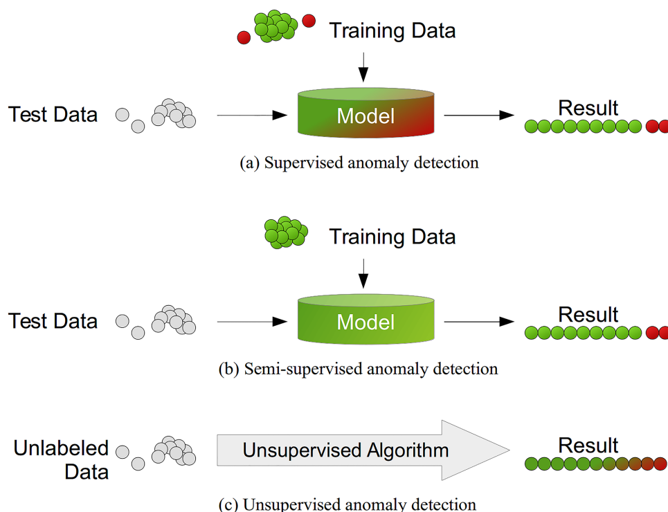
FIGURE 3.1: Differences between supervised, semi-supervised and unsupervised AD approaches. From: Goldstein and Uchida (2016)
