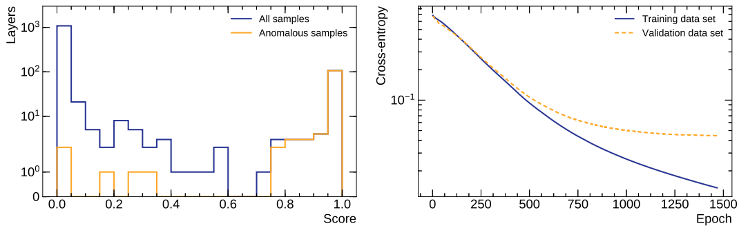
FIGURE 4.5: The distribution of scores (left), and the loss function as a function of the number of training epochs (right) for the CNN model used in the local approach.
