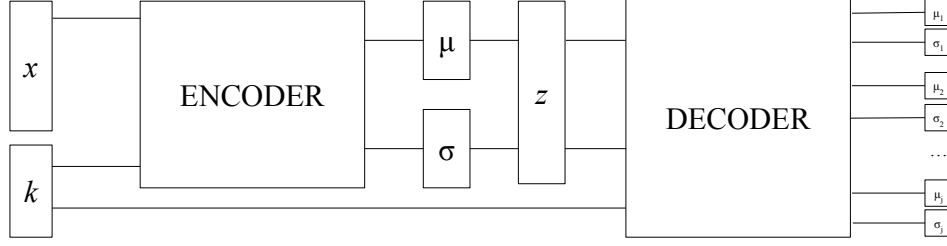
FIGURE 6.5: Architecture of AD-CVAE targeting structured AD based on the VAE framework. The output \mu and \sigma correspond to optimal reconstruction resolution. Observable data x depends on z (capturing non-observable factors of variation u ) and k vectors.
