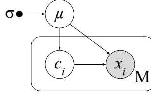
FIGURE 3.7: Graphical model for the Bayesian GMM. The distribution of each observation x_i depends on its corresponding local variable c_i and the global variables \mu .
