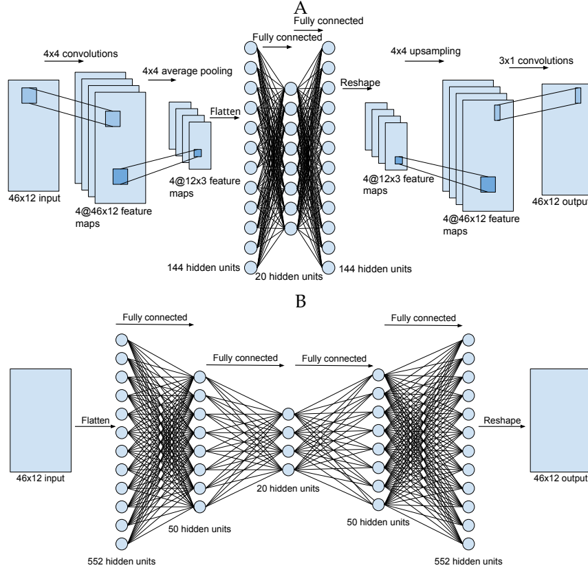
FIGURE 4.11: Convolutional (A) and simple, denoising, sparse (B) autoencoder models architecture used to target regional strategy.
