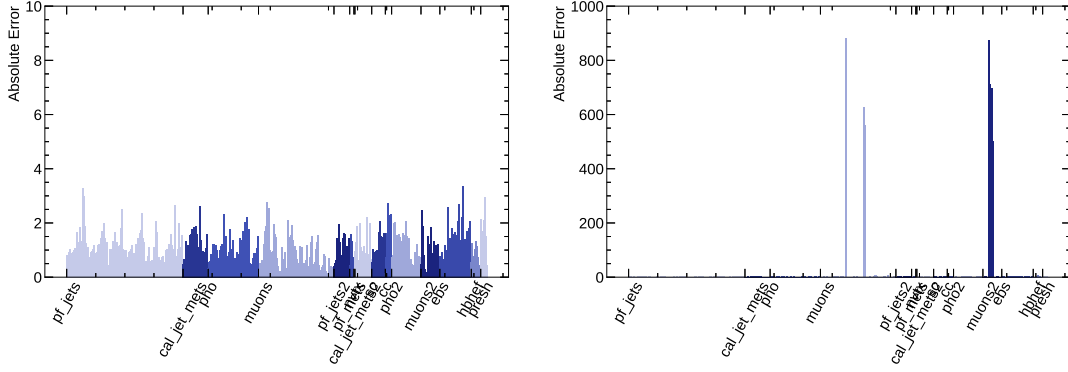
FIGURE 5.7: Reconstruction error of each feature for two samples. Different colours represent features linked to different physics objects. For a negative sample (left) similar autoencoder reconstruction errors are expected across all objects with small absolute scale. Anomalous samples (right) have visible peaks for problematic features (muons).
