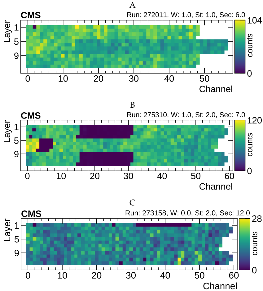
FIGURE 4.1: Example of visualization of input data for three DT chambers. The data in (A) manifest the expected behaviour despite having a dead channel in layer 1. The chamber in the plot in (B) instead shows regions of low occupancy across the 12 layers and should be classified as faulty. According to the run log, this effect was induced by a transient problem with the detector electronics. (C) suffers from a region in layer 1 with lower efficiency, which should be identified as anomalous.
