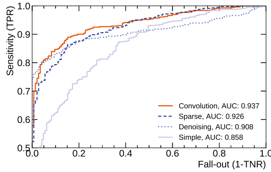
FIGURE 4.13: ROC and AUC of the different autoencoder models used in the regional approach. The anomaly score for the test set is the MSE in layer 9. See Figure 4.12 for comparison of anomaly scores.
