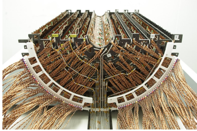
FIGURE 2.7: A barrel pixel detector halves, assembled at Paul Scherrer Institute, with modules made by several European consortia. The photograph shows very lightweight mechanical support, CO 2 cooling tubes and an impressive amount of cabling in a tight volume. From Paul Scherrer Institute (2017) ; Gill and EP-CMX (2017) .
