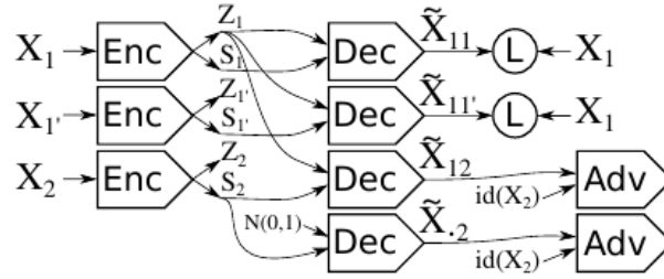
FIGURE 6.4: Architecture of CVAE based on Mathieu et al. (2016) proposal. The inputs x_1 and x'_1 are two different samples with the same label, whereas x_2 can have any label.
