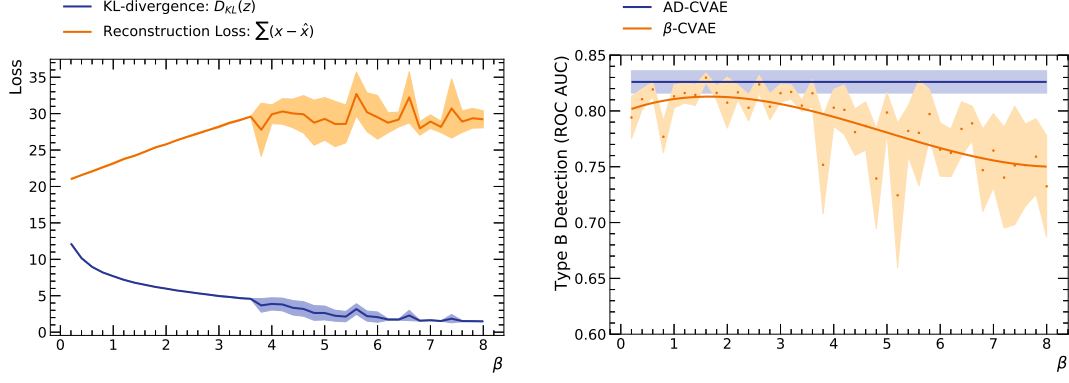
FIGURE 6.9: The final loss function values for a \beta -CVAE (left) and results of the type B detection problem for the synthetic data set as a function of varying \beta (right). The experiment was run five times for each of the chosen \beta values. The orange bands correspond to the standard deviation of the results. The dots correspond to the mean and the solid line to a polynomial fit of the means. The AD-CVAE ROC AUC stays constant as the training procedure does not depend on \beta hyper-parameter (see the loss in equation 6.4).
