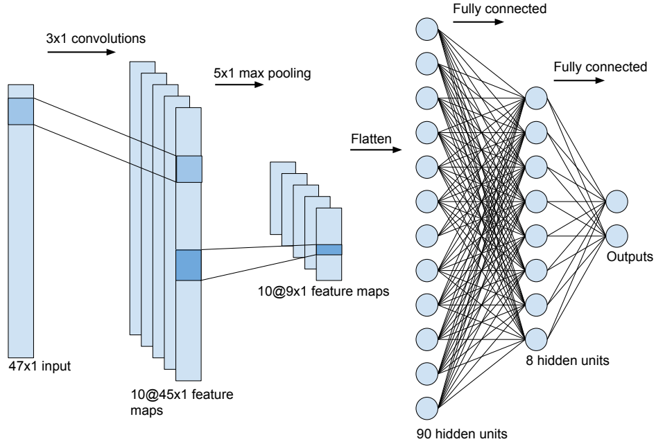
FIGURE 4.3: Architecture of the CNN model used to target the local strategy.
