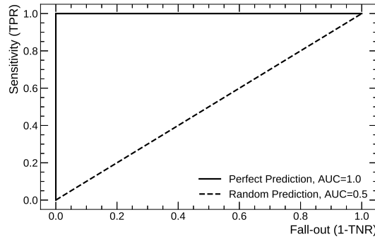
FIGURE 3.2: Examples of ROC curves with Sensitivity as a function of Fall-out. The two lines correspond to a perfect and a random prediction.
