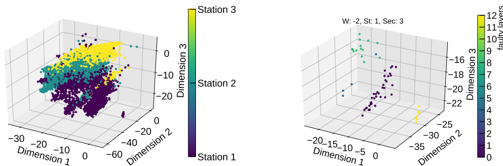
FIGURE 4.14: Compressed representations of chamber level data for all chambers (left) and limited to only one chamber across different runs on a scale of the number of anomalous layers (right). The samples cluster according to their positions in the detector, i.e. station number (left), or according to similar behaviour (right).
