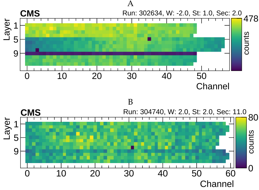
FIGURE 4.10: Example of the impact on hit counting of different voltages applied to layer 9. (A) shows the occupancy map when operating the layer at 3200 V and (B) shows the effect of operating at 3450 V. Both examples should be regarded as anomalies. Since the values in both cases are not equal to zero, the legacy strategy considers those cases as non-problematic.
