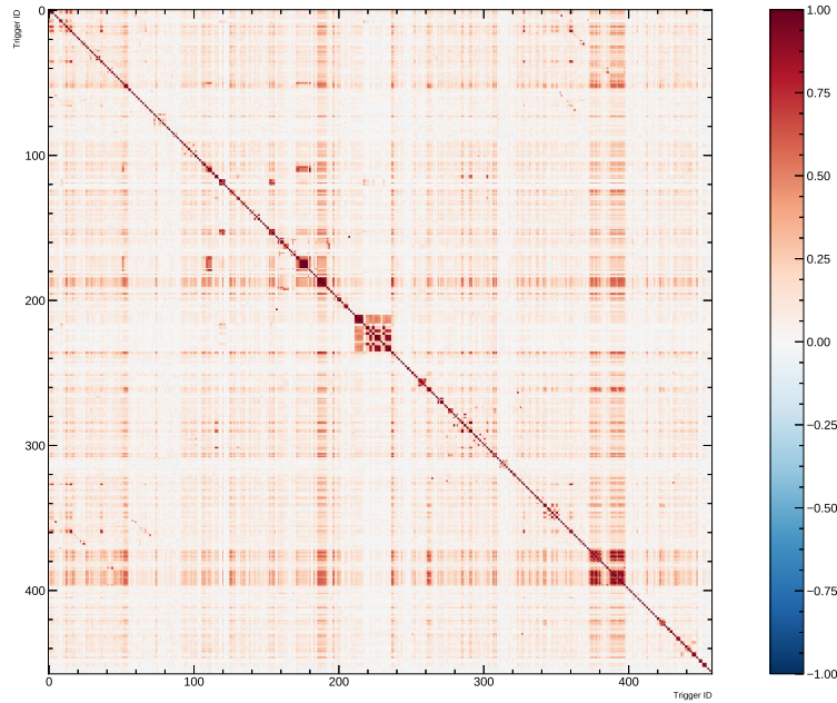
FIGURE 6.1: Correlations between 458 HLT rates of LHC fill 6291 of Run 2. The calculation is performed after correction for down-trend of all trigger rates using first differences.
