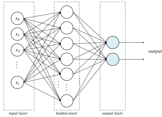
FIGURE 3.6: An illustration of the multi-layer feed-forward ANN from Sun (2019). Neurons are linked by weighted connections to form a network. In this example, there are no in- or cross-layer connections. An input layer receives input feature vector x , with each neuron corresponding to one feature. An output layer size corresponds to given ground truth y size. The layers between the input and output layers are called hidden layers. A non-linear transformation follows each output of a neuron in hidden, and output layers called an activation function , e.g. a sigmoid function.
