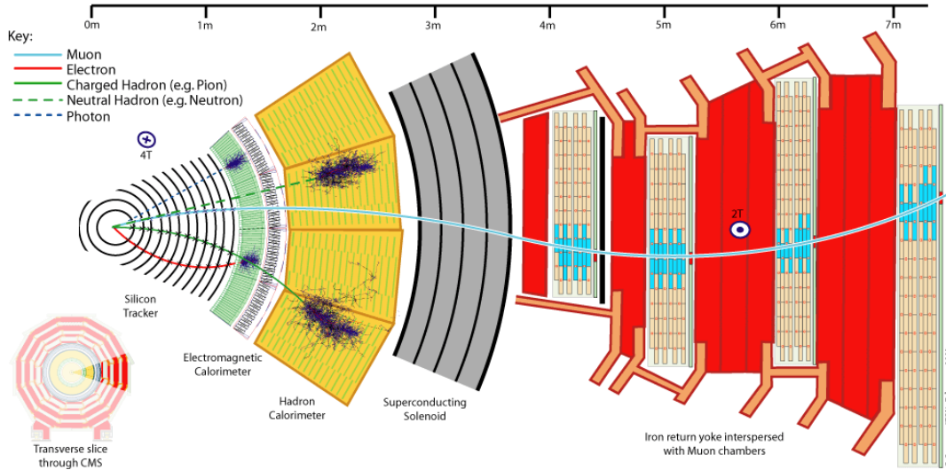
FIGURE 2.6: A sketch of the particle interactions in a transverse slice of the CMS detector, from the collision point to the muon detectors. From Davis (2016).
