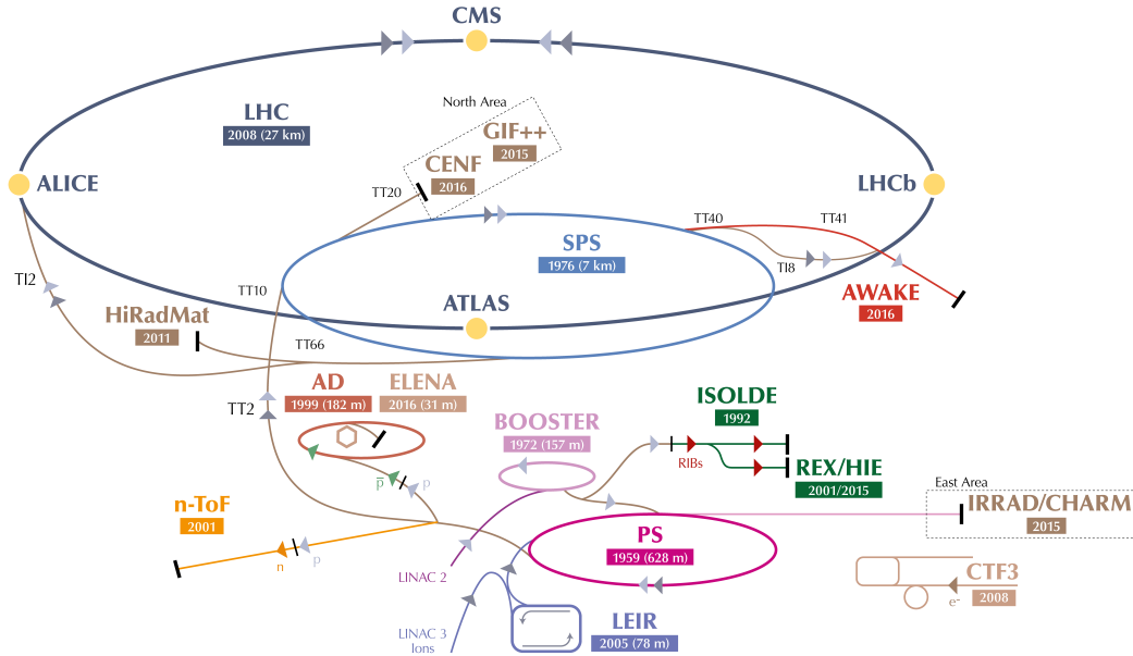
FIGURE 2.2: A view on CERN's accelerator complex. From CERN (2016) .
