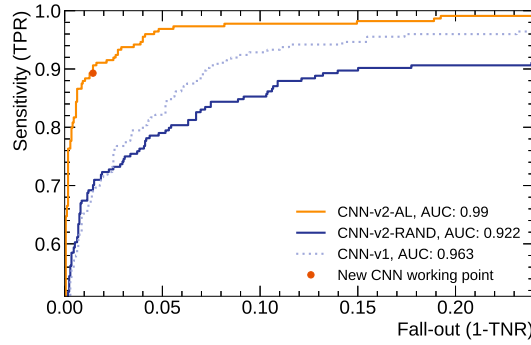
FIGURE 4.9: ROC curves for different versions of CNN. CNN-v1 is the model trained on the initially labelled data set. Its AUC drops compared to Figure 4.4 as the test set is extended with new samples to ease comparison between different versions. CNN-v2-RAND and CNN-v2-AL are models trained on a set \sim 20\% bigger than the original one with additional labels coming from different sources. CNN-v2-RAND uses labels coming from a random selection of chambers while CNN-v2-AL uses uncertainty sampling. The experiment shows that the incorrect choice of samples to label can lead to a drop in model performance.
