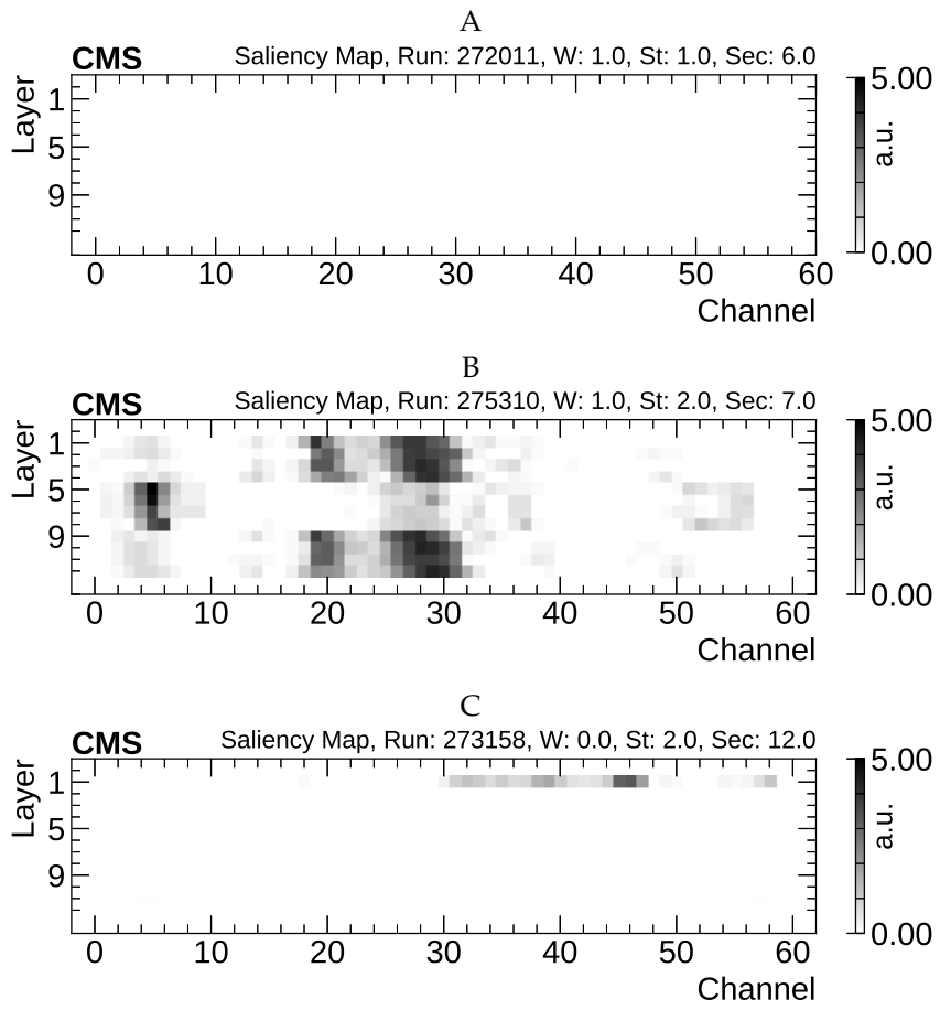
FIGURE 4.8: Example of visualization of saliency maps for three DT chambers corresponding to input occupancies from Figure 4.1. The scale is proportional to the channel influence over classifier decision to flag problems.
