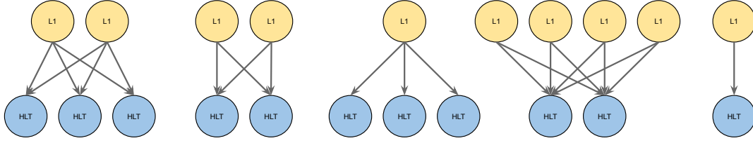
FIGURE 6.2: Simplified, schematic graph inspired by the trigger system configuration. Blue nodes represent HLT while yellow L1 Trigger. Each link is unidirectional starting from yellow nodes. For each LHC fill the graph has a few hundred nodes spread approximately equally between HLT and L1 Trigger. The connection between L1 Trigger and HLT nodes can be seen as a hierarchical directed graph from the L1 Trigger to the HLT system.
