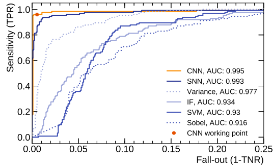
FIGURE 4.4: ROC curves for different models used in the local approach. The AUC is quoted to compare the performance.
