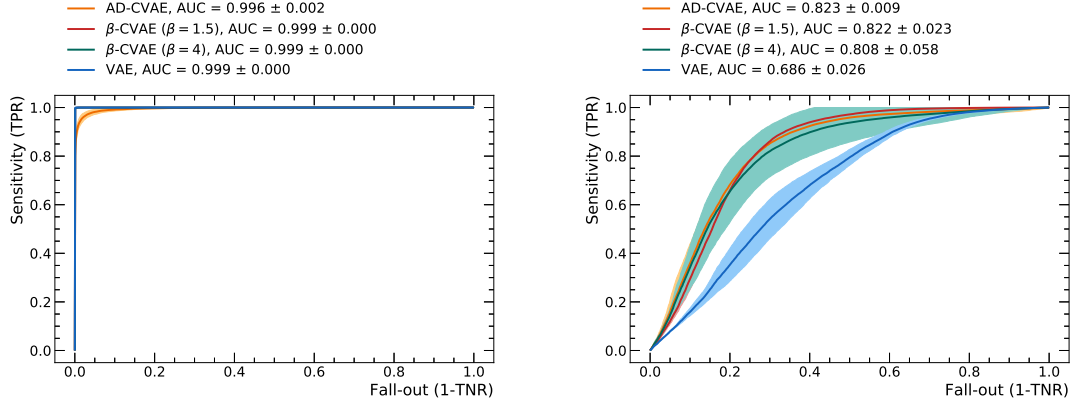
FIGURE 6.11: The ROC curves for two AD problems using synthetic test data set for type A (left) and type B detection (right). The bands correspond to variance computed after running the experiment five times using random weight initialization. Anomaly score for type B is computed for s = 3\sigma using mean \mathbb{D}_{\text{KL}} of z . Anomaly score for type A problem is computed for s = 5\sigma using decoder outputs: \mu and \sigma of each feature.
