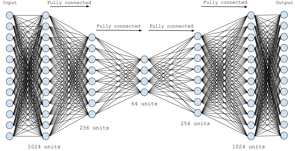
FIGURE 5.2: Proposed base autoencoder architecture for DC novelty detection. The hyper-parameters were chosen using a grid search.
