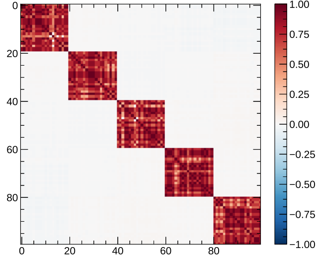
FIGURE 6.6: Correlations between features in the synthetic data set for m = o = 5 and n = 100 . The data set was prepared as a proxy of the trigger system behaviour, seen in Figure 6.1.
