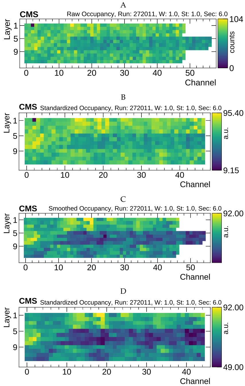
FIGURE 4.2: Example of two kinds of input sample preprocessing. (A) acquired ( raw ) values, (B) standardizing each layer directly from raw values using linear interpolation. (C) smoothing the raw values data with median filter (D) standardizing each layer from smoothed data. In (C), the isolated low-occupancy spot in layer 1, corresponding to a dead channel, is discarded.
