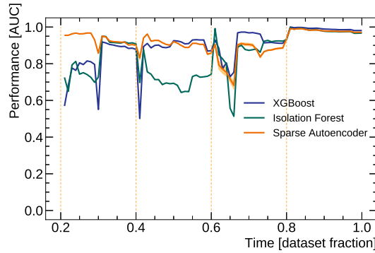
FIGURE 5.6: Performance of different strategies as a function of time. Compared are supervised AD XGBoost, semi-supervised AD sparse autoencoder and unsupervised IF. After every 0.2 fractions of the data set, each method is retrained on all of available past data points using ground truth labels. AUC is reported since last retraining.
