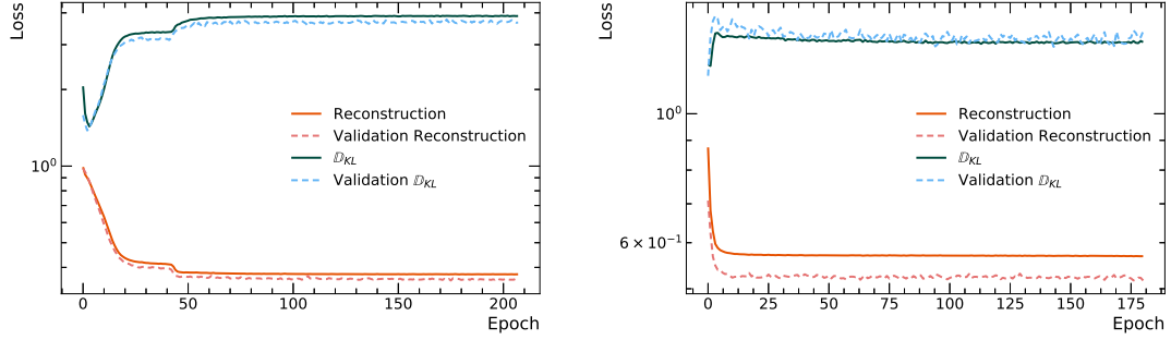
FIGURE 6.10: Loss yield as a function of the number of epochs in the training of the AD-CVAE model (left) and \beta -CVAE (right) used for the anomalous trigger rate detection. The two curves illustrate the behaviour of the training and validation data sets.
