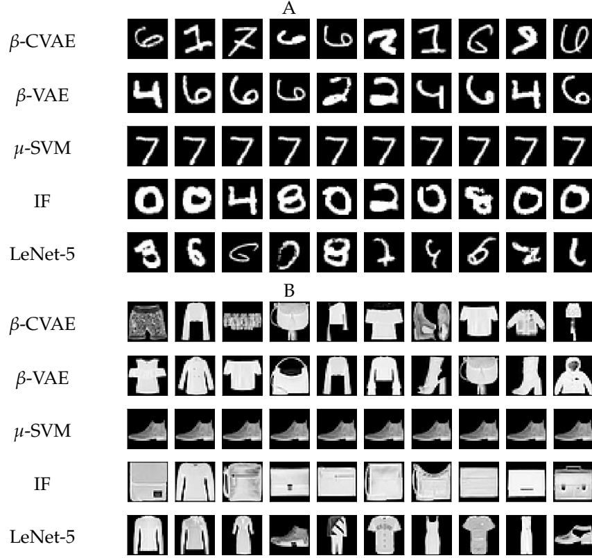
FIGURE 6.7: Most anomalous samples in the test set for MNIST (A) and Fashion-MNIST (B) data sets for each AD method. The samples reported for LeNet-5 classifier are the ones having the biggest classification error.
