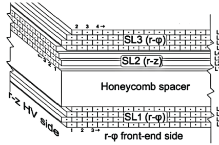
FIGURE 2.8: Schematic view of the one DT chamber showing the position and orientation of the tubes. From CMS Collaboration (2010) .
