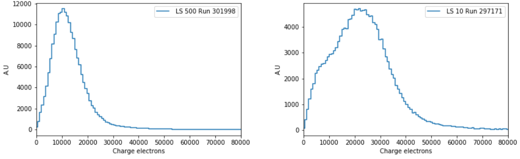
FIGURE 5.1: Two examples of histograms related to the Pixel detector (see Section 2.3.2) status for a normal (left) and anomalous (right) LSs. The reference shape is the Landau distribution. The bad LS manifests anomaly in low charge, which is caused by the Pixel detector not being properly synchronized with the bunch crossing. Such distributions, obtained for each LS, are preprocessed into a summary statistics vector of seven variables: five quantiles, mean and standard deviation.
