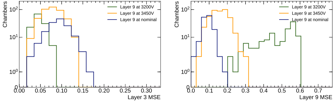
FIGURE 4.12: MSE between reconstructed and input samples for layer 3 (left) and layer 9 (right) for three categories of data for convolutional autoencoder. Despite a problem in layer 9, all \epsilon for layer 3 are comparable for all chambers. The nominal voltage falls between 3550 and 3600 V .
