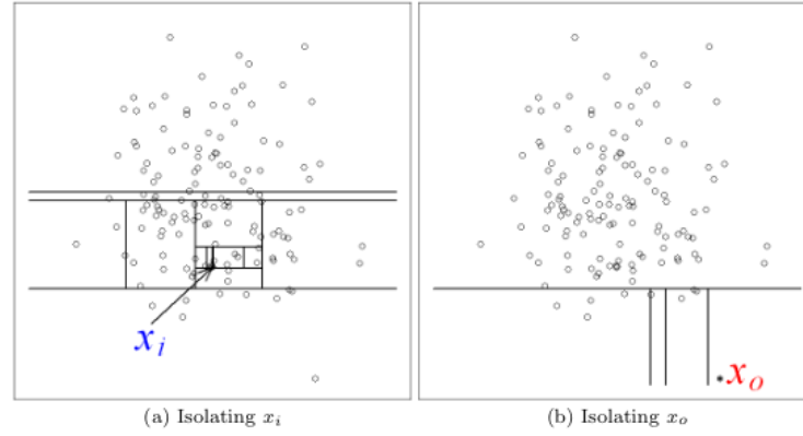
FIGURE 3.4: Two-dimensional, normally distributed data set with 135 points. An inlier x_i requires twelve random partitions to be isolated (a), while outlier x_o only four (b). Anomalies are more susceptible to isolation and hence are isolated faster. From Liu et al. (2012) .
