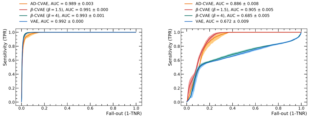
FIGURE 6.12: The ROC curves for two AD problems using trigger rate data set for type A (left) and type B detection (right). The bands correspond to variance computed after running the experiment five times using random weight initialization. Anomaly score for type B is computed for s = 3\sigma using mean \mathbb{D}_{\text{KL}} of z . Anomaly score for type A problem is computed for s = 5\sigma using decoder outputs: \mu and \sigma of each feature.
