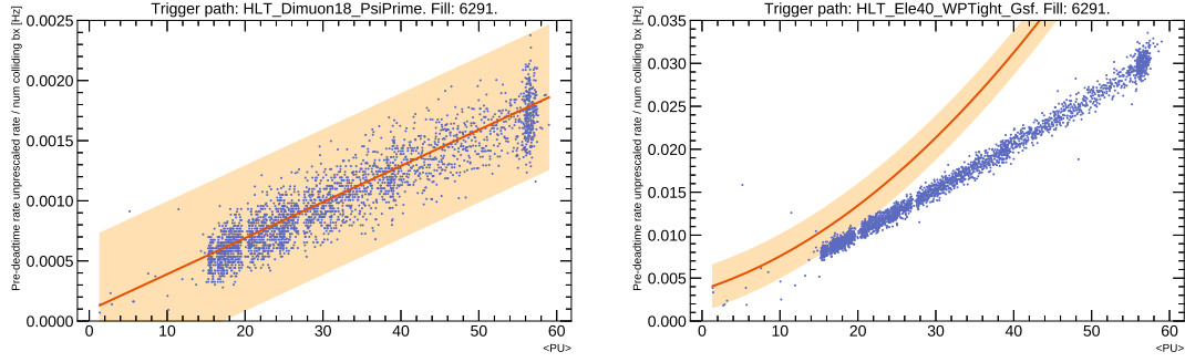
FIGURE 2.12: Observed rates as a function of average PU (blue dots), compared to the predicted dependence (red line) and its uncertainty (in the orange band) generated using TRM software. The plots above show an example of a well (left) and poorly (right) predicting model.
