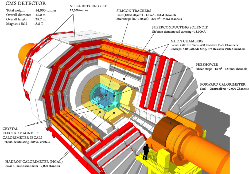
FIGURE 2.5: A cutaway diagram of the CMS detector with elementary information about different sub-detectors. From Marcastel (2013) .
