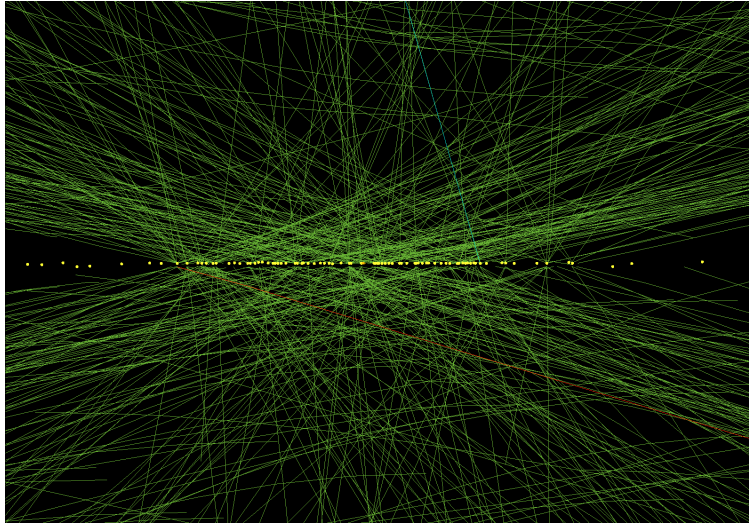
FIGURE 2.3: The spacing of 78 (PU= 78) collisions (yellow dots) at the CMS detector along the z-axis. The green lines represent tracks of the resulting particles. Credit: Andre Holzner.
