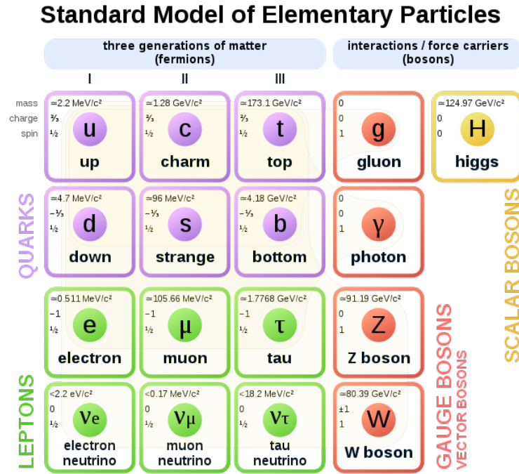
FIGURE 2.1: The SM of elementary particles: the 12 fundamental fermions and five bosons. From MissMJ (2006) .
