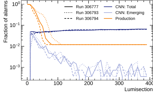
FIGURE 4.7: Stability of the proposed model and the legacy strategy as a function of time ( number of LSs ) for three different runs: 306777, 306793, 306794. The stability test is performed every 10 LSs. The CNN: Total and Production lines follow the total fraction of alarms generated by the methods. Instead, CNN: Emerging reports the fraction of new alarms being generated by the CNN model w.r.t previous test point.
