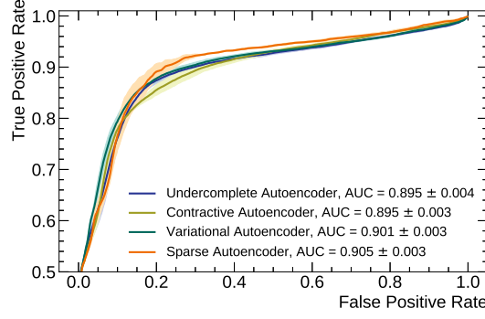
FIGURE 5.3: ROC and AUC of the autoencoder models using different regularization techniques. The bands correspond to variance computed after running the experiment five times using random weight initialization.
