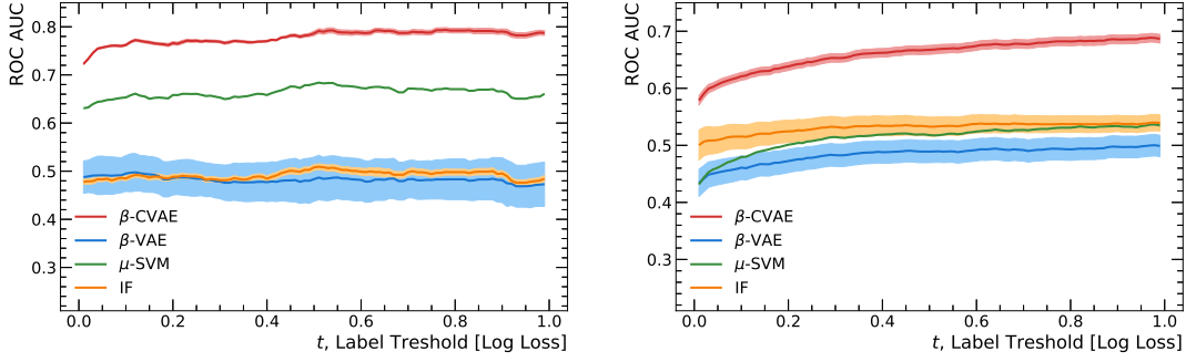
FIGURE 6.8: Reported ROC AUC for MNIST (left) Fashion-MNIST (right) data sets and different AD algorithms as a function of varying anomaly strictness \tau based on LeNet-5 model classification log loss s . Overall classifier accuracy is 98.95% and 89.62% for MNIST and Fashion-MNIST respectively. The curves stay relatively flat due to the high performance of the classifier: most of the test samples have log loss smaller than 0.01. As a consequence, the test sets have low variability when values of \tau change.
