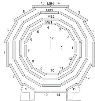
FIGURE 2.10: Numbering schema of the sector and stations of DT chambers in one wheel. From CMS Collaboration (2010) .
