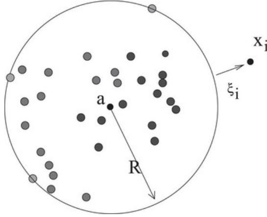
FIGURE 3.5: Illustration of SVDD on two-dimensional data set. The hyper-sphere contains the target data and is described by the centre a and radius R . One data point, an outlier x_i is outside the sphere and has \xi_i > 0 , where \xi is a slack variable to account for errors. From Tax (2001); Khan and Madden (2014).
