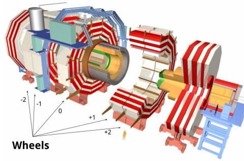
FIGURE 2.9: Magnified view of the CMS detector showing the wheel structure. The white volumes represent the muon chambers while the red volumes represent the iron return yoke.
