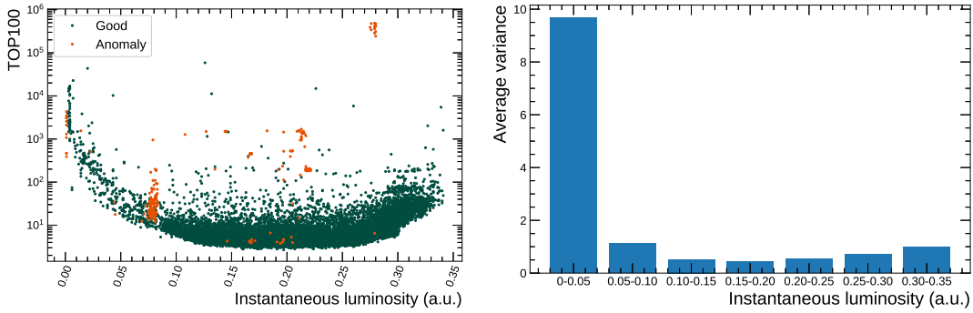
FIGURE 5.4: Anomaly score w.r.t. instantaneous luminosity (left) of sparse autoencoder and the average feature spread in different instantaneous luminosity regions (right).
