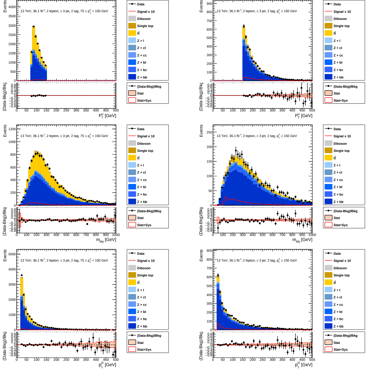
Figure C.16 BDT input variables in \geq 3 jet (3). p_T^V = 75\text{--}150 GeV (left) and 150\text{--} GeV (right). p_T^V , m_{bbj} , p_T^{j3} , from top to bottom. Signal is scaled by 10. Z + \text{HF} and t\bar{t} are scaled by the same factors in section 11.1.
