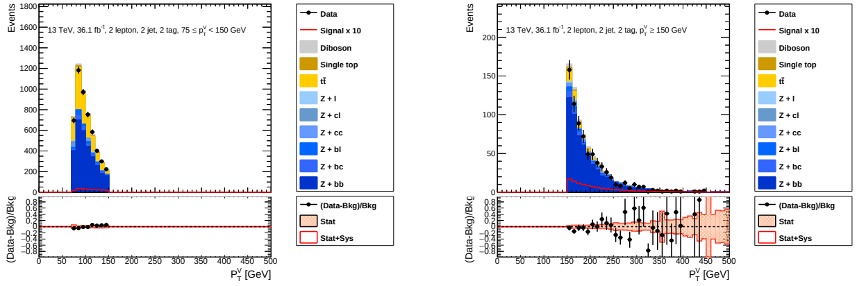
Figure C.13 BDT input variables in 2 jet (3). p_T^V = 75\text{--}150\text{ GeV} (left) and 150\text{--}\text{ GeV} (right). Signal is scaled by 10. Z+HF and t\bar{t} are scaled by the same factors in section 11.1.
