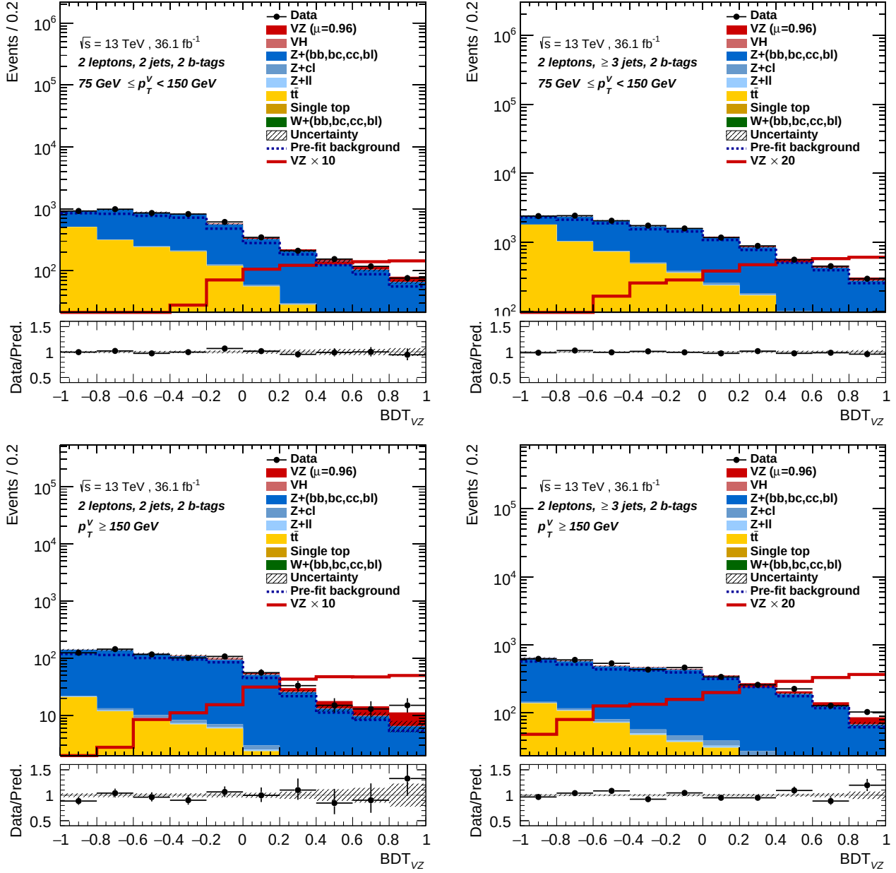
Figure 11.7 BDT VZ postfit distributions in the SR. p_T^V 75–150 GeV (top) and p_T^V 150– GeV (bottom). 2 jets (left) and ≥ 3 jets (right). Filled histograms are postfit background and signal. Unfilled and unstaked histogram is signal, with a scale factor written in the legend. Dashed histograms are prefit background. Hatched bands are total uncertainties of postfit background and signal. Lower panels are ratio of data and postfit background and signal.
