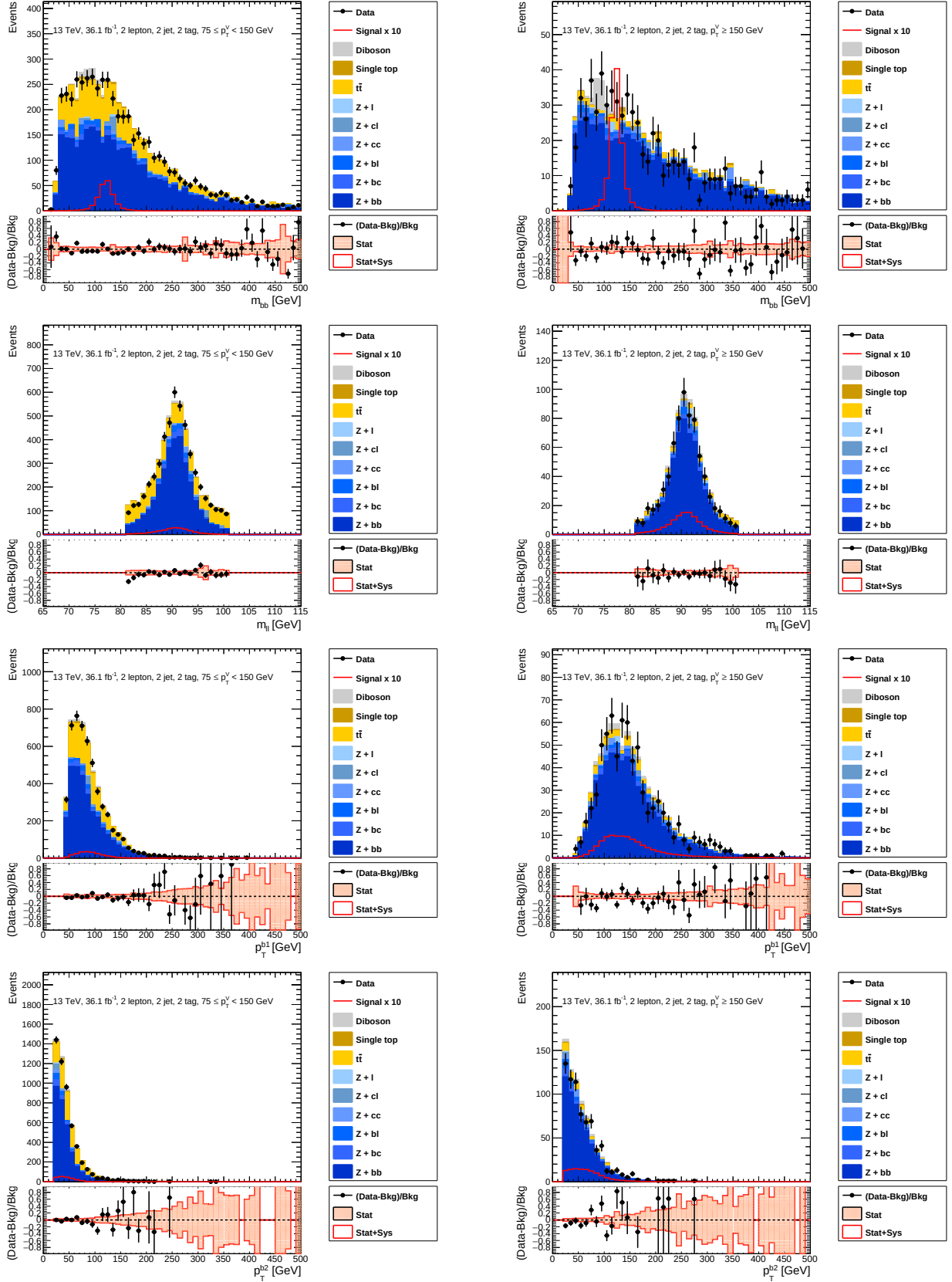
Figure C.12 BDT input variables in 2 jet (2). p_T^V = 75\text{--}150\text{ GeV} (left) and 150\text{--}\text{GeV} (right). m_{bb} , m_{\ell\ell} , p_T^{b1} , p_T^{b2} from top to bottom. Signal is scaled by 10. Z +HF and t\bar{t} are scaled by the same factors in section 11.1.
