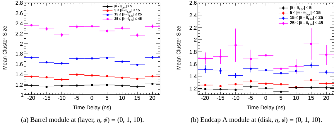
Figure 7: Variation in mean cluster size with time offset, shown for four different ranges of track (to which the cluster belongs) incident angles to the modules, measured with respect to the lorentz angle.
