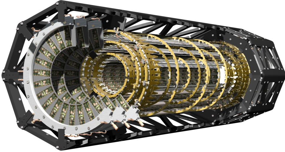
Figure 2.5: A cut-away view of the Pixel detector and support structures, showing the barrel cylinders, endcap disks and the attached modules [1].
