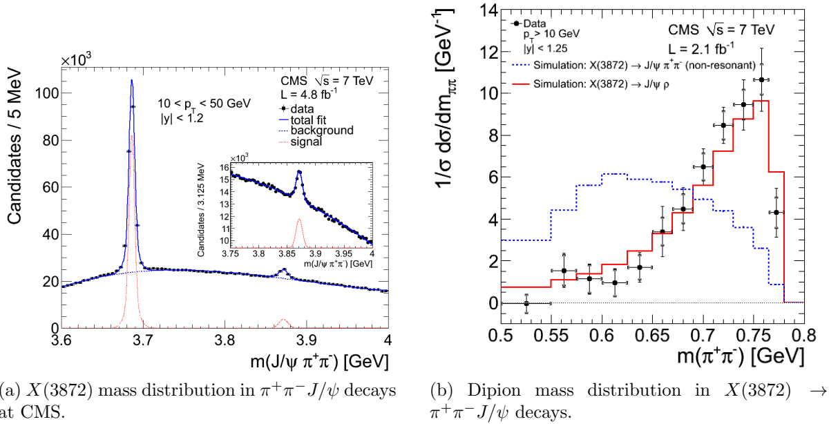
Figure 1.2: The latest X(3872) and dipion mass distributions from CMS [4].
