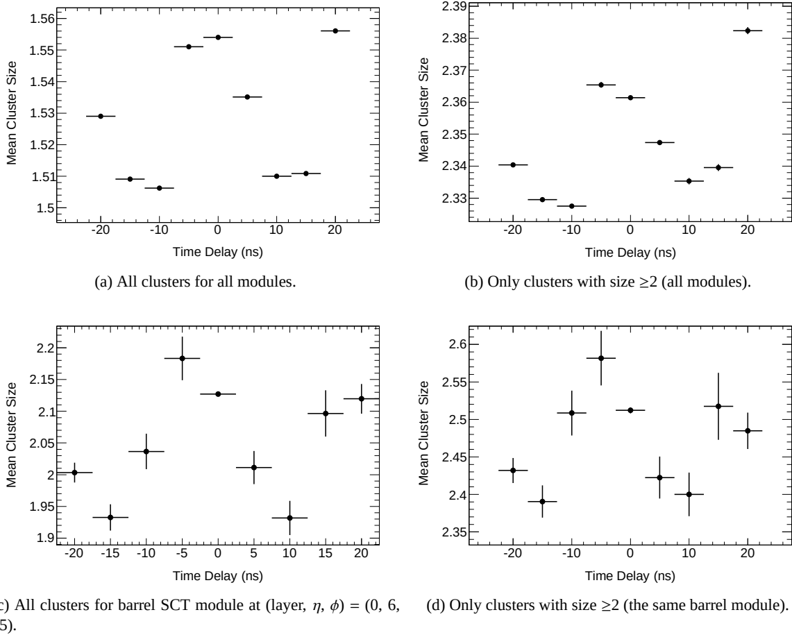
Figure 6: Variation in mean cluster size with time shifts, showing the comparison between all clusters (left) and clusters almost completely from real hits (right). The top plots are the combined results from all modules, whilst the bottom are for a specific example barrel module.
