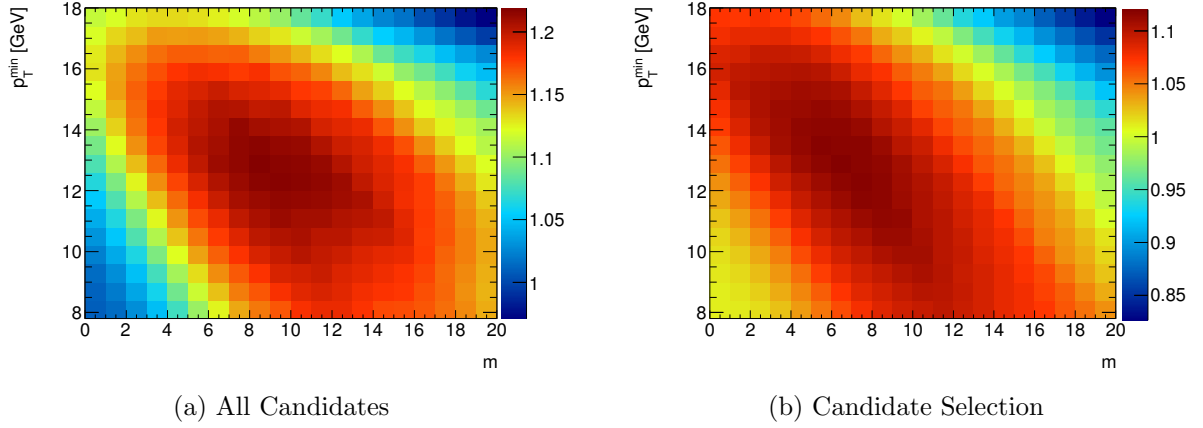
Figure 7.3: The increase in expected statistical significance as a function of the slope, m , and intercept, p_T^{min} , parameters of a diagonal cut through the (p_T, \cos \theta^*) plane. The significance is approximated using a simple formula (see text), and is calculated relative to the baseline (i.e. no diagonal cut – m = 0, p_T^{min} = 0 ) selections.
