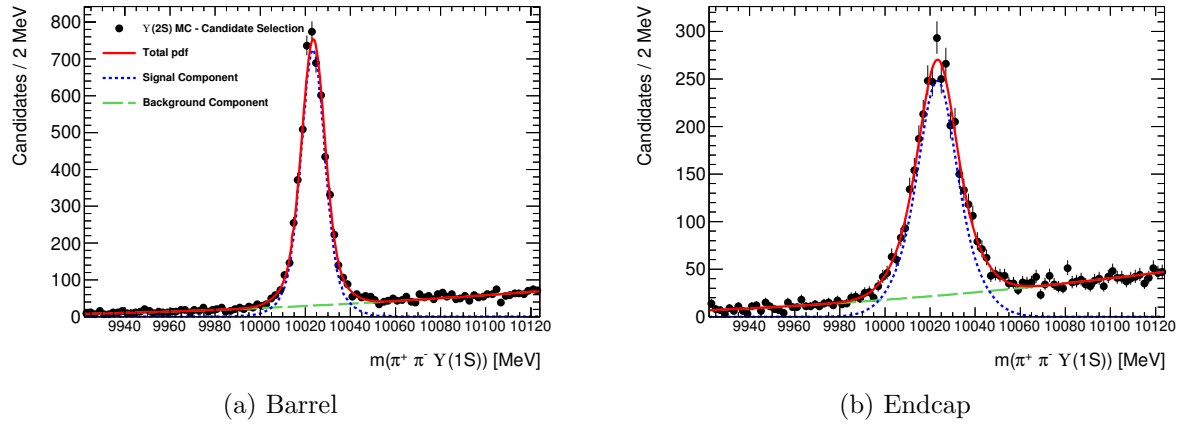
Figure 5.19: The fitted mass spectrum in the \Upsilon(2S) MC sample near m = 10023 MeV, for the barrel (left) and endcap (right) bins.
