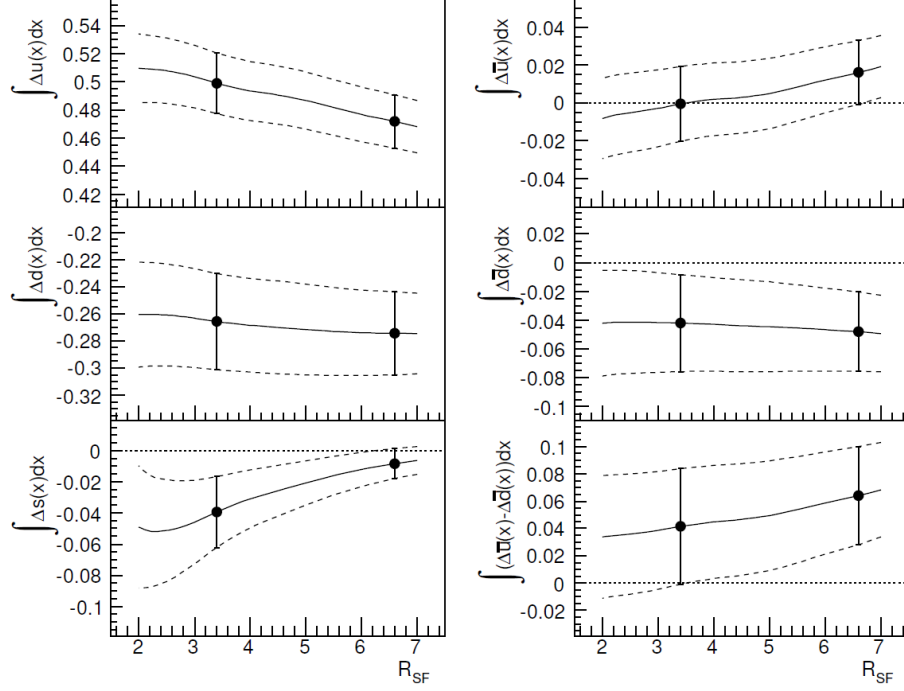
Figure 4.4: Variation of the first moments \Delta u , \Delta \bar{u} , \Delta d , \Delta \bar{d} , \Delta s , \Delta \bar{u} - \Delta \bar{d} , integrated over the interval 0.004 < x < 0.3 as a function of the ratio R_{SF} of s and u quark fragmentation functions into K^+ . The ratio R_{UF} is varied linearly from 0.13 at R_{SF} = 6.6 to 0.35 at R_{SF} = 3.4 . The black dots indicate the values obtained using the EMC and the DSS kaon fragmentation functions, respectively (plot taken from [44]).
