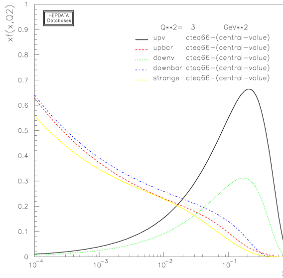
Figure 5.1: Parton distribution functions from the CTEQ6 parametrisation. In a simplified model all sea quark distributions can be considered roughly equal [52].
