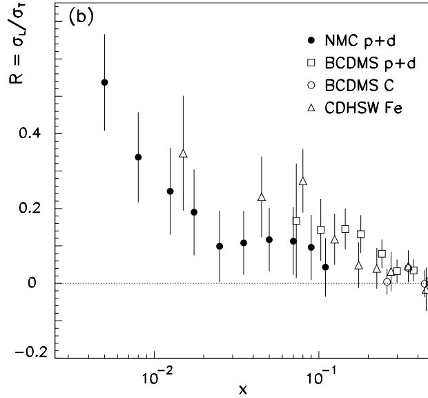
Figure 2.5: Measurements of R . The cross section ratio R = \sigma_L/\sigma_T = (F_2(1+\gamma^2) - 2xF_1)/(2xF_1) as a function of x . The mean value of Q^2 varies from 1.3 \text{ (GeV/c)}^2 in the first x bin to 20.6 \text{ (GeV/c)}^2 in the last x bin [8].
