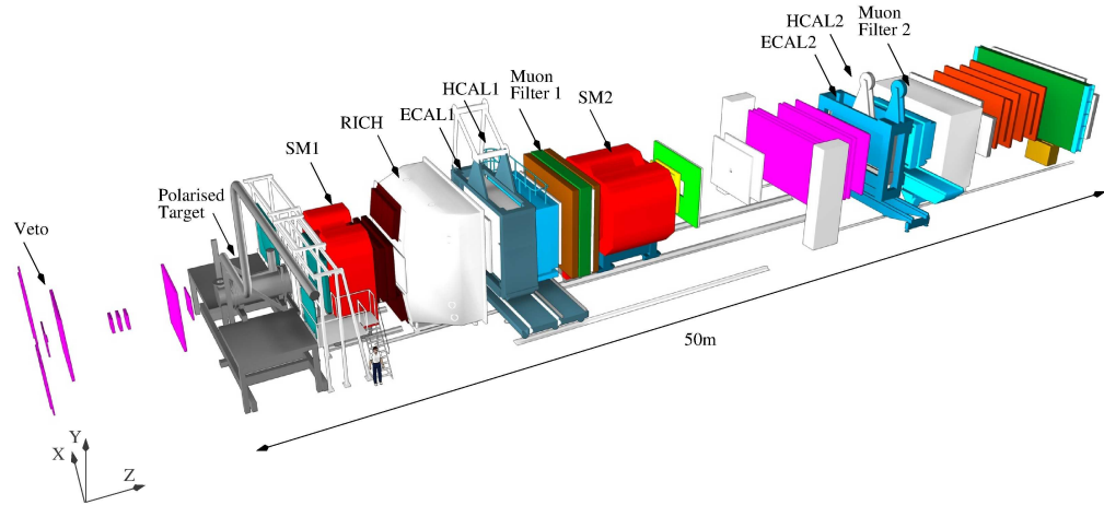
Figure 3.1: Artistic view of the COMPASS spectrometer [30]
