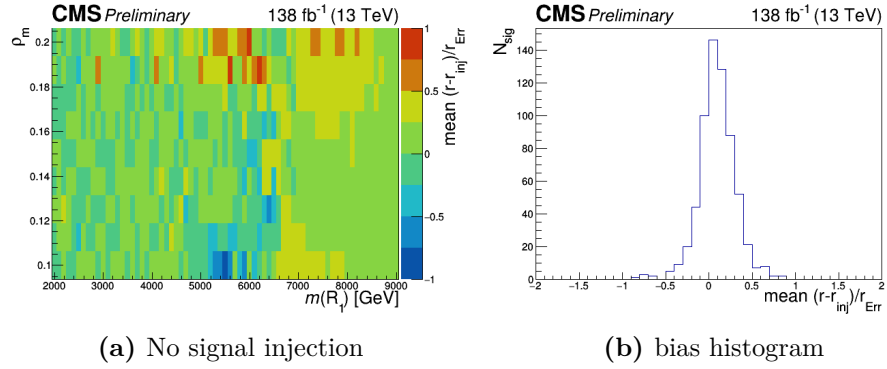
Figure 7.27. Same as Fig. 7.26, but for test performed without the signal injection.
