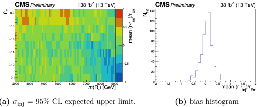
Figure 7.28. Left: bias versus \rho_m and m(R_1) from pseudodata generated with f_2 and fitted with f_1 . A signal is injected with a cross section equal to the expected limit. Right: 1D histogram of the bias ( N_{\text{sig}} = \# of signal hypotheses).
