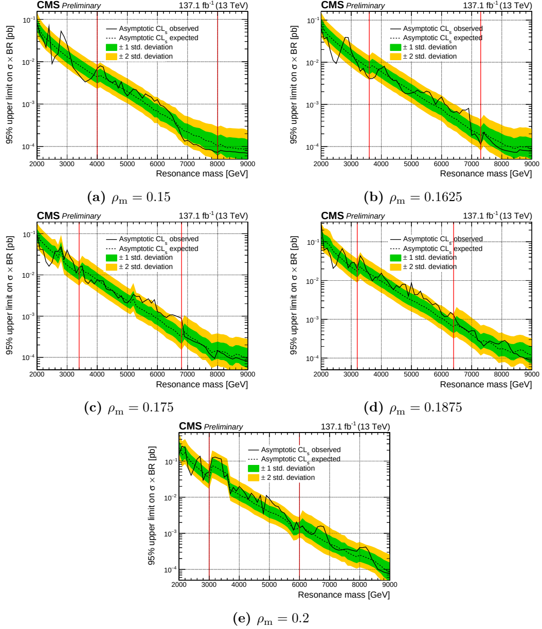
Figure 8.15. Expected (dashed line) and observed (solid line) 95% CL s limits on \sigma(G_{KK}) \times \mathcal{B} \times \mathcal{A} as a function of m(R_1) , for fixed \rho_m . Uncertainty bands ( \pm 1\sigma , \pm 2\sigma ) on expected limits are also shown. Discontinuities in expected limits are present in the transition between sets with different number of categories (red lines). The additional discontinuity for \rho_m = 0.2 at m(R_1) \approx 3.6 TeV is caused by the removal of one category from the final fit, following the procedure described in Sec. 7.3.2.
