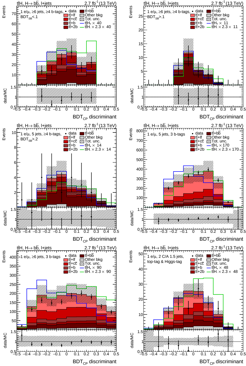
Figure 11.10: Six of the seven BDTs that are sensitive to the \text{t}\bar{\text{t}}\text{H} coupling structure. The observed distribution of data (black dots) is compared with the expected background predicted by simulation (stacked histograms). The signal with pseudoscalar coupling (green line) is scaled to the same integral as the sum of backgrounds. The expected SM signal is drawn as a blue line and scaled by a factor of 1/2.3 less than the CP odd signal, to account for the difference in total cross section. The most important systematic uncertainties are added in quadrature and shown as hashed error bands. Statistical uncertainties are drawn as black horizontal lines on the data points.
