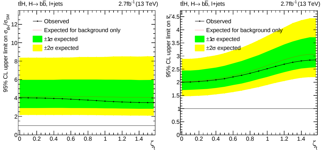
Figure 11.3: Observed and expected 95% CLs upper limit on the t\bar{t}H signal strength (left) and coupling strength \kappa_t (right) as a function of the scalar-pseudoscalar mixing angle \zeta_t , calculated with the asymptotic method. Observed limits are drawn as black lines and points, median expected limits as dashed red lines. The 1\sigma ( 2\sigma ) confidence intervals are shown as green (yellow) bands. \zeta_t = 0 corresponds to the Standard Model, \zeta_t = \pi/2 to a pseudoscalar boson.
