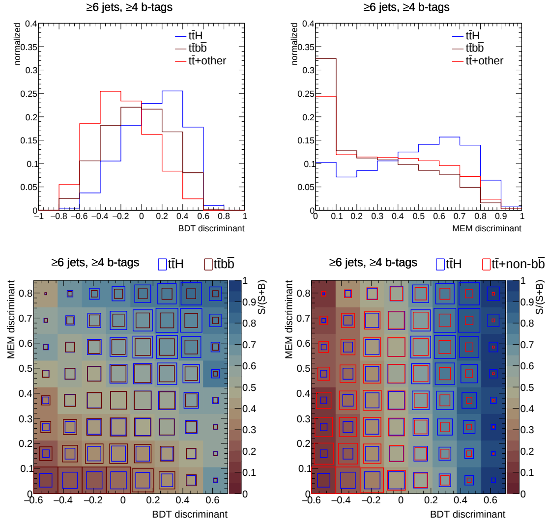
Figure 9.5: Top row: one-dimensional distributions of simulated t\bar{t}H(b\bar{b}) (blue), t\bar{t}b\bar{b} (dark red), and t\bar{t}\text{-non-}b\bar{b} (red) events in the \geq 6 jets, \geq 4 b-tags category. On the left-hand side for the BDT discriminant (without the MEM as input) and on the right-hand side for the MEM discriminant. Bottom row: Distribution of the same events in the space spanned by the MEM discriminant and the BDT discriminant. In the left plot, t\bar{t}H is compared with the t\bar{t}b\bar{b} background and in the right plot with the part of the t\bar{t} background not classified as t\bar{t}b\bar{b} . The relative contribution of the processes is indicated by the area of the rectangles. All processes are normalized to the same total integral. The background color is more blue in regions in which the fraction of t\bar{t}H events is larger and more red in regions where background dominates.
