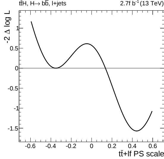
Figure 11.11: Twice the negative log-likelihood relative to the local minimum obtained at a t\bar{t} + l\bar{f} parton shower scale value of -0.35 . The likelihood is minimized with respect to all remaining nuisance parameters.
