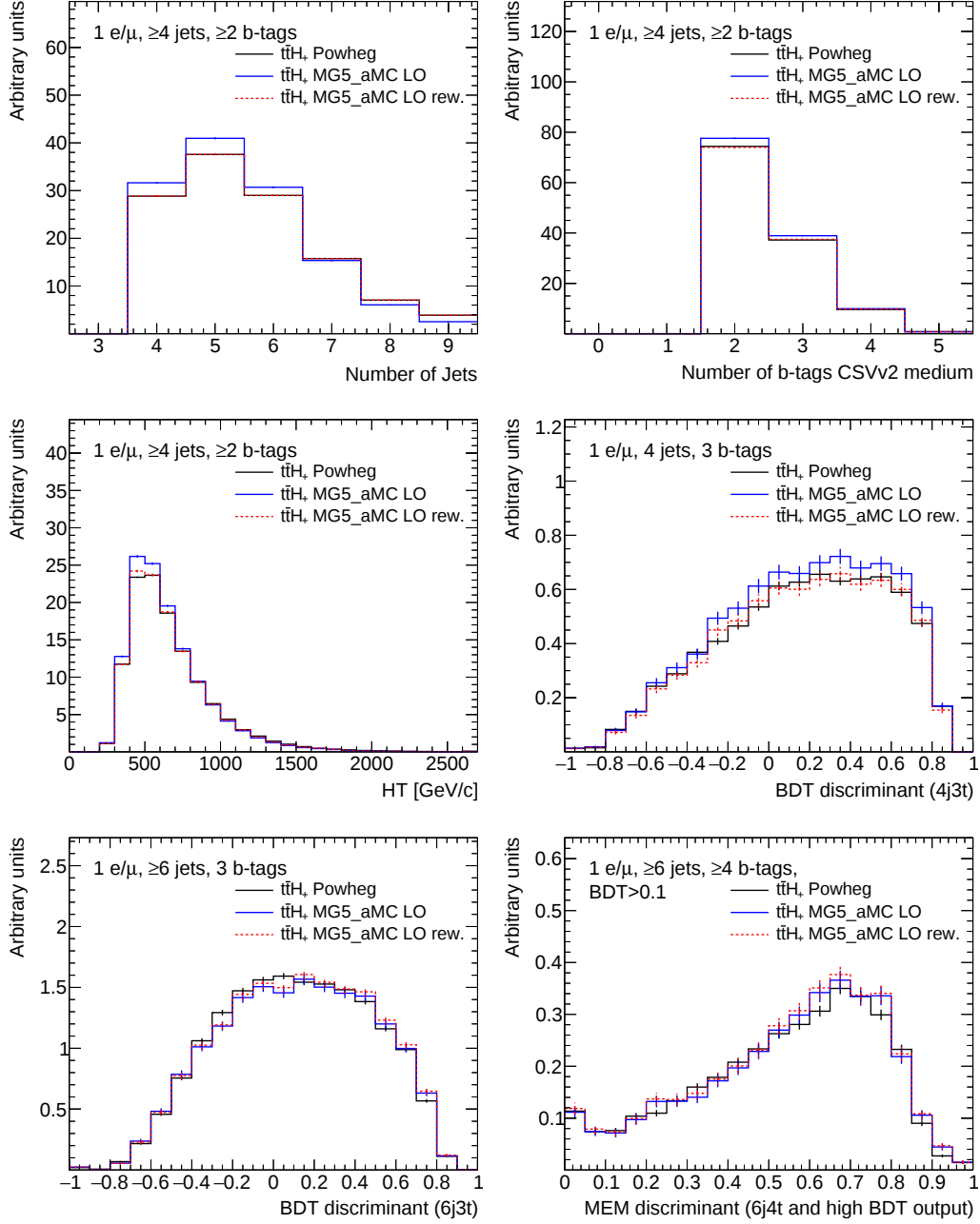
Figure 11.1: Comparison of the Powheg t\bar{t}H simulation (black line) with the privately produced MADGRAPH5_AMC@NLO leading order sample of t\bar{t}H_- (solid blue line) as well as to the latter sample after jet-multiplicity reweighting (dashed red line). Statistical uncertainties are indicated as vertical lines on the histograms. In the top row, jet and b-tag multiplicities are shown and the scalar sum of jet p_T is displayed in the middle row on the left-hand side. Moreover, three discriminants of the signal-strength analysis described in the previous chapter are shown in the middle row on the right-hand side and in the bottom row.
