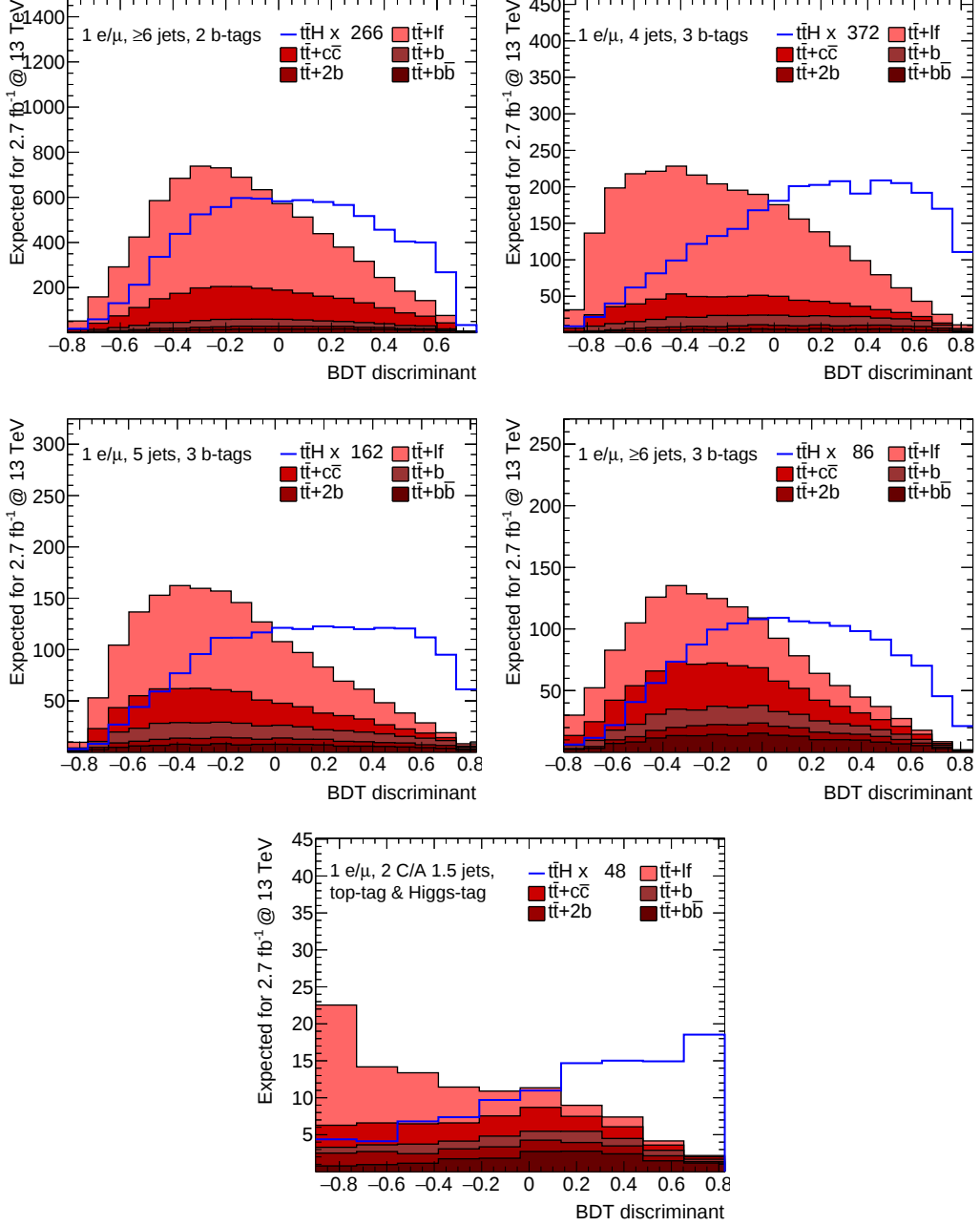
Figure 10.1: Distribution of simulated t\bar{t}H events (blue line) compared to the expected t\bar{t} background (stacked red histograms) for the five categories in that a BDT discriminant containing the MEM discriminant as input is used for signal-background separation. The t\bar{t} backgrounds are scaled to the number of events expected in the 2015 data, the t\bar{t}H signal is scaled to the background to allow for shape comparisons. The scaling factor is indicated in the legend.
