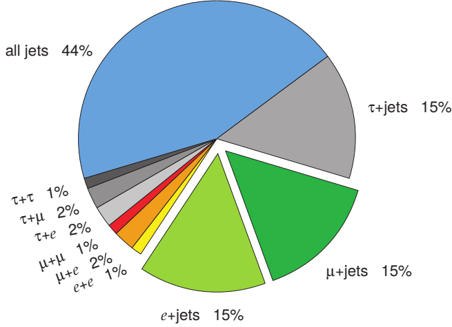
Figure 7.1: Relative size of the t\bar{t} decay channels, classified based on the number of charged leptons from the two W boson decays. Taken from [129].
