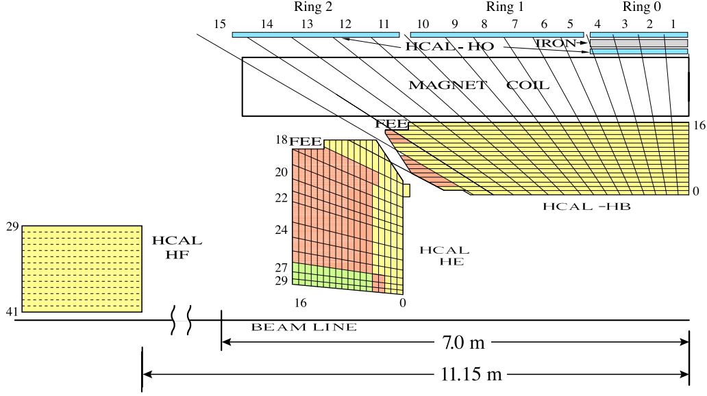
Figure 3.5: Cross section of a quarter of the CMS hadron calorimeter, taken from [99]. Displayed are the barrel, (HB), endcap (HE), outer (HO), and forward (HF) hadron calorimeters. The front end electronics are indicated as FEE. The color indicates independent longitudinal readouts.
