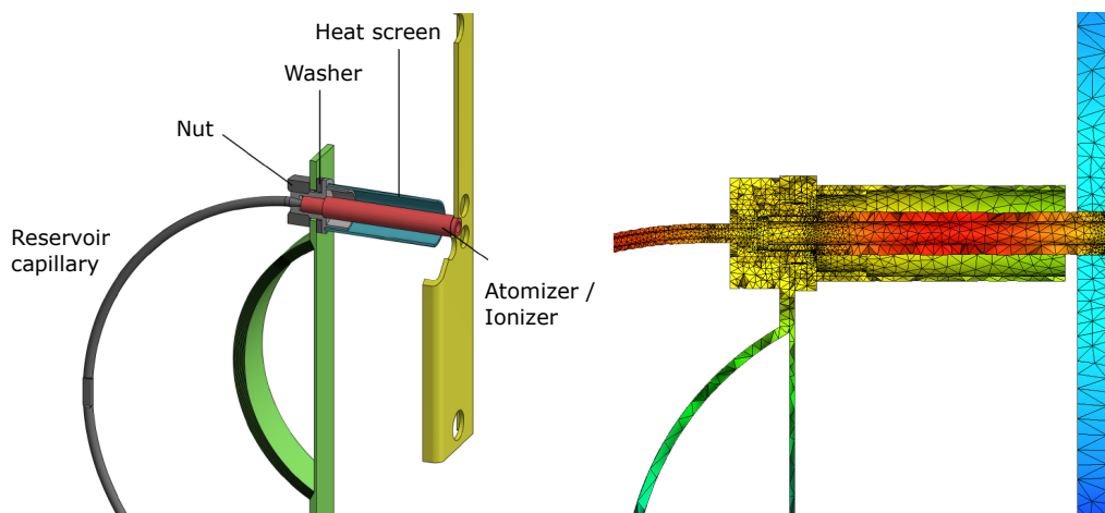
Figure 3.5: Left hand panel (adapted from [26]): CAD cut view of a RILIS setup as installed at the RISIKO mass separator. The ionizer cavity and reservoir capillary can be heated independently. Right hand panel (courtesy of T. Kieck): Simulation of temperature distribution using Autodesk CFD®. A significant gradient is apparent, in the presented case between 2000 °C at the center and 1500 °C at both end parts of the ionizer. Alternatively, a cavity which is completely closed at the hottest part can be used. See text for details.
