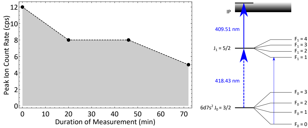
Figure 5.6: Interpolation of the signal rate in PI mode over the course of four longtime scans across the whole hyperfine structure, for assessment of its total efficiency. The count rate on the F_0 = 0 to F_1 = 1 transition as indicated on the right-hand scheme, yielding the highest ionization rate, was used. Comparison of the integrated amount of 38 520 ions to the sample size of 3.7 \cdot 10^9 atoms results in an efficiency value of 1.0 \cdot 10^{-5} .
