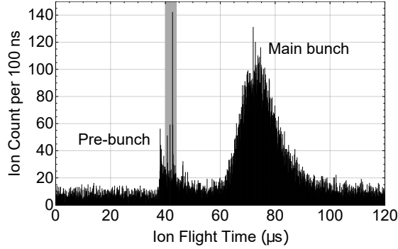
Figure A.7: Time structure of an ion bunch of laser-ionized ^{174}\text{Yb} from a standard RILIS source after transmission through the mass separator on nominal mass 174 u, acquired over several laser pulses. The interval marked in gray shows a very narrow feature within the pre-bunch of immediately extracted ions from the source: These spikes represent heavier ions which are created within the extraction field and which are transmitted on the trajectory of lower nominal mass through the magnet. Figure taken from [30].
