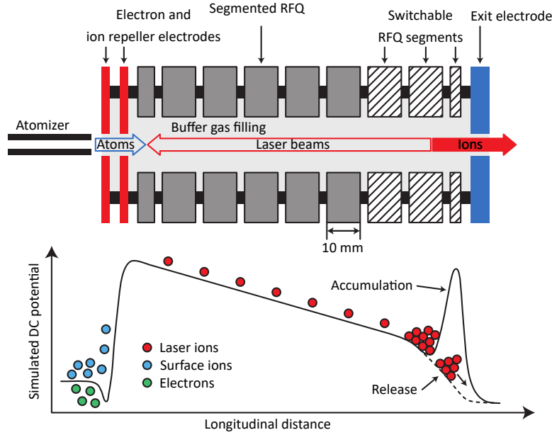
Figure 3.6: Schematic overview of the original setup of the Laser Ion Source and Trap LIST. Both ions and electrons from a hot atomizer are hindered from entering a radio-frequency quadrupole (RFQ) section filled with buffer gas. Ions created by laser radiation inside there are accumulated by a longitudinal guiding field imposed by segmentally controllable DC voltages on the rods. Finally, by switching the potential on the last segments and exit electrode, a contamination-free bunch of ions can be delivered to the beam line system. The bottom panel shows the respective longitudinal electric potential on the central axis, and the effect on the charged species. Figure adapted from [89].
