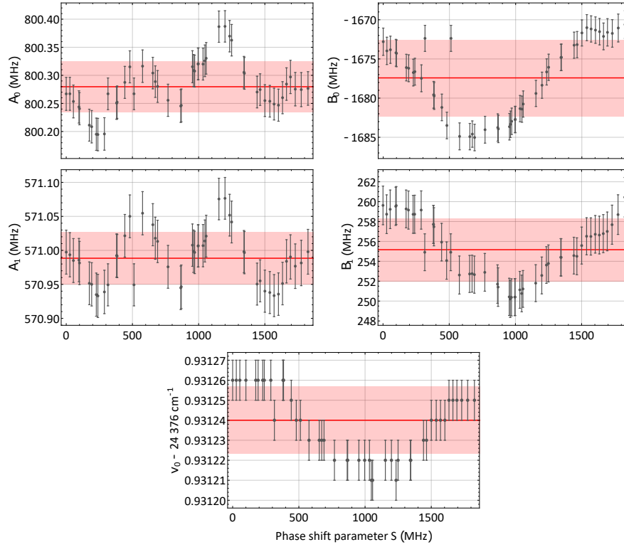
Figure 6.8: Dependence of extracted hyperfine parameters on the phase offset S . Respective mean values and standard deviations are indicated. See text for details.
