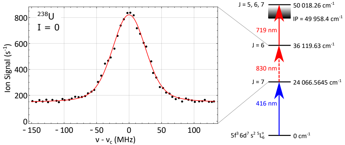
Figure 5.3: Overview of the laser resonance ionization scheme used for ^{238}\text{U} in the PI-LIST in standard configuration. The perpendicular, narrow bandwidth laser was scanned across the second step transition, indicated by the dashed arrow. The remaining steps were provided by broadband lasers in standard collinear geometry. Information on the first and second step was taken from [8, 112], while the third step was found by a quick manual search for auto-ionizing states. The scan of the second step transition on the left-hand side features an FWHM of 60(3) MHz with a dominating Gaussian contribution of 47(2) MHz.
