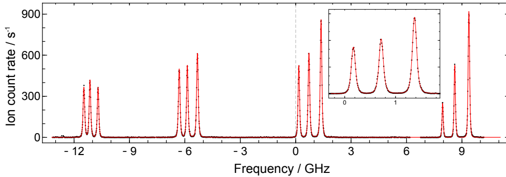
Figure 3.14: Hyperfine structure spectrum of the transition from the ground state 4d^5 5s^2 {}^6S_{5/2} to the excited state 4d^5 5s 5p {}^6P_{7/2}^o at 23\,265.32\text{ cm}^{-1} for ^{97}\text{Tc} with detailed view of the third triplet as inset. The fit of a Voigt profile to the data exhibits an overall FWHM of slightly below 100 MHz. Figure taken from [29].
