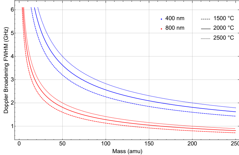
Figure 1.1: Doppler broadening of spectral linewidths in the optical regime for typical hot cavity vapor temperatures.
