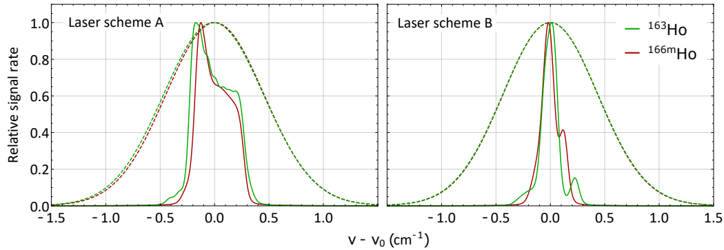
Figure 6.17: Simulated spectra of the two transitions investigated in this work, with adjusted line widths as they would occur in in-source operation. Besides the thermal Doppler broadening calculated from an oven temperature of 1500 °C, the dashed lines use the FWHM of 33(2) GHz as measured in [67], while the solid lines indicate the minimum possible resolution using a 1.4 GHz broad laser profile.
