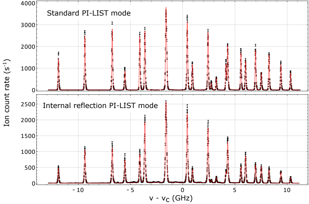
Figure 6.6: Full scans of the 1st step hyperfine structure of ^{165}\text{Ho} both in standard PI-LIST mode with lateral laser incoupling through a window in the ion source vacuum vessel, and internal reflection mode via the built-in metal mirrors. Frequency is given in respect to the transition’s measured center of \nu_c = 24\,376.9312(6)\,\text{cm}^{-1} . The fit using Voigt profiles exhibits an average FWHM of 99 MHz for the first and 114 MHz for the latter case. See text for details.
