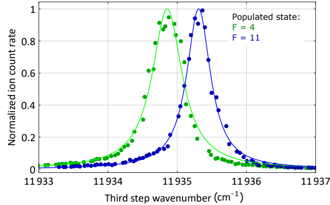
Figure 6.5: Laser wavelength scans of the third step broad band laser. The first step narrow band laser only populates one of the outer most hyperfine structure levels of the first excited state, and the second step laser is tuned to respective maximum signal rate according to fig. 6.4. The data is scaled to its respective maximum and fitted with a Lorentzian profile. Analog to the second step, a working point to guarantee ionization via all channels is found at the intersection at 11935.1 \text{ cm}^{-1} .
