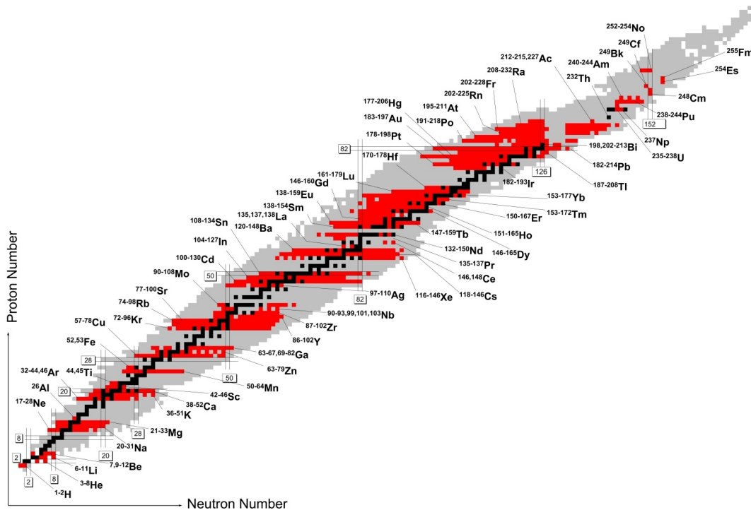
Figure 1.2: The chart of nuclides in respect to nuclear structure investigations by optical laser spectroscopy. Stable isotopes are shown in black, red squares indicate published result. “Magical” proton and neutron numbers are marked. The graphic was compiled and made publicly available online by the group of W. Nörtershäuser at TU Darmstadt.
