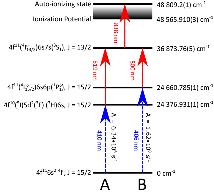
Figure 6.1: Holmium laser resonance ionization schemes, with the respective steps for hyperfine structure investigations marked by dashed lines. Scheme A denotes the dedicatedly chosen weak transition for highest possible spectral resolution, while scheme B is used for highly efficient ionization and implantation in the ECHo project [86]. Level configurations, energies and Einstein coefficients are taken from [86, 99, 122–124] and this work.
