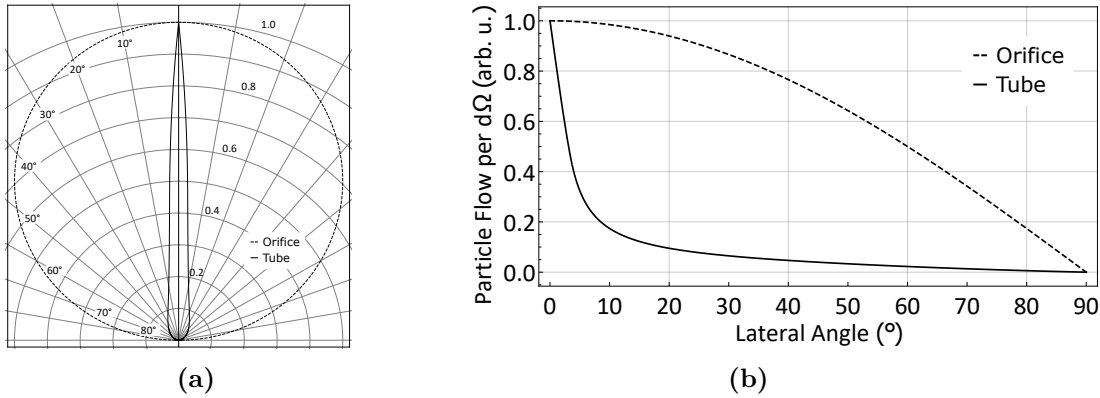
Figure A.1: Visualization of the atom beam shape (relative atom flow per solid angle element d\Omega ) in respect to lateral angle as predicted by models for a simple orifice [143] and a tubular channel [146] with the dimensions of the atomizer. Figure (a) follows the presentation in [146], while (b) gives the correlation in a direct way. Figures taken from [30].
