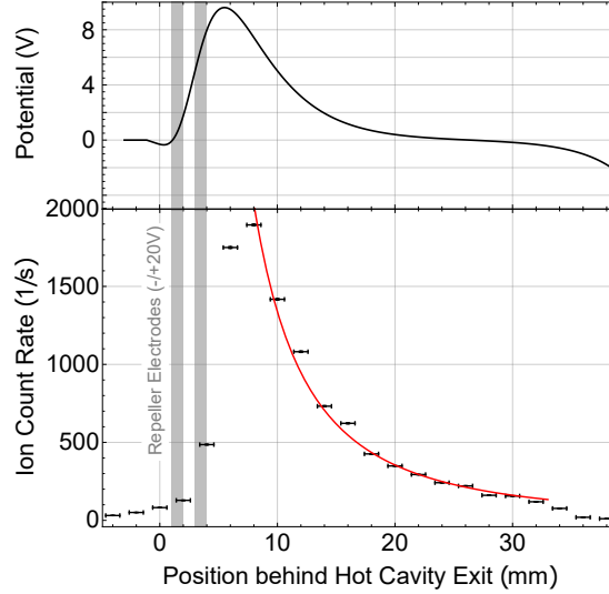
Figure A.3: Evolution of ion signal rate in a tubular volume defined by the diameter of the collinear lasers on the LIST's central axis as a function of distance from the hot cavity exit. After a steep increase behind the repelling electrode structure, up to where the top of the electric potential on the central axis (upper panel) is located. Subsequently, a reciprocally quadratic behavior is observed, fitted with a solid red line. Lower panel taken from [30].
