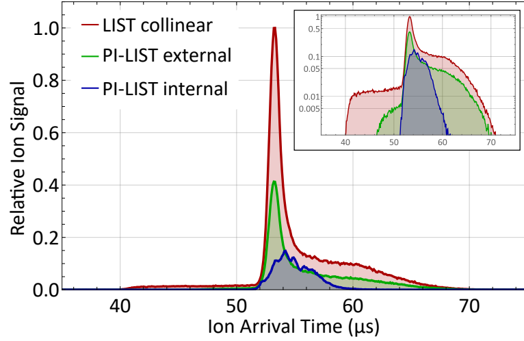
Figure 5.4: Ion bunch time structure for different operation modes of the LIST and PI-LIST, in linear and logarithmic scale. LIST and PI-LIST external reflect actual signal ratios for that setup, while the data for the internal reflection has been taken on a different occasion and is arbitrarily scaled. The structure clearly shows the different ionization volumes. See text for details.
