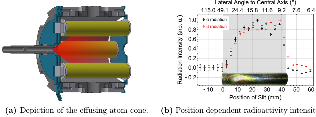
Figure A.10: (a) CAD view of the LIST with sketched emersion cone of atoms from the hot cavity, constrained by the repeller electrodes. (b) Spatial radiation screening of the LIST's four quadrupole rods after operation for long-lived radioisotopes over several months. The data is normalized to solid angle coverage. A photograph of one rod is shown for comparison to the heat radiation induced coloring, which also indicates direct line of sight to the hot cavity. The lateral angle is calculated in respect to a point 1.5 mm inside the hot cavity, as indicated from section A.1.3. Figures taken from [30].
