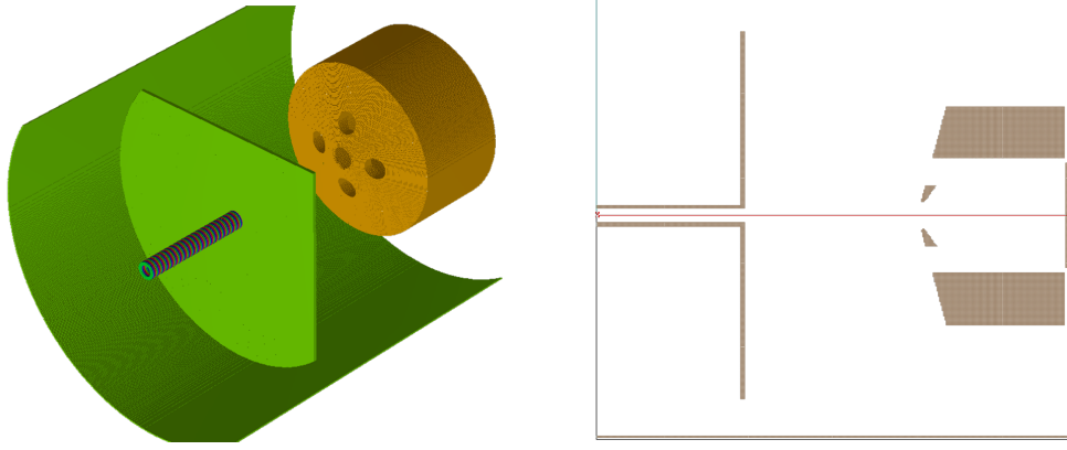
Figure 4.6: Overview of the simulation model as implemented in SIMION 8.1, at the example of the four side hole geometry. A 34 mm long cavity (with the ability to apply a longitudinal potential gradient) is placed 40 mm apart from the tip of the extraction electrode. Another 34 mm inside, the path is terminated by a solid “virtual” plate (on the same potential as the extractor), where simulated ions splat and their properties are recorded.
