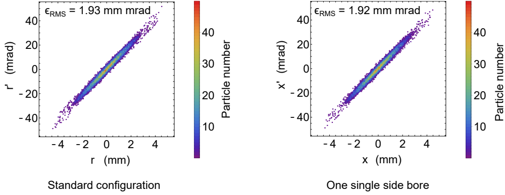
Figure 4.7: Exemplary density histogram plots for the emittance derived from simulations for the standard extractor geometry, and with one additional side bore. As well as in the absolute number for \epsilon_{\text{RMS}} , no significant difference is visible in the plot shape.
