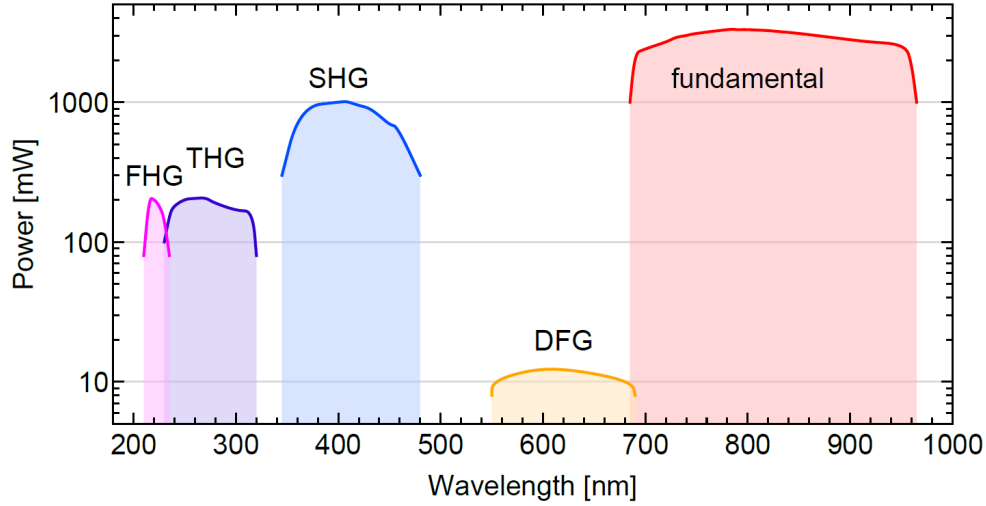
Figure 2.4: Accessible wavelength regimes of the Ti:sapphire, expanded by frequency conversion with maximum achievable power output. See text for details. Graph adopted from [66]
