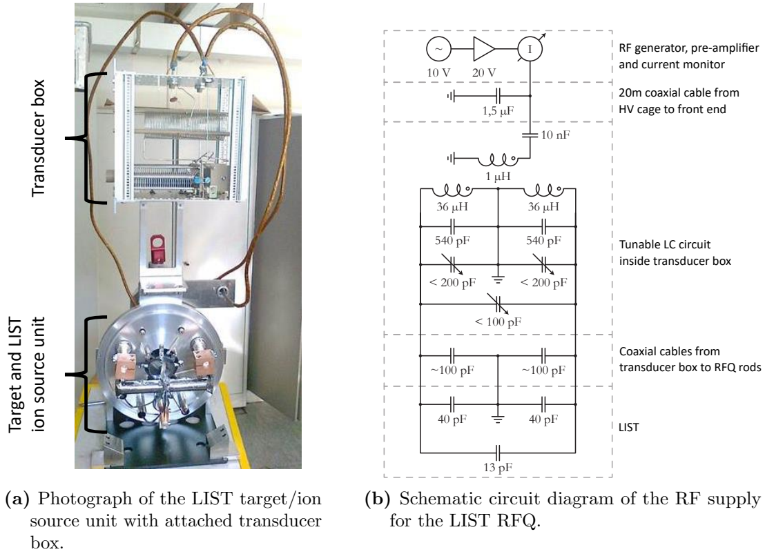
Figure 3.7: Overview of the LIST transducer box for transformation and symmetrization of the RF voltages for the RFQ as implemented for the harsh radiation environment at the ISOLDE on-line front ends. Figures adapted from [77].
