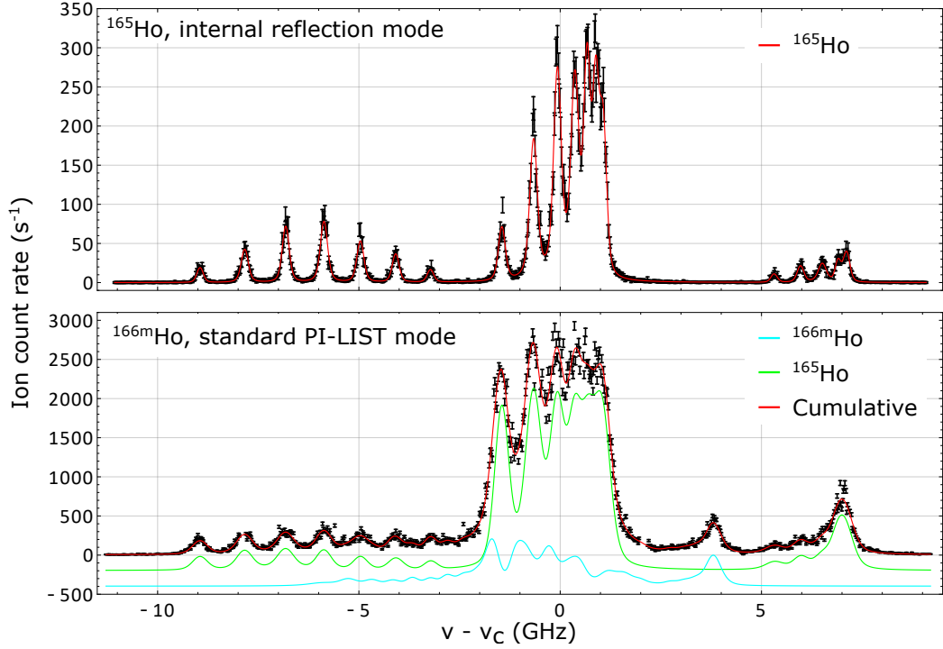
Figure 6.16: Recorded hyperfine structure patterns for ^{165}\text{Ho} and ^{166\text{m}}\text{Ho} in indicated operation mode on the “ECHO-transition” of laser scheme B in respect to the ^{165}\text{Ho} center frequency \nu_0 = 24\,660.7846(8)\,\text{cm}^{-1} . In the lower panel, the individual fit functions for both isotopes are shown with an artificial offset for better visibility. Although most of the ^{166\text{m}}\text{Ho} pattern is superimposed by interfering ^{165}\text{Ho} admixture, the structure between 2 and 5 GHz is reproduced. See text for details.
