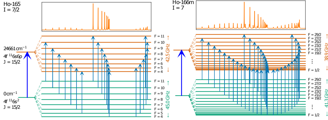
Figure 6.15: Schematic overview of the ^{165}\text{Ho} and ^{166\text{m}}\text{Ho} hyperfine structure pattern in the first step transition of laser scheme B as depicted in fig. 6.1.
