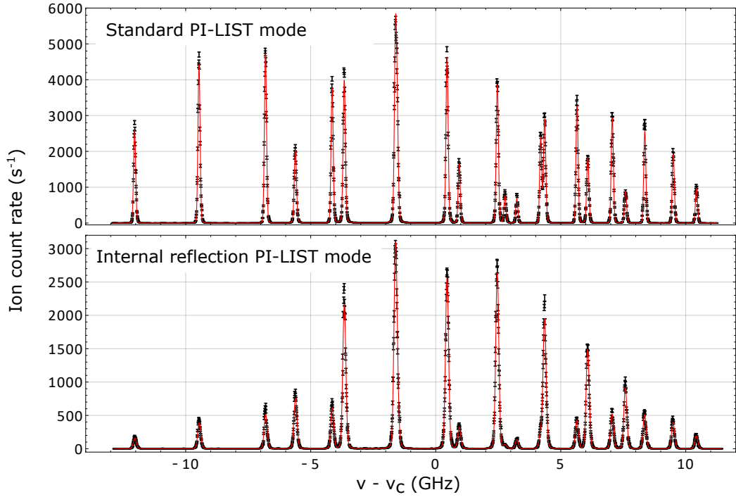
Figure 6.9: Full scans of the 1st step hyperfine structure of ^{163}\text{Ho} both in standard PI-LIST and internal reflection mode, relative to the transition's center frequency of 24\,376.9312(6)\,\text{cm}^{-1} .
