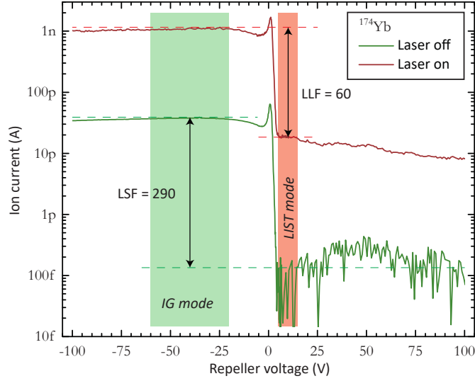
Figure 3.9: Exemplary repeller scan with the standard LIST as implemented at ISOLDE, measured on the isotope ^{174}\text{Yb} . Negative voltages resemble “standard” RILIS operation (IG mode), while positive voltages block all ions created in the hot cavity and only allow laser-ionized species from inside the RFQ structure in the beam (LIST mode). The LIST loss factor ( LLF ) describes the intensity loss between both situations, while the LIST suppression factor ( LSF ) gives the reduction of charged species from inside the hot cavity when the lasers are switched off. Figure adapted from [77].
