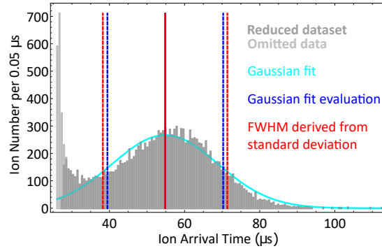
Figure A.17: Visualization of data handling for the simulation of direct extraction from the ion source, without a shielding LIST structure. The high peak at the very beginning stems from ions created at the exit of the source, where the penetrating extraction field causes transmission on lower nominal masses, thus they are omitted for evaluation. The resulting structure's width is extracted by the methods b) and c) described in the text.
