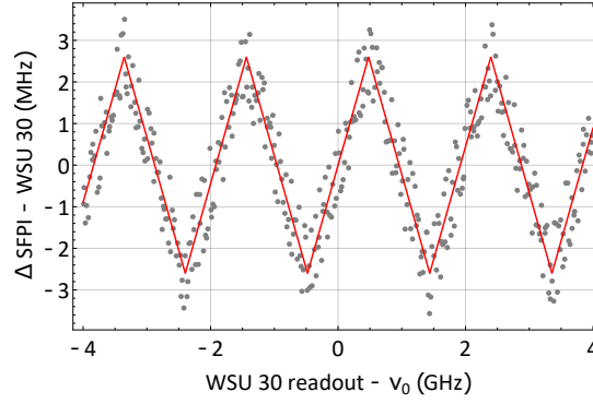
Figure 6.7: Visualization of the periodic, triangle-like deviation of the measured wavelength differences \Delta between WSU 30 readout and scanning Fabry-Perot interferometer (SFPI) in respect to the WSU 30 readout around an arbitrarily chosen absolute frequency \nu_0 . The red line is given by eq. 6.4, the data is randomly computer generated for illustration. Actual data is subject to an upcoming publication [127].
