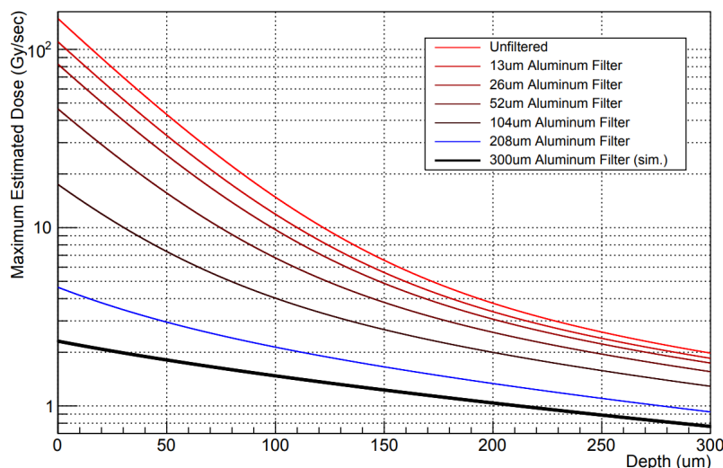
FIGURE 3.38. Maximum local estimated dose rate, in Gy/s, as a function of the depth in silicon, in \mu\text{m} , for different Al filters. A 100\ \mu thick Al filter is able to reduce the local dose rate at the surface by an order of magnitude, and in the bulk (at 150\ \mu\text{m} ) by a factor \sim 2 .
