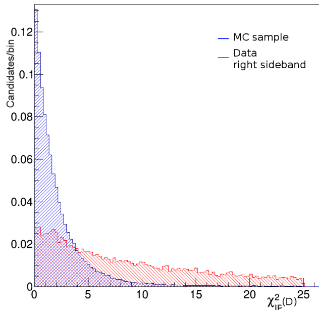
FIGURE 4.3. Normalised \chi^2_{\text{IP}} distributions for 2017 D^0 \rightarrow \pi^+ \pi^- \mu^+ \mu^- candidates, from MC sample (blue) and data right sideband (red) defined by m(D^0) > 1890 \text{ MeV}/c^2 , after the trigger, preselection and \Delta M cut.
