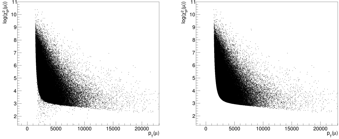
FIGURE 4.1. Scatter plot of the \log(\chi^2_{\text{IP}}(\mu_1)) with respect to p_T(\mu_1) before the TrackMuonMVA fiducial cut (left) and after the fiducial cut (right), for the 2016 D^0 \rightarrow \pi^+ \pi^- \mu^+ \mu^- data sample after the stripping selection and with only TrackMuonMVA_TOS on \mu_1 required.
