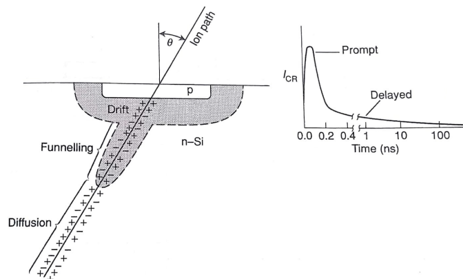
FIGURE 3.12. Scheme of e-h creation due to a ion passing through the device. The corresponding current pulse with the fast and slow components is shown on the right. Figure taken and modified from [276].
