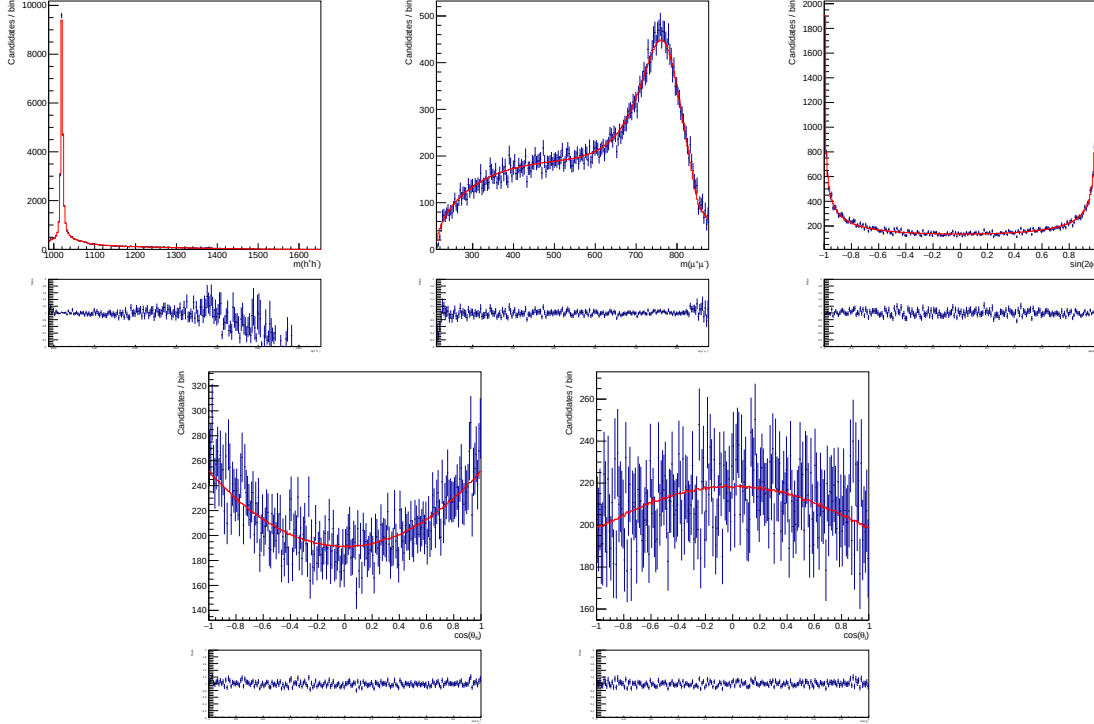
FIGURE 4.15. Phase-space distributions of simulated D^0 \rightarrow K^+ K^- \mu^+ \mu^- candidates at generator level (red) and fully selected and efficiency corrected (blue). The bottom panels show the ratio between the two distributions.
