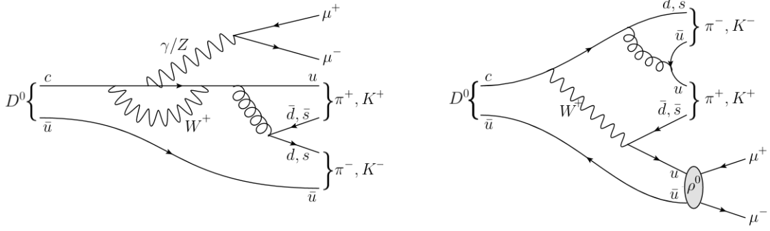
FIGURE 1.6. Example of two Feynman diagrams showing a SD penguin contribution to the D^0 \rightarrow \pi^+ \pi^- \mu^+ \mu^- decay (left), and a diagram representing a LD contribution via the \rho^0 meson decaying in two muons (right).
