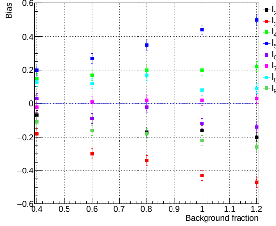
FIGURE 5.8. Bias of the fitted angular coefficients for the D^0 \rightarrow \pi^+ \pi^- \mu^+ \mu^- decay, integrated in m(\mu^+ \mu^-) spectrum, as a function of the background fraction sampled in each pseudoexperiment. The nominal background fraction as observed in data is equal to 1.
