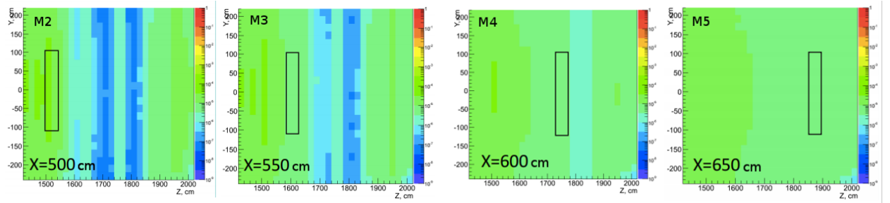
FIGURE 3.14. Output of the FLUKA simulations for hadrons fluence, measured in hadrons per collision per \text{cm}^2 , in the interesting regions near each station.
