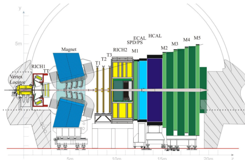
FIGURE 2.3. Scheme of the vertical section of the LHCb detector.
