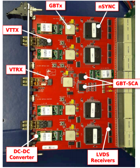
FIGURE 3.7. Picture of the first nODE prototypes, with the main components highlighted.
