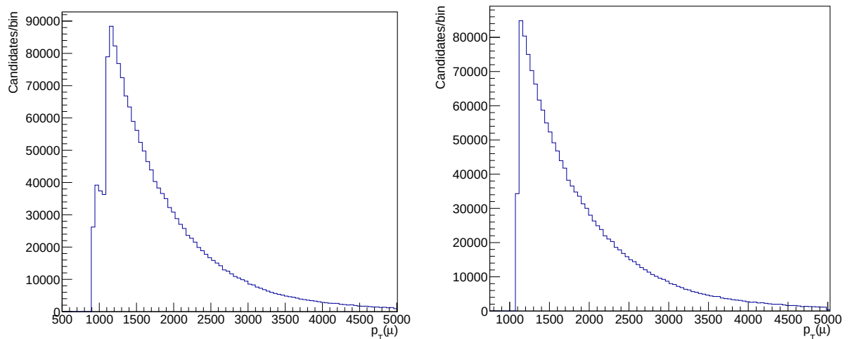
FIGURE 4.2. Distribution of p_T(\mu_1) before the TrackMuon fiducial cut (left) and after the fiducial cut (right), for the 2016 D^0 \rightarrow \pi^+ \pi^- \mu^+ \mu^- data sample after the stripping selection and with only TrackMuon_TOS on \mu_1 required.
