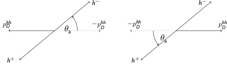
FIGURE A.2. Schematic representation of the variable \cos\theta_h for \bar{D}^0 (left) and D^0 (right). Modified from [300].
