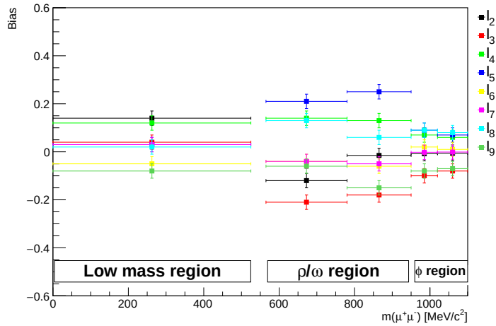
FIGURE 5.7. Bias of the fitted angular coefficients for the D^0 \rightarrow \pi^+ \pi^- \mu^+ \mu^- decay, in each m(\mu^+ \mu^-) region, with the observed Run II nominal signal and background yields.
