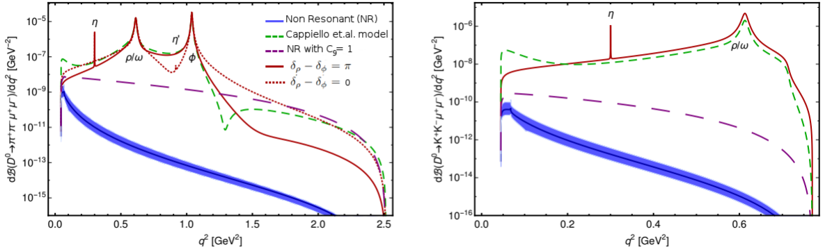
FIGURE 1.7. Differential branching fraction (modified from [168]) of D^0 \rightarrow \pi^+ \pi^- \mu^+ \mu^- (left) and D^0 \rightarrow K^+ K^- \mu^+ \mu^- (right) as a function of q^2 , considering different models to highlight the theoretical uncertainties on the strong phases. The Cappiello et al. model refers to the theoretical model used in [165].
