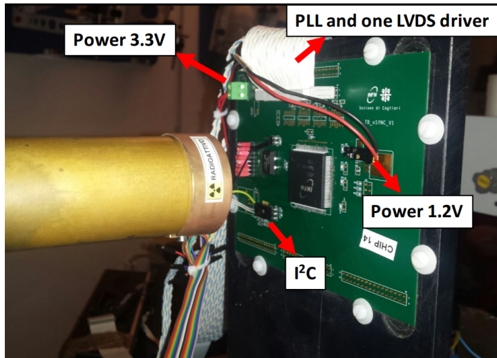
FIGURE 3.22. Picture of the nSYNC test board in front of the beam collimator. The I 2 C bus, the power connections and the probes for the PLL and LVDS drivers are highlighted.
