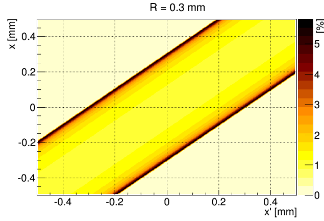
Figure 15: Visualization of the displacement of electrons on neighbouring bins. This is similar to the corresponding distortion matrix.
