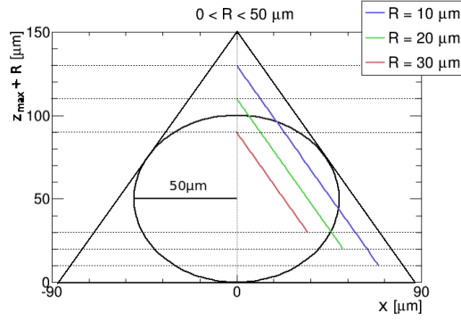
Figure 43: z_{\max} in dependency of x for different gyroradii for equilateral triangular sieve openings.
