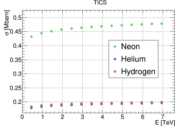
Figure 5: Total ionization cross sections for Hydrogen, Helium and Neon after equation (5) during the energy ramp. The Bethe coefficients are taken from table 2.
