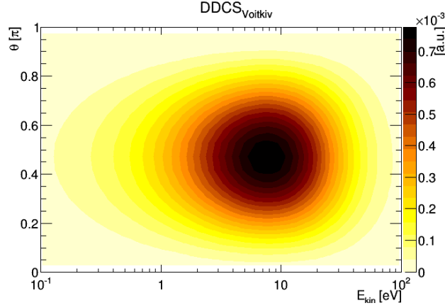
Figure 6: Double differential cross section for Neon after equation (6) for protons at 4 TeV and an effective charge of Z_t = 5.758 . The cross section is given in atomic units.
