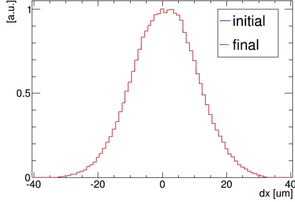
Figure 14: Deviation of the gyration centers of electrons at detector level from their production points with respect to x . The binning is 1 \mu m . The data was obtained for initial velocities corresponding to section 4.2.2.
