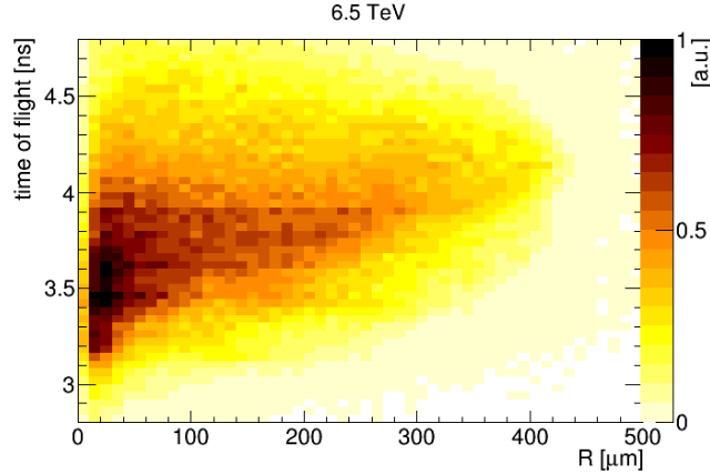
Figure 13: Time-of-flight distribution of electrons in dependency of their gyroradii. The binning is 0.04 ns for the time and 10 \mu\text{m} for the radius.
