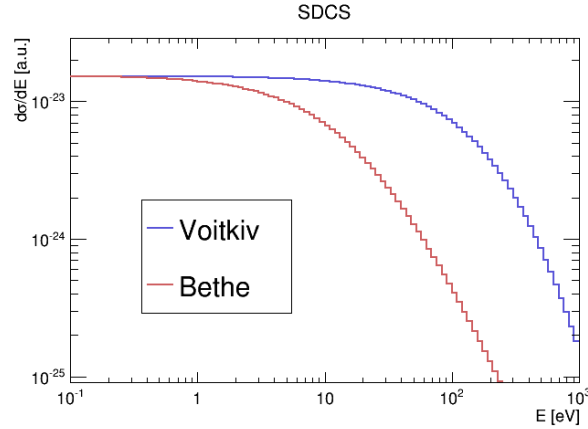
Figure 7: Single differential cross sections after Bethe and Voitkiv for protons at 4 TeV. The cross sections are scaled for comparison.
