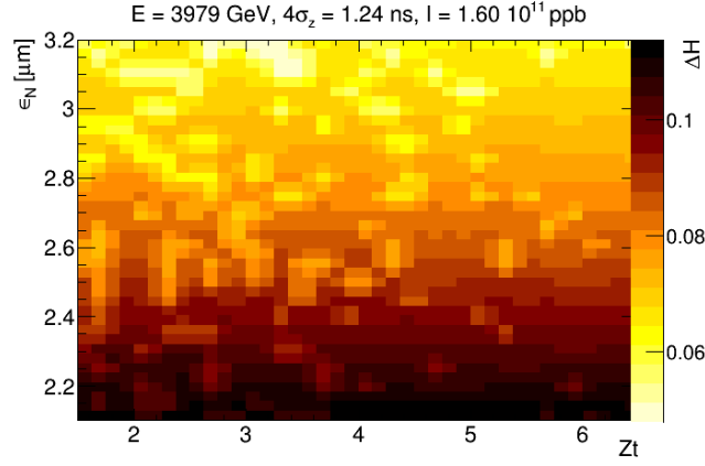
Figure 36: Results of the parameter scan for the effective charge Z_t of Neon. A profile obtained by the vertical device of beam 2 at E = 3979 \text{ GeV} , 4\sigma_z = 1.24 \text{ ns} , I = 1.60 \cdot 10^{11} \text{ ppb} was compared against the simulation results. \Delta H \equiv (\sum \Delta x_i^2)^{-1/2} / \sum x_i gives the relative deviation of the simulated profile from the reference profile. The binning is 0.2 and 0.05 \mu\text{m} for Z_t and \epsilon_N respectively.
