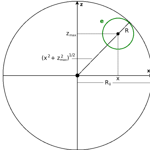
Figure 38: Visualization of the maximum free length z_{\max} at a given position x for circular sieve openings.
