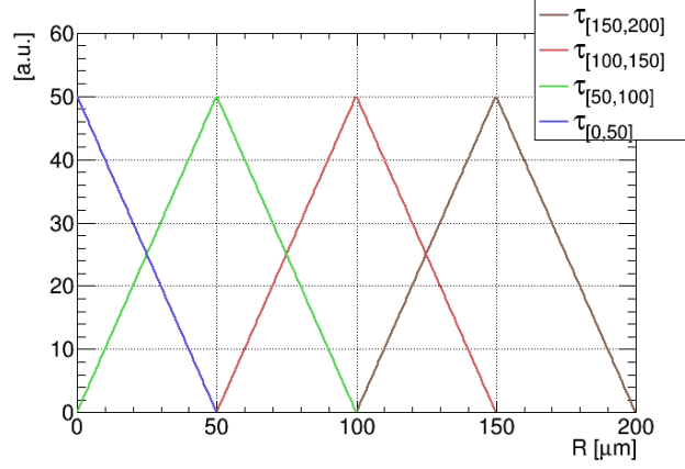
Figure 22: Transmission functions obtained by recursive subtraction of all preceding profiles.
