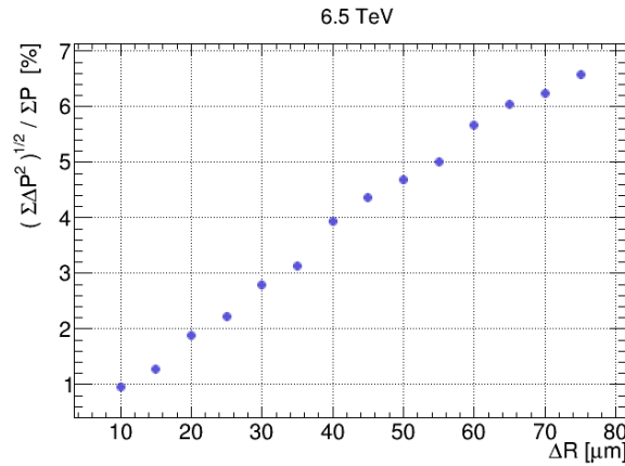
Figure 35: Deviation of the reconstructed profile from the original beam profile for different binnings of the sieve. The non-uniform transmission introduced by the sieve was considered. A single point spread function corresponding to the mean gyroradius of each interval was used.
