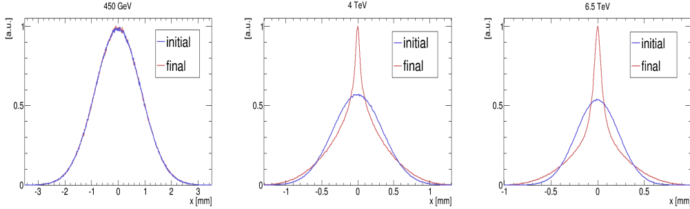
Figure 9: Profile distortion due to interaction with space charge for different beam energies.
