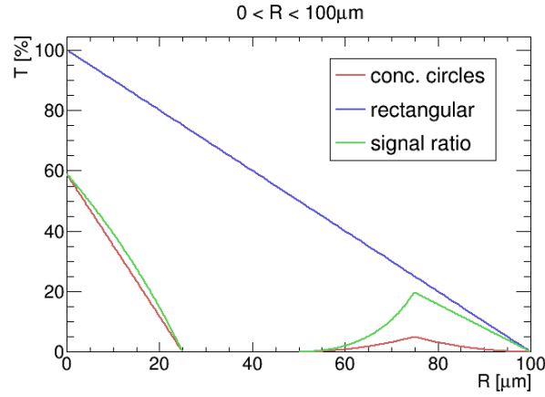
Figure 46: Transmission for concentric circles compared against the transmission for rectangular sieve openings.
