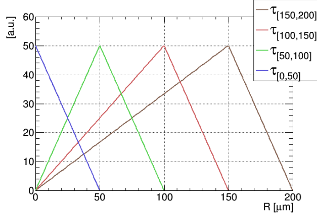
Figure 21: Transmission functions obtained by scaled subtraction of the preceding profile.
