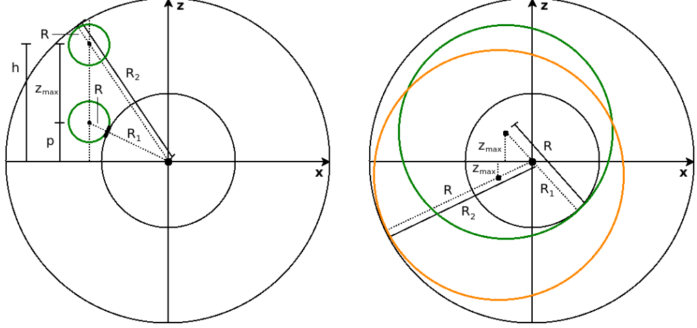
Figure 45: Visualization of the maximum free length z_{\max} at given positions x for a concentric circle geometry.
