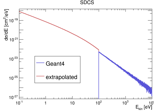
Figure 4: Single differential cross section resulting from the extrapolation of the Geant4 data for electron momenta.
