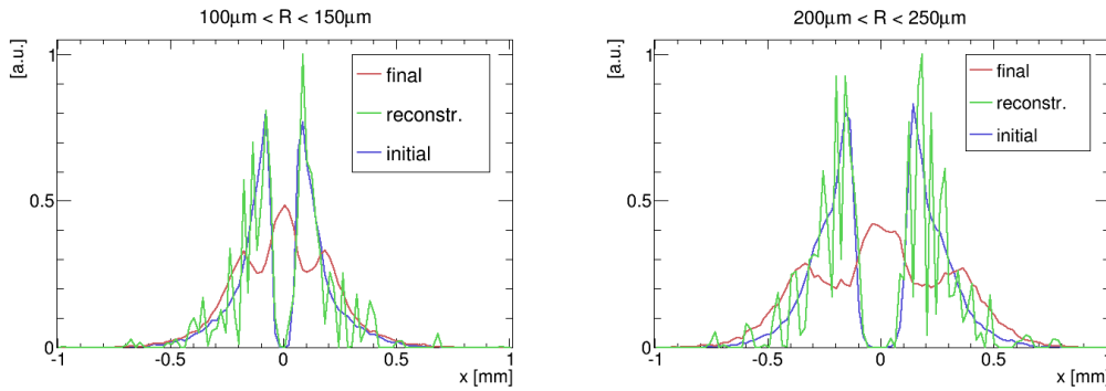
Figure 25: Reconstruction of two partial profiles. A uniformly weighted point spread function was used.
