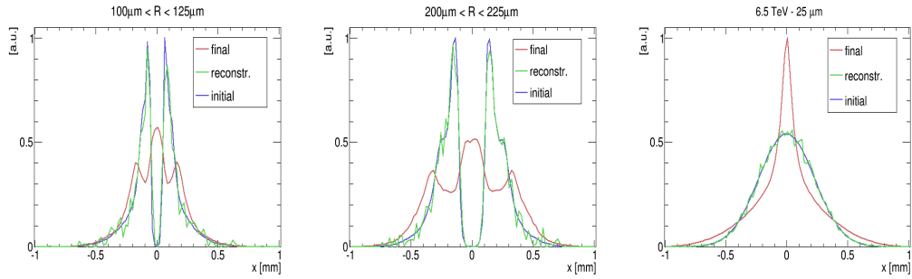
Figure 27: Reconstruction of the beam profile for a gyroradius binning of 25 \mu m . A uniformly weighted point spread function was used.
