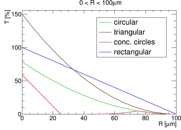
Figure 47: Comparison of the transmission for the different geometries.
