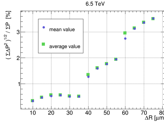
Figure 33: Deviation of the reconstructed profile from the original beam profile for different binnings of the sieve. A single point spread function corresponding to the mean and average value of each interval was used.
