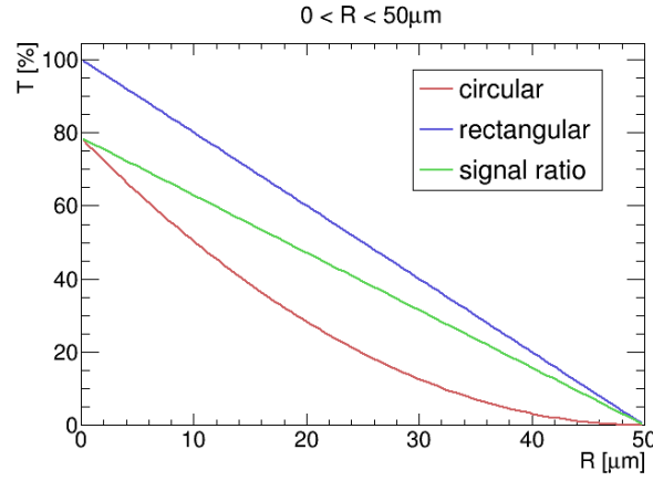
Figure 40: Transmission for circular sieve openings compared against the transmission for rectangular openings.
