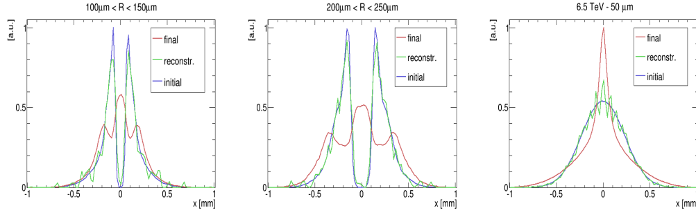
Figure 32: Reconstruction of the beam profile for a binning of 50 \mu m . A single point spread function corresponding to the average gyroradius of each interval was used.
