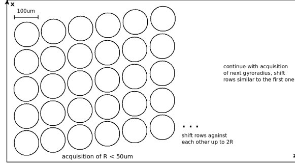
Figure 37: Sketch for a sieve with circular openings. Each partial profile is acquired by a group of rows where each row is slightly shifted against the previous one to ensure a uniform transmission along x .
