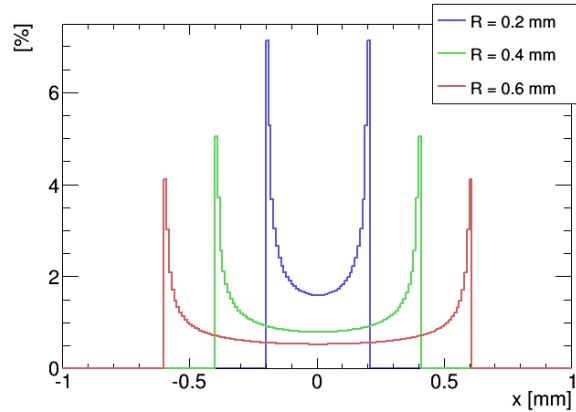
Figure 17: Point spread functions corresponding to different gyroradii.
