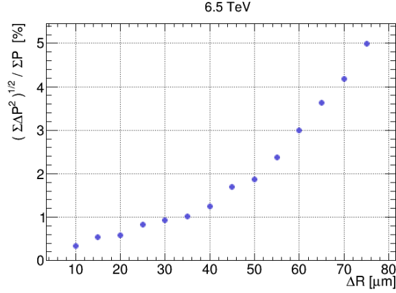
Figure 29: Deviation of the reconstructed profile from the original beam profile for different binnings of the sieve. A uniformly weighted point spread function was used.
