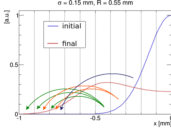
Figure 16: Visualization of the iterative reconstruction of the original profile for a known gyroradius.
