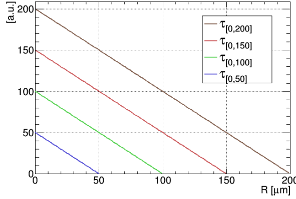
Figure 20: Plot of the different transmission functions for the example sieve of Fig. 18.
