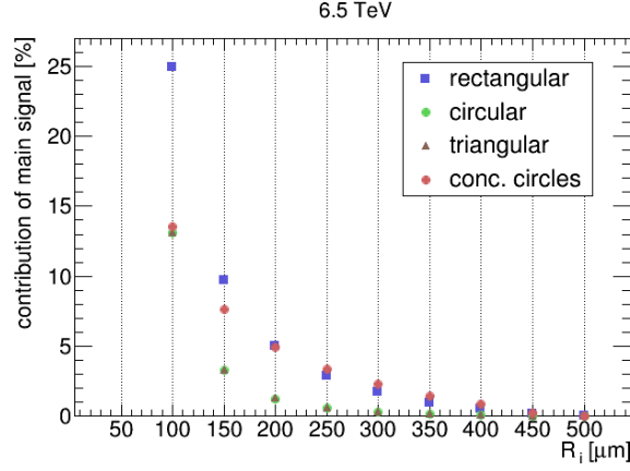
Figure 48: Contribution of the primary signal to the total signal that will be recorded by a group of sieve openings. R_i denotes the upper limit in gyroradius for each sieve opening.
