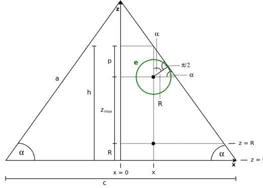
Figure 42: Visualization of the maximum free length z_{\max} at a given position x for triangular sieve openings.
