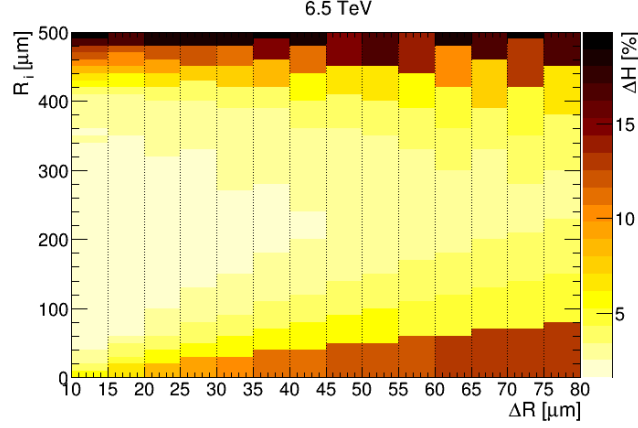
Figure 24: Quality of the assumption that the intrinsic profiles of each interval are uniform. The binning is 5\,\mu\text{m} for \Delta R and 1\,\mu\text{m} for the intrinsic profiles. The total range covered along R is always [0, 500]\,\mu\text{m} . \Delta H is the root mean square of the difference between the first and the last profile of each interval and is indicated on the full size of the respective interval.
