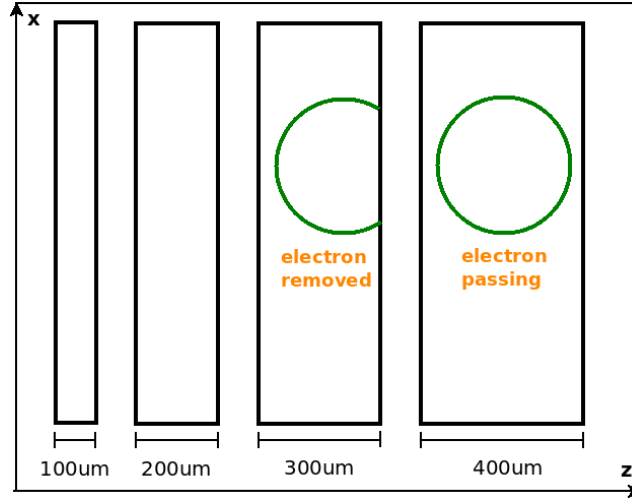
Figure 18: Sketch of an electron sieve with rectangular gaps. The electron on the right will pass through the sieve while the one on the left will be absorbed because its gyroradius is too large.
