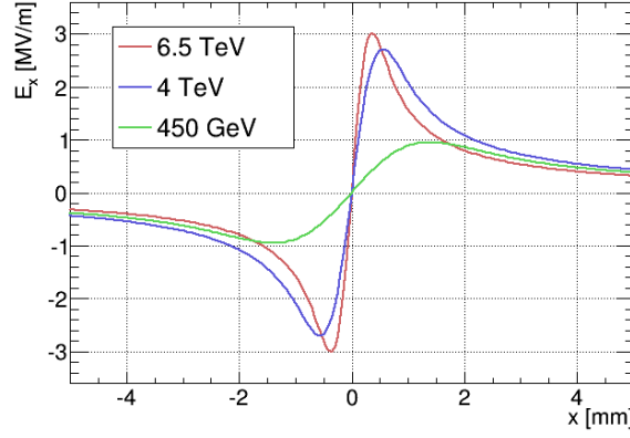
Figure 8: Bunch electric field along x for different beam energies (compare table 1).
