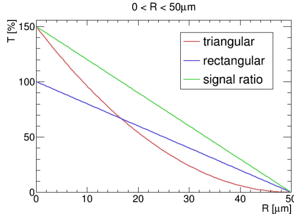
Figure 44: Transmission for equilateral triangular sieve openings compared against the transmission for rectangular openings.
