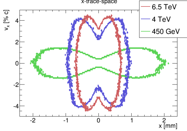
Figure 10: Trace space plots (95% surface) after space charge interaction for different beam energies. The binning is 10\ \mu\text{m} for x and 0.1\ \%c for v_x .
