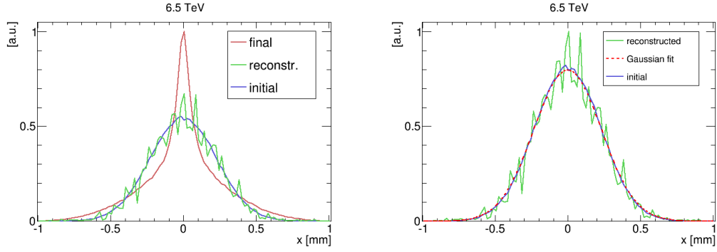
Figure 26: Reconstruction of the beam profile for a gyroradius binning of 50 \mu m . A uniformly weighted point spread function was used. The result is fitted with a Gaussian shape.
