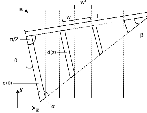
Figure 49: Sketch of a sieve with constant gap width and varying thickness. The sieve is tilted towards the magnetic field lines with the angle \theta .
