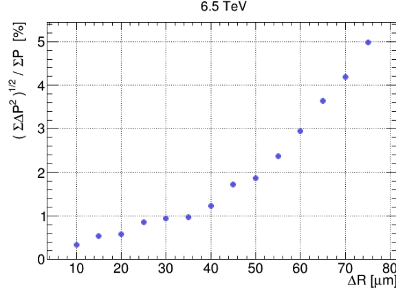
Figure 31: Deviation of the reconstructed profile from the original beam profile for different binnings of the sieve. A weighted point spread function with weights obtained after equation (33) was used.
