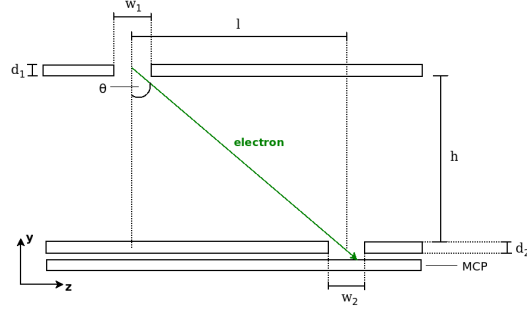
Figure 50: Sketch of two stacked sieves. The trajectory of the electron is indicated to be linear but in fact it is parabolic due to the acceleration by the external extraction field.
