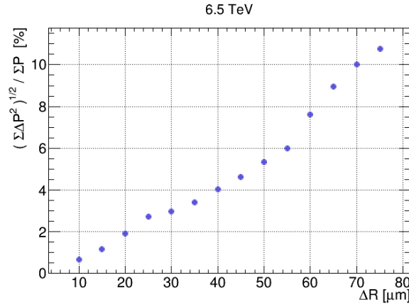
Figure 34: Deviation of the reconstructed profile from the original beam profile for different binnings of the sieve. The non-uniform transmission introduced by the sieve was considered. A weighted point spread function with weights obtained after equation (33) was used.
