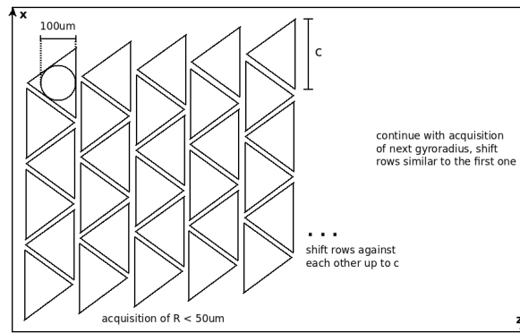
Figure 41: Sketch for a sieve with triangular openings. Each partial profile is acquired by a group of rows where each row is slightly shifted against the previous one to ensure a uniform transmission along x .
