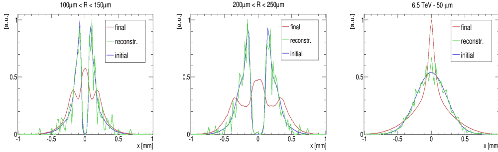
Figure 30: Reconstruction of the beam profile for binning of 50 \mu m . A weighted point spread function with weights obtained after equation (33) was used.
