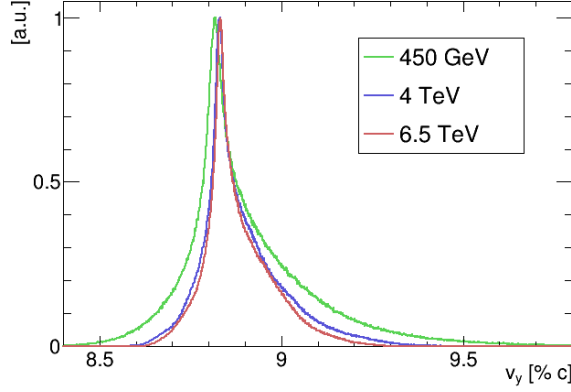
Figure 19: Electron velocities with respect to y at the moment of detection for different beam energies.
