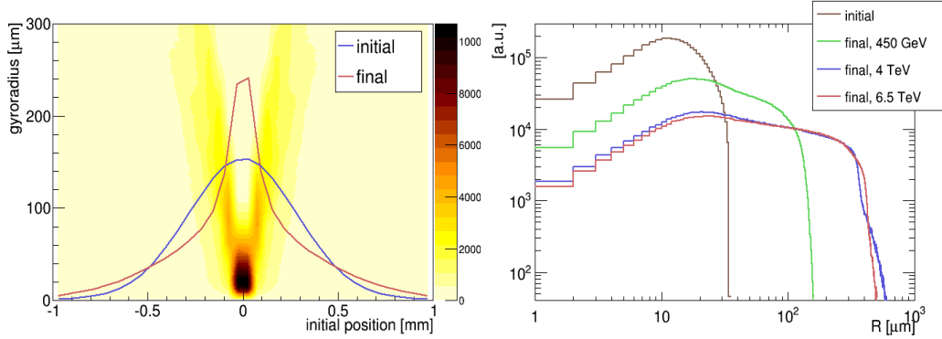
Figure 11: Impact of space charge on the gyroradius distribution of electrons. Left: Correlation between final gyroradii and initial x-position for the 6.5 TeV case. Right: Comparison of initial and final gyroradius distributions.
