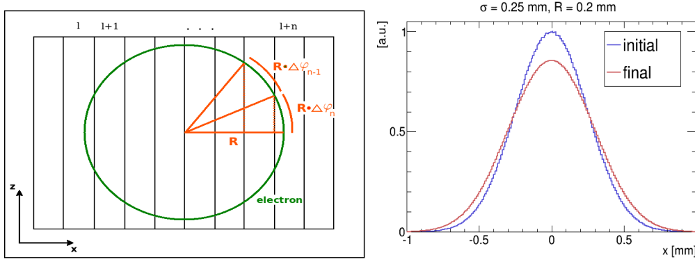
Figure 12: Mechanism of profile distortion due to spiraling of electrons. Left: Visualization of the gyration of electrons above the detector; for the sake of clarity the binning with respect to z has been spared. Right: Profile distortion due to a uniform gyration of electrons with gyroradii R = 0.2 \text{ mm} .
