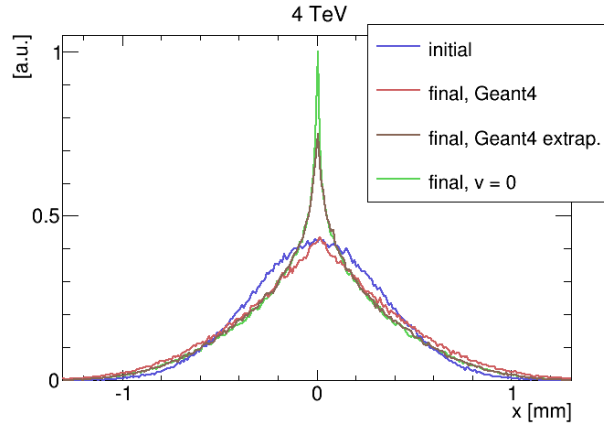
Figure 2: Comparison of the effect of different initial velocity distributions on the registered profiles (denoted by final ). Initial denotes the original beam profile. The obtained results include space charge effects.
