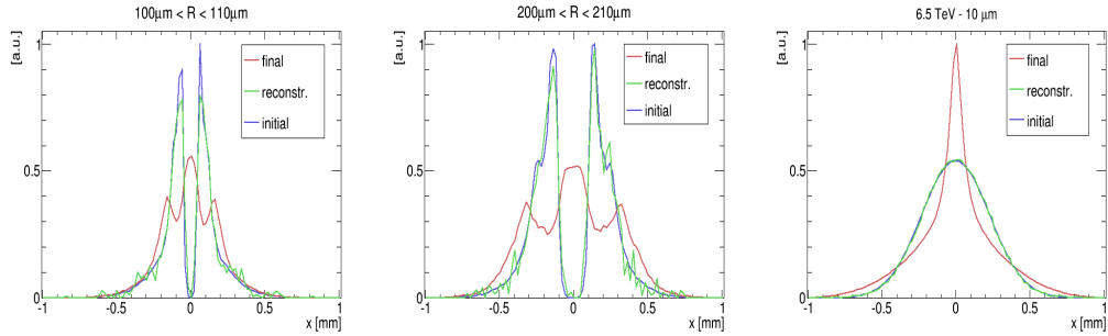
Figure 28: Reconstruction of the beam profile for a gyroradius binning of 10 \mu m . A uniformly weighted point spread function was used.
