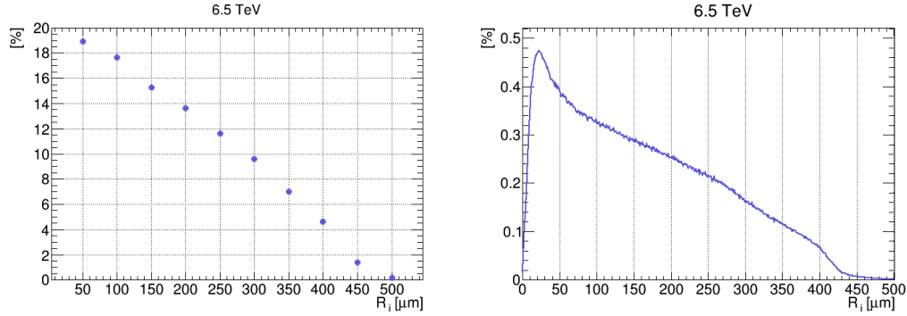
Figure 23: Percentage of electrons of different gyroradii to the final electron distribution. Left: Binning is 50 \mu m ; Right: Binning is 1 \mu m .
