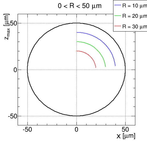
Figure 39: z_{\max} in dependency of x for different gyroradii for circular sieve openings.
