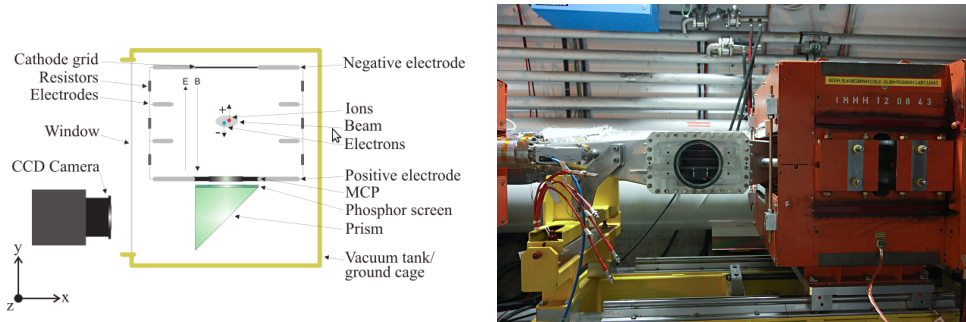
Figure 1: Left: Operating principle of an Ionization Profile Monitor [2, H.Refsum]. Right: Picture of one of the horizontal devices in the LHC; the magnet (orange) is shifted, the window for the camera is visible [2].
