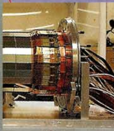
CMS-CERN
