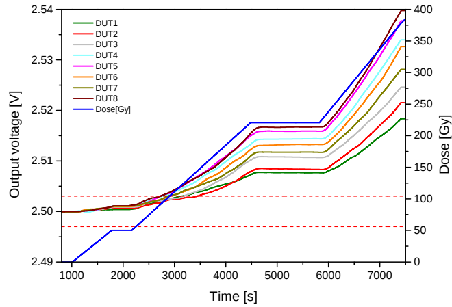
Figure 9.12: Measured output voltage of the ADR421 in relation to the increasing TID. Due to beam stops during the measurement the TID is plotted as separate graph over the measurement time. The red dotted line shows the tolerance to be expected due to production [61]. As can be seen the cumulative damage due to TID causes the output voltage to increase.
