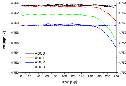
Figure 9.5: Drift of the maximum of the MAX1162 ADC data (top) and a close up view of the range until 220 Gy. This drift is caused by to the influence of cumulative damage to the ADC silicon fabric.
