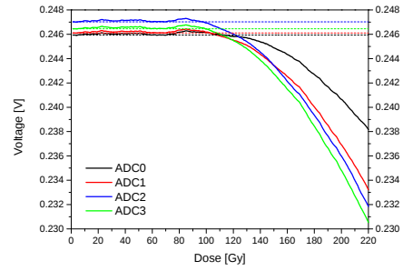
Figure 9.6: Drift of the minimum of the MAX1162 ADC data (top) and a close up view of the range until 220 Gy. This drift is caused by to the influence of cumulative damage to the ADC silicon fabric.
