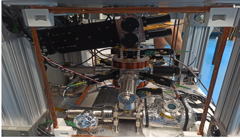
Fig. 3. Six lasers (blue wires with green stripes) are used for optical molasses and manipulation. At the bottom, the instrument for thermally vaporizing caesium atoms is visible. The copper cylinder houses a Helmholtz coil, which generates a magnetic field to trap the atoms based on their magnetic properties,
