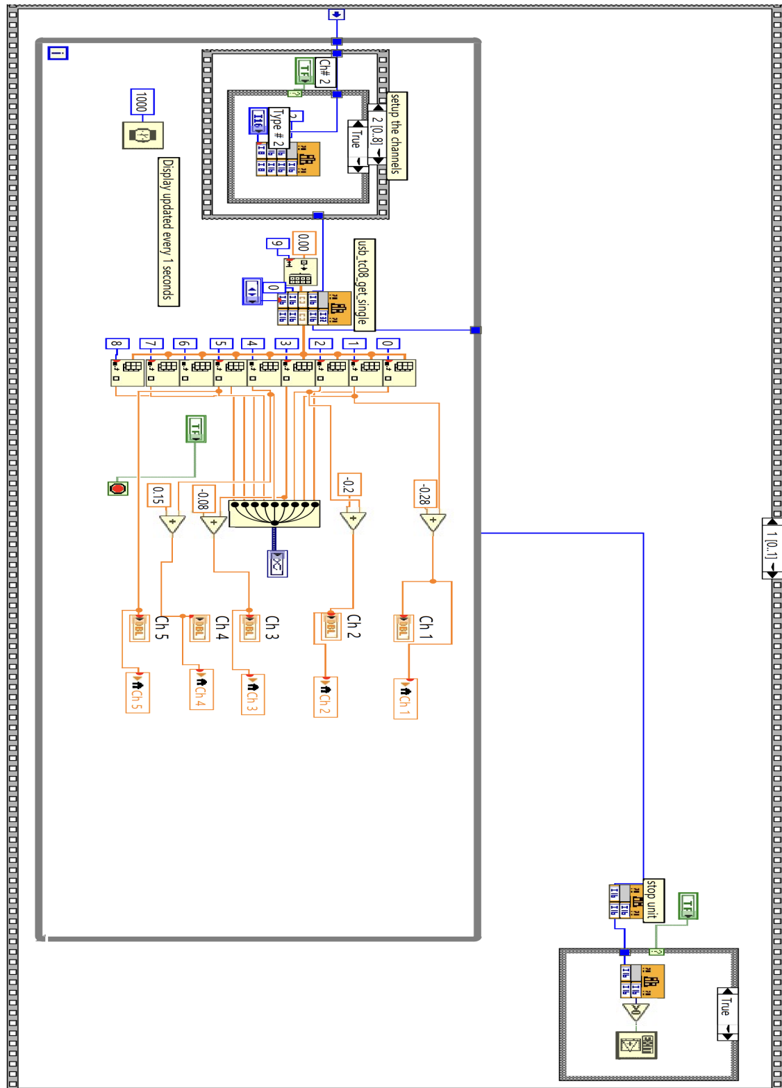
Fig. 7. Acquiring the temperatures via the thermocouples
