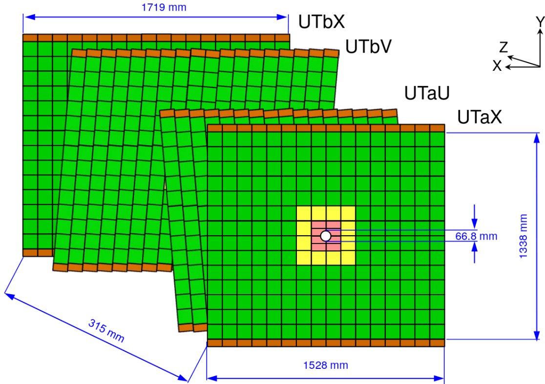
Figure 2.4: UT geometry overview, looking downstream [11]. The pink sensors have a pitch of 93.5\text{ }\mu\text{m} and a length of around 5 cm, the yellow sensors have the same pitch, but double the length, and the green sensors have a pitch of 187.5\text{ }\mu\text{m} at 10 cm of length.
