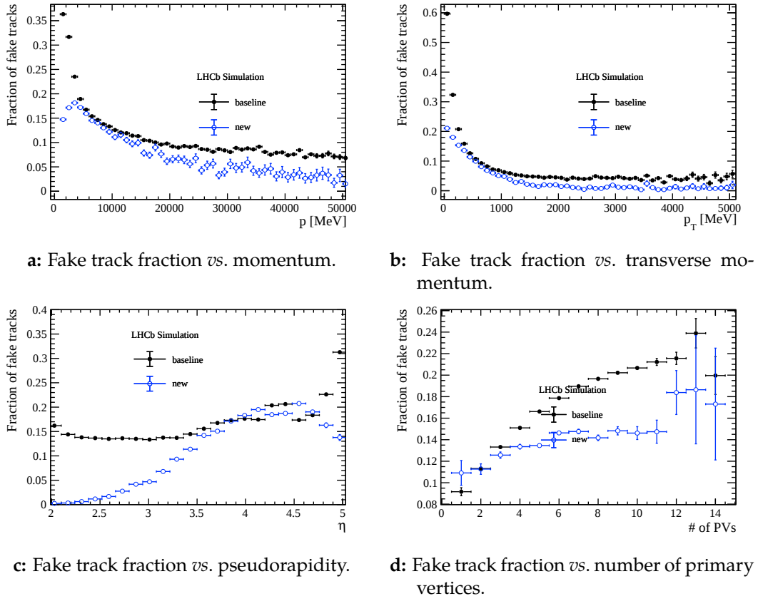
Figure 7.10: Fake track fraction of the electron Matching algorithm with perfect VELO and T track selection of input tracks in dependence on kinematic variables and the number of primary vertices.
