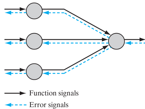
Figure 2.8: Illustration of the directions of signal flows in an MLP [16].
