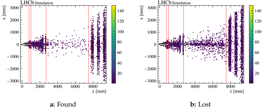
Figure 6.3: Distributions of bremsstrahlung vertices where more than 0.1 of the electron’s current energy is emitted. The distributions are representative of the same amount of electrons. The red lines in the plots mark the sub-detectors’ locations ( l.t.r. : end of the VELO, beginning of the RICH1, end of the UT, and beginning of the SciFi tracker).
