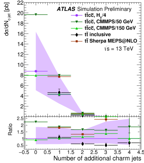
Figure 8.3.: The differential cross section as a function of the number of the charm jets not produced as part of the top quark decay chain. A cut at 0.4 was applied on the fraction of the charm hadron p_T w.r.t. the p_T of the corresponding jet. The predictions of the zero c -jet bin from the inclusive t\bar{t} and Sherpa samples lie above the range of the axis. The band around the sample generated with the H_T/4 scale option and the bars on the inclusive t\bar{t} sample show the simultaneous variations of the renormalisation and factorisation scales by factors of 1/2 and 2 . For the other samples, only the statistical uncertainties are shown. All samples are normalised to the respective fiducial cross sections and the ratio in the lower pane is given w.r.t. the calculation with the H_T/4 scale option. Taken from [175].
