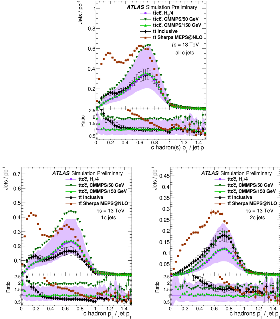
Figure 8.1.: The fraction of the charm hadron p_T w.r.t. the p_T of the corresponding charm jet. The upper shows all charm jets, whereas only jets with exactly one associated c -hadron (1c-jets) are shown in the lower left plot and only jets with two or more associated c -hadrons (2c-jets) are shown in the lower right figure. The band around the sample generated with the H_T/4 scale option (lilac circle markers) and the bars on the inclusive t\bar{t} sample (black diamond markers) show the simultaneous variations of the renormalisation and factorisation scales by factors of 1/2 and 2. For the other samples, only the statistical uncertainties are shown. All samples are normalised to the respective fiducial cross sections and the ratios in the lower panes are given w.r.t. the calculation with the H_T/4 scale option. The charm p_T fraction may exceed unity since the jets are built from stable particles, i.e. particles with a mean lifetime \tau > 3 \cdot 10^{-11} s, and stable decay products of the charm hadron may end up outside of the jet cone. Taken from [175].
