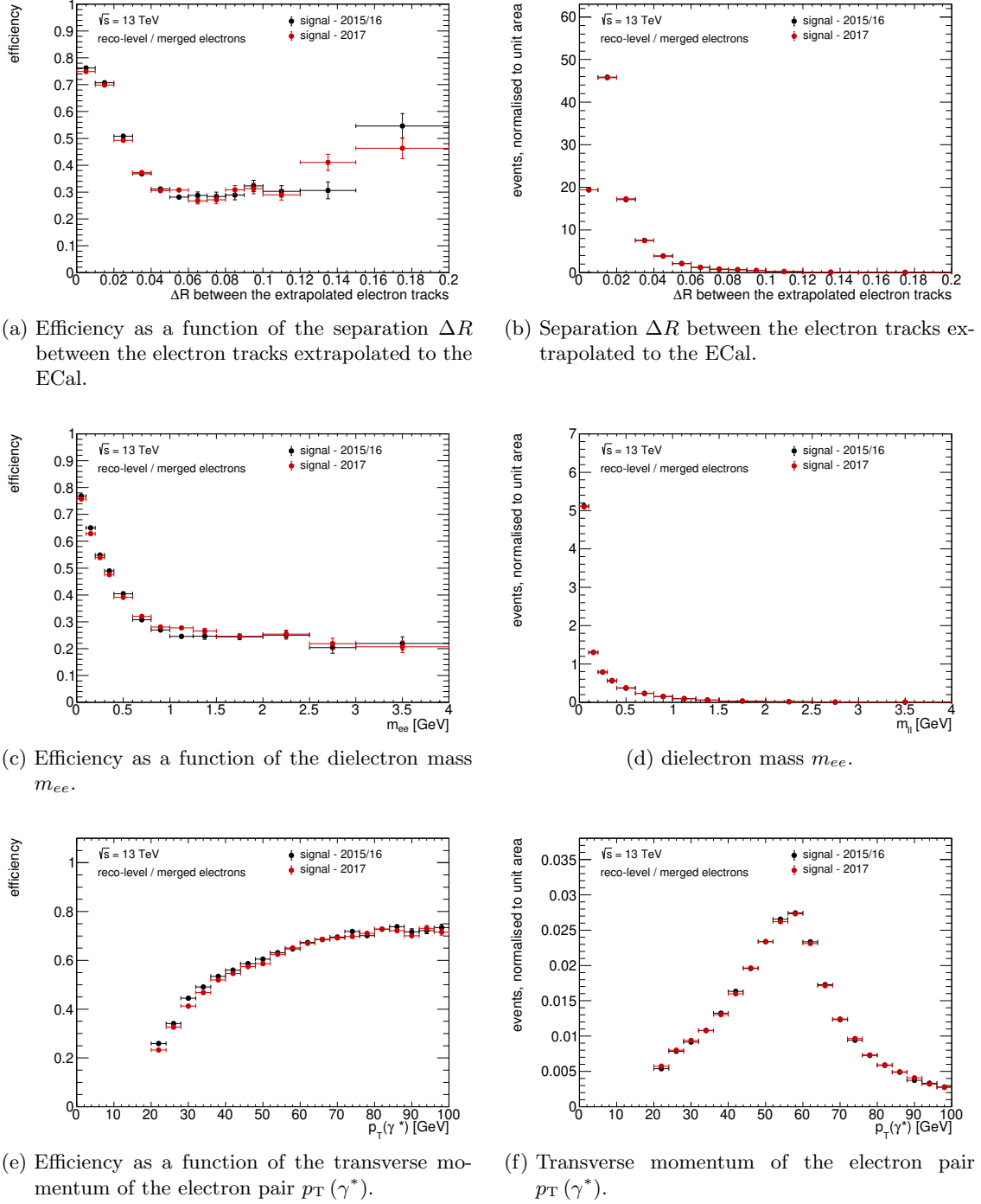
Figure 15.5.: Efficiency of the merged electron identification as a function of the separation \Delta R between the tracks extrapolated to the ECal, the dielectron mass m_{ee} and the transverse momentum p_T(\gamma^*) (left column) and of the distributions of the corresponding observables (right column) for the ggF signal. The distributions in the right column are normalised to unit area. All observables are at the reconstruction level.
