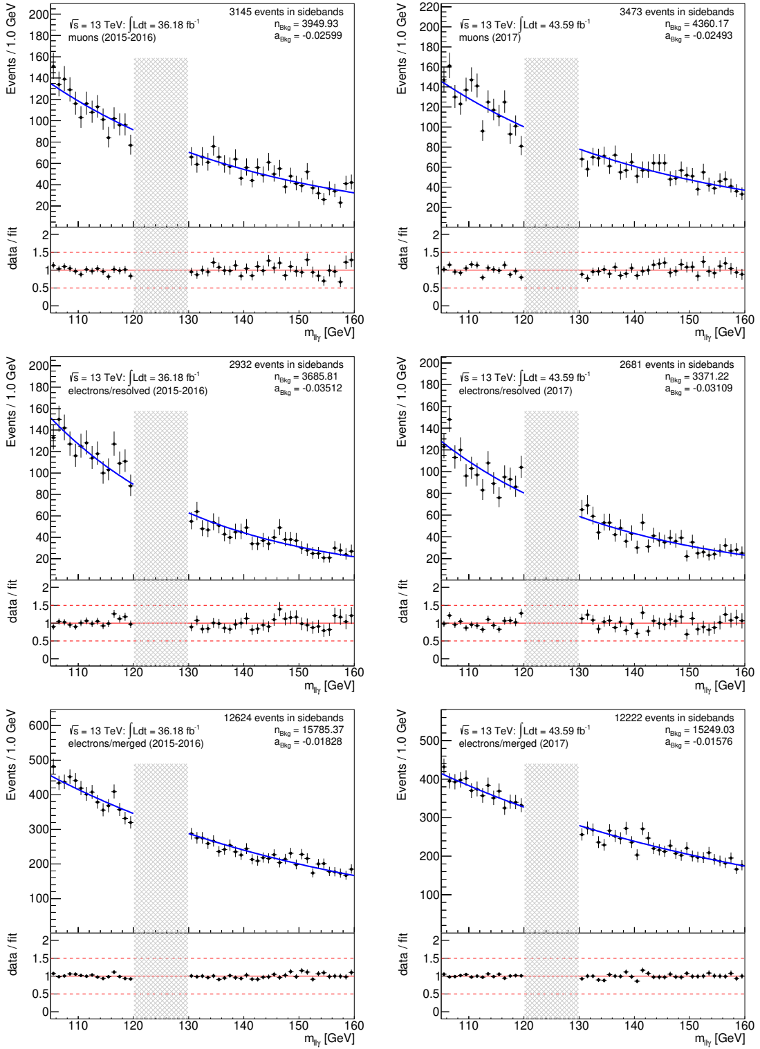
Figure 16.2.: Background parameterisation for the 2015-2016 (left column) and 2017 (right column) run period for the muon, resolved and merged electron categories. The chosen background model is a falling exponential function fitted separately in each category. The model is fitted to data events using an extended unbinned likelihood fit. Events with three-body invariant masses m_{\ell\ell\gamma} between 120 and 130 GeV are excluded. The events are only binned for display purposes and are shown as black data points, with the error bars indicating the statistical uncertainty. The obtained background model curves are shown with solid blue lines.
