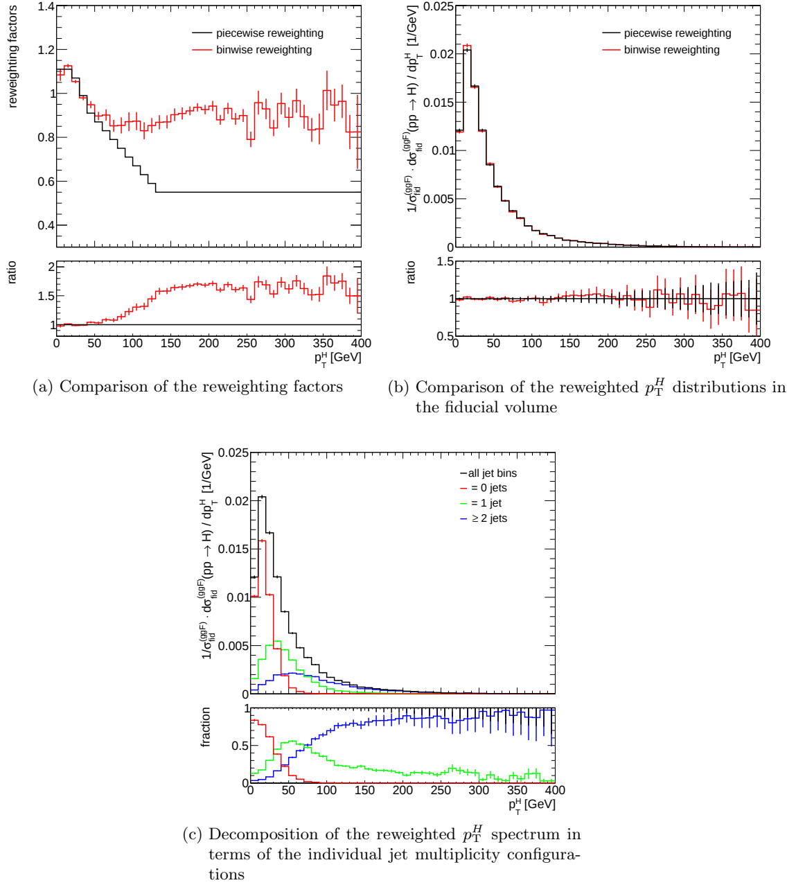
Figure 12.5.: Comparison of the piecewise and binwise Higgs p_T reweighting strategies in the low-mass search. The error bars indicate the statistical uncertainties.
