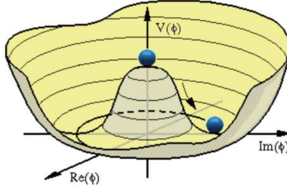
Figure 2.4.: Mexican hat shape of the Higgs potential. Taken from [28].
