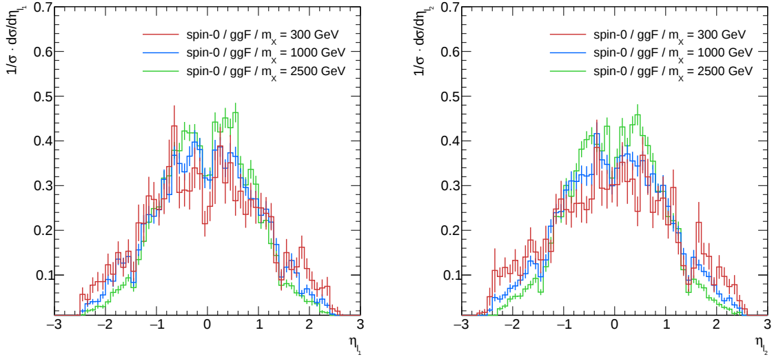
Figure B.5.: Normalised \eta distributions of the leptons for the ggF production of a spin-0 resonance for resonance masses of m_X = 300 GeV, 1 TeV and 2.5 TeV as derived from Monte Carlo simulations after the common preselection stage.
