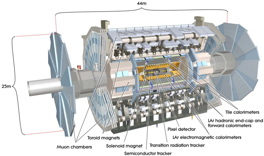
Figure 4.1.: Cut-away overview of the ATLAS detector. Picture taken from [107].
