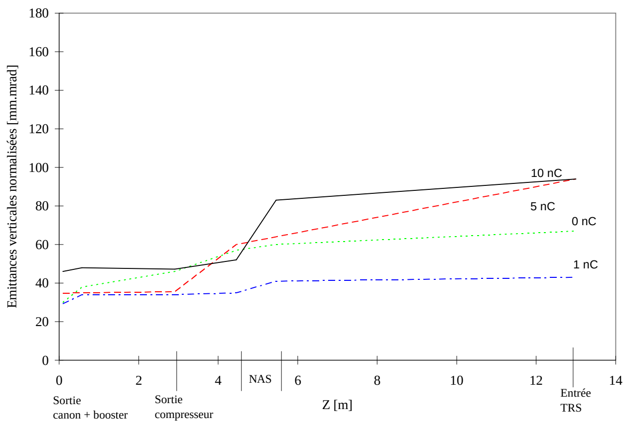
(b) Emittances verticales
