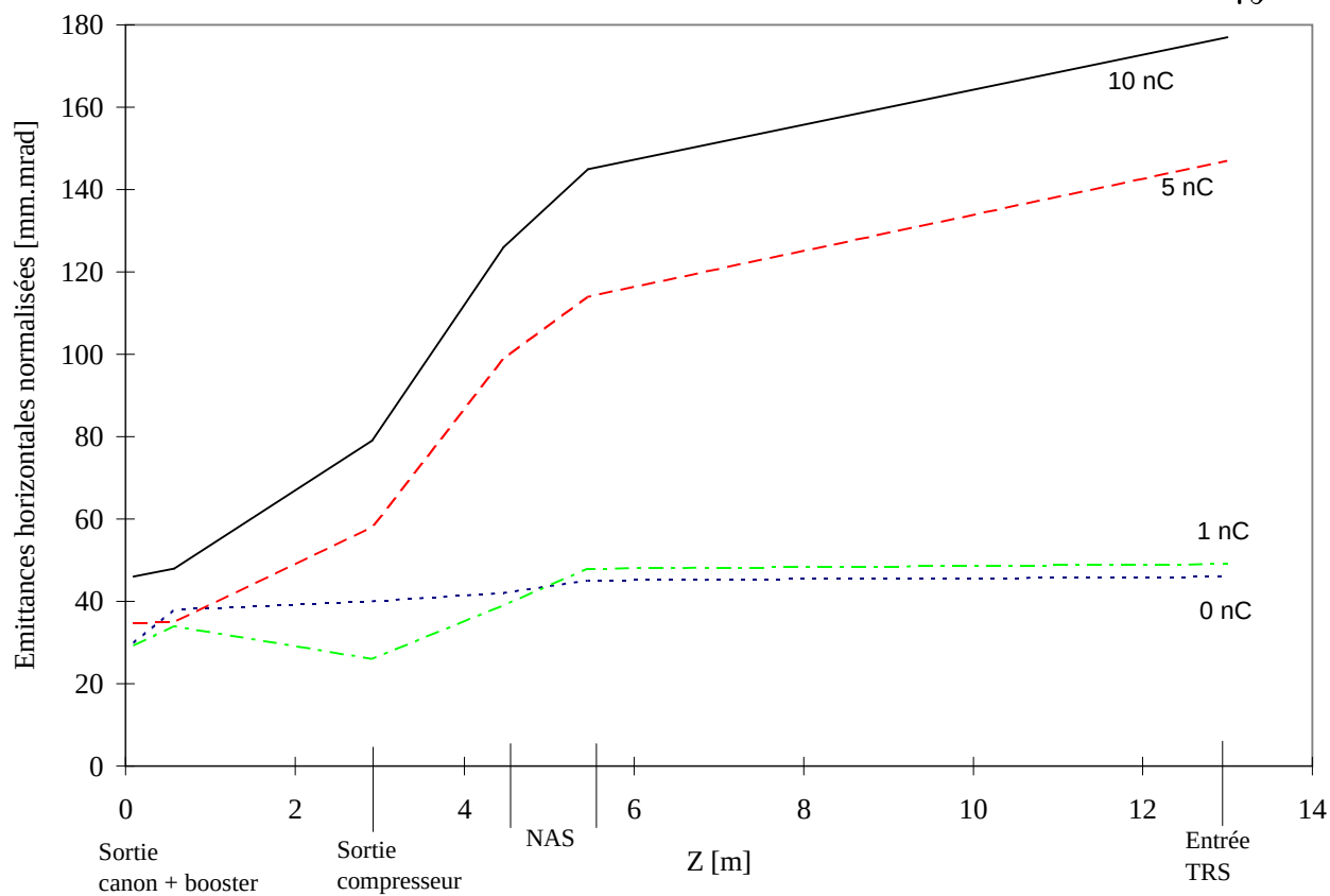
(a) Emittances horizontales
