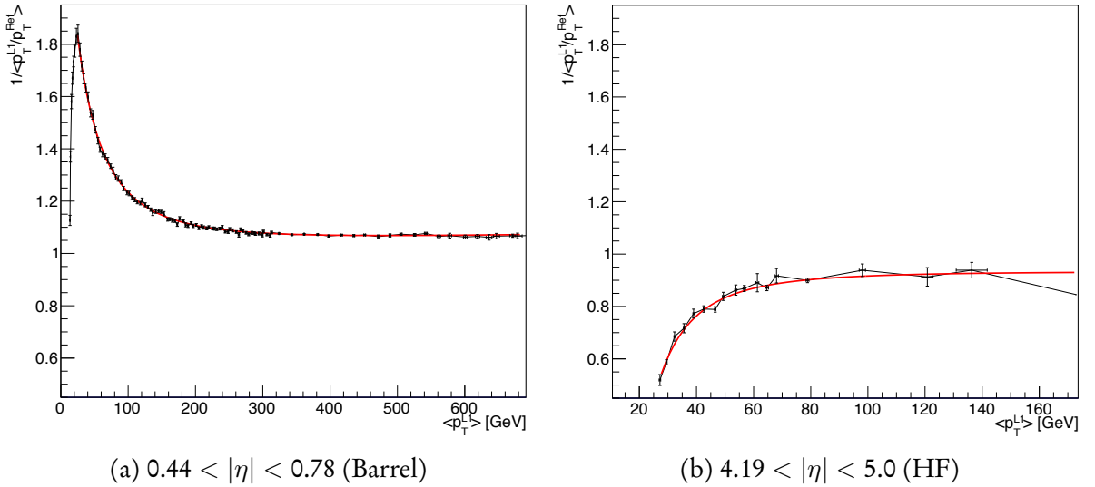
Figure 3.8: Examples of correction curves used to calibrate the jet energies in two |\eta| bins. The reciprocal of the response is plotted against the p_T of the Level-1 jet, and a complex function (Eq. 3.9) fits the points. These plots are from the jet energy corrections performed on 2018 QCD Monte Carlo.
