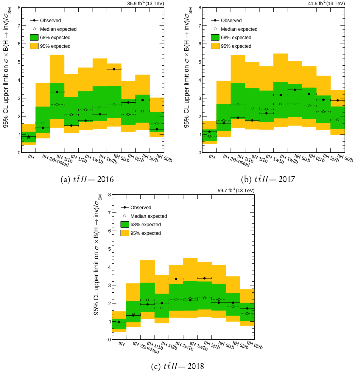
Figure A.11: Observed and expected 95 % CL upper limits on the Higgs boson to invisible state branching fraction in the t\bar{t}H channel, for both the individual categories, and the combination of them, for each data-taking year in Run-2.
