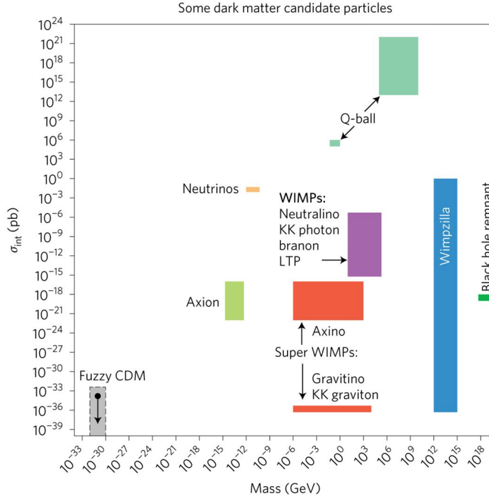
Figure 2.4: The expected masses and interaction cross sections of a set of dark matter candidates. The LHC, with its centre of mass energy of 13 TeV, is best suited to targeting Weakly Interacting Massive Particles (WIMPs). Figure acquired from Ref. 71.
