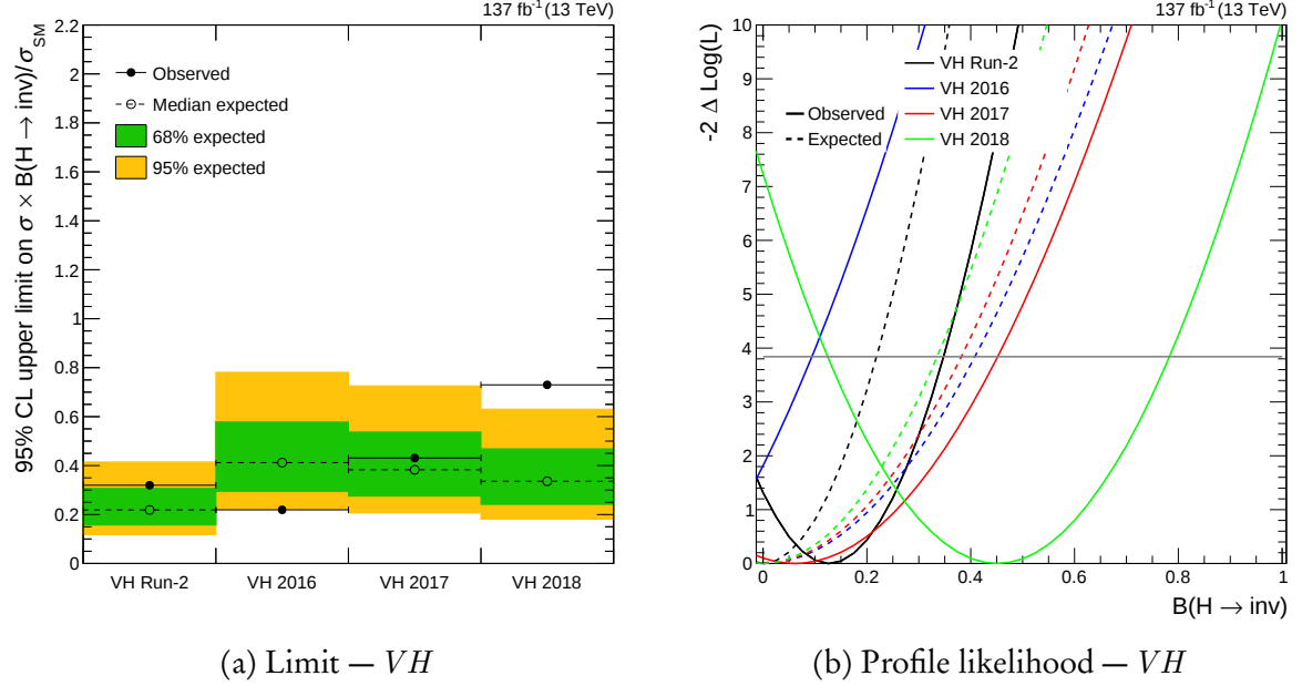
Figure 6.23: Observed and expected 95 % CL upper limit on the Higgs boson to invisible state branching fraction \mathcal{B}(H \rightarrow \text{invisible}) (left) and the corresponding profile likelihood scan (right) in the VH channel. The result from each data taking period is presented along with their combination.
