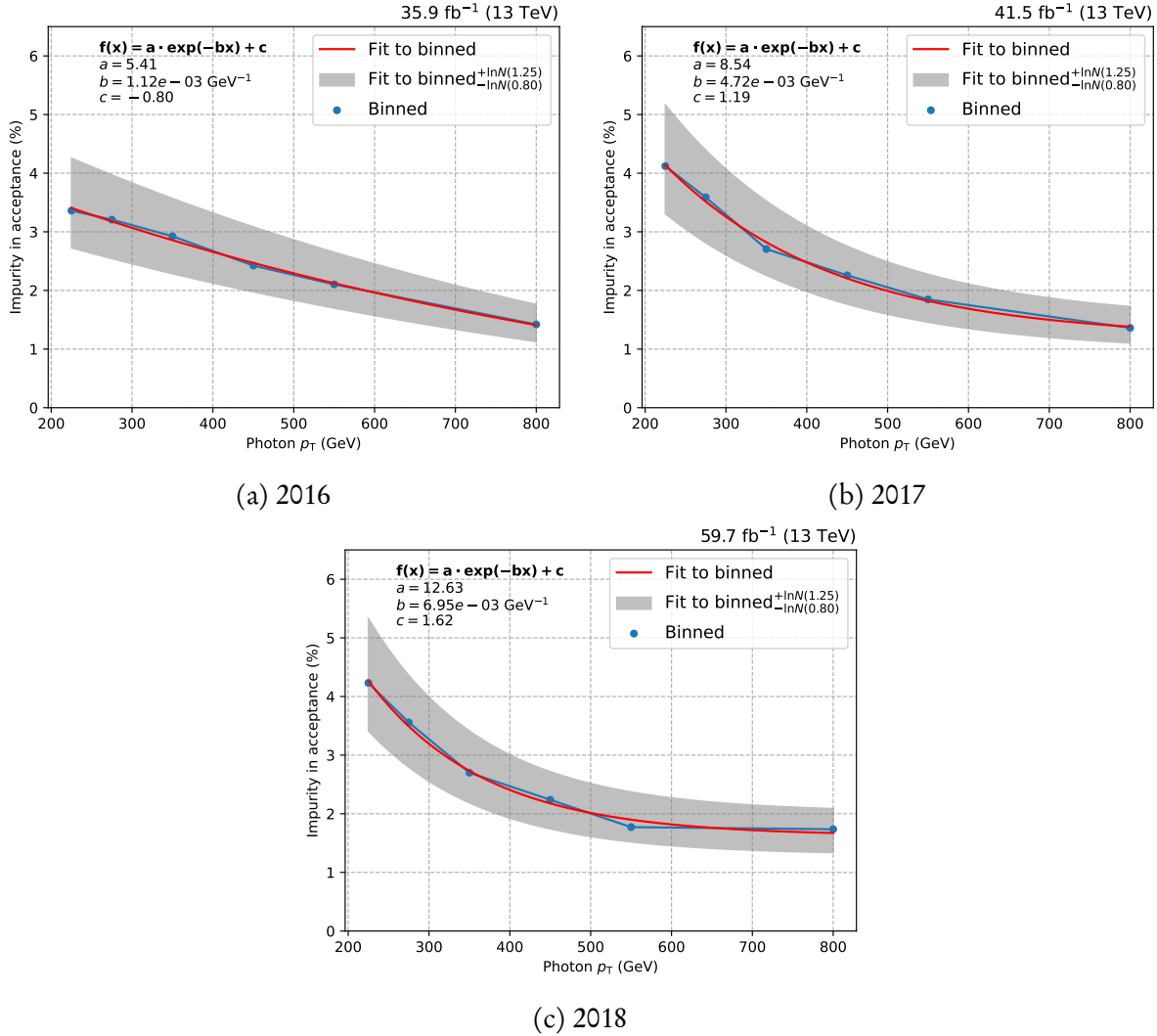
Figure 6.11: The fraction of impure photons in data as a function of p_T for each data taking year in Run-2. An exponential is fit to the binned data with a 25 % uncertainty assigned to account for binning effects.
