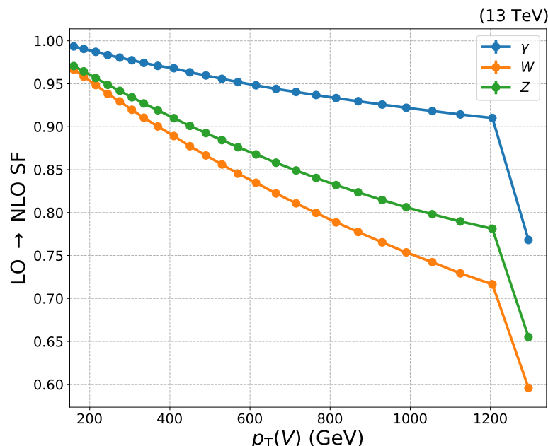
Figure 6.17: NLO k -factors as a function of generator-level boson p_T for reweighting QCD V + \text{jets} events generated at NLO electroweak accuracy. Separate k -factors correct the W , Z , and \gamma + \text{jets} processes. Values obtained from Ref. 112.
