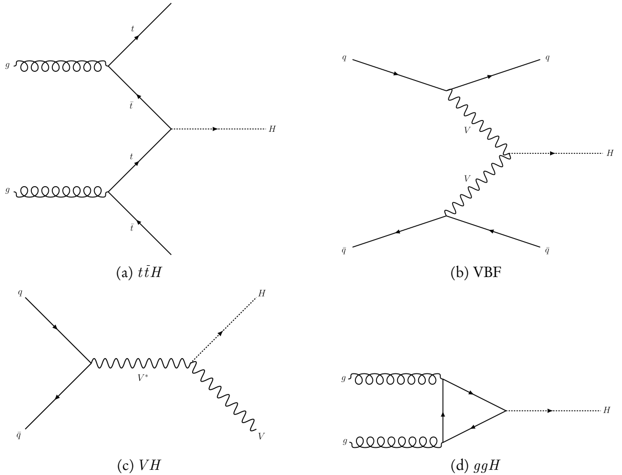
Figure 2.5: A subset of the Feynman diagrams for the four predominant production mechanisms of the Higgs boson at the LHC.
