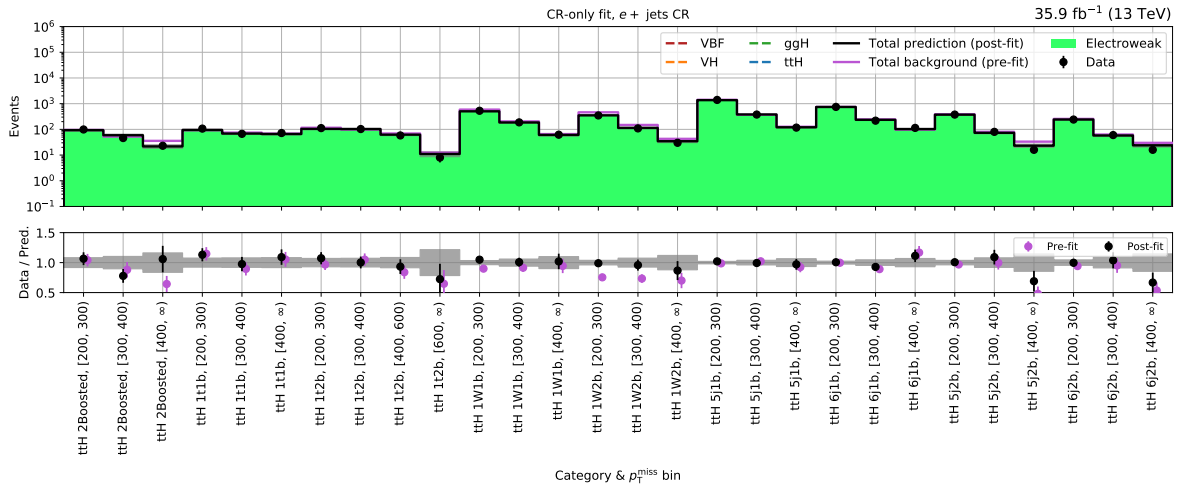
(b) t\bar{t}H - e + \text{jets} control region (2016)
