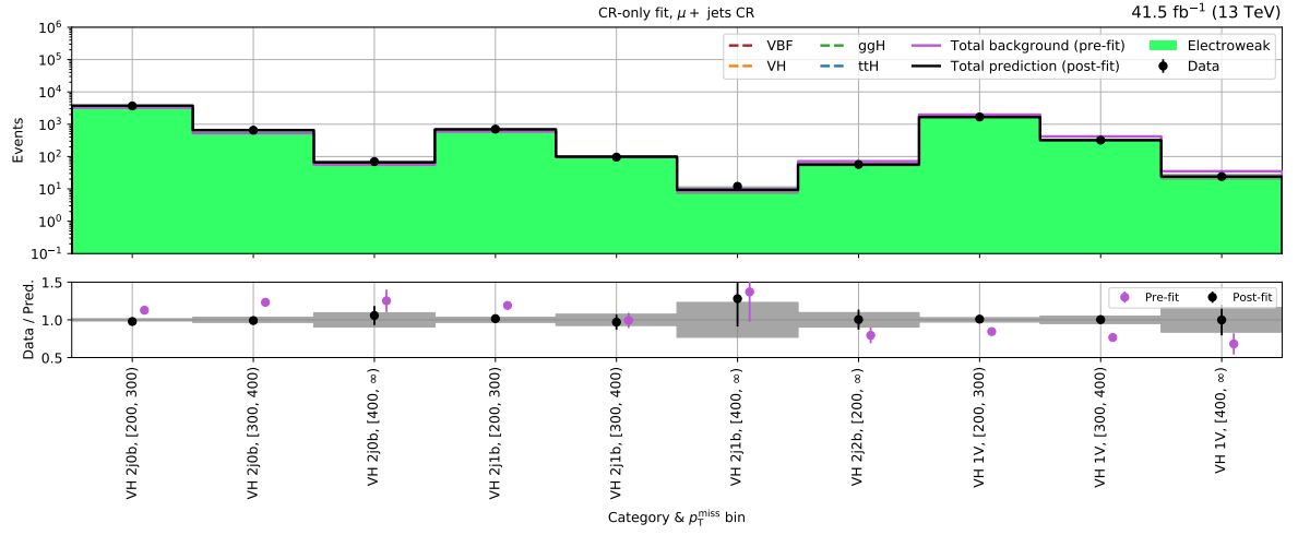
(a) VH - \mu + \text{jets} control region (2017)
