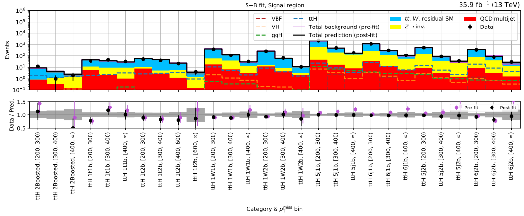
(a) t\bar{t}H — 2016
