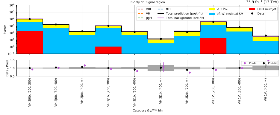
(a) VH — 2016
