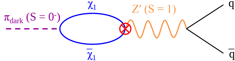
Figure 5.1: A diagram of the mass insertion decay of \pi_{\text{dark}} mesons in the s -channel semi-visible jet model.
