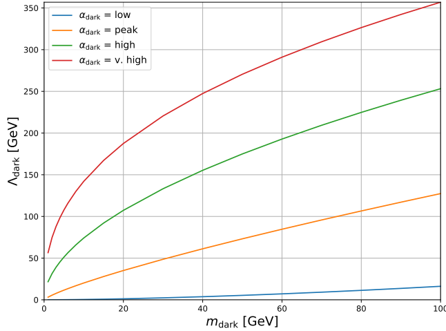
Figure 5.2: The dependence of the dark force scale \Lambda_{\text{dark}} on the dark hadron mass m_{\text{dark}} for each value of \alpha_{\text{dark}} used in the thesis.
