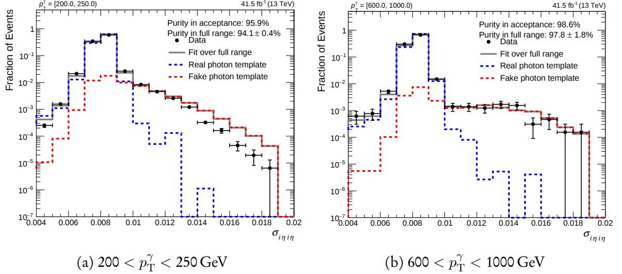
Figure 6.10: Fits of real and fake photon templates to data in the \sigma_{i\eta i\eta} spectrum. Two bins of p_T^\gamma are illustrated, demonstrating the different shapes of the templates and data, with the purity over the full range and within acceptance ( \sigma_{i\eta i\eta} \leq 0.01 ) noted.
