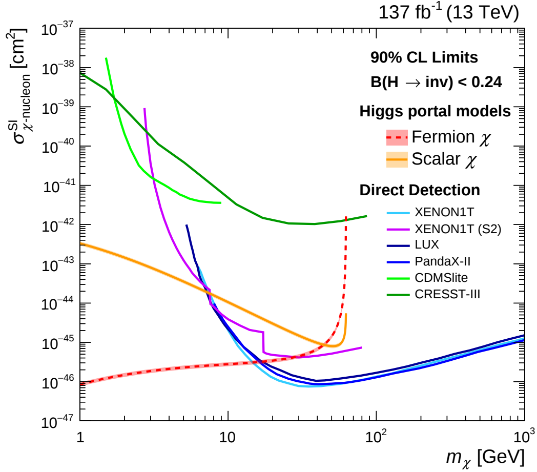
Figure 6.25: 90 % confidence level upper limits on the spin-independent dark matter–nucleon scattering cross section in Higgs portal models, where the standard model Higgs boson decays into a pair of scalar (solid orange) or fermion (dashed red) dark matter particles. Comparisons to direct detection experiments are also provided: XENON1T [18] (additionally with the S2-only analysis [19]), LUX [12], PandaX-II [73], CDMSlite [9], and CRESST-III [6].
