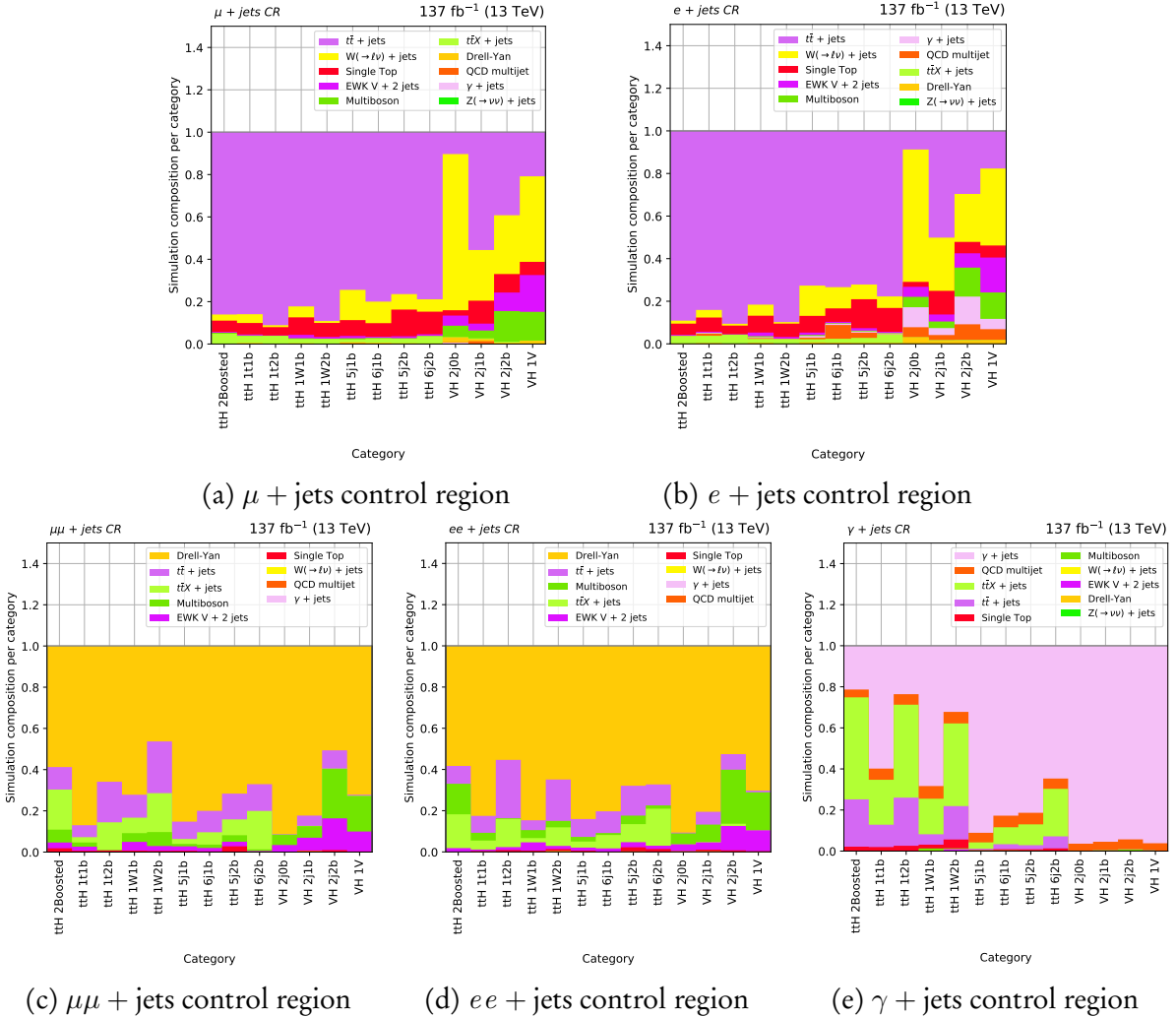
Figure 6.7: Composition of each category in each of the control regions for simulated background processes after the analysis-level selection.
