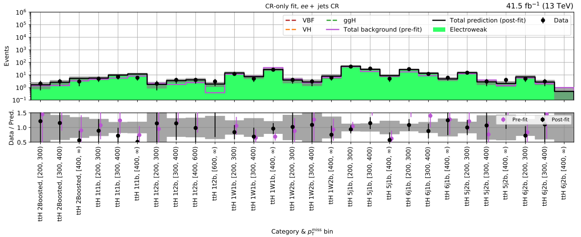
(b) t\bar{t}H - ee + \text{jets} control region (2017)
