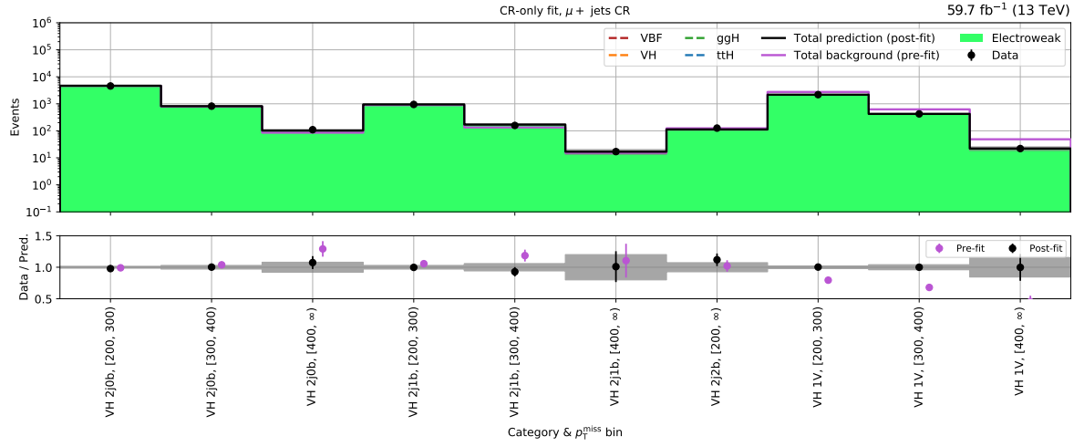
(a) VH - \mu + \text{jets} control region (2018)
