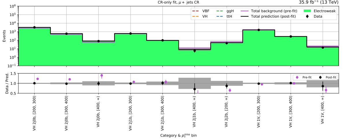
(a) VH - \mu + \text{jets} control region (2016)
