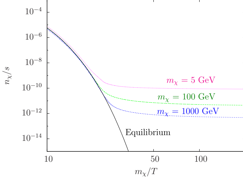
Figure 2.2: A measure of the comoving number density of WIMP dark matter as a function of time, with projections for several particle masses. The black curve represents the scenario in which dark matter remains in equilibrium with the standard model. Figure taken from Ref. 90.
