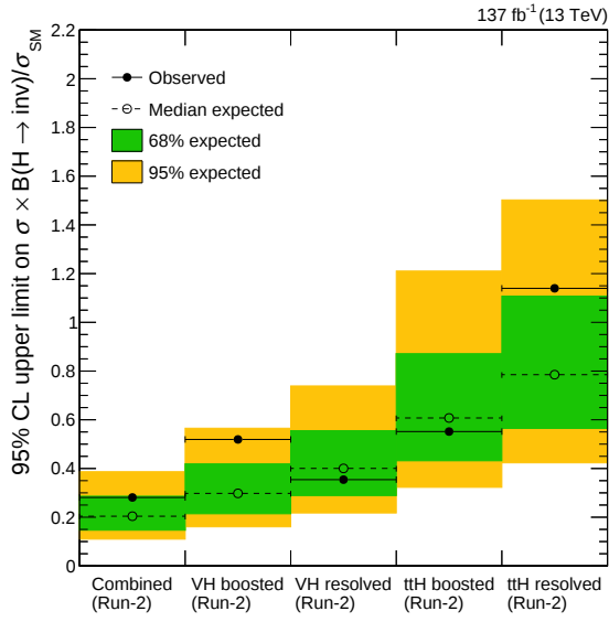
(a) Limit — Run-2
