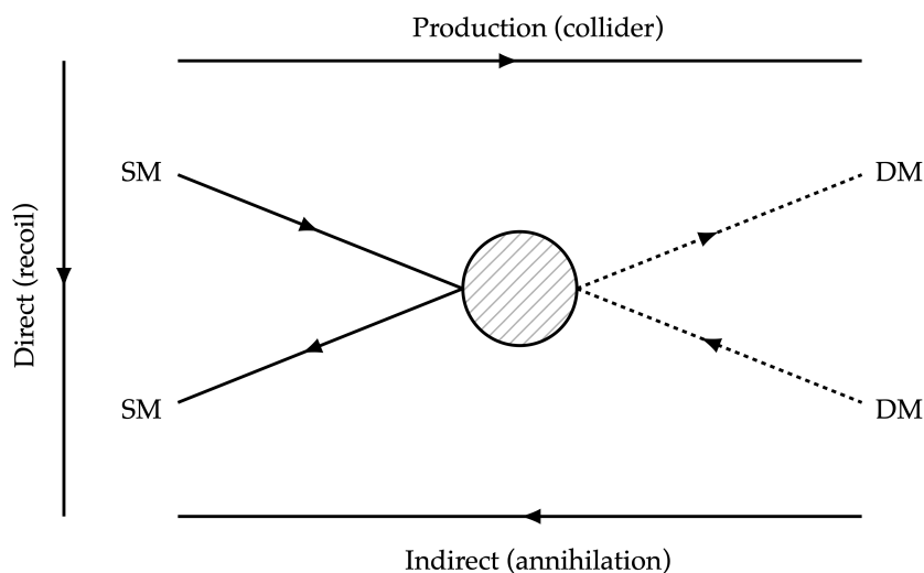
Figure 2.3: A visual representation of the three main types of dark matter detection: direct (dark matter recoiling from standard model particles); indirect (annihilation of dark matter); and production (dark matter created in high energy particle collisions).
