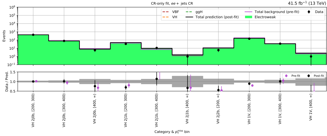
(b) VH - ee + \text{jets} control region (2017)
