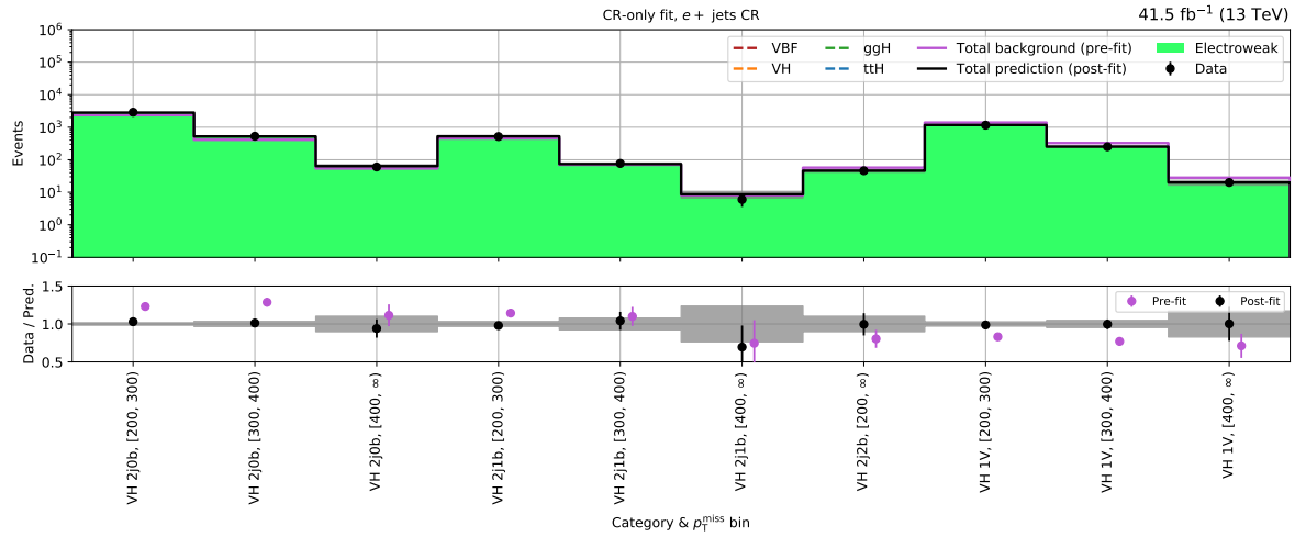
(b) VH - e + \text{jets} control region (2017)
