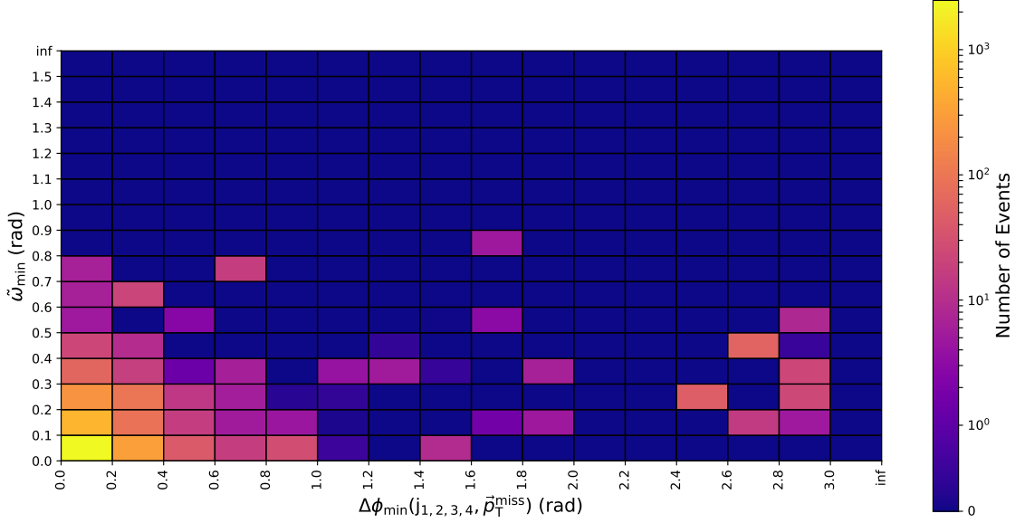
Figure 6.2: The distribution of QCD multijet events in the signal region as a function of \tilde{\omega}_{\min} and \Delta\phi_{\min} . The full event selection, except the cuts pertaining to the variables of interest, is applied.
