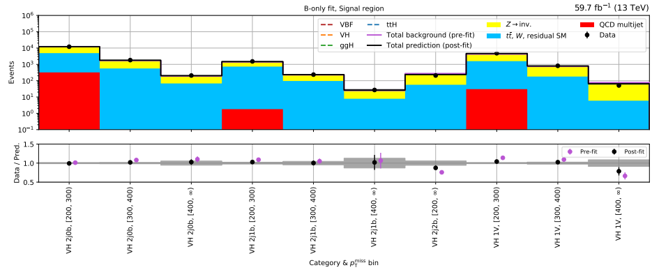
(c) VH — 2018
