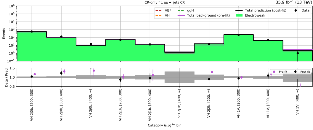
(a) VH - \mu\mu + \text{jets} control region (2016)
