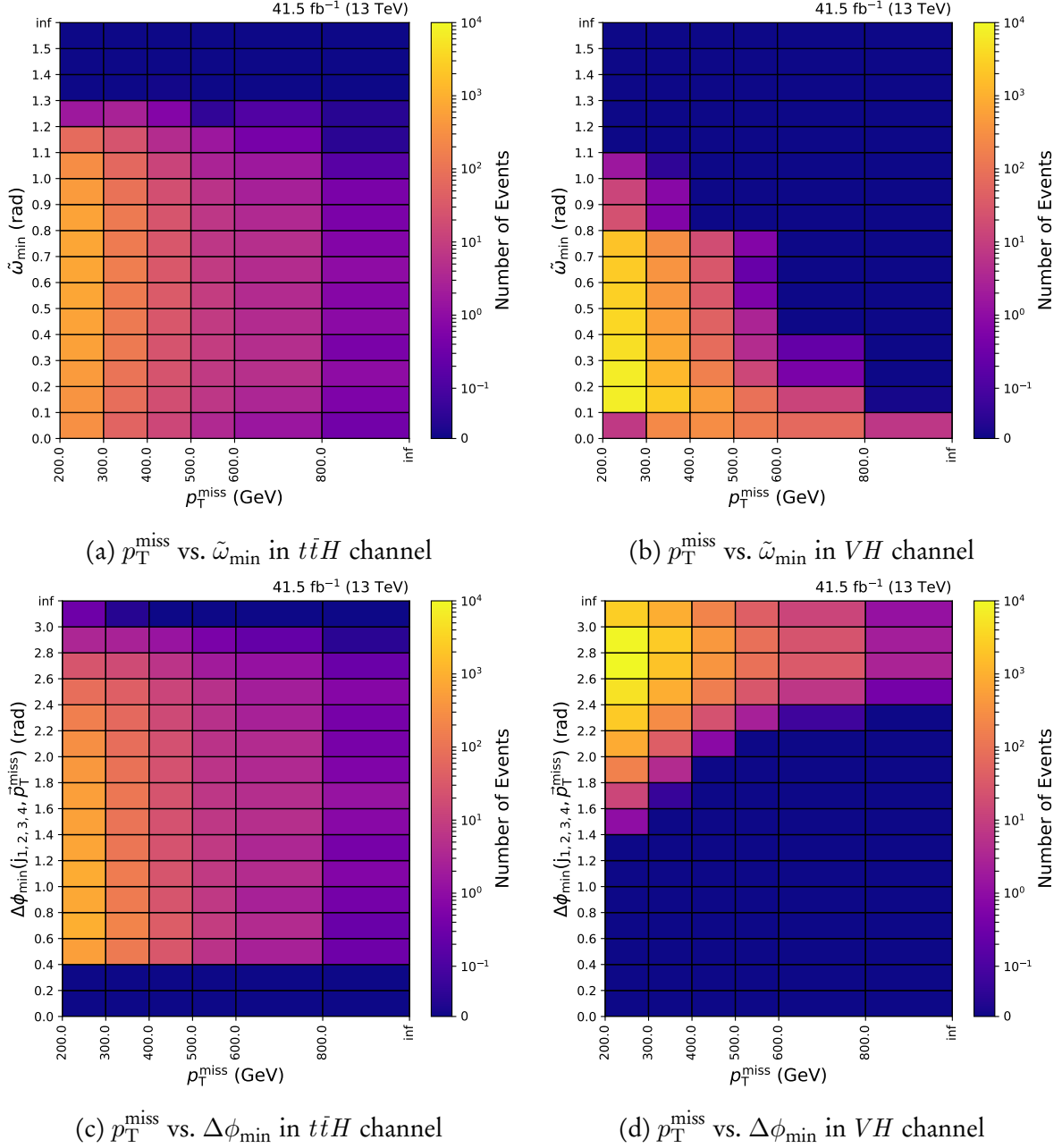
Figure 6.4: Histograms of the background event counts in the t\bar{t}H and VH channels of the signal region for the search variable p_T^{\text{miss}} against the optimisation variables \tilde{\omega}_{\text{min}} and \Delta\phi_{\text{min}} .
