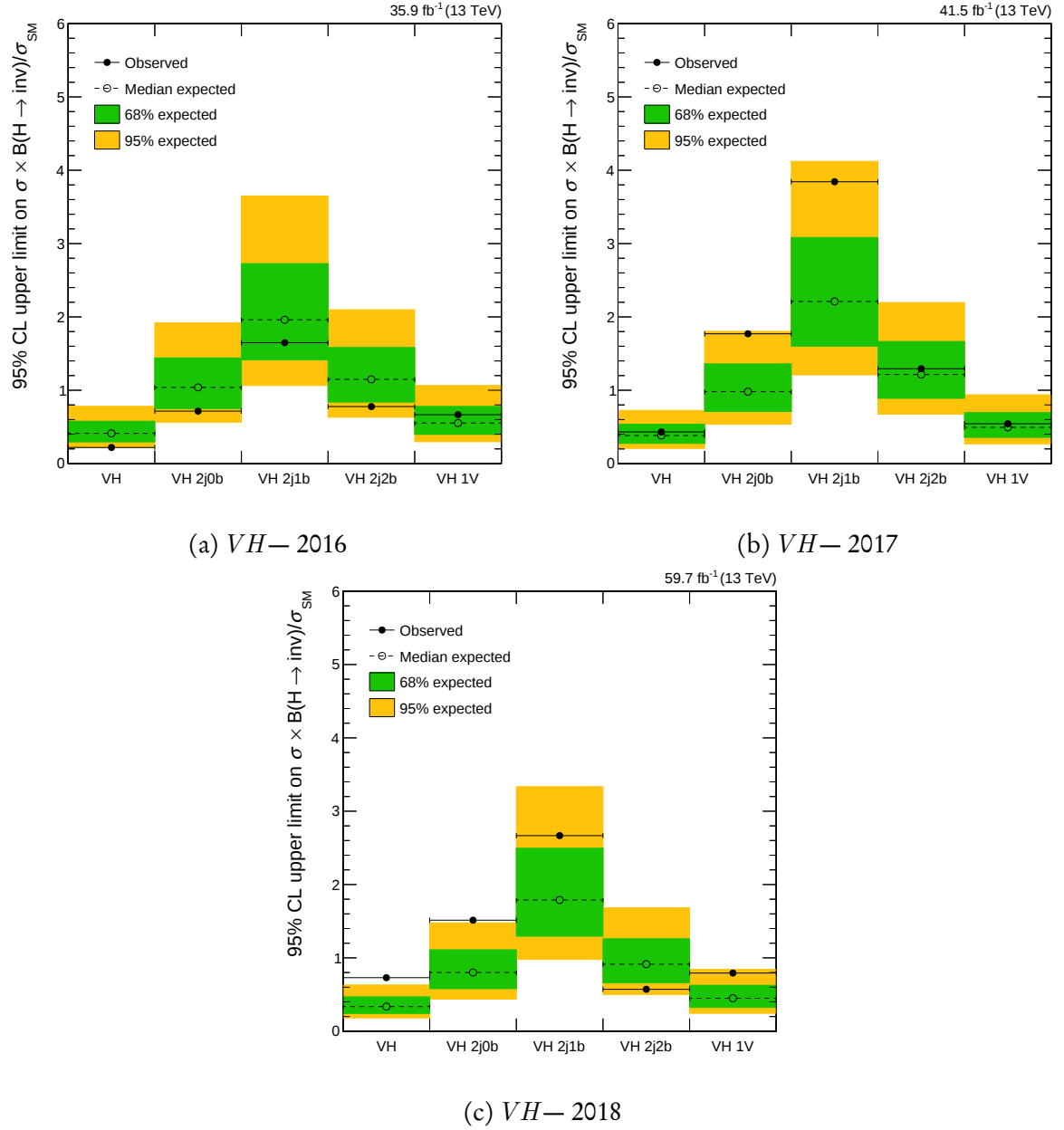
Figure A.12: Observed and expected 95 % CL upper limits on the Higgs boson to invisible state branching fraction in the VH channel, for both the individual categories, and the combination of them, for each data-taking year in Run-2.
