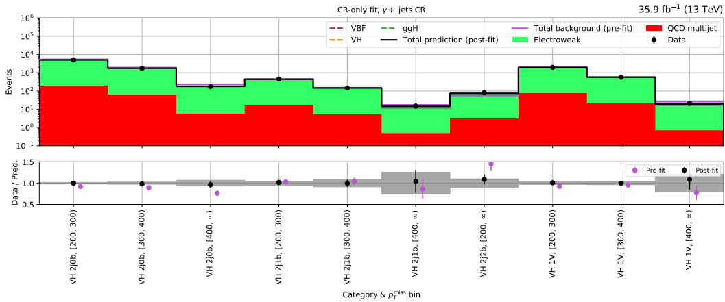
(c) VH - \gamma + \text{jets} control region (2016)
