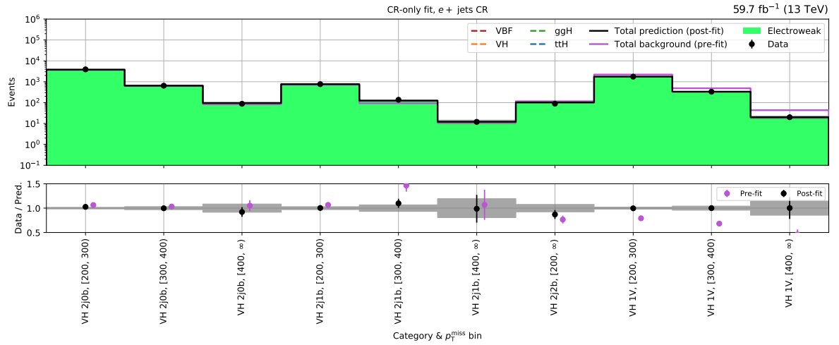
(b) VH - e + \text{jets} control region (2018)
