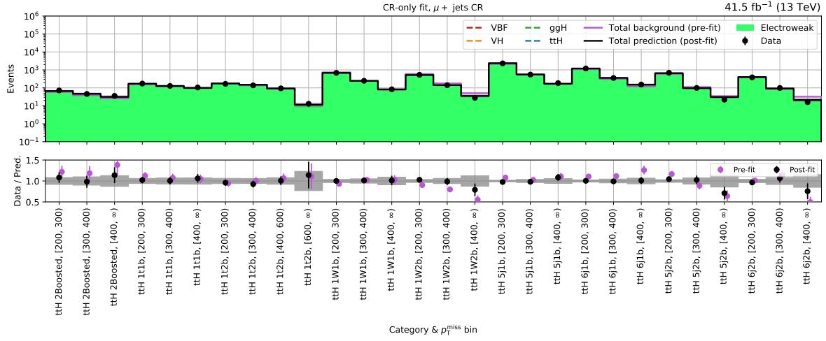
(a) t\bar{t}H - \mu + \text{jets} control region (2017)
