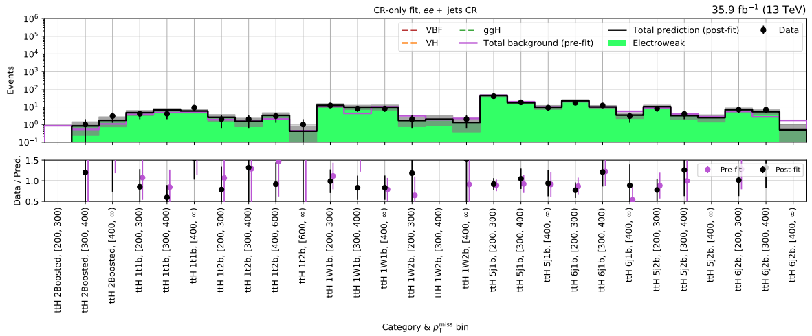
(b) t\bar{t}H - ee + \text{jets} control region (2016)
