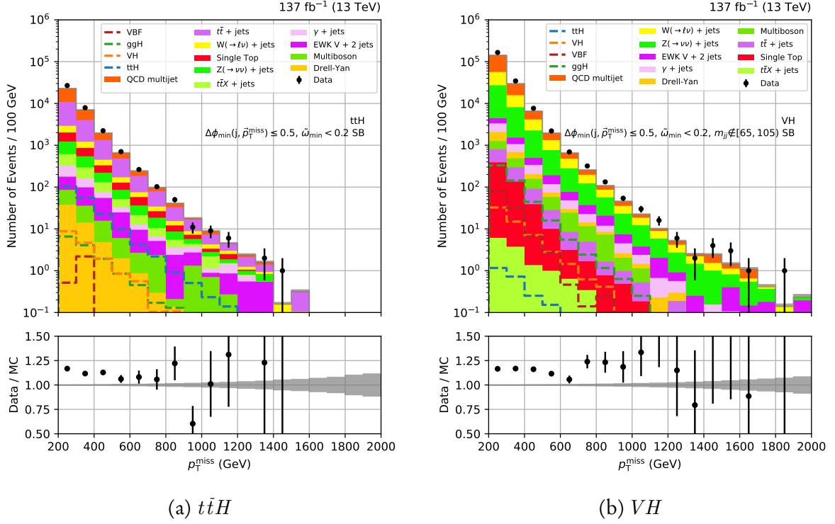
Figure 6.14: Data-simulation comparisons of the p_T^{\text{miss}} distribution in the t\bar{t}H and VH sidebands, aggregated over the full Run-2 dataset.
