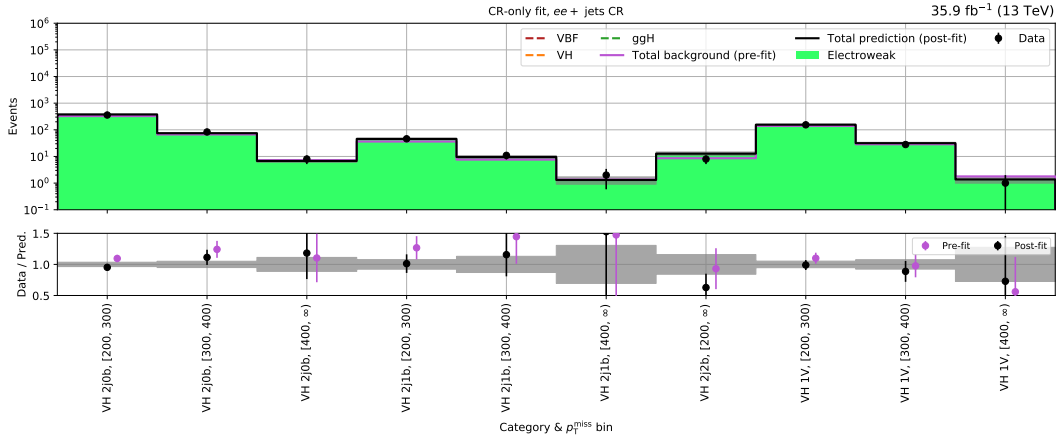
(b) VH - ee + \text{jets} control region (2016)
