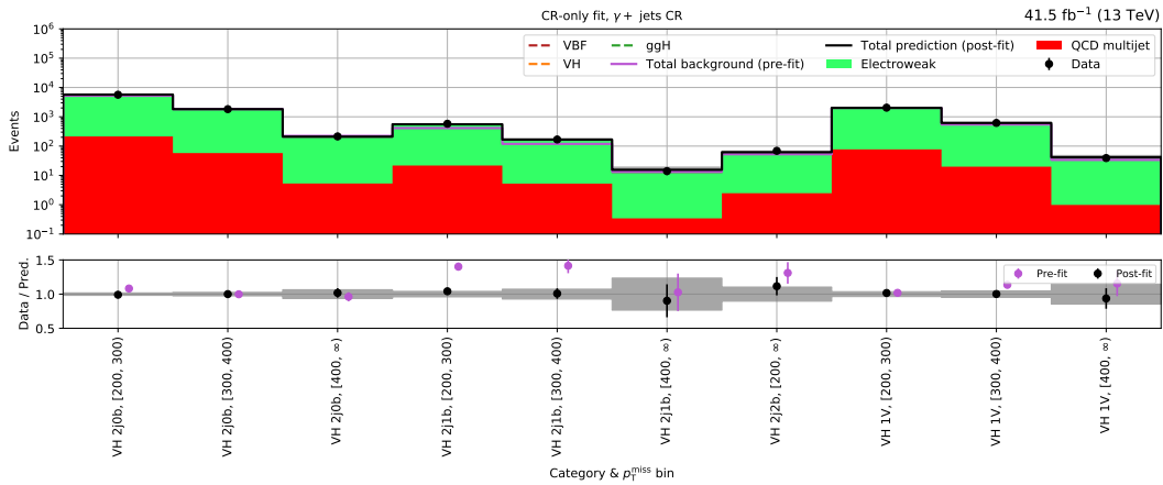
(c) VH - \gamma + \text{jets} control region (2017)
