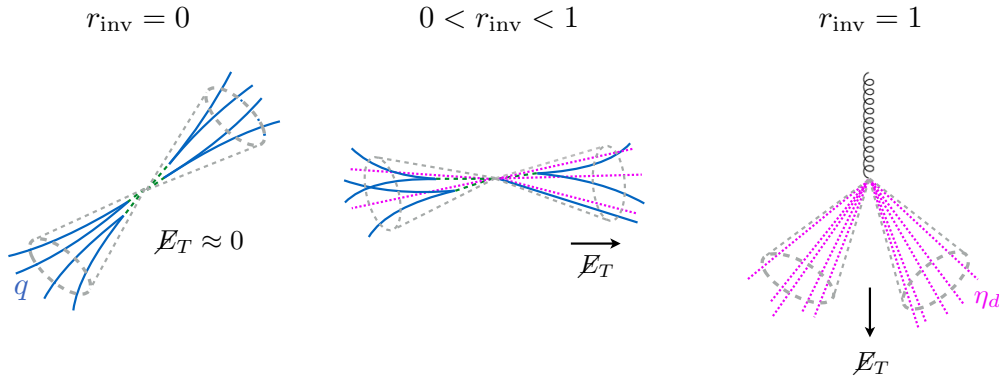
Figure 2.8: The typical direction of the missing transverse energy E_T (or \vec{p}_T^{\text{miss}} ) relative to the semi-visible jets as a function of their invisible fraction r_{\text{inv}} . The green dashed lines signify visibly decaying dark hadrons, blue the SM quarks, and pink the stable dark hadrons. Figure from Ref. 70.
