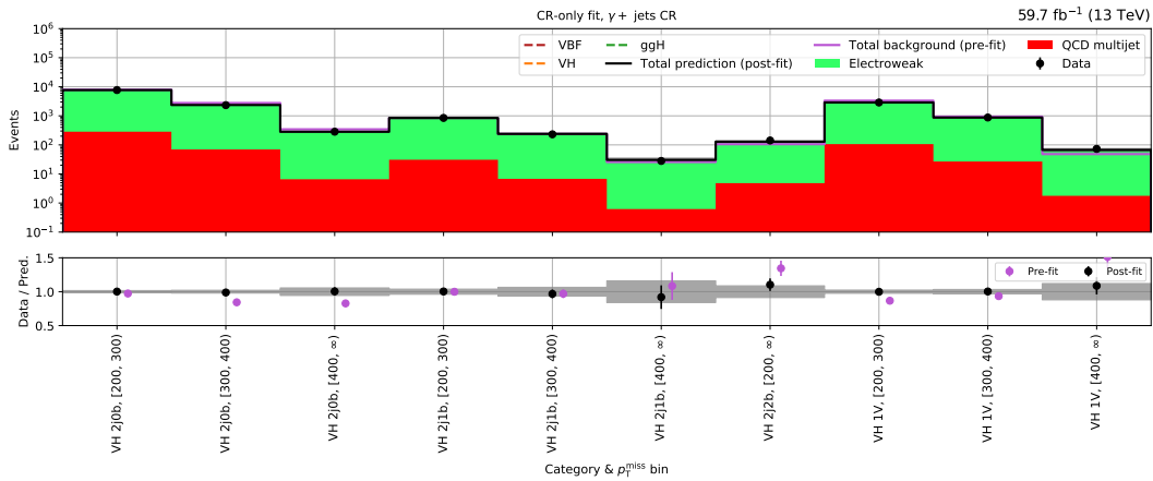
(c) VH - \gamma + \text{jets} control region (2018)
