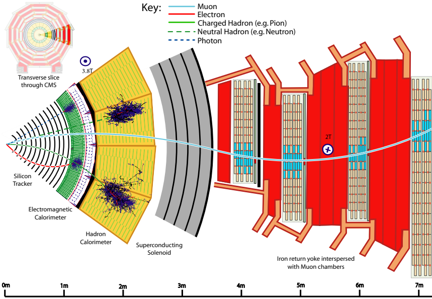
Figure 3.6: A transverse slice through the barrel section of the CMS detector with the main subsystems and components visible. Several particles produced at the primary vertex and their interactions with the detector are also depicted. Figure obtained from Ref. 129.
