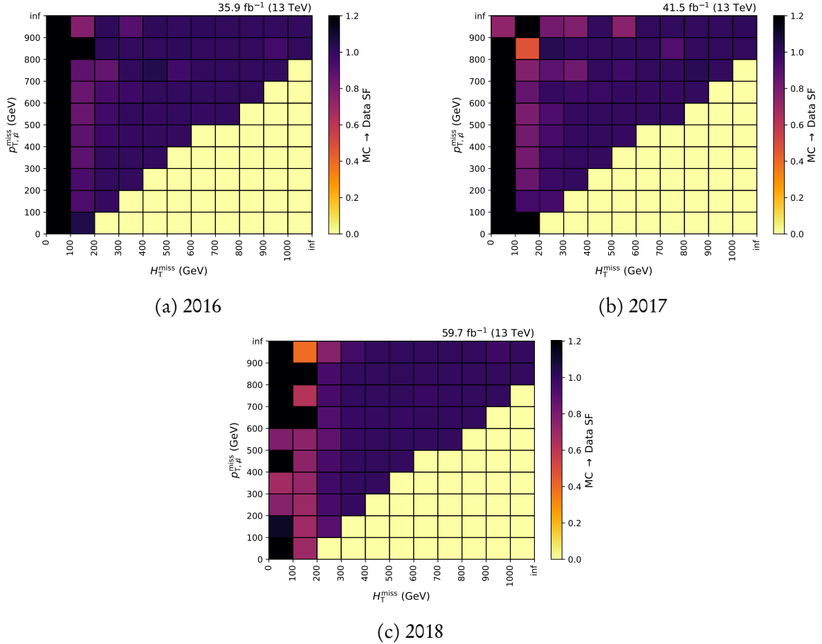
Figure 6.15: Scale factors accounting for the efficiencies of the HLT p_T^{\text{miss}}-H_T^{\text{miss}} cross triggers in each data taking year of Run-2. The momentum of the muon used to select events that compute the efficiency is added to the \vec{p}_T^{\text{miss}} (with a magnitude p_{T,\mu}^{\text{miss}} ) in order to approximate the calculation in the High-Level Trigger.
