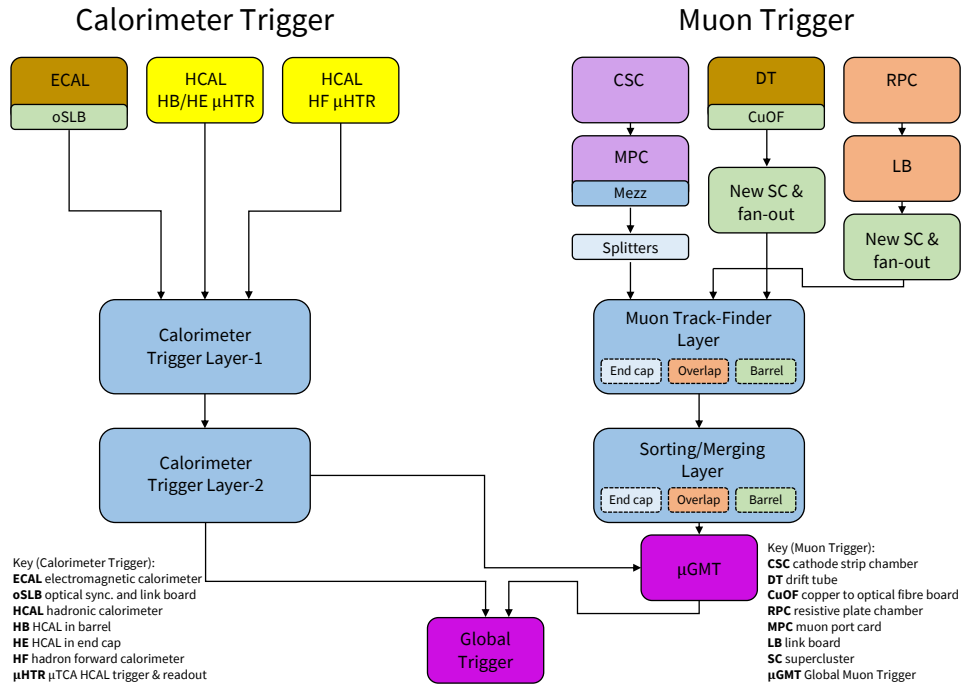
Figure 3.7: A summary of the CMS Level-1 Trigger data flow from the hits recorded by the subsystems to the Global Trigger. Figure reproduced from Ref. 75.
