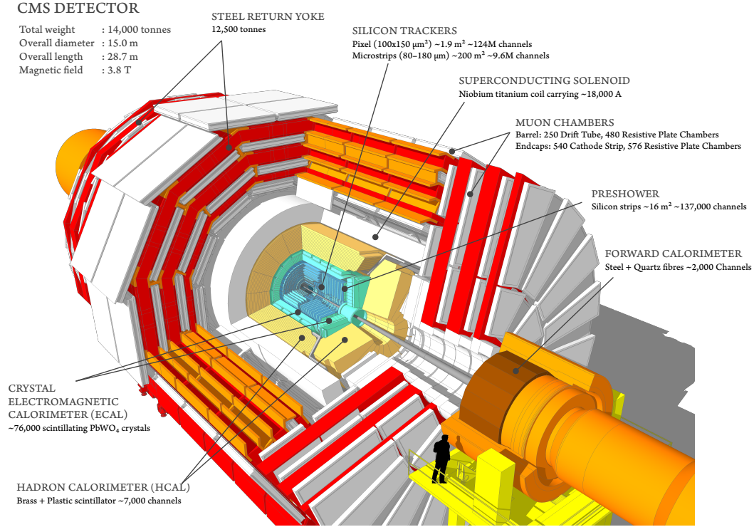
Figure 3.4: A cutaway diagram of the CMS detector with all of the principal components labelled. This detector configuration was used for the 2017–18 data taking years, where the coverage of the pixel detectors in the silicon tracker were upgraded. Image taken from Ref. 122.
