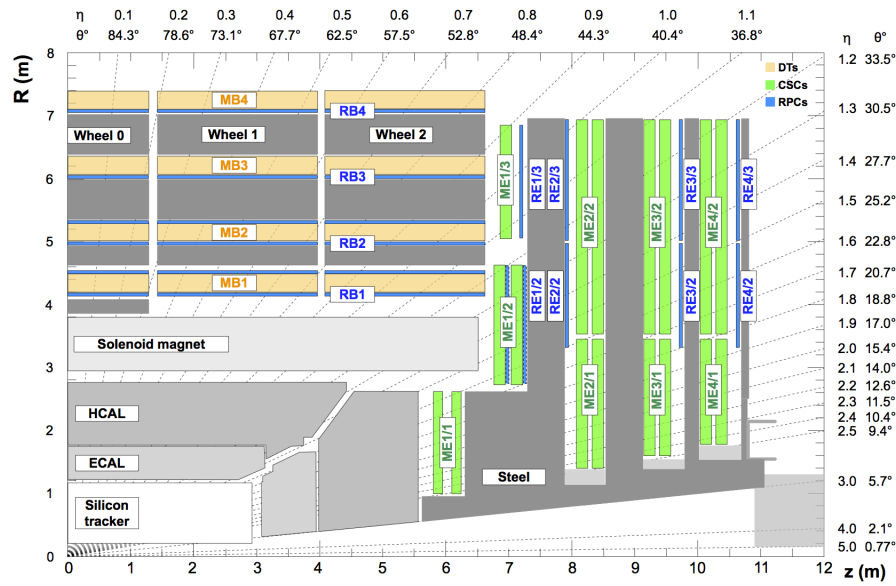
Figure 3.5: A quadrant of the CMS detector illustrating the main subsystems with their radius R , longitudinal distance z , and pseudorapidity \eta from the interaction point. The grey box at 3 < |\eta| < 5 and 11 < z < 12 m is the hadron forward calorimeter. Figure taken from Ref. 115.
