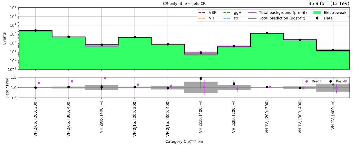
(b) VH - e + \text{jets} control region (2016)
