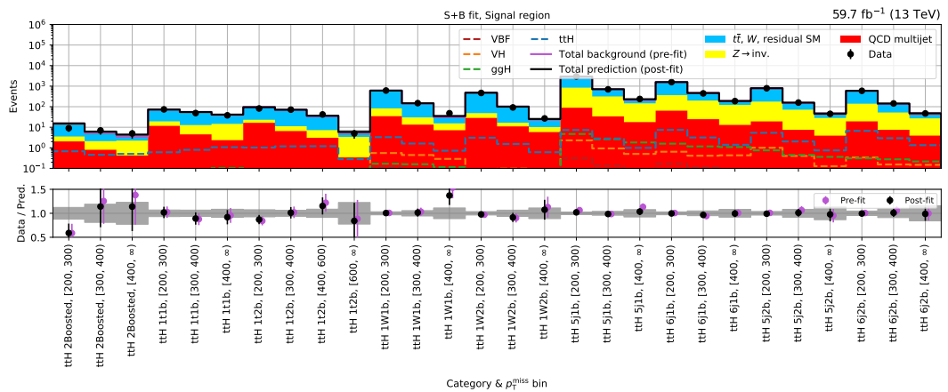
(c) t\bar{t}H — 2018
