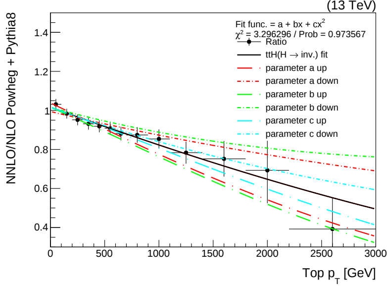
Figure 6.19: The ratio of the NNLO to NLO t\bar{t} cross section as a function of top quark p_T . The fit to the distribution—along with the uncertainties in the parameters—is shown.
