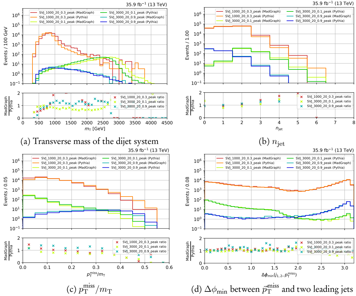
Figure 5.5: Distributions of several observables for the models SVJ_1000_20_0.3_peak, SVJ_3000_20_0.1_peak, and SVJ_3000_20_0.9_peak. Generation in MADGRAPH5_amc@NLO is compared to PYTHIA8, with the ratios between them for each model displayed in the respective subplot.
