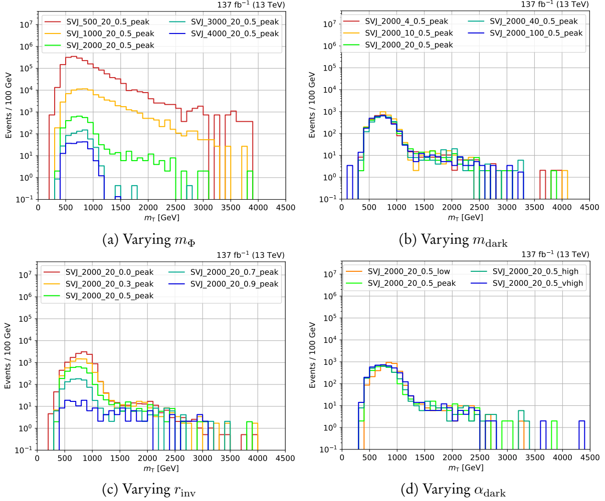
Figure 5.4: Distributions of the transverse mass of the dijet system m_T for t -channel semi-visible jet samples emulating the 2016 data taking period. In each panel, one of the free parameters of the model is varied with respect to the benchmark point SVJ_2000_20_0.5_peak (bright green line).
