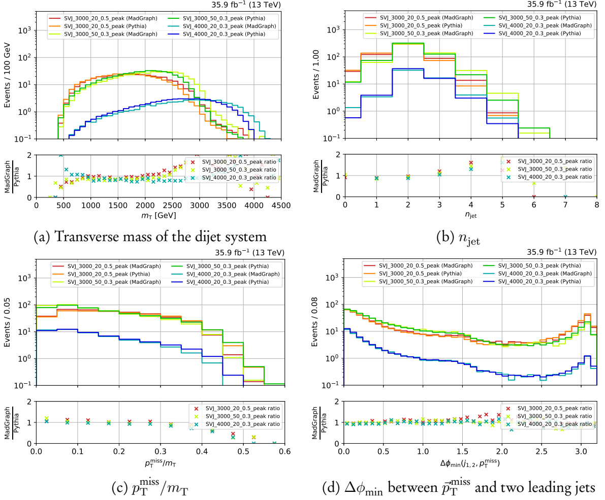
Figure 5.6: Distributions of several observables for the models SVJ_3000_20_0.5_peak, SVJ_3000_50_0.3_peak, and SVJ_4000_20_0.3_peak. Generation in MADGRAPH5- amc@NLO is compared to PYTHIA8, with the ratios between them for each model displayed in the respective subplot.
