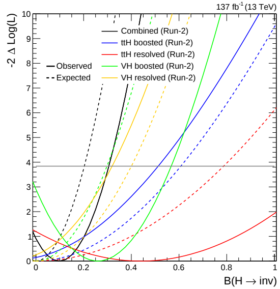
(b) Profile likelihood — Run-2
