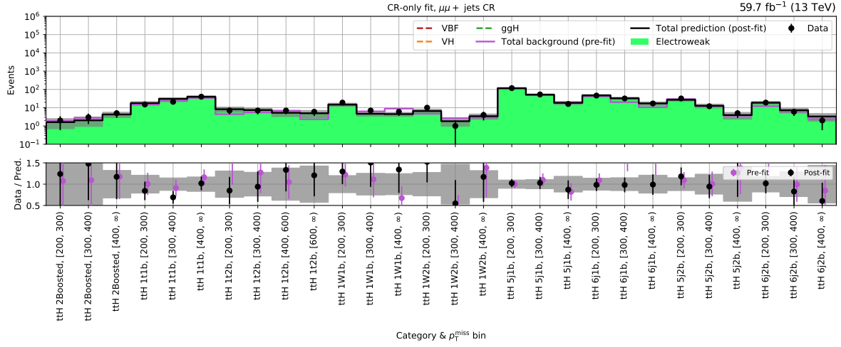
(a) t\bar{t}H - \mu\mu + \text{jets} control region (2018)
