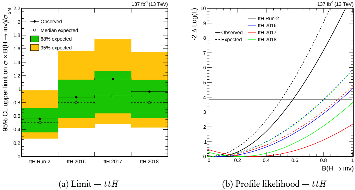
Figure 6.21: Observed and expected 95 % CL upper limit on the Higgs boson to invisible state branching fraction \mathcal{B}(H \rightarrow \text{invisible}) (left) and the corresponding profile likelihood scan (right) in the t\bar{t}H channel. The result from each data taking period is presented along with their combination.
