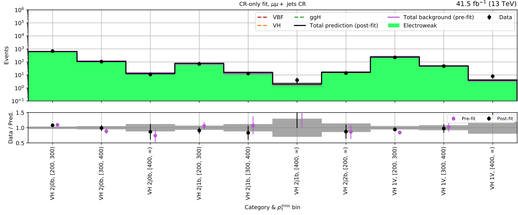
(a) VH - \mu\mu + \text{jets} control region (2017)
