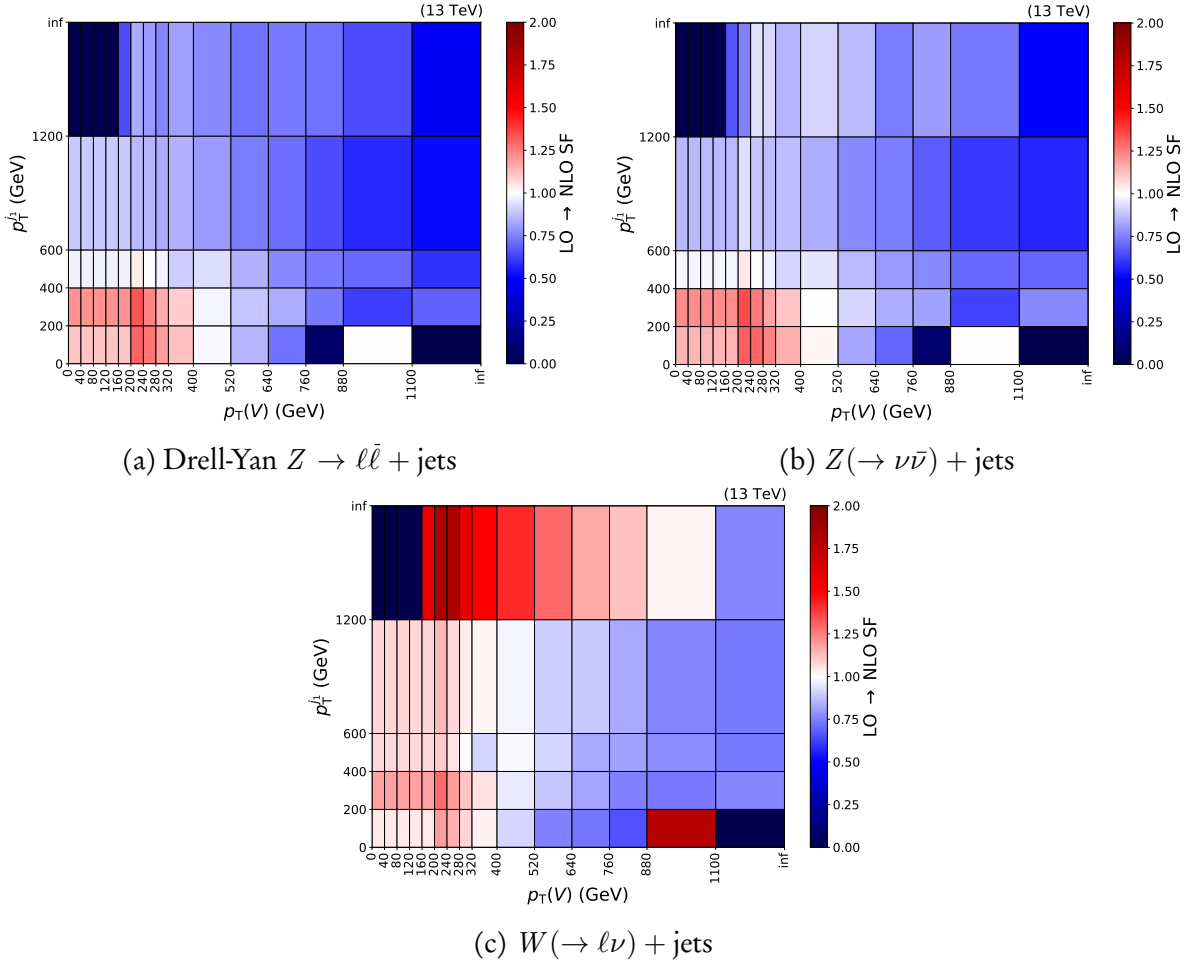
Figure 6.16: NLO k -factors—as a function of the generator-level boson p_T and leading jet p_T —for reweighting reweight events in LO QCD W and Z + jets simulation to NLO accuracy in QCD.
