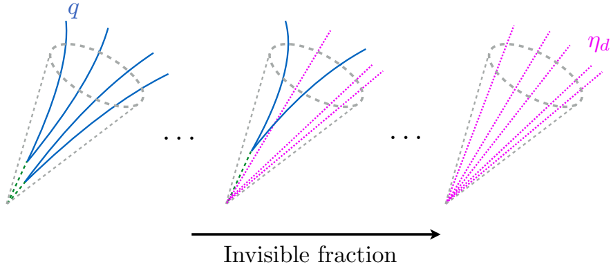
Figure 2.7: The constituents of a semi-visible jet as a function of its invisible fraction r_{\text{inv}} . The green dashed lines signify visibly decaying dark hadrons, blue the SM quarks, and pink the stable dark hadrons. Figure taken from Ref. 70.
