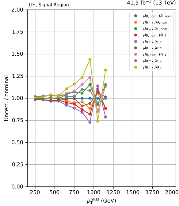
Figure 6.18: The deviations relative to the nominal weight of the combinations of QCD renormalisation and factorisation scale variations. They are presented as a function of p_T^{\text{miss}} inclusive over the t\bar{t}H categories for the t\bar{t} samples. Events are from the signal region in the 2017 dataset after the analysis-level selection.
