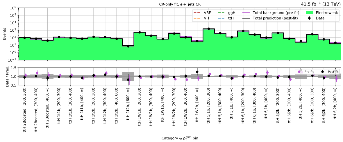
(b) t\bar{t}H - e + \text{jets} control region (2017)
