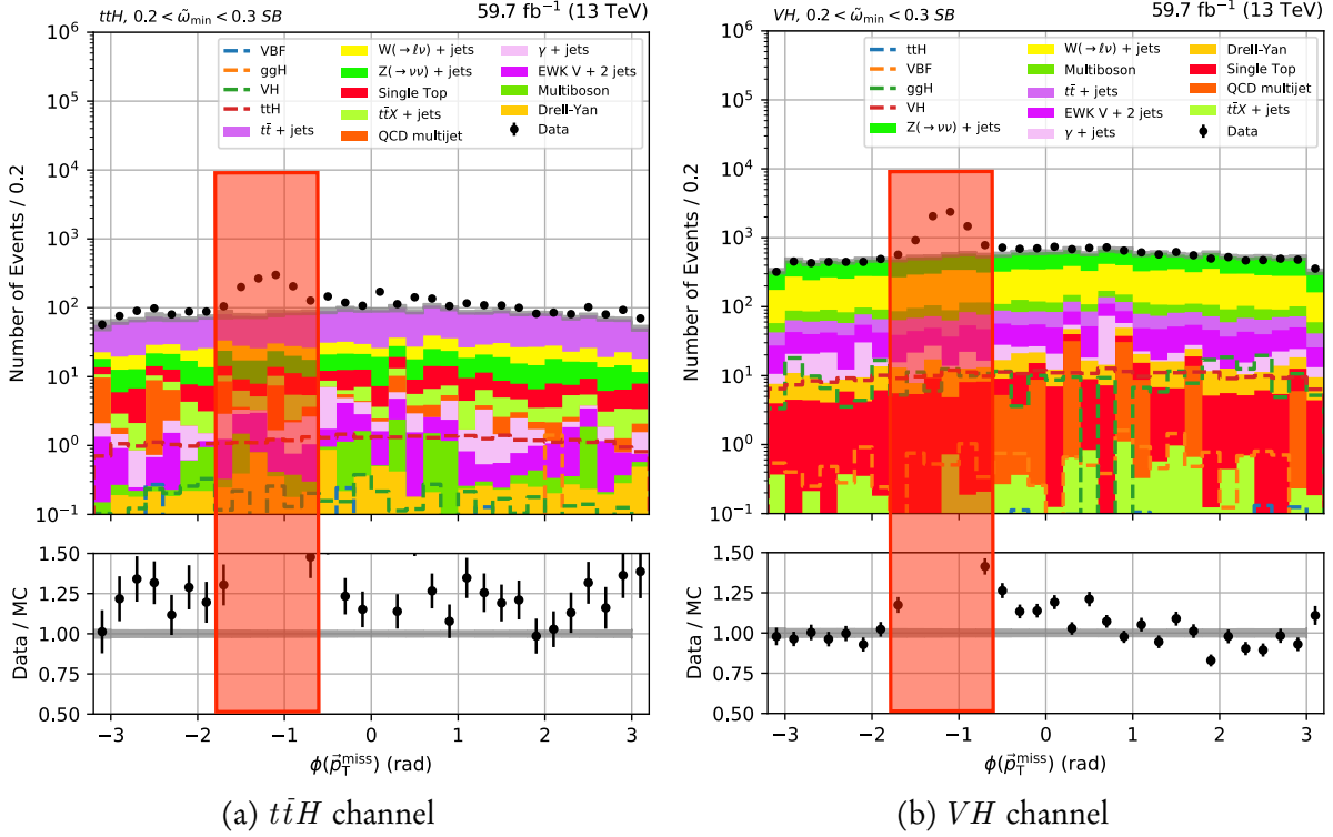
Figure 6.1: The azimuthal angle of the \vec{p}_T^{\text{miss}} in the t\bar{t}H and VH channels before applying the selections designed to mitigate the HEM Issue in 2018. The loose \tilde{\omega}_{\text{min}} sideband is used to demonstrate the effect. A red box encloses the sector that is removed by the selection applied in the signal region and sidebands.
