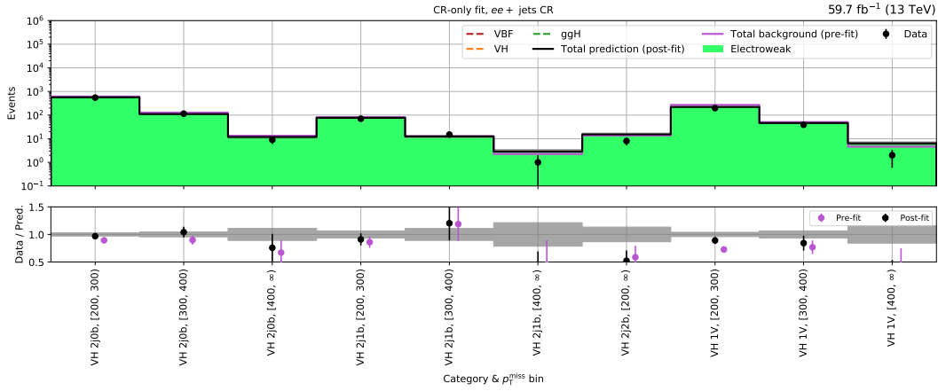
(b) VH - ee + \text{jets} control region (2018)
