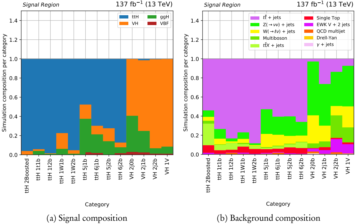
Figure 6.5: Composition of each category in the signal region for simulated signal and background processes after the analysis-level selection.
