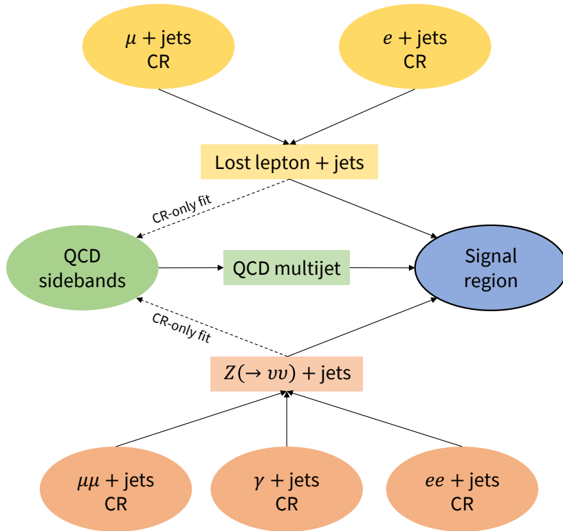
Figure 6.6: An infographic showcasing the role of each analysis region in the fit to data. The control regions predict the lost lepton and Z \rightarrow \nu\bar{\nu} backgrounds, and a control region (CR)-only fit informs the QCD multijet prediction that contributes to the eventual background determination in the signal region.
