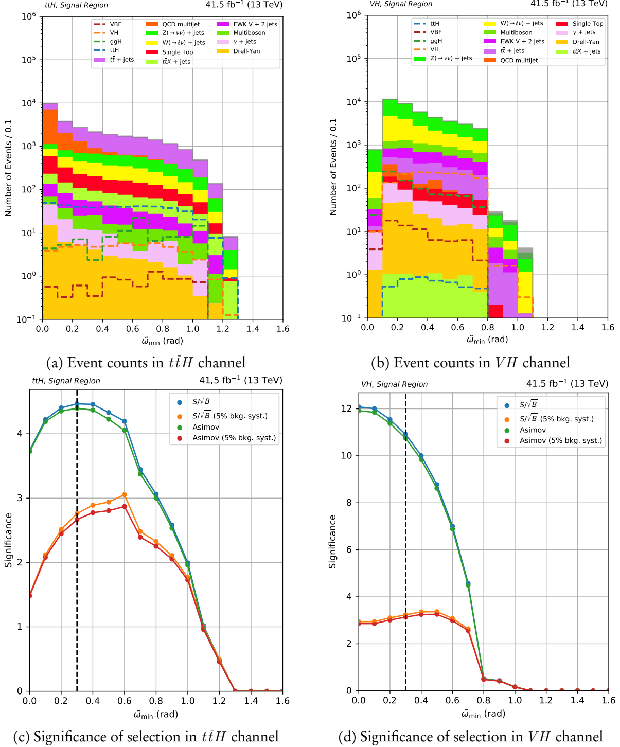
Figure 6.3: Top row: distributions of \tilde{\omega}_{\min} in the signal region inclusive in the t\bar{t}H and VH categories. Bottom row: the significance—from several figures of merit—if a cut is placed to the right of a given value. The black dotted line indicates the threshold used in the analysis. These are showcased after the analysis-level selection on signal and background simulation for the 2017 data-taking era.
