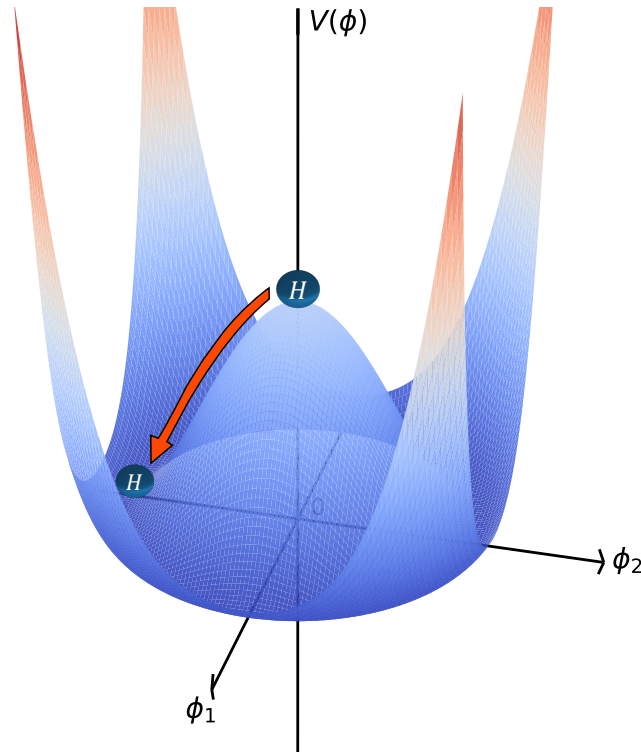
Figure 2.1: A depiction of the Higgs potential V as a function of the component fields. The Higgs boson is initially at (\phi_1, \phi_2) = (0, 0) , an unstable local maximum. It then tumbles into the minimum value of V and triggers electroweak symmetry breaking.
