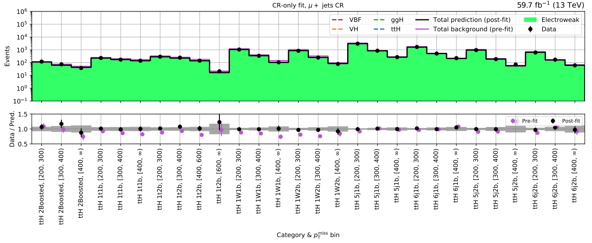
(a) t\bar{t}H - \mu + \text{jets} control region (2018)
