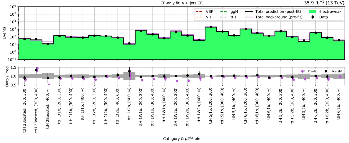
(a) t\bar{t}H - \mu + \text{jets} control region (2016)
