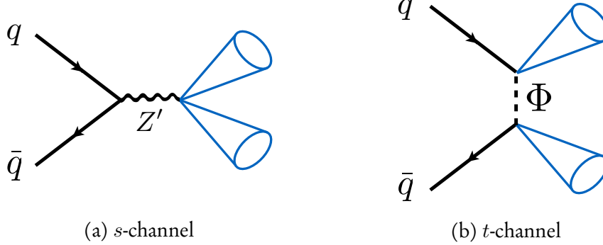
Figure 2.6: Example Feynman diagrams for the two main production modes of semi-visible jets. A Z' boson mediates the s -channel process while a bi-fundamental \Phi mediates the t -channel process. Figure from Ref. 70.
