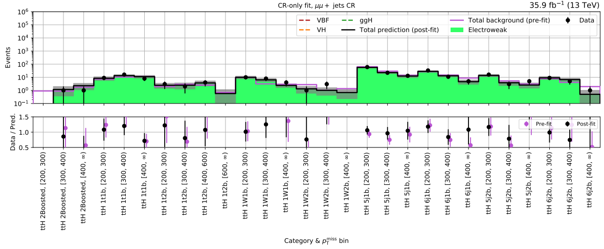
(a) t\bar{t}H - \mu\mu + \text{jets} control region (2016)
