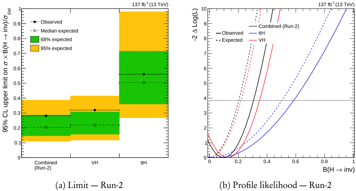
Figure 6.24: Observed and expected 95 % CL upper limit on the Higgs boson to invisible state branching fraction \mathcal{B}(H \rightarrow \text{invisible}) (left) and the corresponding profile likelihood scan (right), for both the individual categories, as well as the combination of them, for the full Run-2 dataset. The standard model Higgs boson with its associated mass and production cross section are assumed.
