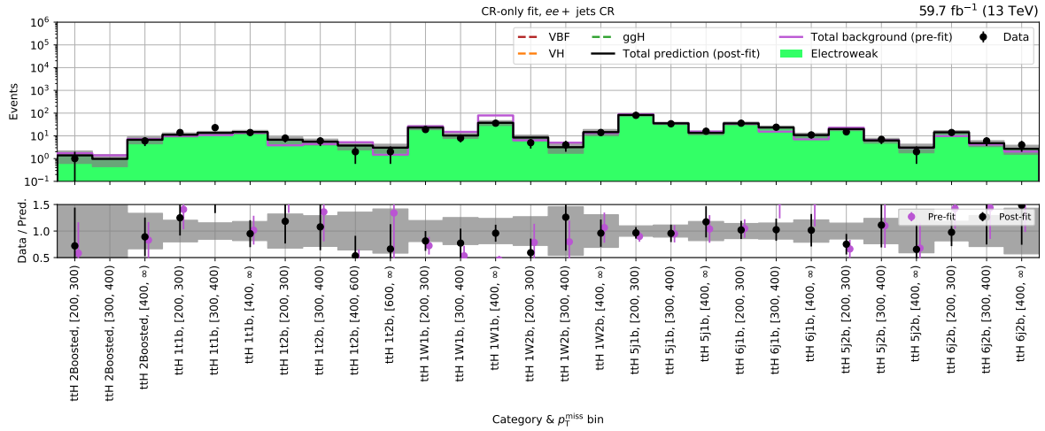
(b) t\bar{t}H - ee + \text{jets} control region (2018)
