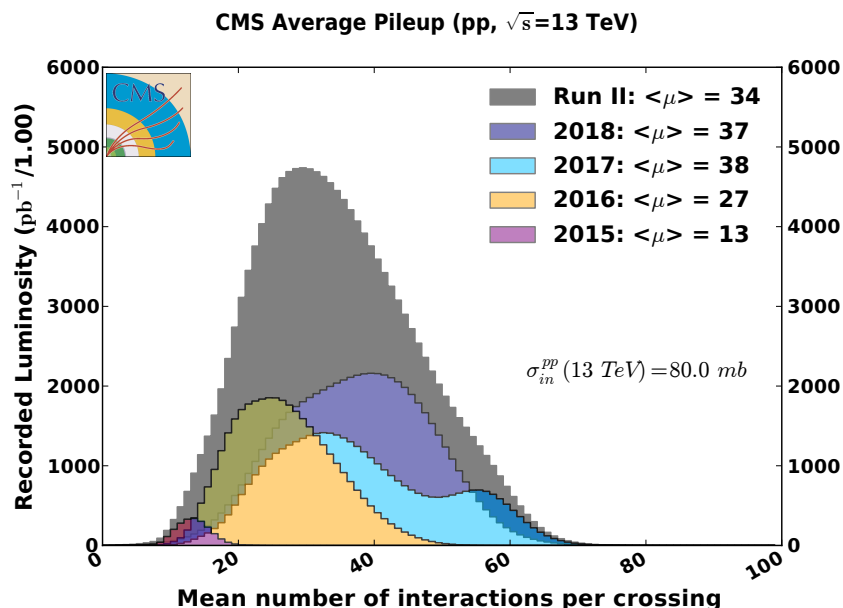
Figure 3.2: The average number of pileup interactions per bunch crossing at CMS during Run-2 of the LHC. Figure obtained from Ref. 53.
