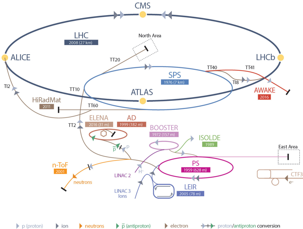
Figure 3.1: A schematic of the CERN accelerator complex. Various particles are shown from their sources to the interaction points enveloped by the detectors. Figure obtained from Ref. 127.
