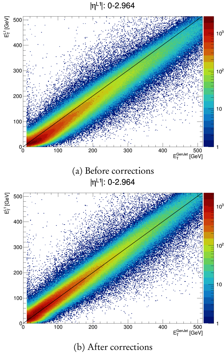
Figure 3.9: The energies of matched pairs of jets from simulation in the entire barrel and end cap, in the pileup 40–50 range, before and after jet energy corrections have been applied.
