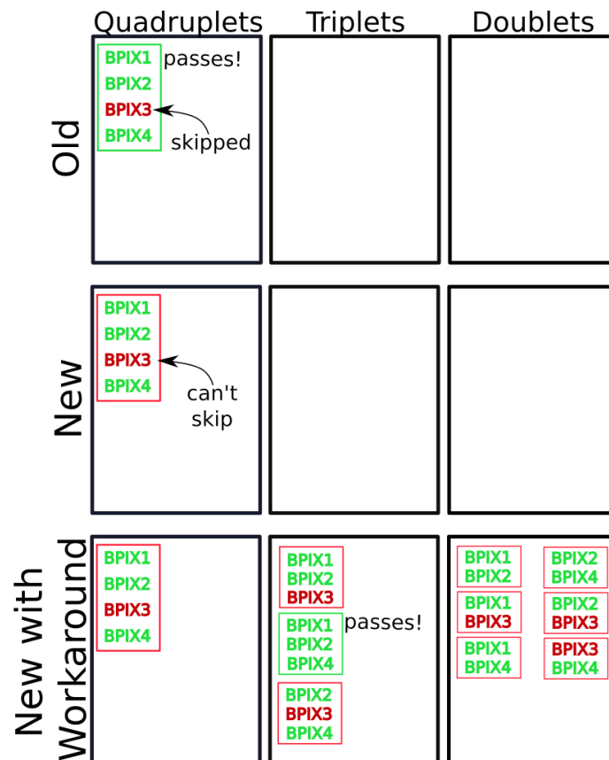
Figure 4.10: Demonstration of how the lack of hit-skipping can lead to the loss electron seeds. Top: Behavior of original matching code with hit skipping. Middle: New code without hit skipping. Bottom: New code with workaround that recovers the seed.
