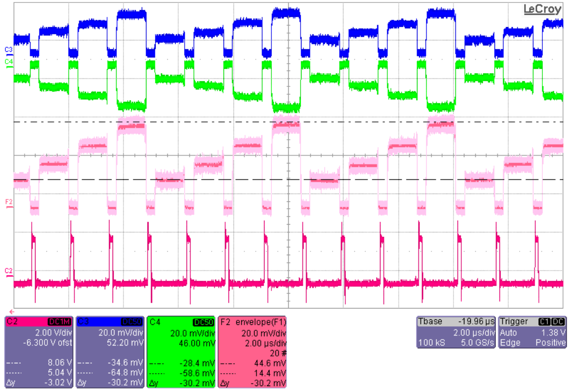
Figure 6.23: The calibration “step curve” for an APC128 chip. In this oscilloscope trace the signal has been routed through a differential amplifier, thus the inverted blue and green traces. The pink envelope shows the subtraction of the differential signals and clearly demonstrates the “step” nature of the signal. The dark pink curve shows the R\Phi 1 signal which, together with R\Phi 2 , steps the channel selection bit through the readout shift register.
