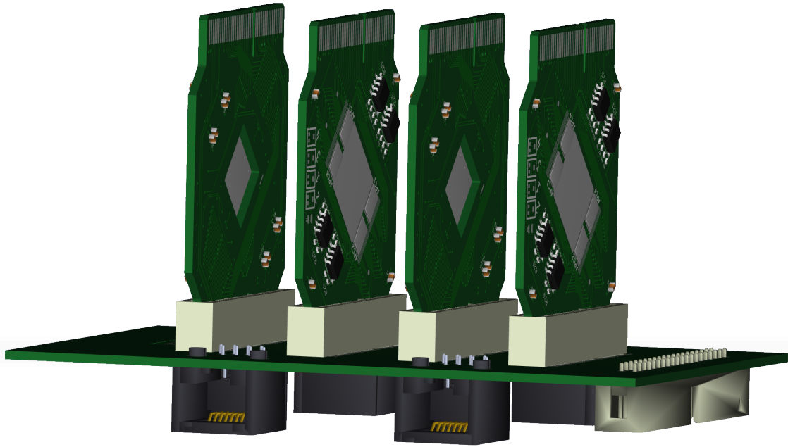
Figure 6.27: One of the two identical back-plane boards that make up the in-beam part of the telescope. The silicon micro-strip detectors are mounted at a 45 degree angle relative to the back-plane board, and each of the cards has board-edge connectors on both the top and bottom. This means that the cards can be rotated 180 degrees to change the relative orientation of the strips. They can be alternating horizontal-vertical (as shown), all vertical, all horizontal or any combination according to the operator's needs.
