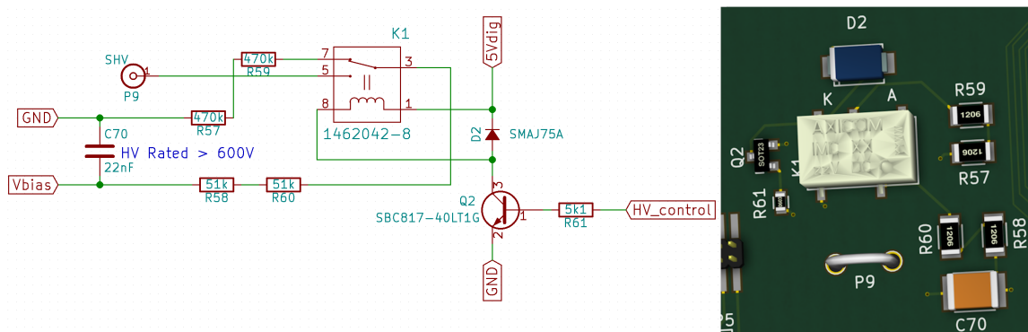
Figure 6.32: Bias voltage control. High voltage is supplied by an external source and connected to the board via a chassis mounted SHV connector. A mechanical relay, controlled by a signal coming from the FPGA, controls whether bias voltage gets supplied to the micro-strip detectors. Large value serial resistors are used to limit any potential shock hazard.
