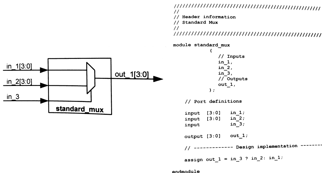
Figure 6.33: A simple example of some Verilog code[97]. This shows how one may implement a 2-input 4-bit multiplexer. Note many of the C-like syntax features.
