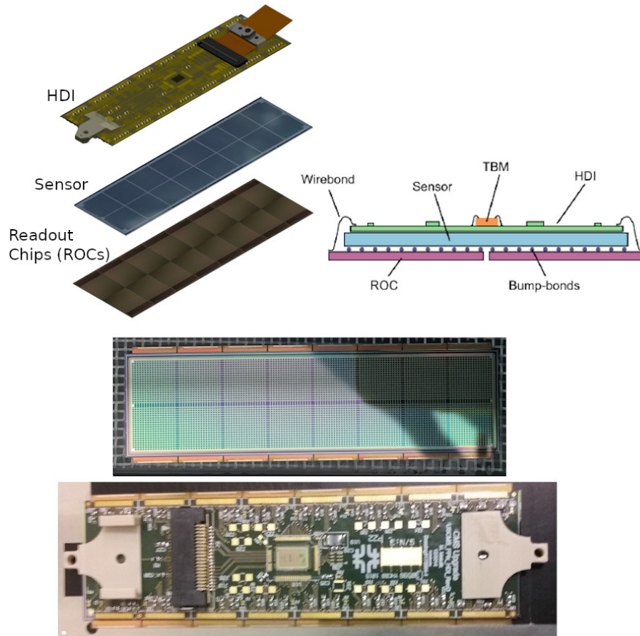
Figure 6.4: The Phase I FPIX module. Top Left: Exploded view showing the three layers that makeup a module. Top Right: Profile view showing the components, including the wirebonds and bump-bonds. Bottom: Photographs of a BBM (top) and full module (bottom).
