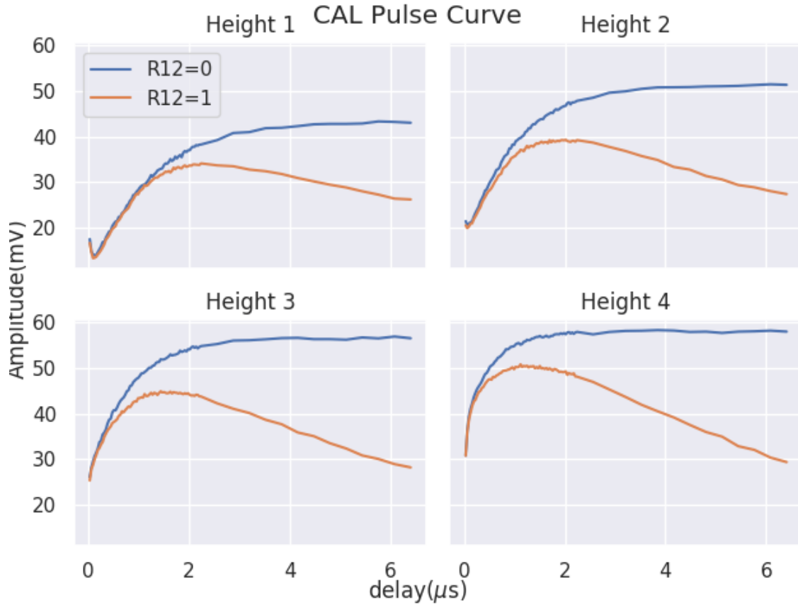
Figure 6.26: The relationship between the output voltage and the time delay between when the calibration charge is injected and when the pre-amplifier is sampled. Height 1-4 correspond to the four calibration capacitor values. The value of R12 indicates whether or not the switch enabling the feedback resistor is open(0) or closed(1).
