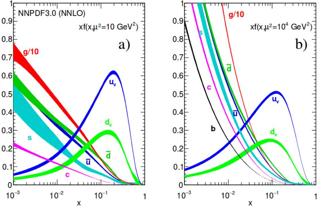
Figure 2.3: Parton distribution functions for two values of momentum transfer, \mu . The u_v and d_v refer to the proton’s valence up and down quarks. Other quark flavors exist through the temporary splitting of gluons into quark-antiquark pairs.[6]
