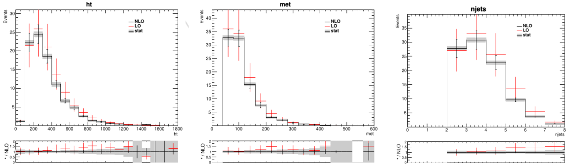
Figure 5.8: Comparison of the LO and NLO kinematics for t\bar{t}Z . The error bars on the NLO (black) and LO (red) are the corresponding scale uncertainties. The grey band shows the NLO statistical uncertainty.
