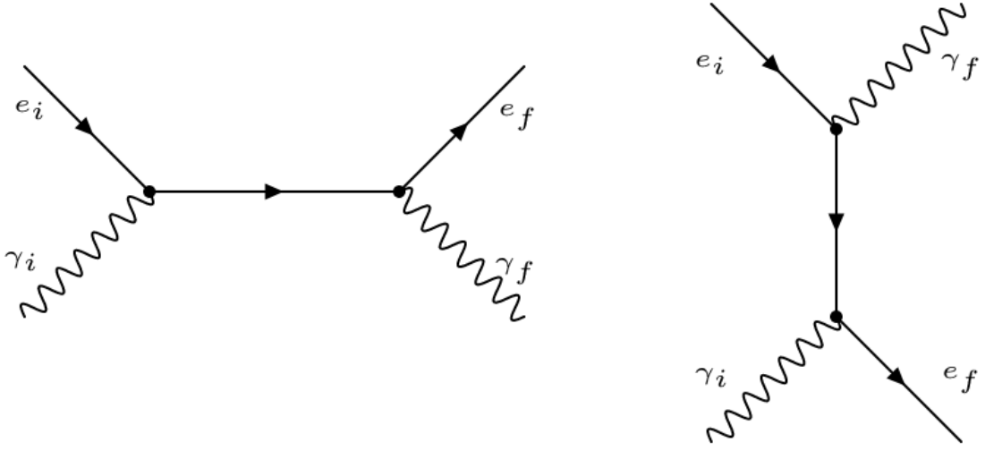
Figure 2.2: Leading order Feynman diagrams for Compton scattering. The topology of the left diagram is conventionally referred to as “s-channel” while the right’s is called “t-channel”. Initial particles are on the left of each diagram, and final state particles are on the right.
