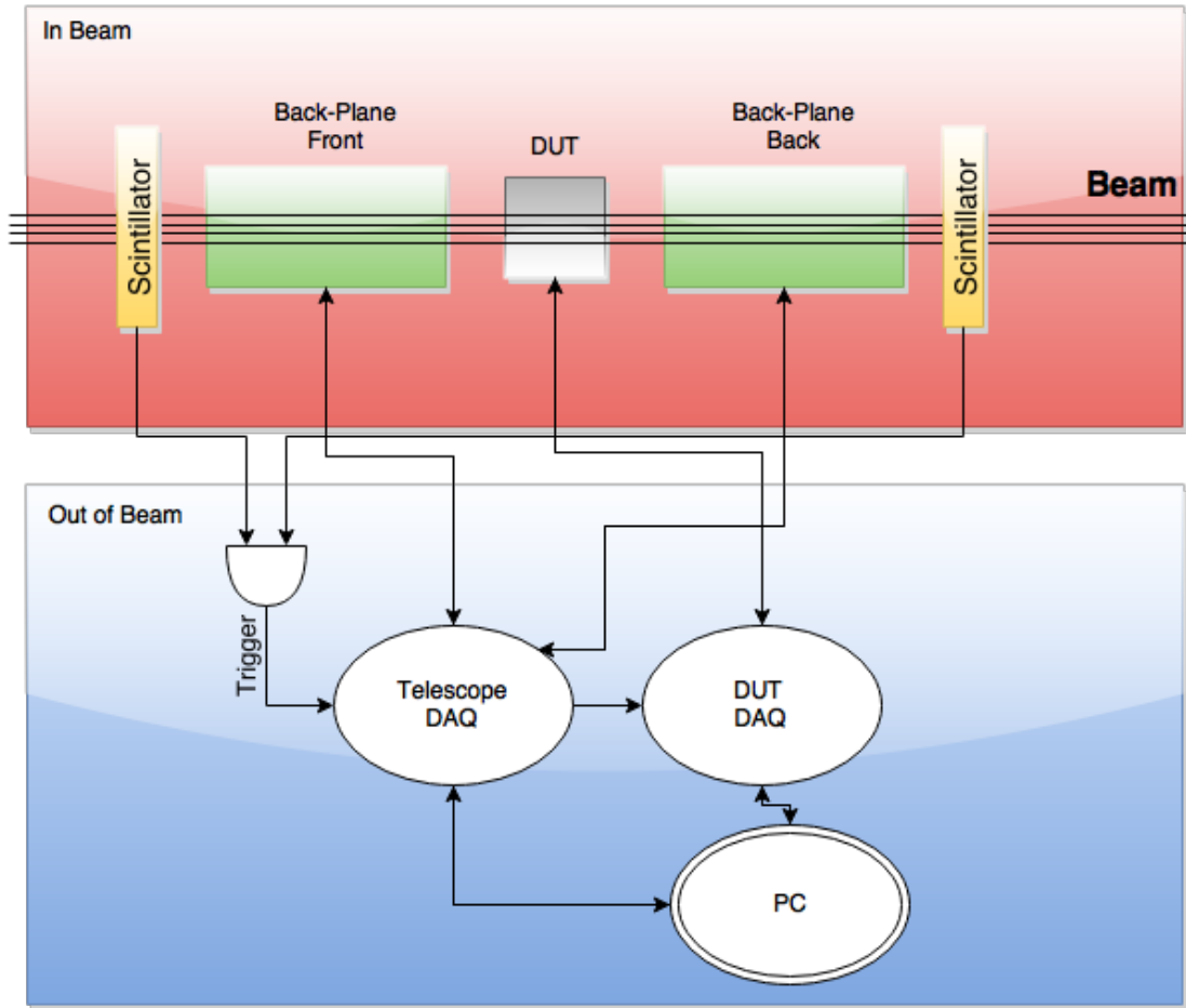
Figure 6.20: Block diagram of the telescope. The lines represent signal flow. Two scintillation detectors are used to trigger the readout of the system. The trigger is handled first by the Telescope DAQ, and then passed on to the DUT's DAQ. Collection of data from the telescope and DUT then occurs in parallel.
