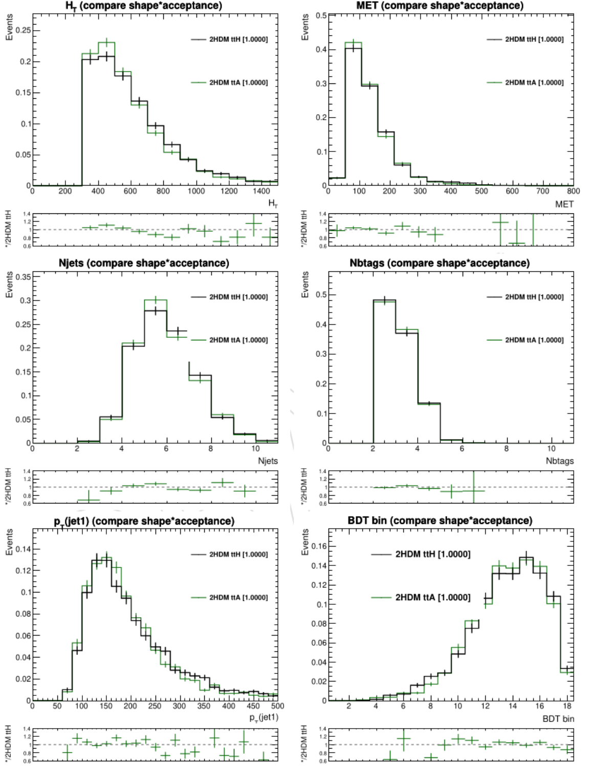
Figure 5.19: Distributions comparing analysis-level observables for the scalar and pseudoscalar processes with both masses set to 450 GeV at \tan \beta = 1 . The distributions have been divided by their corresponding cross section so both the shape and acceptance of the distributions are comparable.
