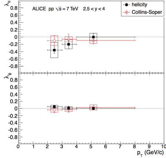
Figure 1.21: \lambda_\theta and \lambda_\phi parameters of the inclusive J/\psi polarization as a function of p_T , measured in the Helicity (closed squares) and Collins-Soper (open circles) reference frames [151].
