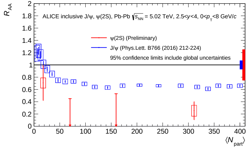
Figure 3.20: Nuclear modification factor of the \psi(2S) (red) compared to the one of the J/\psi (blue) as a function of N_{\text{part}} . For the centrality bins where the signal could not be extracted, only the 95% confidence limit is shown. The global systematic uncertainty is drawn in the box around unity. The global uncertainties are already included in the confidence limit calculation.
