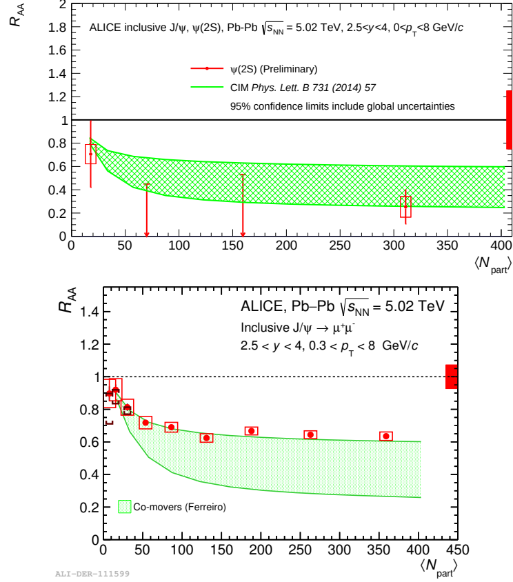
Figure B.2: Nuclear modification factor R_{AA} versus N_{part} compared to the CIM for the \psi(2S) (top) and the J/\psi (bottom). For the centrality bins where the signal could not be extracted, only the 95% CL is shown. The red box around unity corresponds to the global uncertainty which are included in the confidence limits calculation and therefore do not apply to the CL. Uncertainties in the model correspond to different values of the c - \bar{c} pairs production cross sections, \sigma_{c\bar{c}} = 0.70 mb for the upper limit and \sigma_{c\bar{c}} = 0.45 mb for the lower limit.
