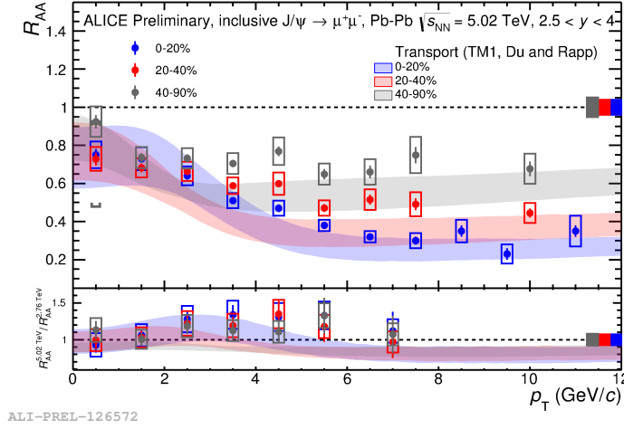
Figure 1.26: Inclusive J/\psi R_{AA} at \sqrt{s_{NN}} = 5.02 TeV as a function of p_T measured in three different centrality bins, compared to Transport Model Calculations. The lower panel presents the ratio of this R_{AA} with respect to the \sqrt{s_{NN}} = 2.76 TeV [158].
