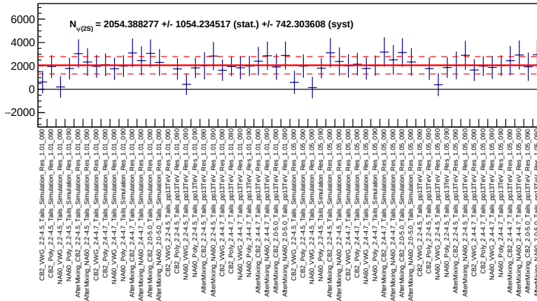
Figure 3.8: Different signal extraction tests, for the rapidity and p_T -integrated invariant mass distributions, in the centrality range 0-90%.
