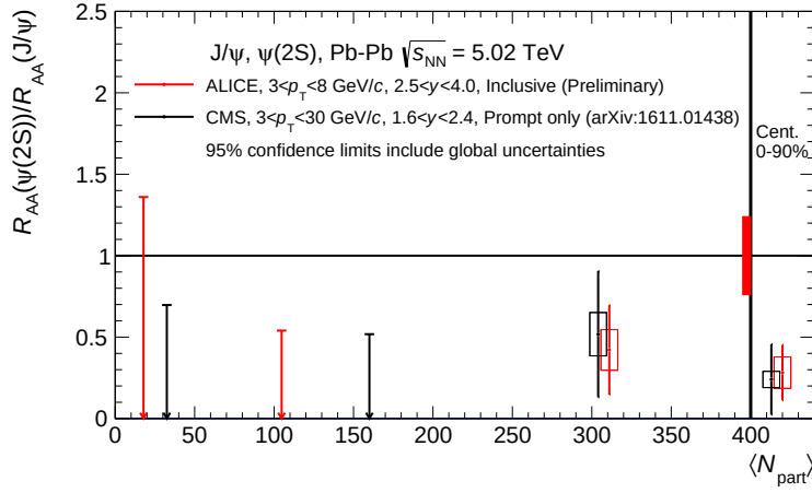
Figure 3.25: Double-ratio R_{AA}^{\psi(2S)}/R_{AA}^{J/\psi} as a function of N_{\text{part}} (red) compared to the values of CMS (black) for p_T > 3 GeV/ c . For the centrality bins where the signal could not be extracted, only the 95% confidence limit is shown. The global systematic uncertainty is drawn in the box around unity. The global uncertainties are already included in the confidence limit calculation. The value quoted for N_{\text{part}} > 400 corresponds to the centrality-integrated value (0-90%).
