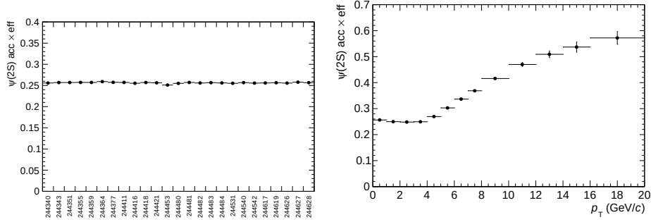
Figure 3.15: p_T - and y -integrated \psi(2S) acceptance \times efficiency as a function of run number (left) and acceptance \times efficiency as a function of p_T (right) using p_T and y input distributions from the J/\psi measurement at \sqrt{s} = 5 TeV.
