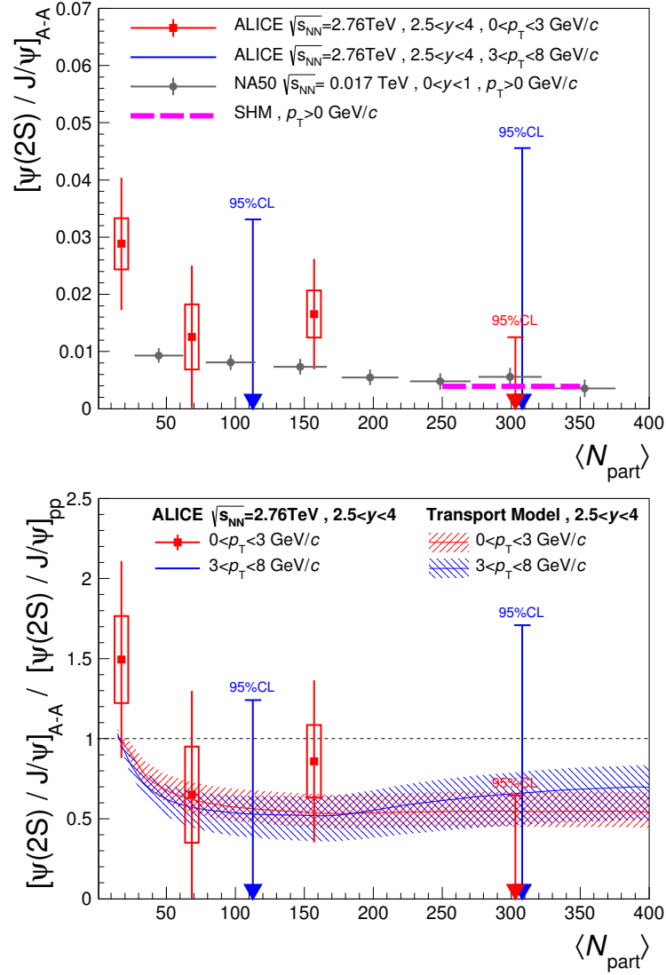
Figure 1.27: Inclusive \psi(2S) -to- J/\psi ratio measured as a function of centrality in Pb – Pb collisions at \sqrt{s_{NN}} = 2.76\text{ TeV} for two p_T intervals, compared to NA50 results [159] and to a theoretical calculation [160] (left). Double ratio as a function of centrality, between the \psi(2S) and J/\psi measured in Pb – Pb collisions at \sqrt{s_{NN}} = 2.76\text{ TeV} and pp collisions at \sqrt{s} = 7\text{ TeV} , compared to theoretical calculations [161] (right) [156].
