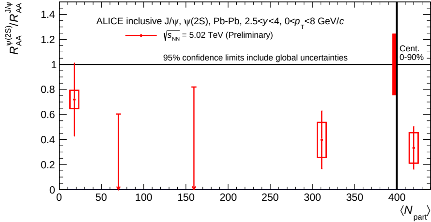
Figure 3.23: Double-ratio R_{AA}^{\psi(2S)}/R_{AA}^{J/\psi} as a function of N_{\text{part}} for 0 < p_T < 8 \text{ GeV}/c . For the centrality bins where the signal could not be extracted, only the 95% confidence limit is shown. The global systematic uncertainty is drawn in the box around unity. The global uncertainties are already included in the confidence limit calculation. The value quoted for N_{\text{part}} > 400 corresponds to the centrality-integrated value (0-90%).
