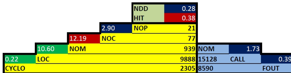
Figure 5.7: Overview Pyramid for the FFMM 3.0 source code.
