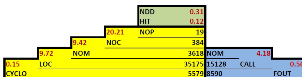
Figure 5.6: Example of a complete Overview Pyramid.
