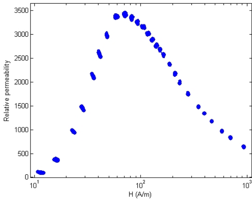
Figure 6.13: Relative permeability of the soft steel sample.
