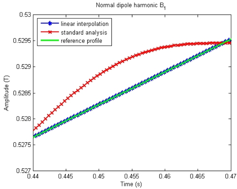
Figure 4.5: Detail of first normal harmonic ( B_1 ) comparison: linear profile, m=1 , ramp rate 0.0628 \text{ T/s} .
