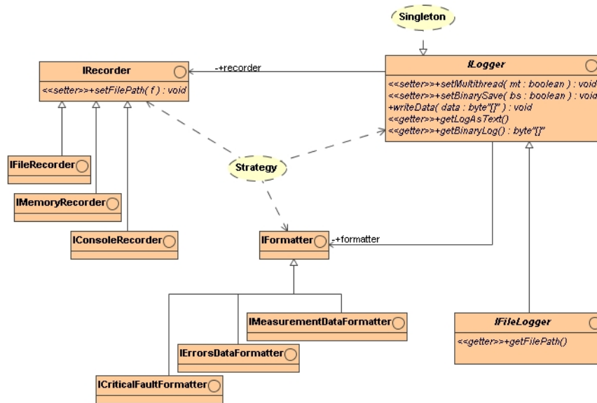
Figure 3.7: FFMM logger architecture.
