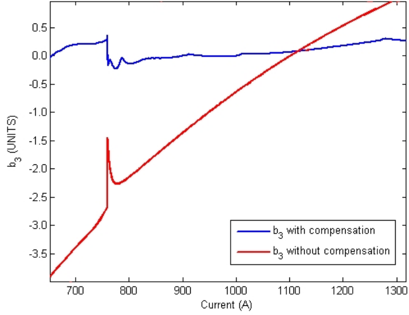
Figure 6.5: Integral b_3 component vs. current with and without compensation, in the dipole magnet MB2524 during an LHC cycle.
