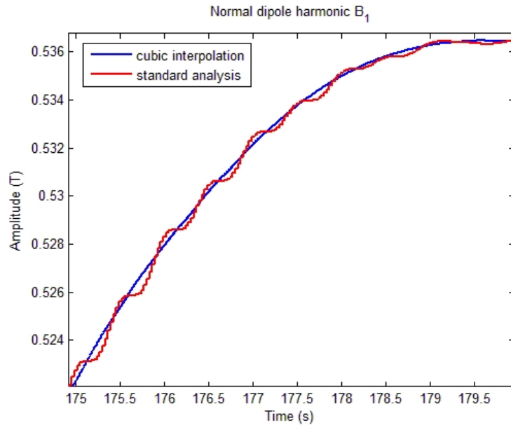
Figure 7.3: Main normal harmonic ( B_1 ) over a linear-parabolic current profile, m = 4 .
