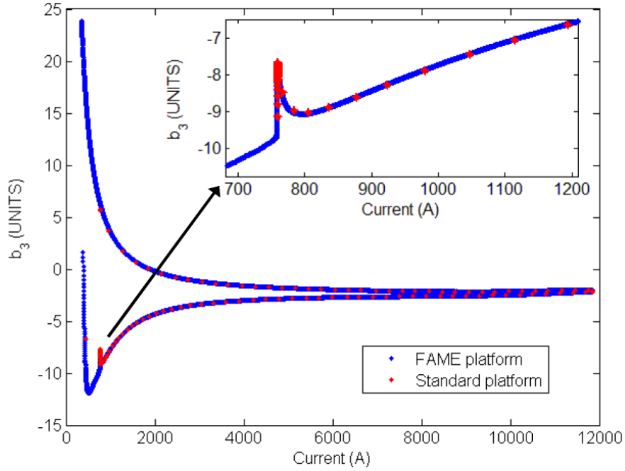
Figure 6.7: Estimation of the sextupole with the old and the new acquisition system.
