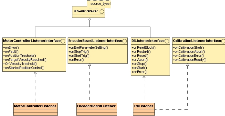
Figure 3.6: FFMM actions and listeners infrastructure.
