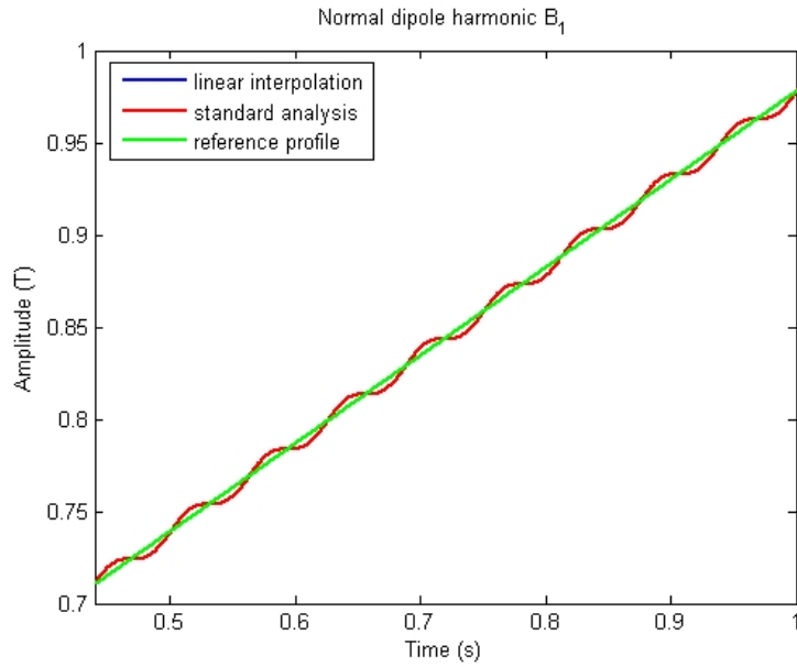
Figure 4.6: First normal harmonic ( B_1 ) comparison: linear profile, m=1 , ramp rate 0.4776 \text{ T/s} .
