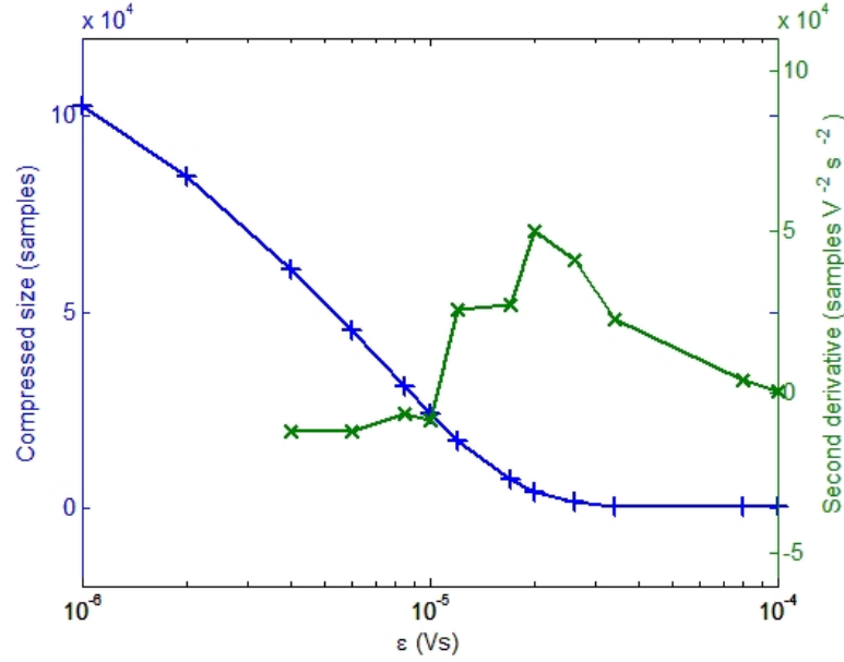
Figure 4.2: Rate-distortion plot and heuristic determination of the noise strength ( \epsilon = 2 \times 10^{-5} Vs), corresponding to the maximum of the second derivative.
