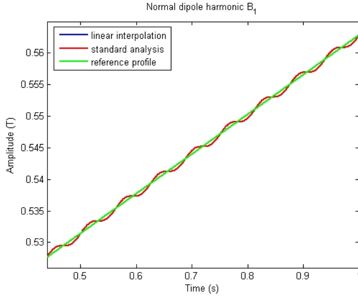
Figure 4.4: First normal harmonic ( B_1 ) comparison: linear profile, m=1 , ramp rate 0.0628 \text{ T/s} .
