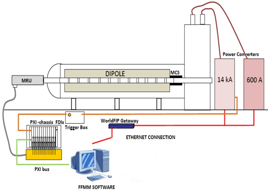
Figure 6.2: Architecture of the tracking test measurement station.
