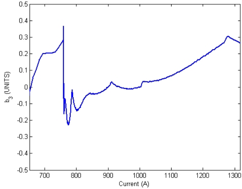
Figure 6.6: Residual integral b_3 component vs. current with compensation, in the dipole magnet MB2524 during an LHC cycle.
