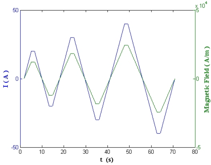
Figure 6.11: Measured current and computed magnetic field without sample.
