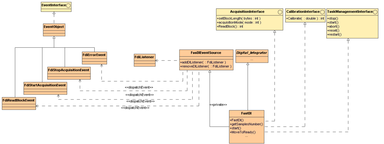
Figure 3.5: FFMM event handling architecture.
