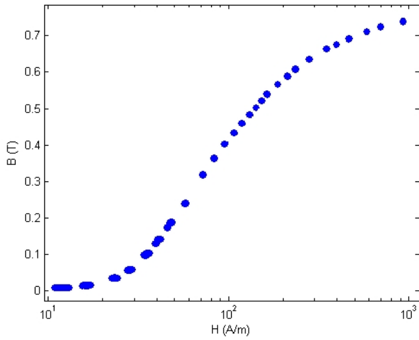
Figure 6.12: First magnetization curve of the soft steel sample.
