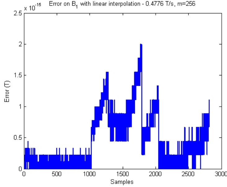
Figure 4.13: Error on B_1 with linear interpolation: linear profile, m=256 , ramp rate 0.4776 \text{ T/s} .
