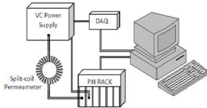
Figure 6.9: Architecture of the new permeability measurement bench.
