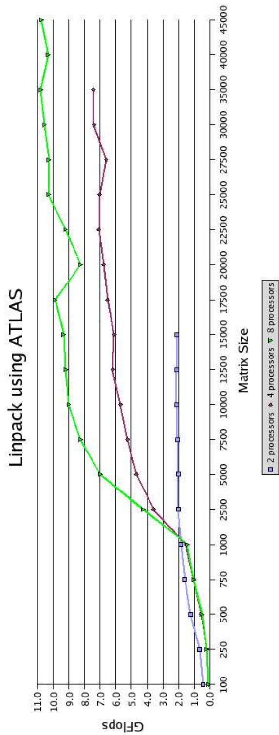
Figure 5.9: Results of varying processor numbers using ATLAS
