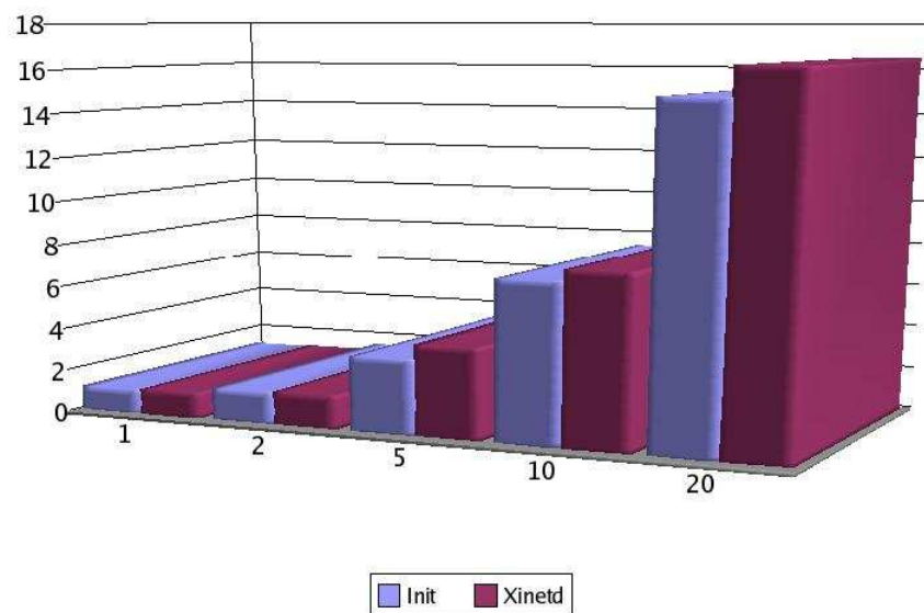
Figure 5.8: Effect on real time when increasing the number of concurrent users of a 2.4.3 gatekeeper in seconds
