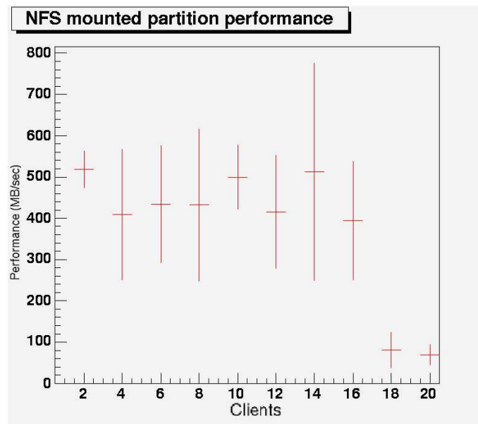
Figure 5.11: Read performance for NFS mounted RAID partition in MB/sec using 100MB file
