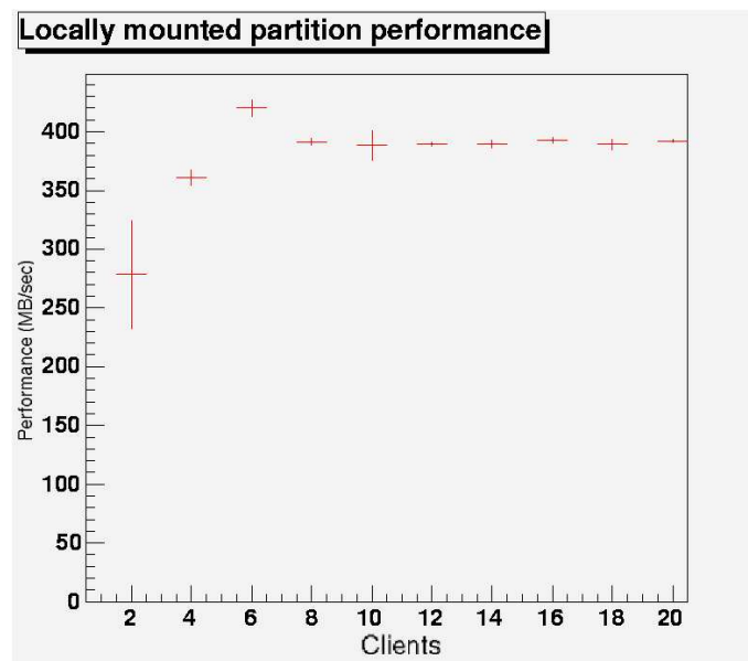
Figure 5.12: Read performance for locally mounted RAID partition in MB/sec using 100MB file
