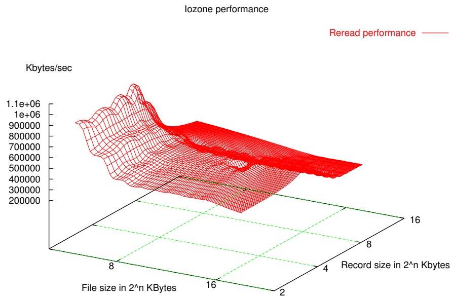
Figure 5.15: Re-Read performance for locally mounted RAID partition using the IOZone benchmark
