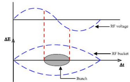
Figure 2.4: A sketch showing formation of a bunch.
