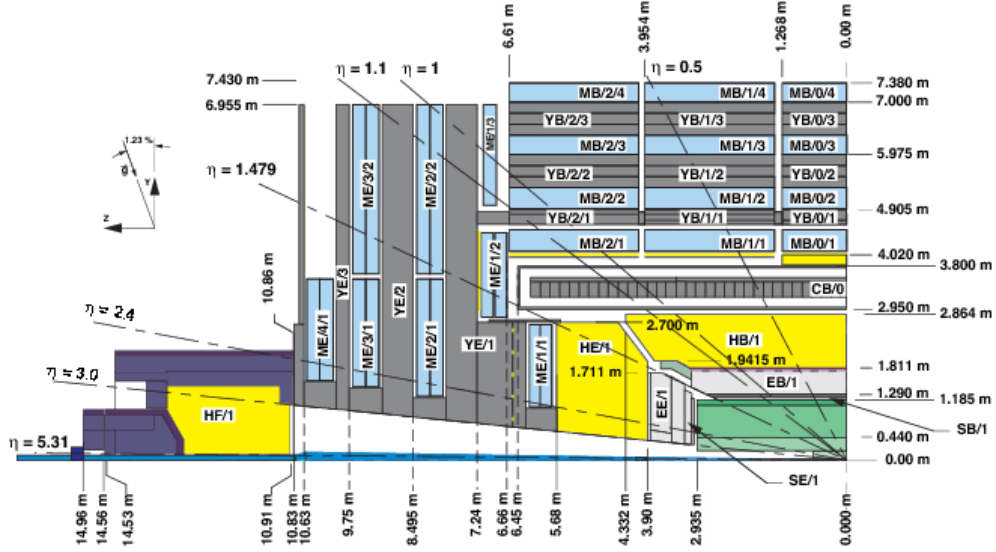
Figure 2.15: A schematic view of a quadrant of the CMS Hadron calorimeter presenting different sub-detectors (in yellow color).
