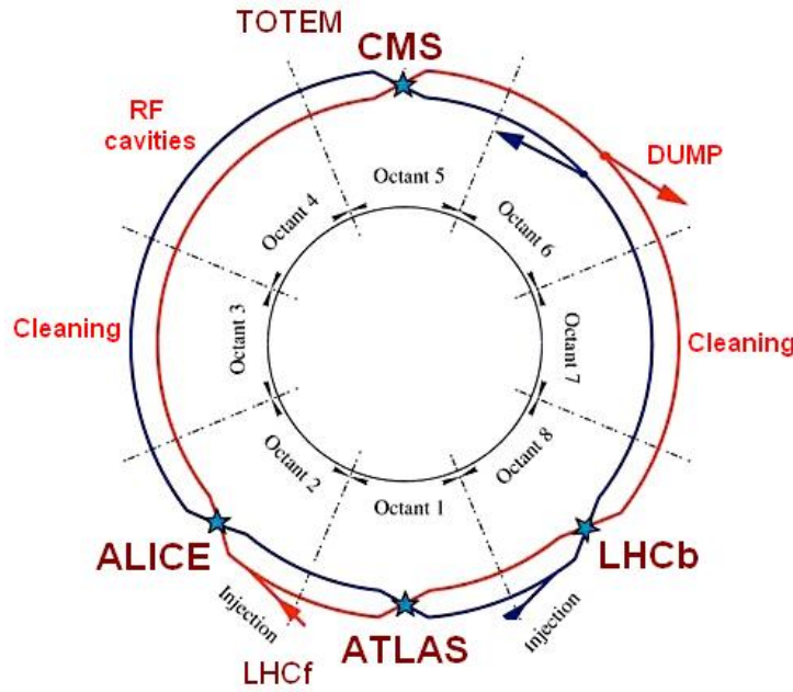
Figure 2.2: A schematic layout of the LHC tunnel.
