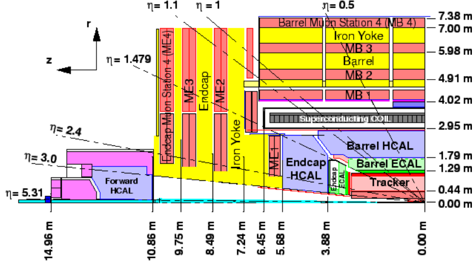
Figure 2.9: Longitudinal contour of a quadrant of the CMS detector.
