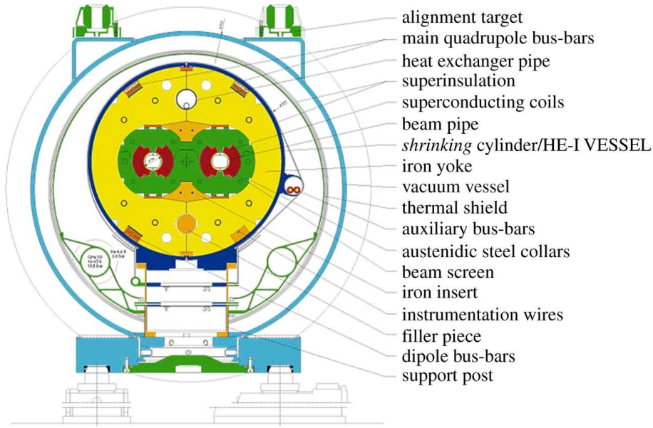
Figure 2.5: The LHC twin-bore magnet system
