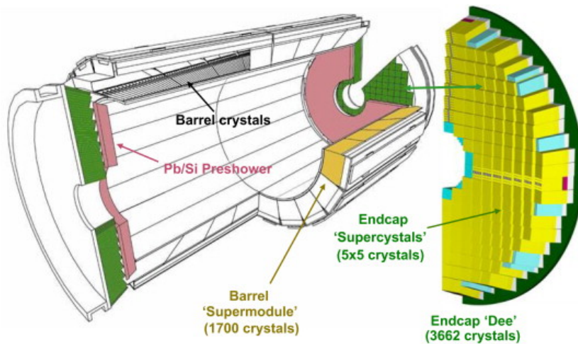
Figure 2.14: A layout of the CMS Electromagnetic calorimeter displaying the arrangement of crystals in barrel and endcaps with the preshower present in front.
