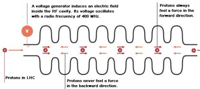
Figure 2.3: A Radio Frequency cavity.
