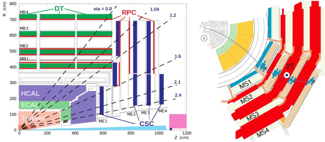
Figure 2.17: A schematic view of the solenoidal magnet used in CMS, showing the coil and the central return yoke. The trajectory of a muon through the muon stations is also presented.
