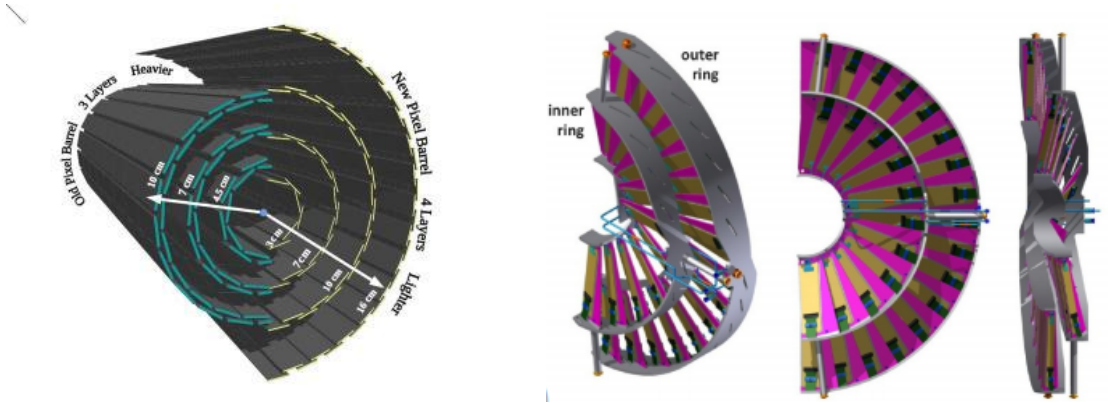
Figure 2.12: A schematic representation of the upgrades in pixel detector barrel (left) and endcaps (right) during Phase1 Pixel Upgrade.
