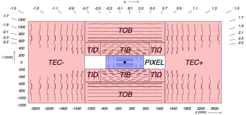
Figure 2.10: A cross-sectional view of the CMS tracker system in r - z plane, with each line representing a silicon detector module.
