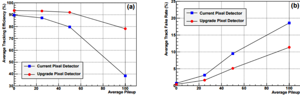
Figure 2.13: Performance measurement of the older pixel detector (blue) and the upgrade pixel detector (red) using t\bar{t} events, showing tracking efficiency (left) and fake rate (right) as a function of per event pileup [115].
