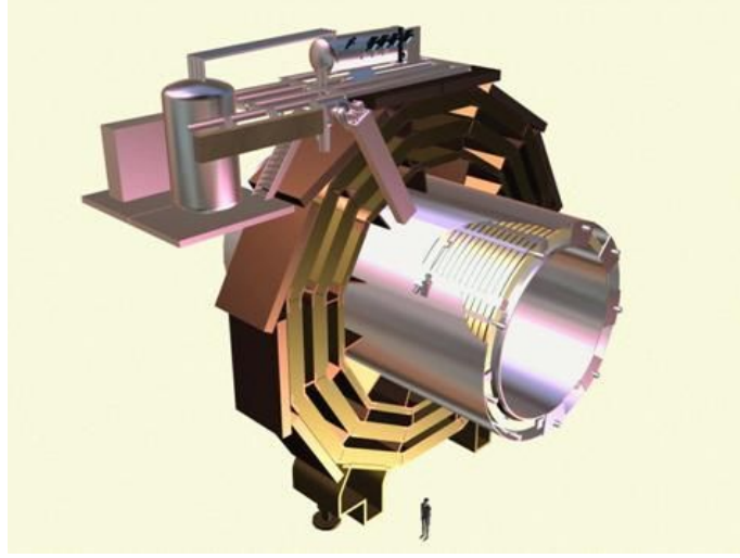
Figure 2.16: A schematic view of the solenoidal magnet used in the CMS detector, showing the coil and the central return yoke.
