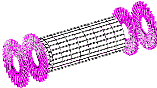
Figure 2.11: A schematic layout of the CMS pixel detector.
