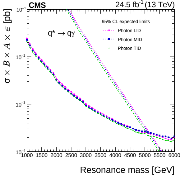
Figure 4.22: Expected 95% CL upper limits on \sigma \times \text{BR} \times A \times \epsilon versus q^* mass for different photon ID cuts corresponding to SM coupling f = 1.0 .
