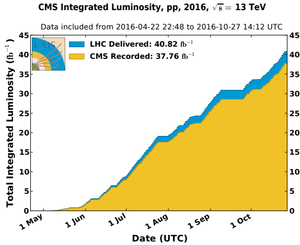
Figure 2.7: Total integrated luminosity delivered by the LHC and recorded by CMS as a function of time, during the year 2016 [108].
