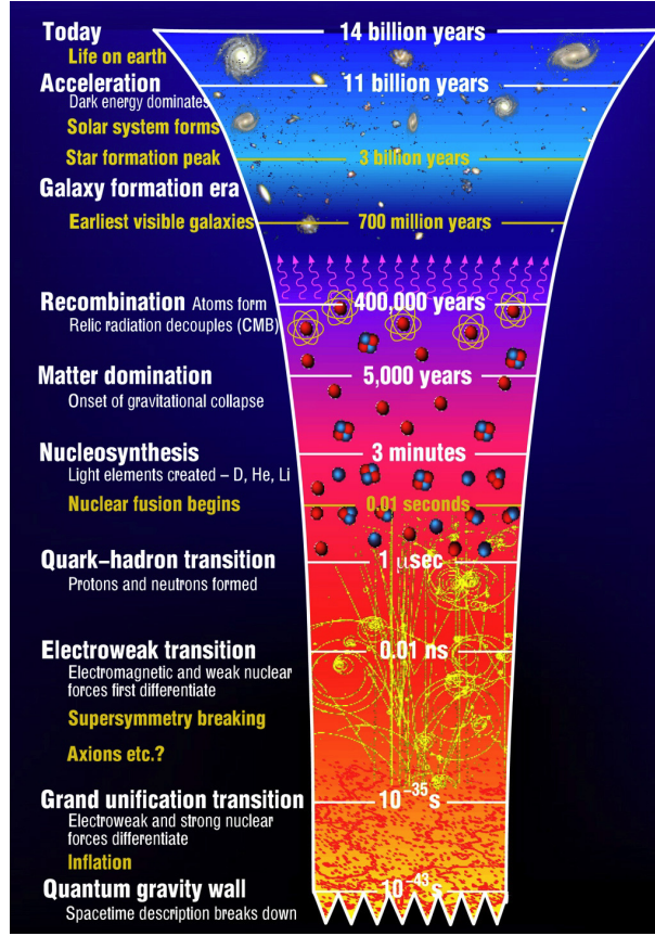
Figure 2.1: Big-Bang timeline.
