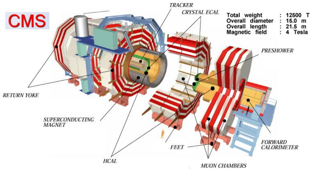
Figure 2.8: A layout of the CMS experiment at CERN.
