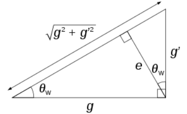
Figure 1.2: W^{\mu3} - B^\mu plane
