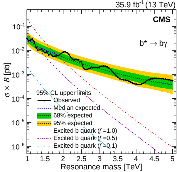
Figure 4.46: The observed and expected 95% CL upper limits on \sigma \times B as a function of the mass of the excited b-quark, for f = 1.0 . The limits are also compared with theoretical predictions for excited b-quark production for the three couplings. The inner (green) band and the outer (yellow) band indicate the regions containing 68% and 95%, respectively, of the expected limits.
