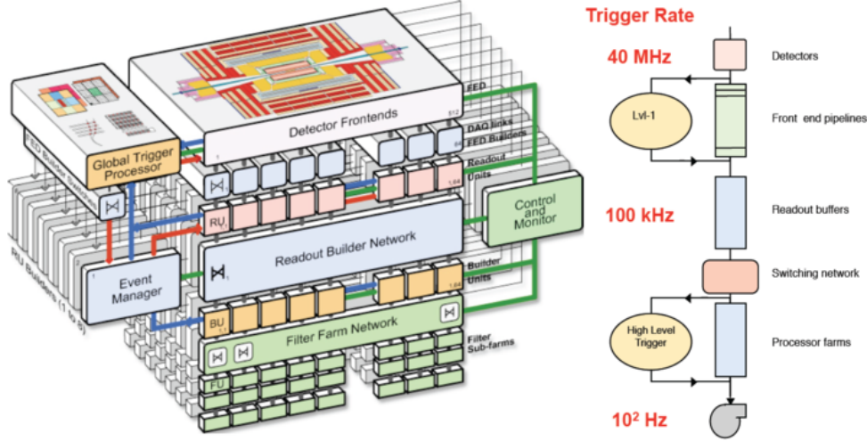
Figure 2.18: CMS Data Acquisition and trigger system.
