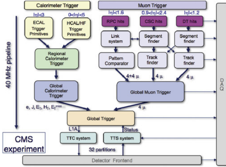
Figure 2.19: An architecture of CMS Level-1 trigger system.
