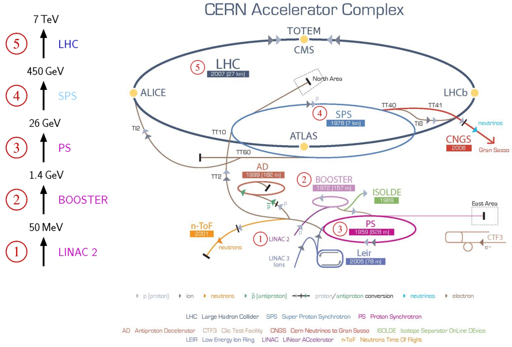
Figure 2.6: A schematic view of CERN accelerator complex representing the different accelerators deployed for providing acceleration to the proton beam.
