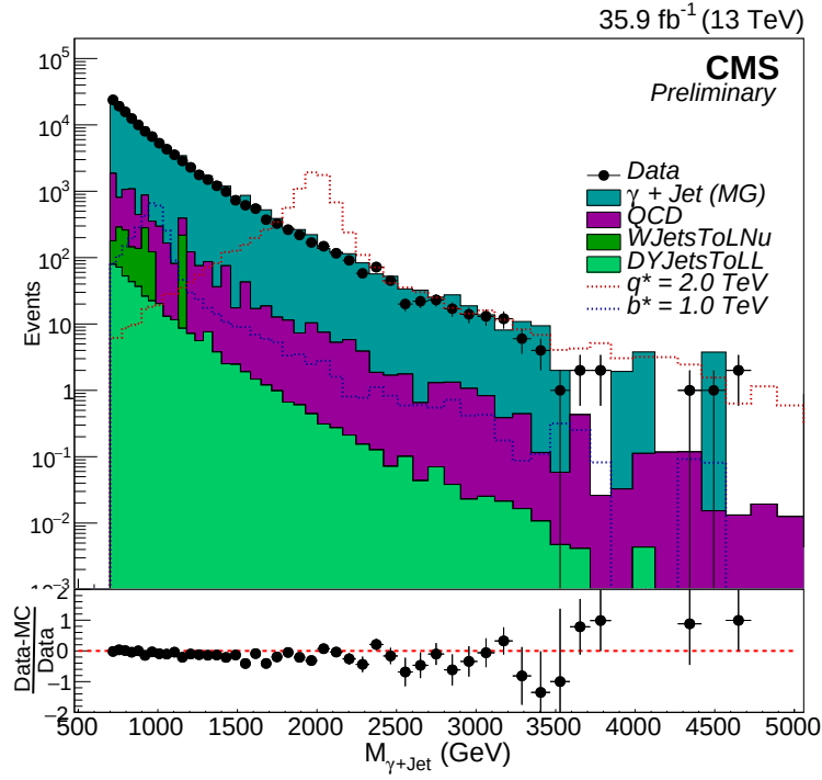
(a) M_{\gamma+\text{jet}}
