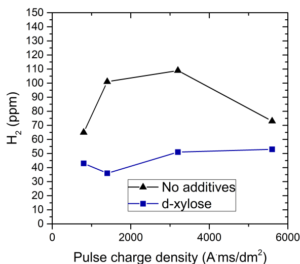
Figure 6.9. \text{H}_2 concentration (atomic ppm) as a function of pulse charge density per period ( J_{on} \times T_{on} ). The two electrolytes are compared.
