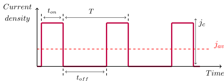
Figure 6.2. Schematic of pulse plating sequence and definition of the parameters.
