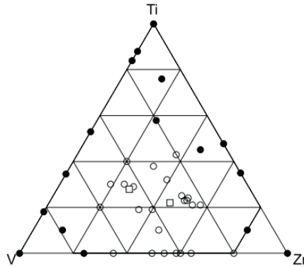
Figure 1.4. Quality composition of TiZrV coatings based on the R criteria as a function of the in-depth elemental composition (measured by EDX). The samples with a R \geq 0.5 are represented by empty symbols and the samples with a R < 0.5 are represented with black symbols. From Prodromides [24].
