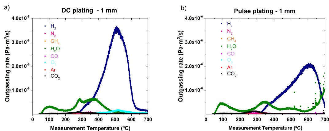
Figure 5.9. H_2 , H_2O , O_2 , CO_2 , CH_4 , N_2 outgassing for the DC (a) and PC (b) electroformed copper, 1 mm thickness, 4\text{ A dm}^{-2} cathodic current (for the pulse plated with t_{on}=7\text{ms} , t_{off}=8\text{ms} , J_{average} of 1.86\text{ A dm}^{-2} ).
