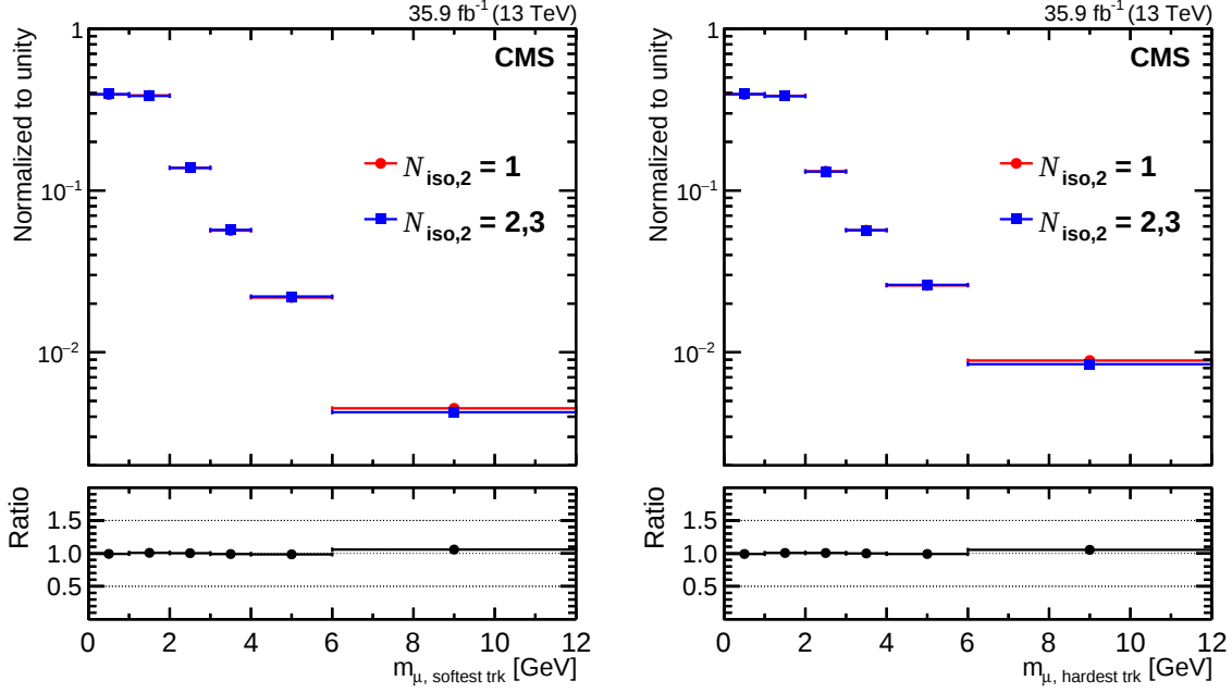
Figure 5.6: The observed normalized invariant mass distributions of the first muon and the softest (left) or hardest (right) “signal” track in control regions N_{\text{iso},2} = 1 (red circles) and N_{\text{iso},2} = 2, 3 (blue squares).
