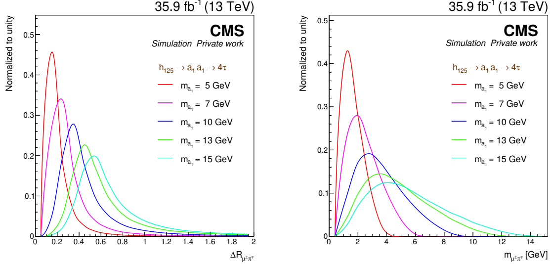
Figure 5.3: Distributions of \Delta R (left) and invariant mass m (right) of the muon-track pairs for different mass points of the h_{125} \rightarrow a_1 a_1 \rightarrow 4\tau channel in the ggF process. The distributions are obtained using generator-level information by selecting \mu^\pm\pi^\mp pairs that emerge from the a_1 \rightarrow \tau_\mu\tau_{\text{one-prong}} decay.
