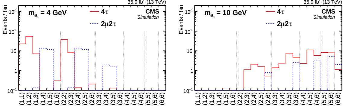
Figure 5.10: The unrolled f_{2D}(i, j) distribution of both signal channels 4\tau (red histogram) and 2\mu 2\tau (blue histogram) for two representative mass points m_{a_1} = 4 \text{ GeV} (left) and m_{a_1} = 10 \text{ GeV} (right). The notation of the bins follows that of Fig. 5.5.
