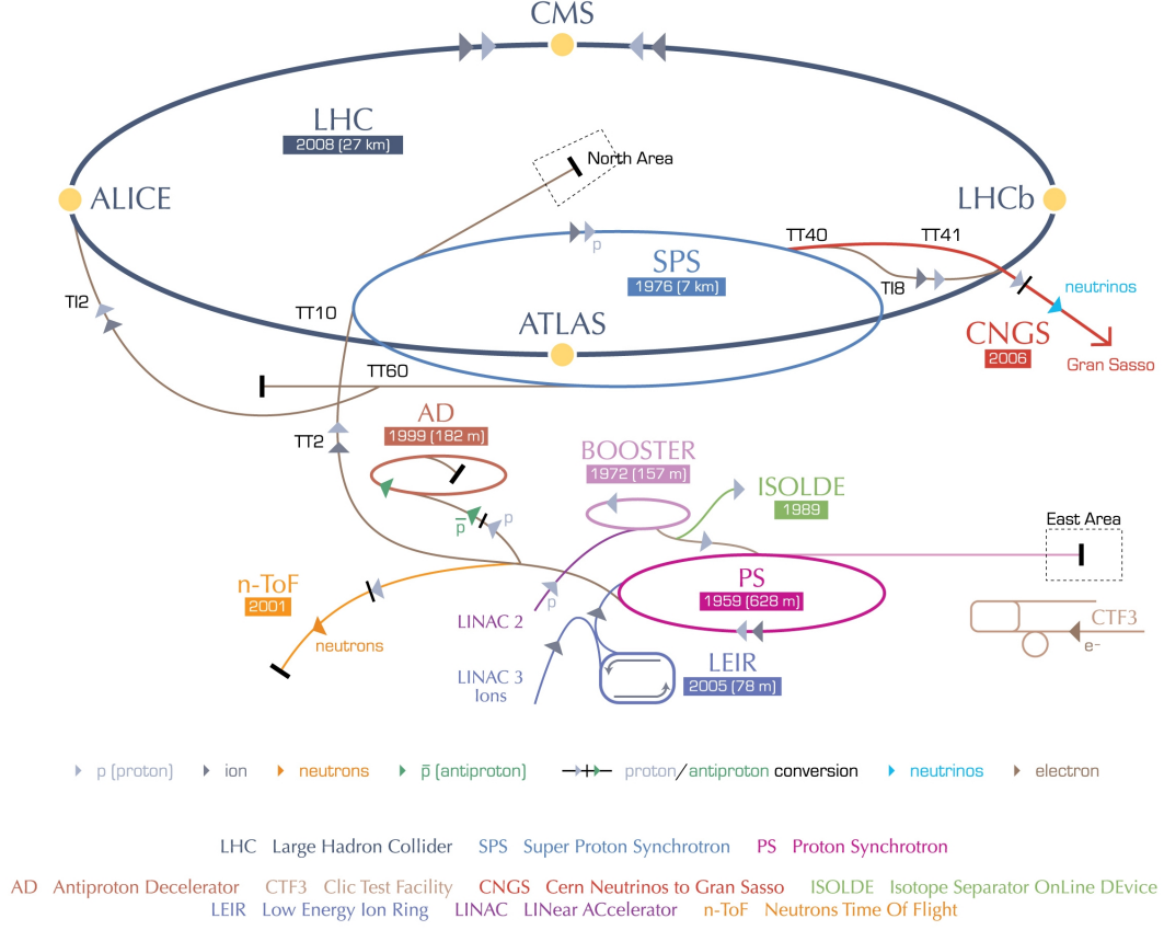
Figure 4.1: Accelerator complex at CERN [239]
