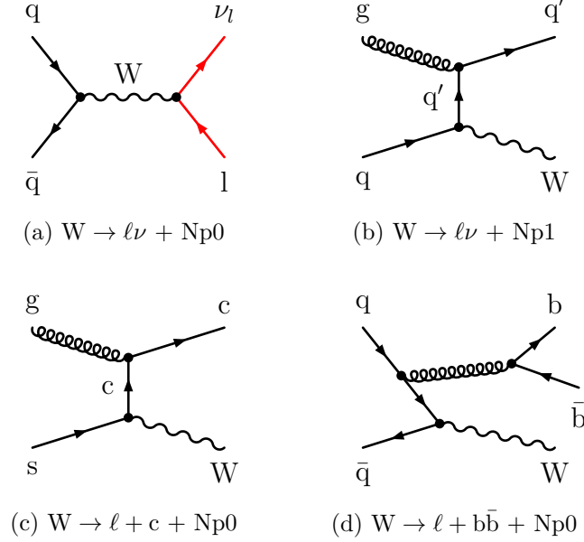
Figure 2.10.: Some exemplary W+Jets production modes. The production modes of a W boson with and without an additional light flavour parton are shown in (a) and (b). The production of a W boson in association with only one charmed quark without additional partons is shown in (c). In (d) the production of a b\bar{b} pair in the final states is shown.
