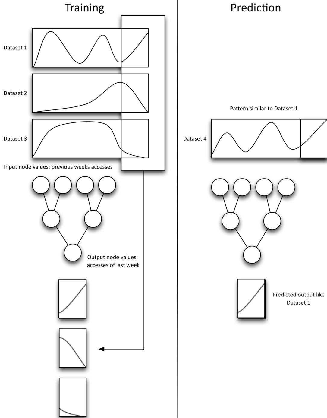
Figure 4.3: The ANN training and prediction.
