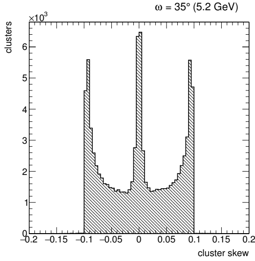
(c) Sickie and central part are of equal magnitude around \omega = 35^\circ
