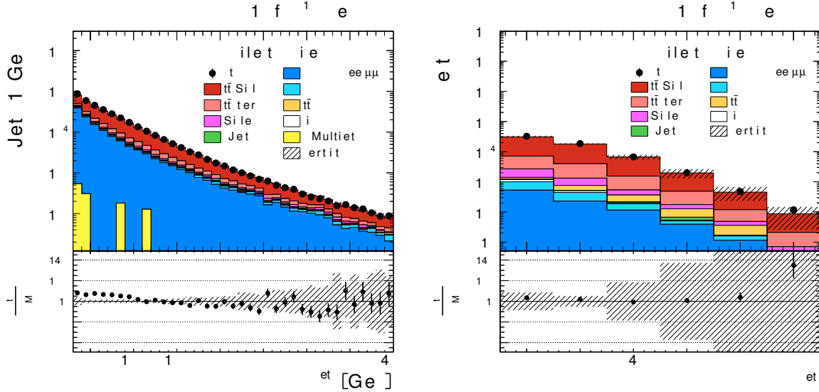
(a) Jet p_T distribution for events passing the lepton and jet selection criteria.
