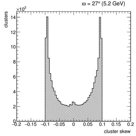
(b) Appearance of a central contribution around zero at \omega = 27^\circ
