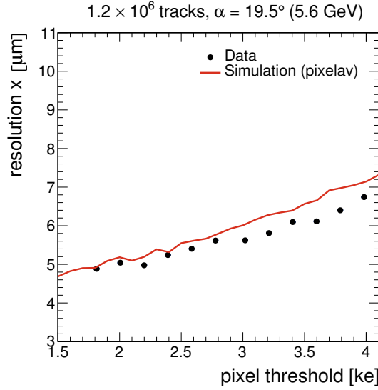
Figure 8.28: Spatial resolution as a function of the ROC pixel threshold, for a tilt angle of \alpha = 19.5^\circ . The resolution improves with lower thresholds as expected.
