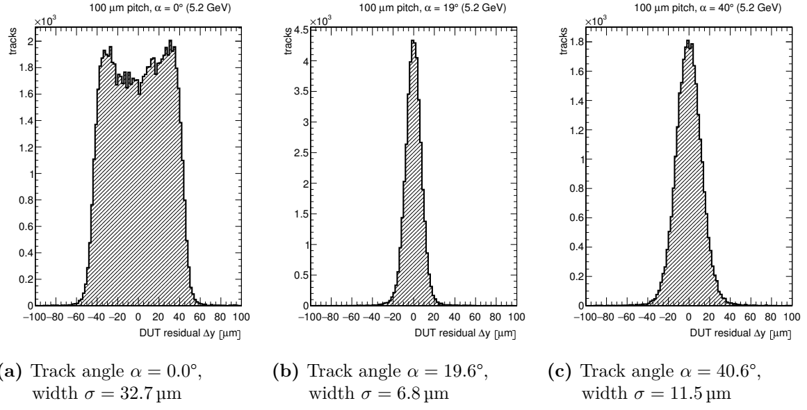
Figure 8.23: Sample residual distributions for SCM 504 along the 100 \mu\text{m} pitch side for different tilt angles \alpha . In addition, the residual width from a fit with the generalized error function is provided.
