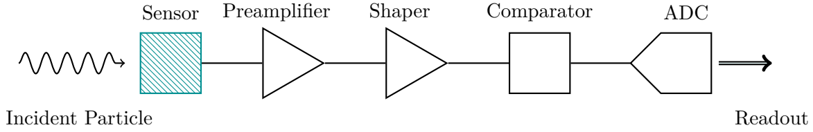
Figure 3.3: Typical building blocks of pixel front-end electronics. The incident particle induces a signal in the sensor, which is processed by the preamplifier and shaper. The comparator discriminates the signal before it is digitized by the ADC and read out. Modified from [98].
