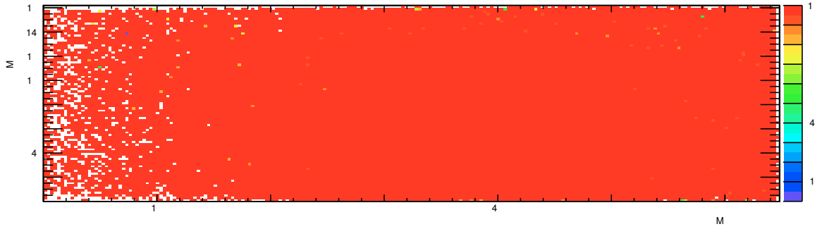
Figure D.7: Efficiency map of module C. The efficiency is above 99% except for the left part of the module where no tracks have been registered due to the size of the beam spot.
