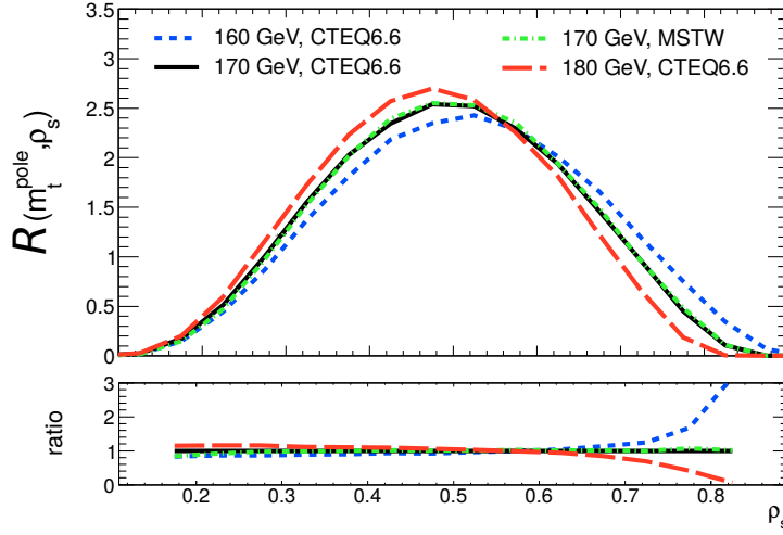
Figure 10.5: \mathcal{R} distribution as a function of \rho_S for different top quark pole masses. Shown are NLO accuracy calculations for m_t^{\text{pole}} = 160 GeV, 170 GeV, and 180 GeV. The lower plot shows the ratio with respect to a mass of m_t^{\text{pole}} = 170 GeV [12].
