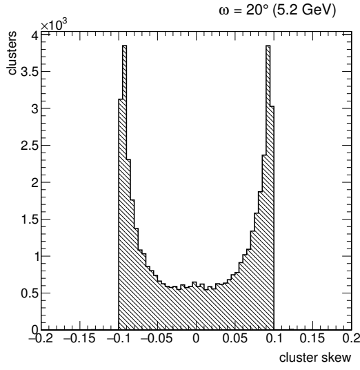
(a) Sickie shaped skewness distribution at small angles around \omega = 20^\circ
