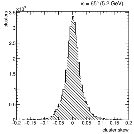
(d) Gaussian shape dominating the skewness for large angle \omega = 65^\circ
