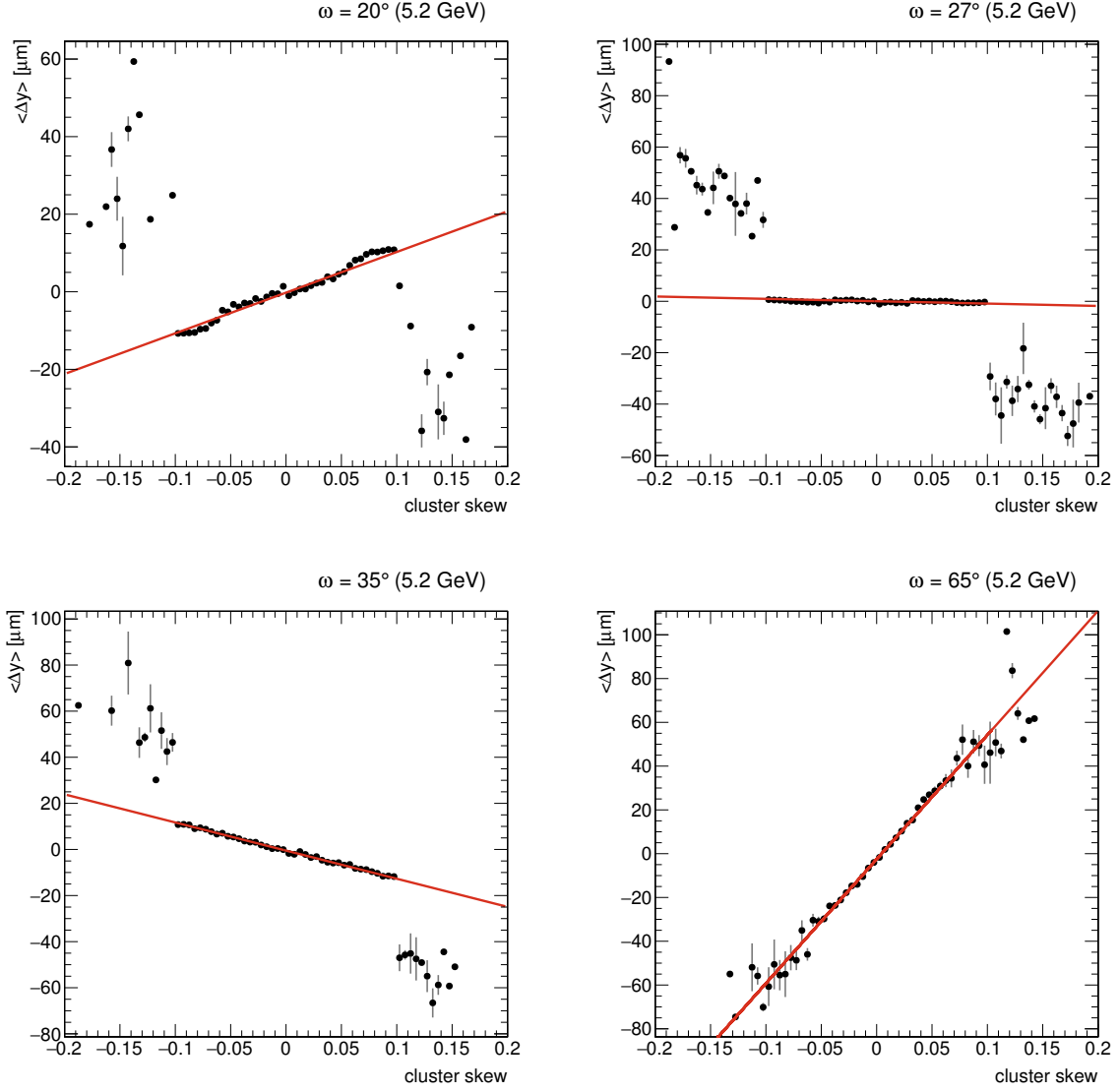
Figure 9.3: Residual mean position in y as function of the cluster skewness for different track incidence angles \omega . Shown is the distribution as obtained from data as well as a linear fit to the central part of the distribution with |\mu_3| \leq 0.1 .
