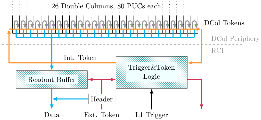
Figure 4.4: Mechanism of the internal and external ROC tokens. Pixels receiving a charge above threshold initiate the DCol readout token to store the pixel hits in the DCol periphery. The arriving L1 trigger releases the internal token which collects the data from the DCol buffers, and transmits them to the global readout buffer. Upon arrival of the external readout token, the ROC header is transmitted, followed by the pixel data.
