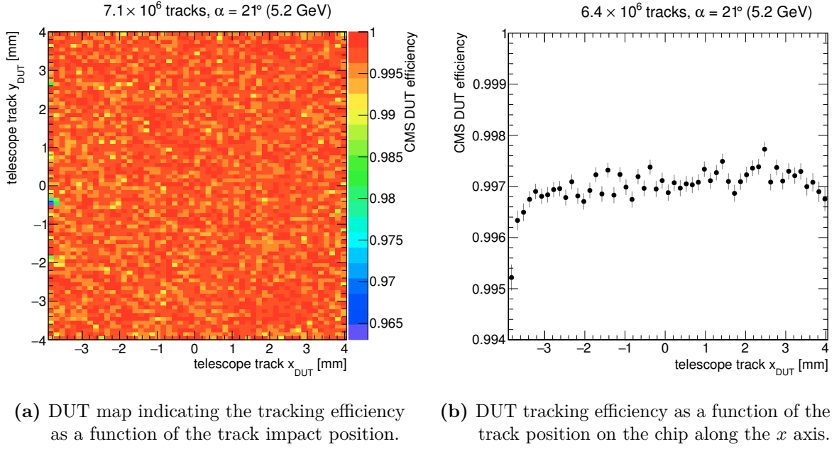
Figure 8.14: Tracking efficiency for the full fiducial volume of the DUT, shown as map (a) and as projection onto the track position along x (b). Both distributions show a uniform efficiency with minor effects from shifted pixel thresholds.
