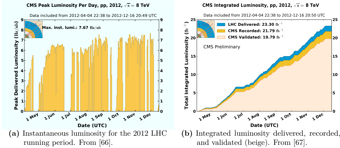
Figure 2.1: Evolution of the instantaneous (a) and integrated (b) luminosity. Blue denotes the luminosity delivered by the LHC while orange marks the luminosity recorded by the CMS experiment.
