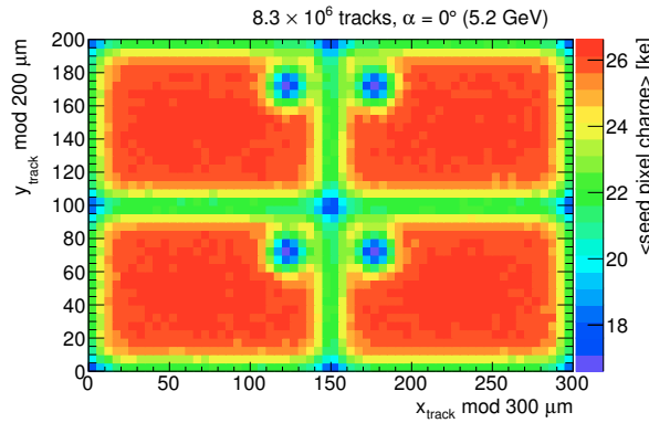
Figure 8.17: Mean charge of the cluster seed pixel as a function of the position within a 2 \times 2 pixel array. The implant regions can be distinguished from the p -spray isolation and the bias dots.
