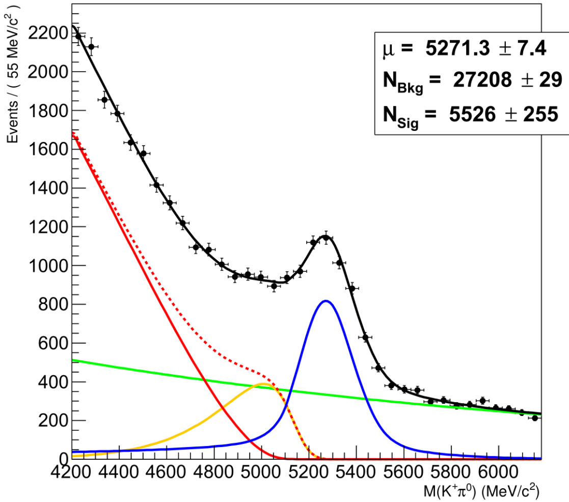
Figure 4.17: Mass distribution of the B^+ candidates, selected from the 2016 data set. The data are drawn as black points. The total fit model is drawn as a solid black line. The signal component is drawn in blue, the combinatorial background is drawn in green, and the partially reconstructed backgrounds are drawn together in dashed red. The component representing partially reconstructed backgrounds where only one decay product is not reconstructed is drawn in yellow, while that representing cases where two or more decay products are not reconstructed is drawn in red.
