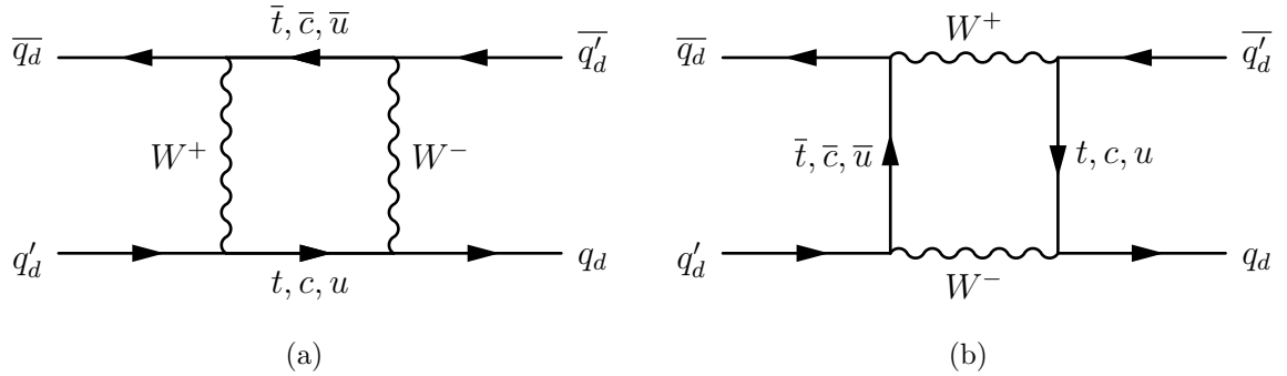
Figure 2.2: The lowest-order box diagrams for the K^0/\bar{K}^0 , B^0/\bar{B}^0 , and B_s^0/\bar{B}_s^0 mesons, where q_d is a down-type quark and q_d' is a distinct down-type quark. The corresponding diagrams for the D^0/\bar{D}^0 mesons can be produced by the substitutions q_b \rightarrow c , q_b' \rightarrow u , and (t, c, u) \rightarrow (b, s, d) .
