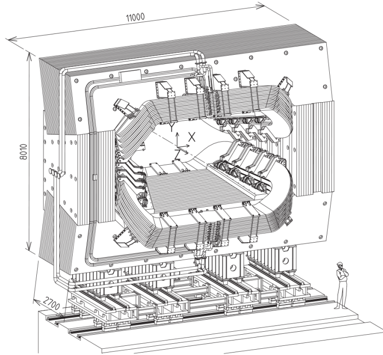
Figure 3.6: Perspective view of the magnet from downstream; the VELO is behind the magnet in this view.
