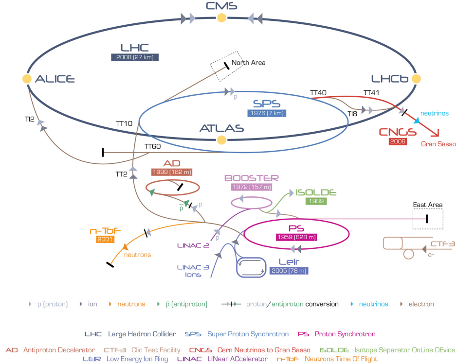
Figure 2.2: Scheme representing the CERN accelerator complex.
