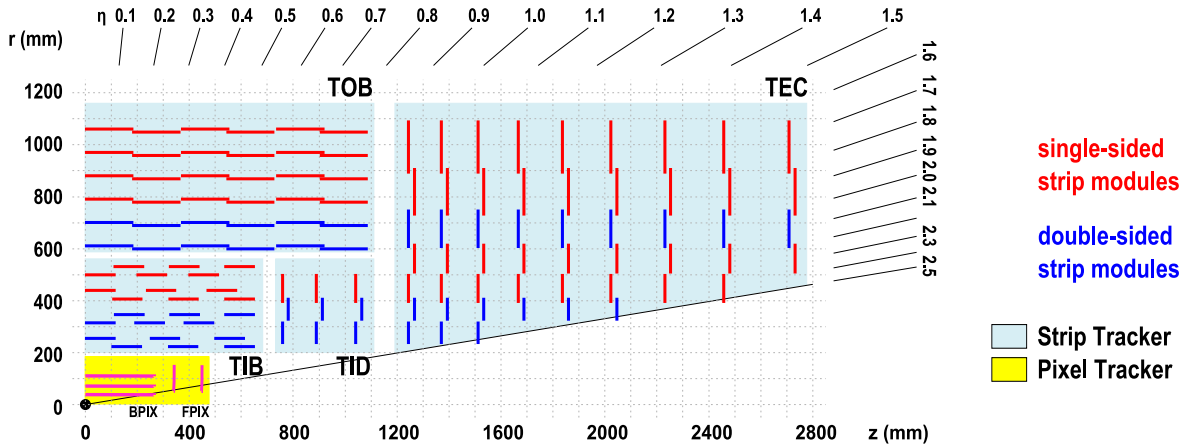
Figure 2.6: Layout of the CMS silicon tracker showing the relative position of hybrid pixels, single-sided strips and double-sided strips. Figure from [46].
