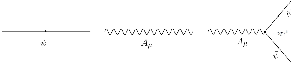
Figure 1.1: Feynman diagrams describing the particles (left), the propagators (middle) and the interaction vertex (right). \psi represents the matter fields and A_\mu the gauge fields.
