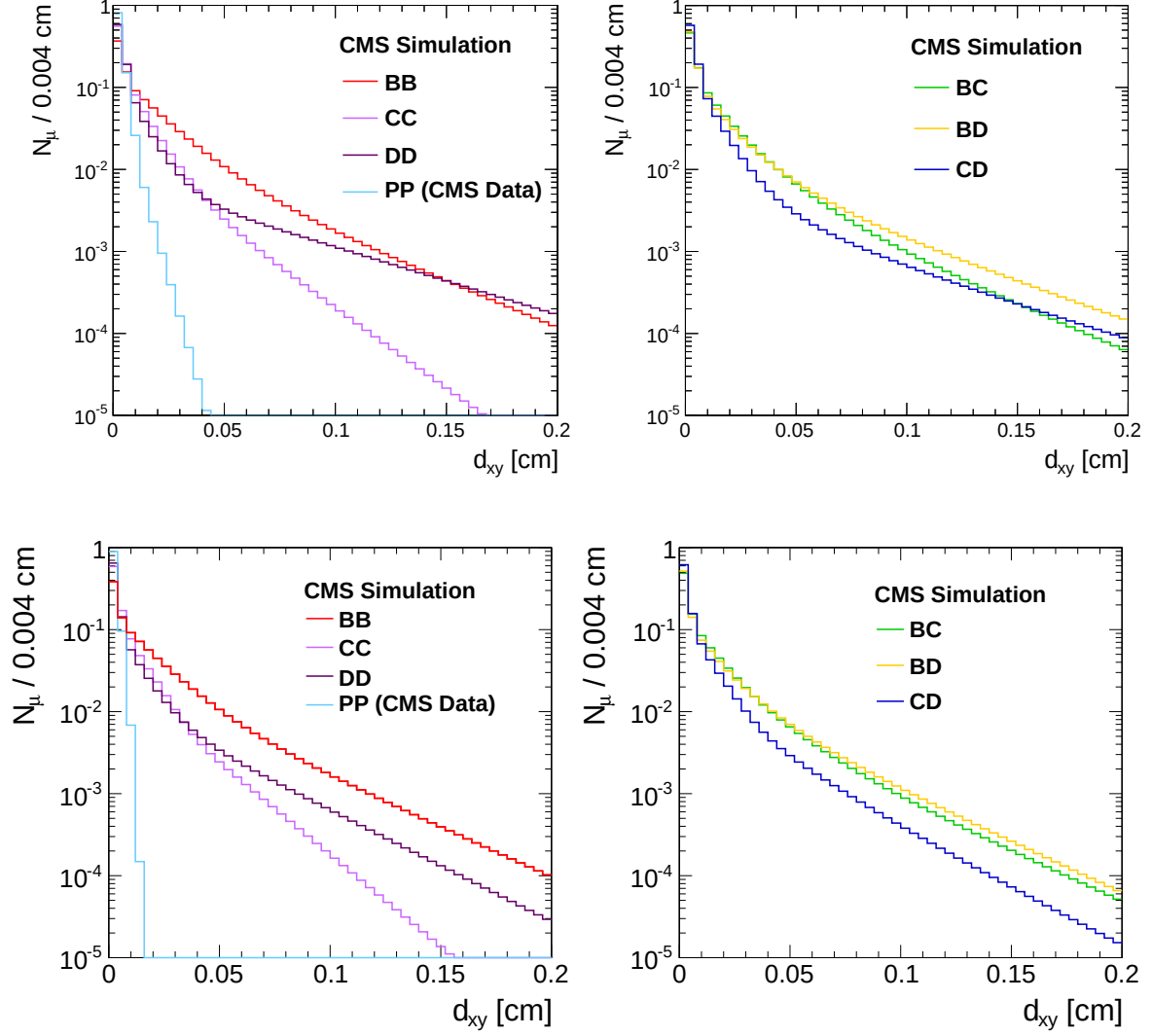
Figure 5.10: The 1D projections of the seven templates used in the analysis for muons with p_T > 4 GeV (top row) and p_T > 6 GeV (bottom row), for the diagonal components (BB, CC, PP, DD) on the left, and for the off-diagonal ones (BC, BD, CD) on the right.
