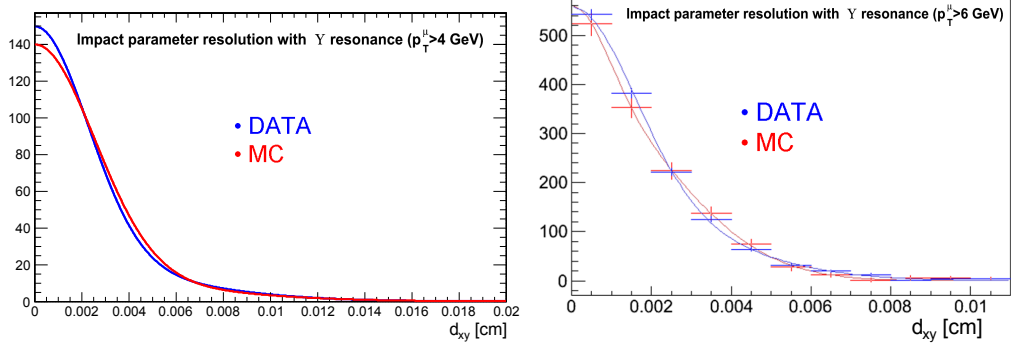
Figure 5.6: Comparison of the fit results in MC (RED) and data (BLUE). Both curves are renormalized to the same integral. Left: muons with p_T^\mu > 4 GeV, right: muons with p_T^\mu > 6 GeV.
