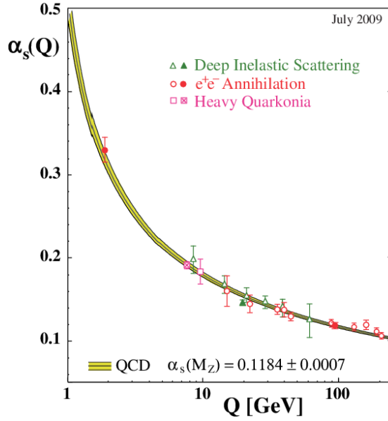
Figure 3.1: Summary of measurements of \alpha_s as a function of the respective energy scale [84].
