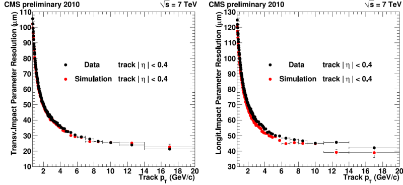
Figure 2.18: The measured resolution of the track transverse (left) and longitudinal (right) impact parameter as a function of track p_T . Figures from [66].
