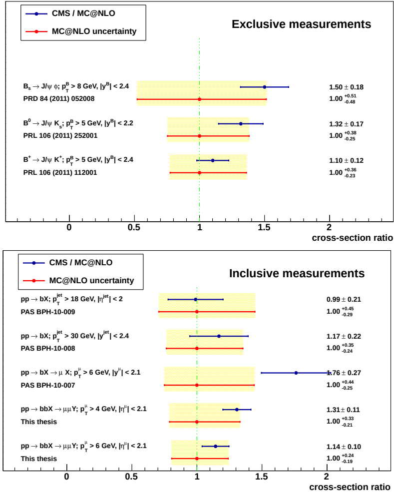
Figure 7.2: Summary of b -quark production cross section measurements performed within the CMS experiment. The ratio with respect to the MC@NLO prediction is shown, together with the total uncertainty. Top: exclusive measurements. Bottom: inclusive measurements.
