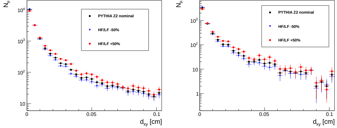
Figure 6.2: Direct comparison of D templates obtained by varying the heavy flavor content compared to the nominal simulation, in the range [0, 0.1] cm, for muons with p_T > 4 GeV (left) and p_T > 6 GeV (right). The distributions are normalized to the same area.
