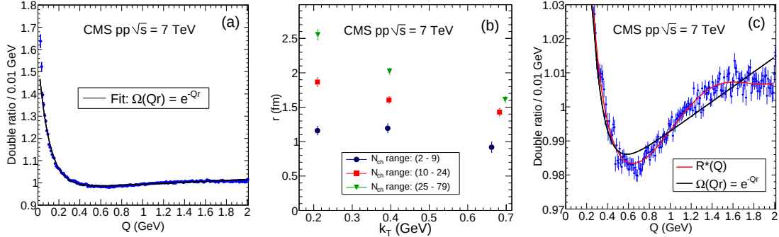
Figure 2.24: Data points for the double ratio are shown in (a), together with the fit given by the exponential parameterization in Eq. 2.6. Part (b) shows the behavior of the r parameter obtained with this \Omega(Qr) = e^{-Qr} form as a function of k_T for three bins in N_{\text{ch}} . The plot in (c) shows the anticorrelation structure in the double ratio [note the zoomed ordinate axis with respect to the plot of part (a)]. The uncertainties in the plots are statistical only. Figures from [78].
