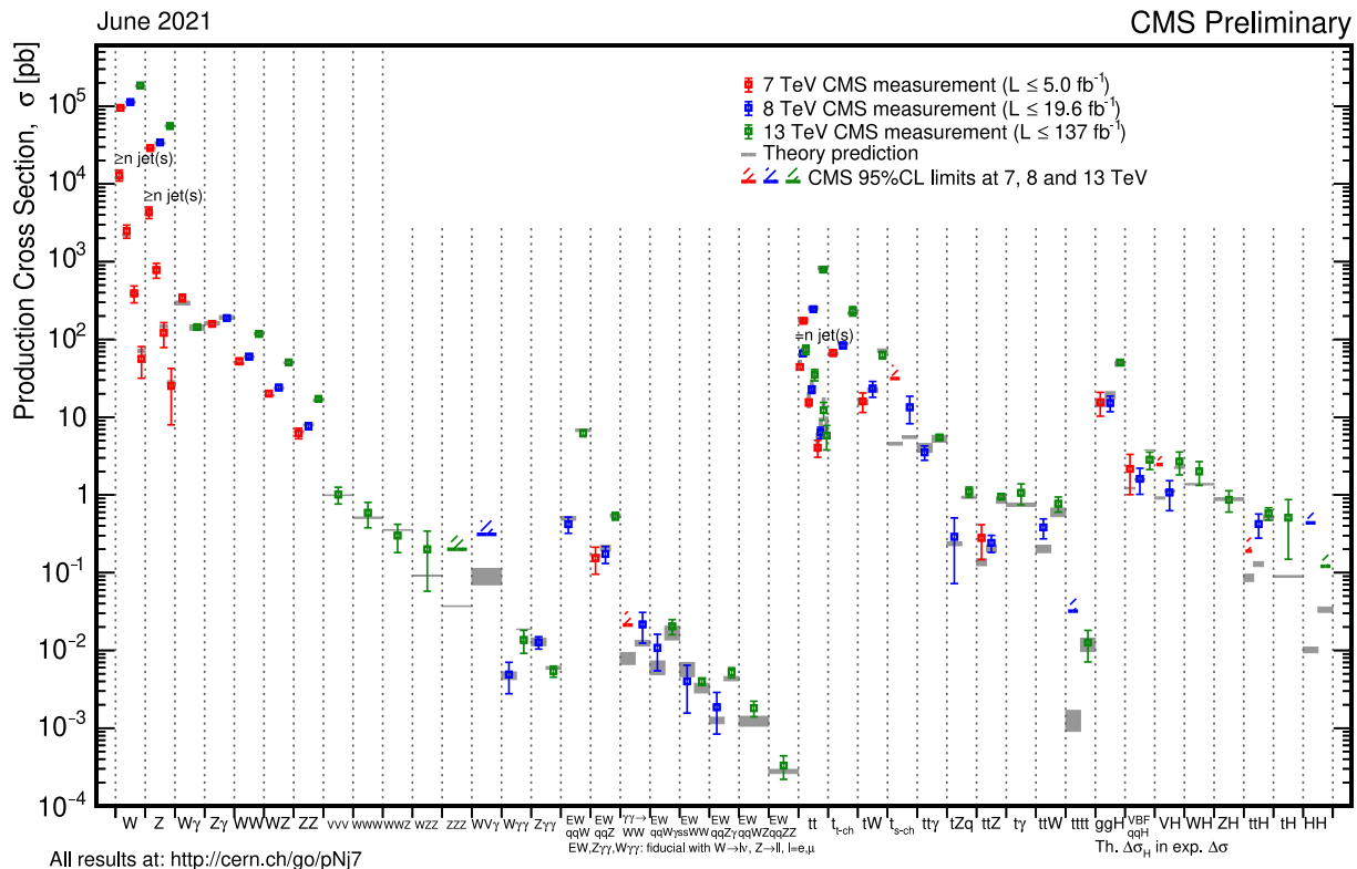
Figure 2.8: Predicted and observed cross sections at different center-of-mass energies for various SM processes with the CMS experiment. The measurements are in agreement with the SM for cross sections spanning over nine orders of magnitude. Figure adapted from Ref. [164].
