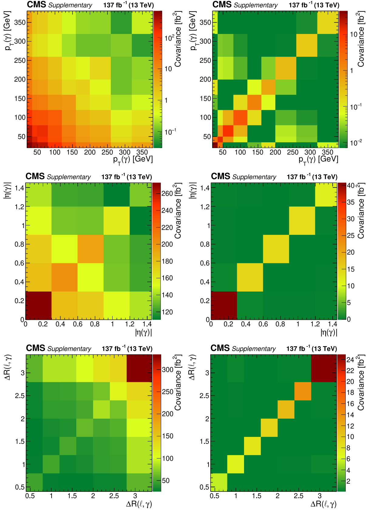
Figure A.5: The covariance matrices of the systematic (left) and statistical (right) uncertainties for p_T(\gamma) (upper), |\eta(\gamma)| (center), and \Delta R(\ell, \gamma) (lower) in the fiducial phase space defined at the particle level.
