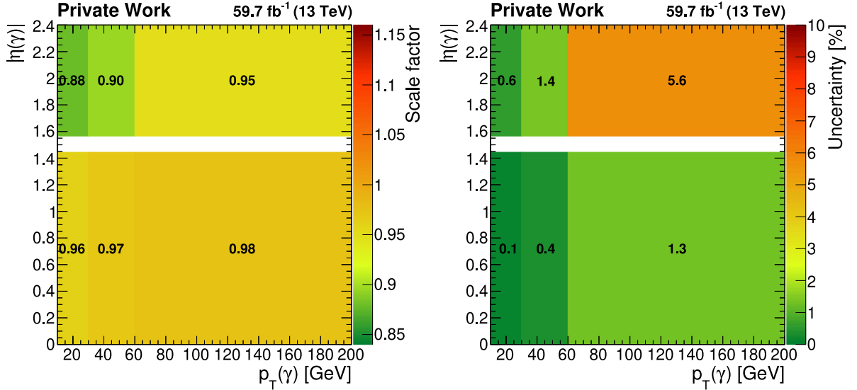
Figure 4.5: Pixel-seed veto SFs (left) and uncertainties (right) of the measurement in the 2018 data-taking period.
