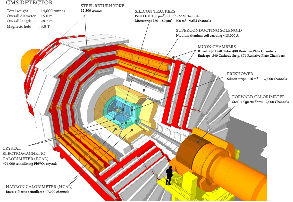
Figure 3.5: Illustration of the CMS detector and its subdetectors. The tracker is the closest subdetector to the IP, surrounded by the electromagnetic and hadronic calorimeters, a superconducting magnet, and the muon chambers. Figure taken from Ref. [232].
