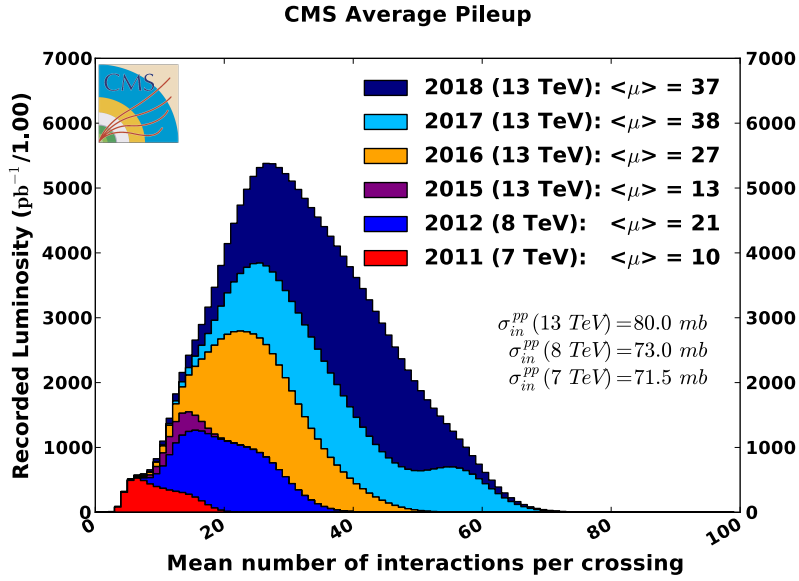
Figure 3.2: Distributions of average numbers of interactions per bunch crossing in pp collisions measured by the CMS experiment at the LHC. The distributions are overlayed for the data-taking periods of 2011 (red), 2012 (blue), 2015 (purple), 2016 (orange), 2017 (light blue), and 2018 (dark blue), with an average number of 10, 21, 13, 27, 38, and 37 simultaneous collisions, respectively. Figure taken from Ref. [223].
