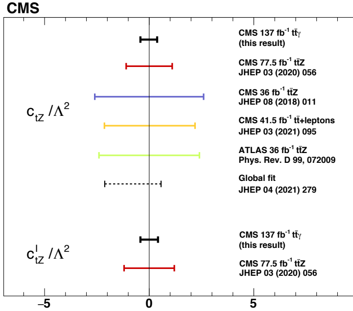
Figure 5.8: Comparison of observed 95 % CL intervals of the Wilson coefficients c_{tZ} and c_{tZ}^I from the presented measurement (black), previous results of the CMS collaboration from inclusive [297] (blue) and differential [135] (red) t\bar{t}Z measurements, from t\bar{t} measurements with additional leptons [294] (yellow), results from the ATLAS collaboration [298] (green) and global SM-EFT fits [299] (dashed).
