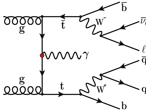
Figure 5.1: Representative diagram of the t\bar{t}\gamma process for a photon originating from the top quark with a modified top quark-photon coupling indicated by a red circle.
