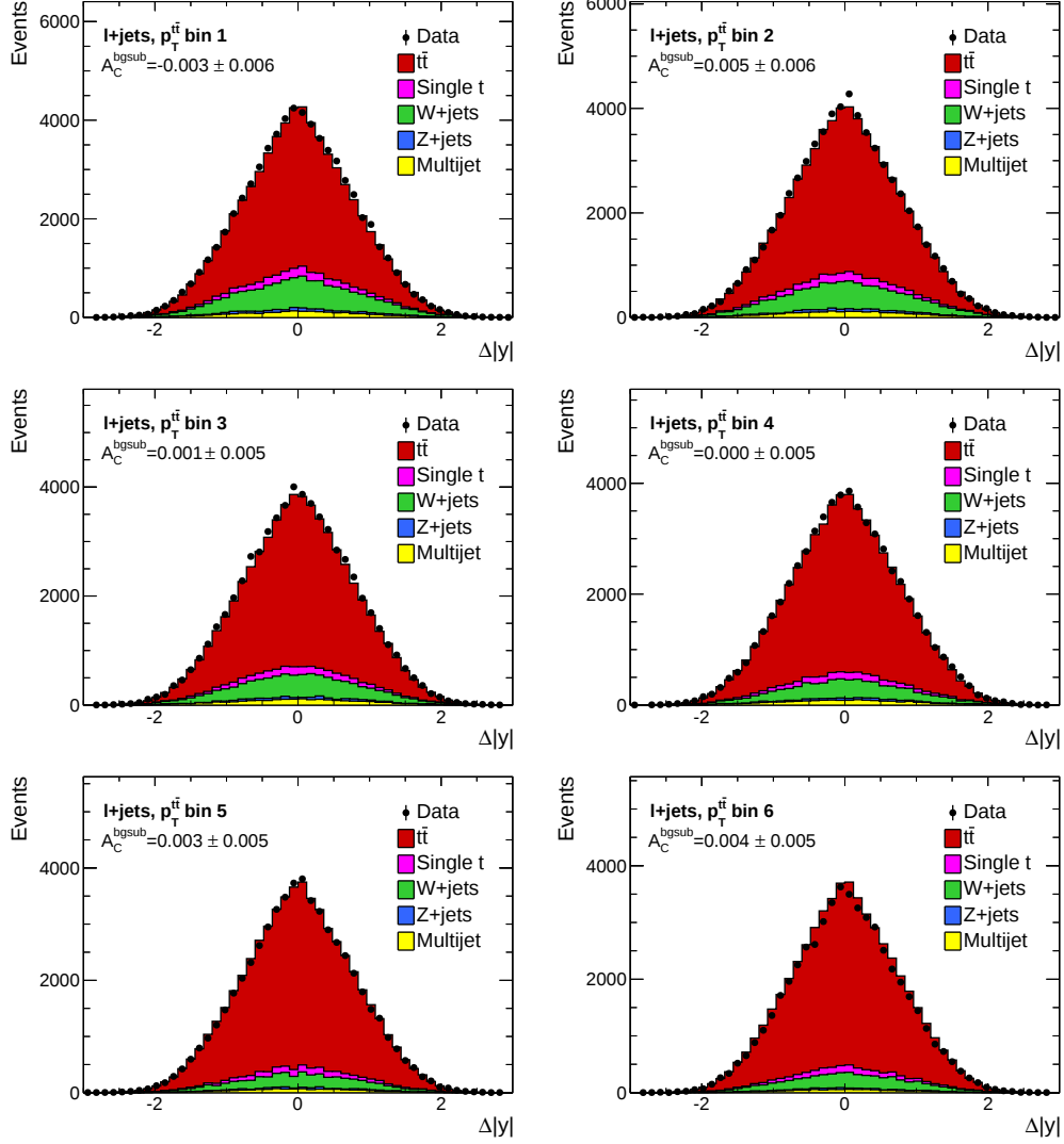
Figure 5.10: Reconstructed distributions of \Delta|y| in six bins of the reconstructed p_T^{t\bar{t}} . The background-subtracted asymmetry A_C^{bgsb} is shown for each bin. The simulation is normalized to the fit results.
