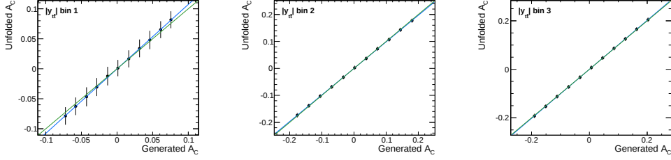
Figure E.9: Linearity test: Mean of unfolded A_C in the fiducial phase space as a function of the true simulated value in three bins of |y_{tt}| . The error bars indicate the statistical uncertainty of a single measurement. The result of a linear regression is drawn in blue, whereas the bisector is shown in green.
