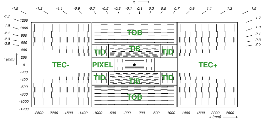
Figure 2.5: Schematic overview of the longitudinal structure of the CMS tracking system [72]. The interaction point is indicated as a black dot in the center. It is surrounded by silicon pixel detectors on the inside and silicon strip detectors on the outside. The barrel part consists of the Tracker Inner Barrel (TIB) and the Tracker Outer Barrel (TOB), whereas the endcap discs are made up of the Tracker Inner Discs (TID) and the Tracker End Caps (TEC). While single lines indicate normal detector modules, each double line represents a stereo module.
