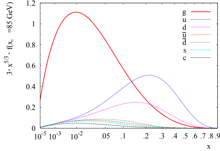
Figure 1.1: The CT10 PDF set [32] for protons, evaluated at a scale of \mu = 85 GeV; adapted from reference [33]. The variable x denotes the Bjorken scale variable, i.e. the momentum fraction of the given particle relative to the proton.
