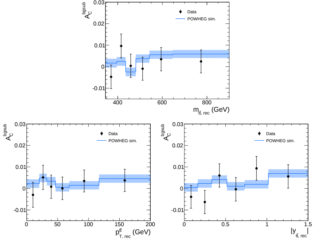
Figure 5.8: Results of the three differential measurements of the background-subtracted charge asymmetry in the three secondary variables m_{\text{tt}, \text{rec}} , p_{\text{T}, \text{rec}}^{\text{tt}} and |y_{\text{tt}, \text{rec}}| . The measurement is compared to the reconstructed asymmetries observed in the simulated POWHEG signal sample. All error bars correspond to statistical uncertainties.
