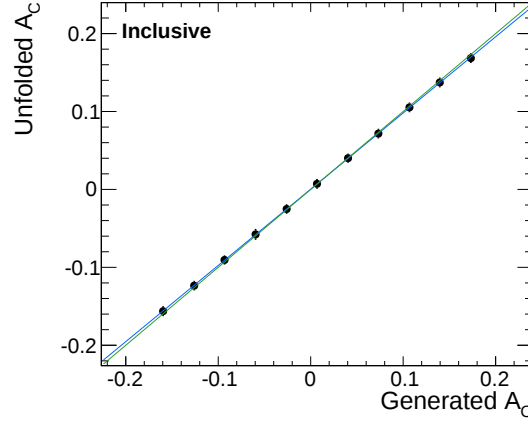
Figure 5.28: Linearity test: Mean of unfolded A_C in the full phase space as a function of the true simulated value. The error bars indicate the statistical uncertainty of a single measurement. The result of a linear regression is drawn in blue, whereas the bisector is shown in green.
