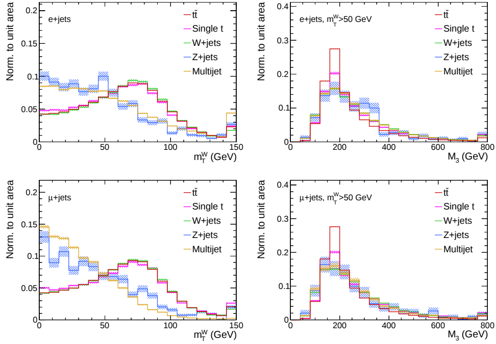
Figure 4.6: Shape comparisons of the m_T^W and M_3 distributions for the processes involved in the background estimation. The electron+jet channel is shown in the upper row, whereas the corresponding distributions for the muon+jet channel are shown in the lower row. The distributions of M_3 have been derived from events with m_T^W \geq 50 GeV. The full m_T^W distribution is shown, even though only bins with m_T^W < 50 GeV enter the background estimation.
