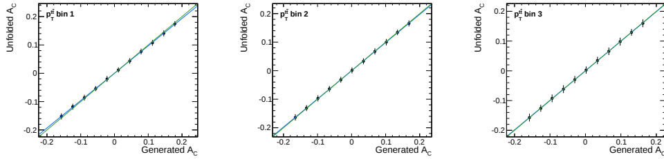
Figure E.3: Linearity test: Mean of unfolded A_C in the full phase space as a function of the true simulated value in three bins of p_T^{t\bar{t}} . The error bars indicate the statistical uncertainty of a single measurement. The result of a linear regression is drawn in blue, whereas the bisector is shown in green.
