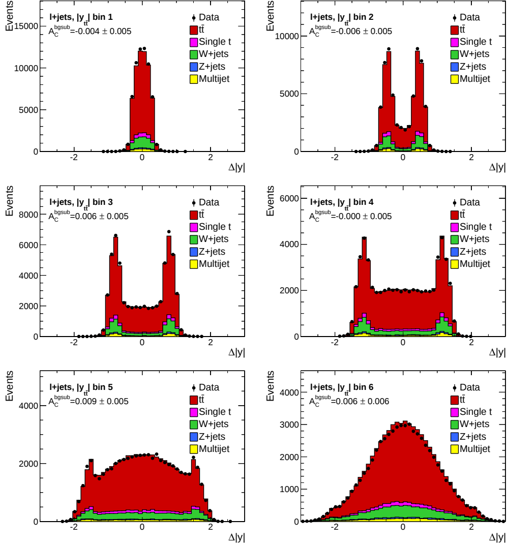
Figure 5.11: Reconstructed distributions of \Delta|y| in six bins of the reconstructed |y_{t\bar{t}}| . The background-subtracted asymmetry A_C^{bgs} is shown for each bin. The simulation is normalized to the fit results.
