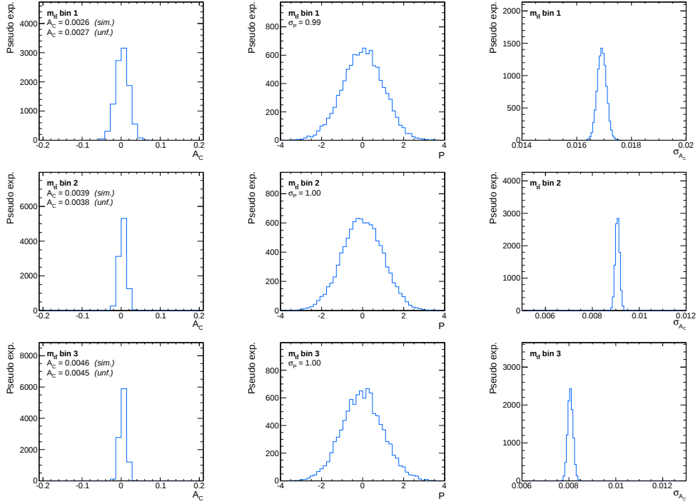
Figure D.7: Distribution of the measured asymmetries (left), the pull distributions (middle), and the distributions of the statistical uncertainties (right) of pseudo experiments corresponding to the differential measurement in three bins of m_{t\bar{t}} in the fiducial phase space . \sigma_P signifies the standard deviation of the pull distribution.
