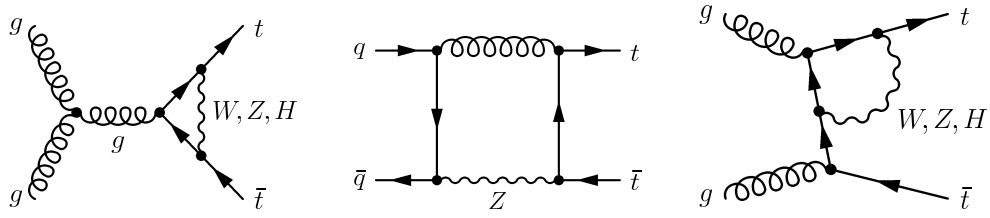
Figure 1.6: Example Feynman diagrams for the electroweak corrections to t\bar{t} production.
