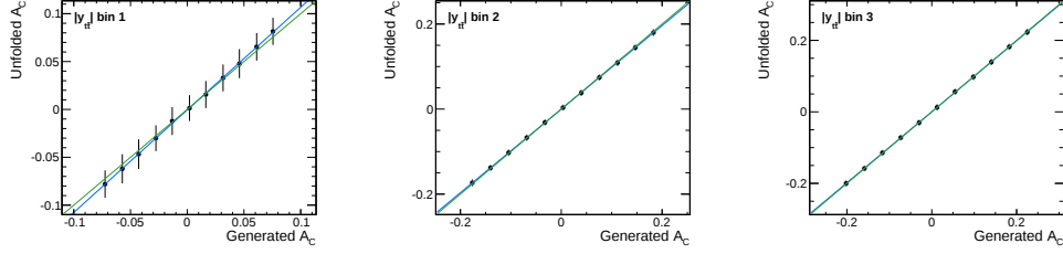
Figure E.4: Linearity test: Mean of unfolded A_C in the full phase space as a function of the true simulated value in three bins of |y_{t\bar{t}}| . The error bars indicate the statistical uncertainty of a single measurement. The result of a linear regression is drawn in blue, whereas the bisector is shown in green.
