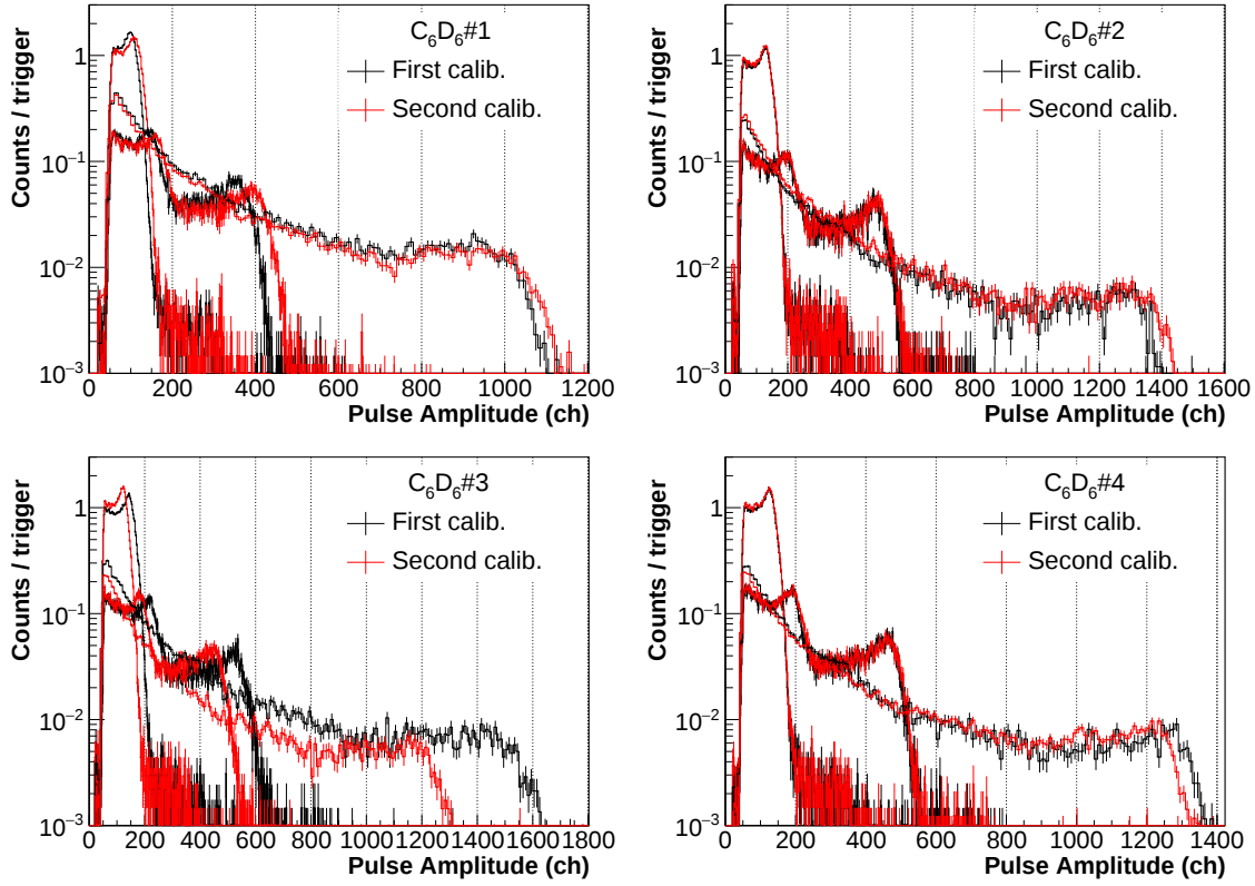
Figure 6.2: Deposited energy spectra of the three calibration sources employed in the two full calibrations of the ^{203}\text{Tl}(\text{n},\gamma) measurement in the four \text{C}_6\text{D}_6 detectors.
