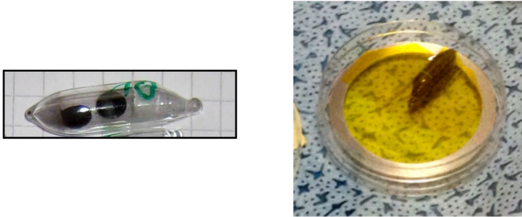
Figure 7.1: Left: The \text{Tl}_2\text{O}_3 pellet had already broken in two pieces before the irradiation in the neutron reactor. Right: The sample after irradiation, already fixed on the aluminium ring by means of kapton foils. The inner walls of the capsule had totally blackened.
