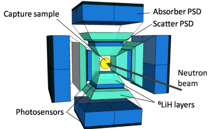
Figure 2.2: Left: Diagram showing the concept of a 4\pi i -TED detector, surrounding a cylindrical sample in the centre. The several assemblies of scatterer and absorber allow to use Compton imaging techniques to reconstruct the emission point of the gamma rays detected, which enables to discriminate between true capture gamma rays arising from the sample and background gamma rays coming the surroundings. Extracted from [62].
