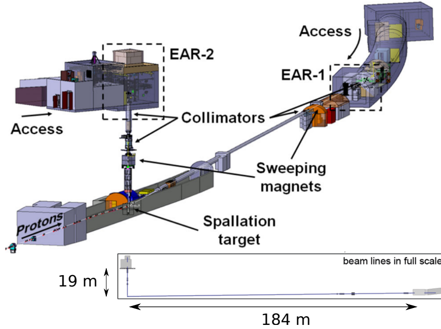
Figure 3.2: Layout of the n_TOF facility, showing its two beam lines and the position of several other beam elements. A full scale profile view of both experimental areas is also shown (Extracted from [71] and [72], respectively.)
