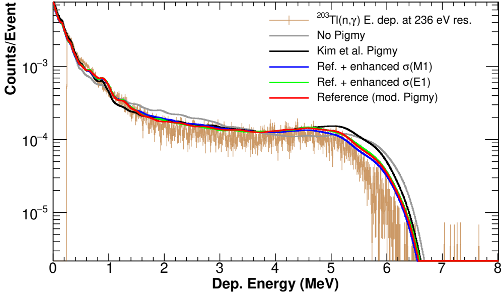
Figure 6.7: Comparison, for \text{C}_6\text{D}_6\#4 , between the experimental capture spectrum for the resonance at 236 eV (light brown) and the simulated response function to several cascade models, described more in detail in the text.
