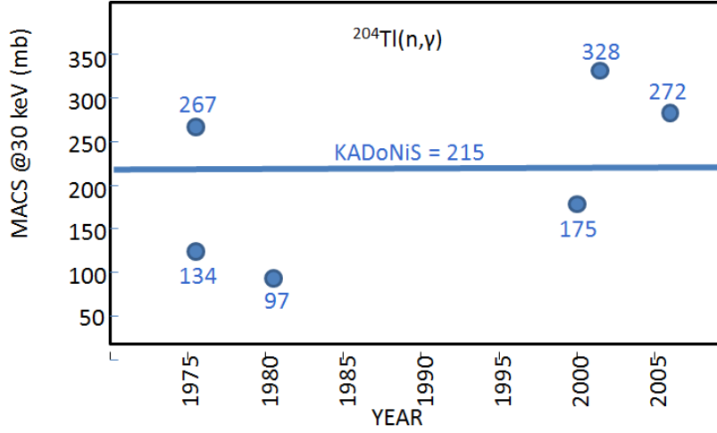
Figure 1.5: The different theoretical evaluations of the ^{204}\text{Tl}(n, \gamma) MACS at kT = 30 \text{ keV} , compared to the recommended value by the KADoNiS database [39]. Figure from [34].
