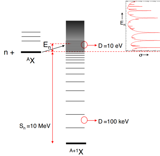
Figure 1.6: Schematic view of the formation of the compound nucleus after the capture of a neutron by the nuclide {}^A\text{X} . The excited levels beyond the neutron separation energy correspond to resonant states of the compound nucleus, which in capture experiments are observed as cross section resonances. Extracted from [49].
