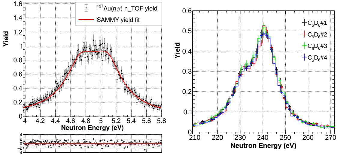
Figure 6.8: Left: for each detector, the normalization constant A_n is obtained by fitting the 4.9 eV resonance of gold. Right: the normalized yield for all detectors, in the 236 eV resonance of ^{203}\text{Tl} .
