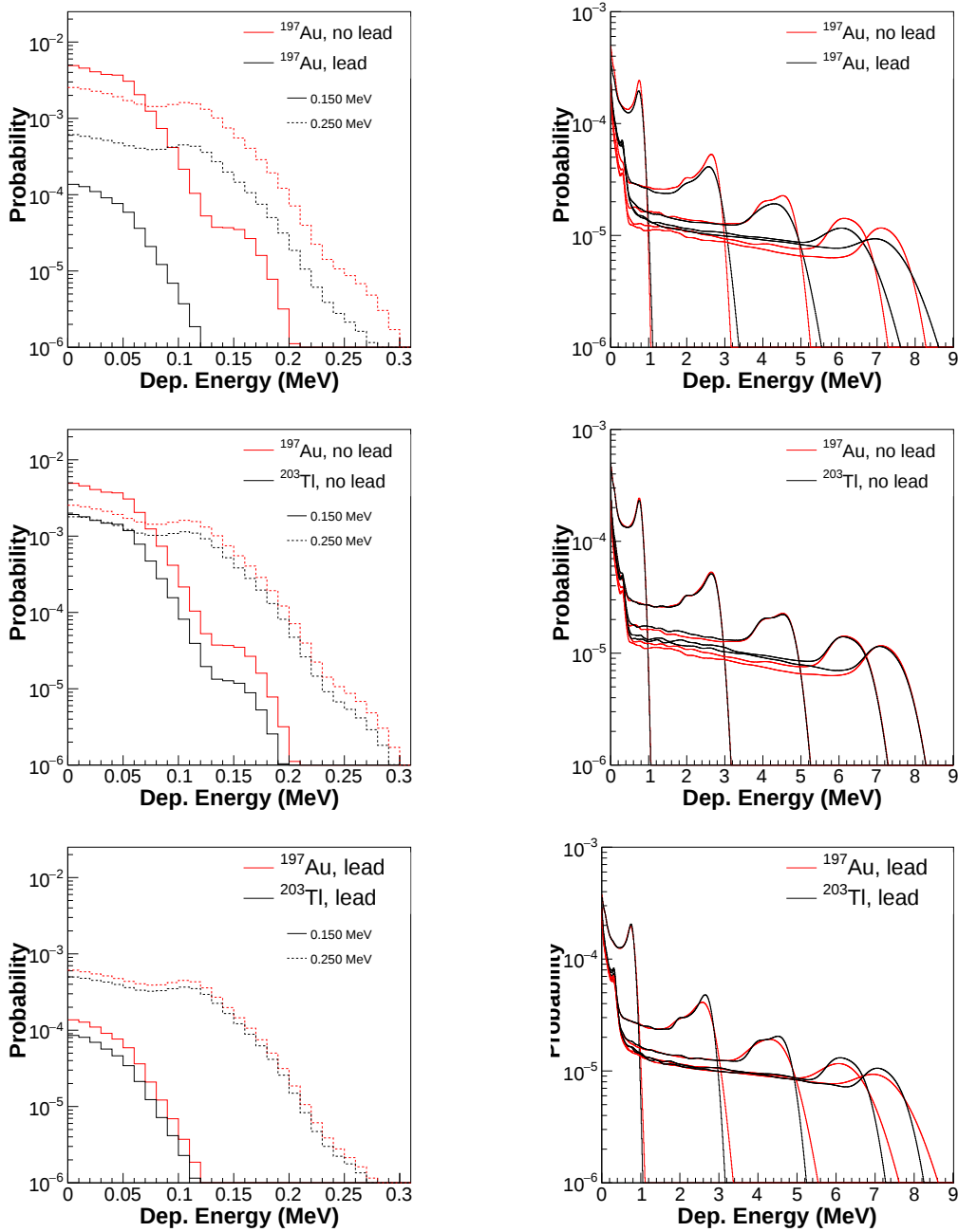
Figure 5.2: Comparison of the RF of \text{C}_6\text{D}_6\#1 to the \gamma -rays emitted by the ^{197}\text{Au} sample with and without lead foils (top plots), ^{197}\text{Au} and ^{203}\text{Tl} without the foils, and ^{197}\text{Au} and ^{203}\text{Tl} with them. The \gamma -rays shown are those with emitted energies of 0.15 and 0.25 MeV (left plots) and 1, 3, 5, 7 and 8 MeV (right plots)
