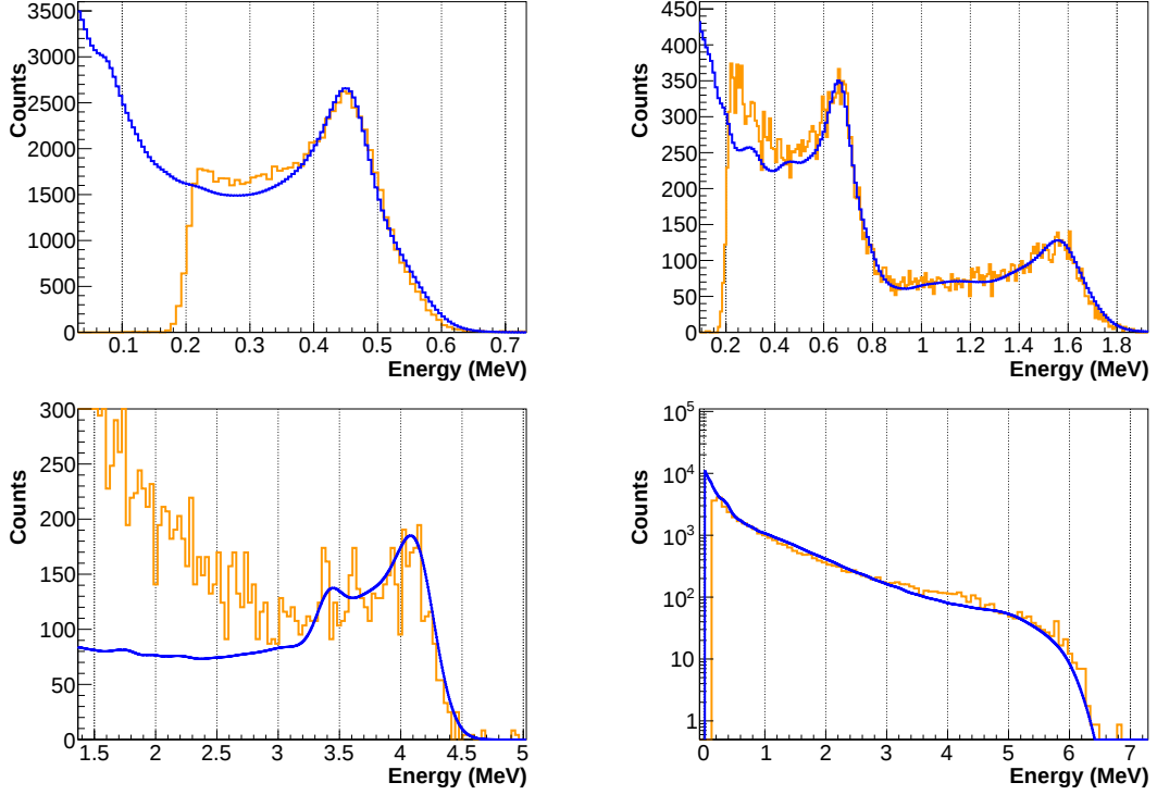
Figure 4.1: Experimental (orange) versus simulated (blue) energy deposited spectra in C_6D_6\#4 , for the July 14 calibrations. The sources are the ^{137}Cs gamma ray at 662 keV (top left), the two gamma rays of ^{88}Y at 1836 and 898 keV (top right), the Am-Be (bottom left), and the deposited energy spectrum at the 4.9 eV ^{197}Au(n, \gamma) resonance, with S_n = 6.512 MeV.
