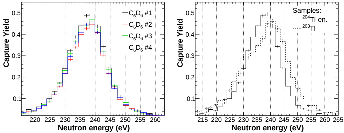
Figure 7.14: Left: Capture yield of the four \text{C}_6\text{D}_6 detectors for the ^{204}\text{Tl} -enriched sample data, in the 236 eV ^{203}\text{Tl} resonance. All the correction factors obtained ^{203}\text{Tl}(n,\gamma) analysis, with a threshold of 600 keV. The histograms have been rebinned to 600 bins per decade to reduce the statistical fluctuation. Right: Comparison of the yield of the ^{203}\text{Tl} sample and the ^{204}\text{Tl} -enriched in the 236 eV resonance, for \text{C}_6\text{D}_6\#1 .
