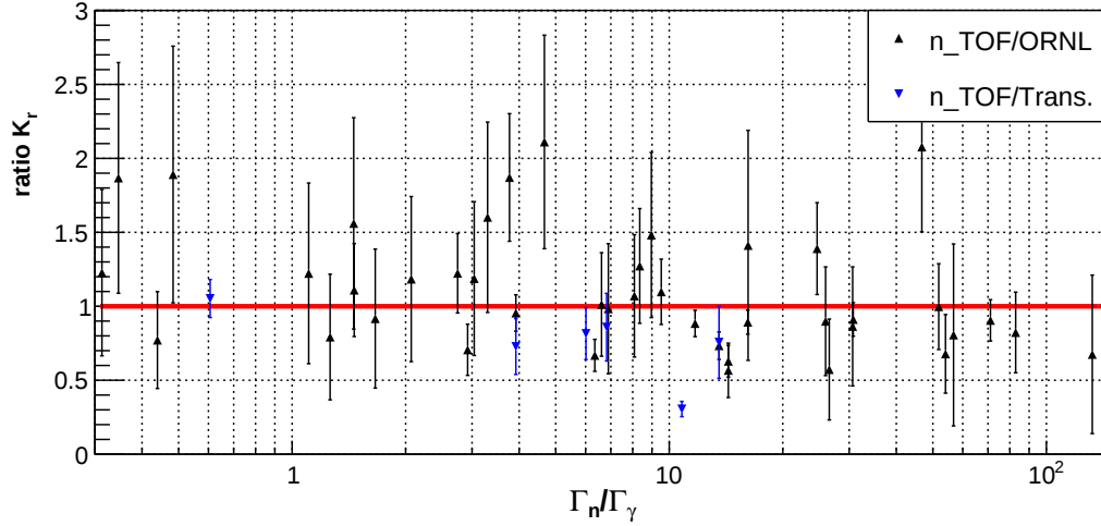
Figure 6.20: Ratio of n -TOF resonance kernels compared to previous experiments as a function of \Gamma_n/\Gamma_\gamma
