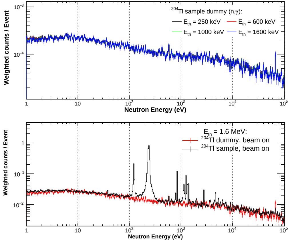
Figure 7.9: Top: Neutron energy distribution of the ^{204}\text{Tl} sample dummy signals, for different values of the deposited energy threshold. The spectra have been normalized to the counting rate in the 5 eV to 30 eV range. Bottom: The ^{204}\text{Tl} sample and the ^{204}\text{Tl} dummy neutron energy spectra, with E_{th} = 1.6 MeV. Both measured with \text{C}_6\text{D}_6\#1 .
