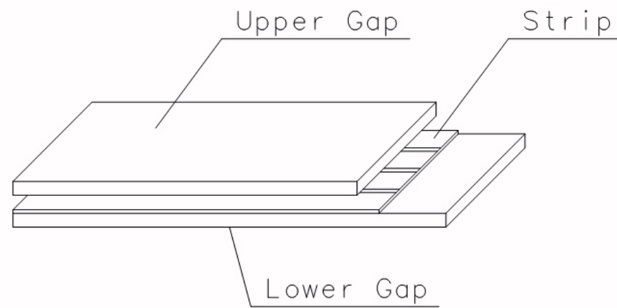
Figure 4.16: Structure of a two-gap RPC module installed in the muon system of CMS. The resistive plate in-between two gaps is visible [166].
