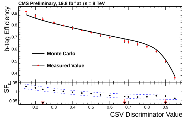
Figure 6.4: B tagging efficiency as function of the CSV discriminator variable shown for Monte Carlo simulation and data in t\bar{t} events. The arrows on the x-axis indicate the three working points (from left to right) – "Loose", "Medium" and "Tight". The lower panel shows the scaling factor between data and simulation [224].
