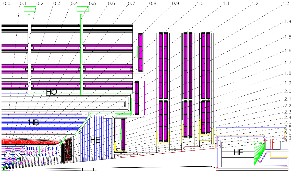
Figure 4.8: A schematic drawing of the hadron calorimeter of CMS – HB stands for the hadron barrel region, HE denotes the hadron endcap region, hadron outer detector is labeled by HO and finally HF marks the hadron forward calorimeter. The dashed lines denote fixed pseudorapidity values. Also the muon detection system is visible [166].
