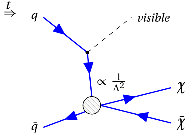
Figure 3.8: Collider production of dark matter in an effective field theory. The approximated vertex is indicated by a hatched circle. In this approach, dark matter particles \chi and \bar{\chi} couple to a pair of quarks exchanging a heavy mediator in the approximated vertex along the production of a visible particle (e.g. Z boson). Two parameters are of interest – the mass of the dark matter particle m_\chi along the coupling strength of dark matter to quarks which is parametrized in terms of the cutoff scale \Lambda .
