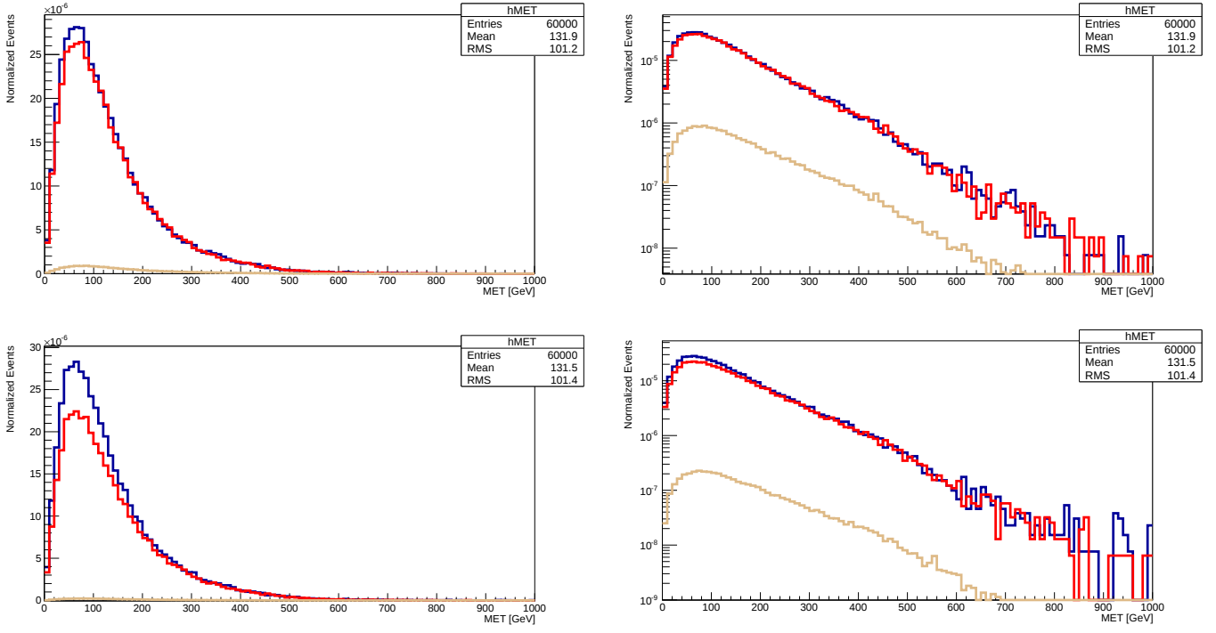
Figure 9.1: E_T^{\text{miss}} distributions for m_\chi = 10, 100, 1000 \text{ GeV} (blue, red and light-brown) for the vector D5 coupling (upper row) and axial-vector D8 (bottom row) in linear and logarithmic scale.
