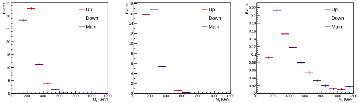
Figure 7.17: Shape uncertainties resulting from muon momentum scale variation for the ZZ (left), WZ (middle) and D8 with m_\chi = 100 GeV (right).
