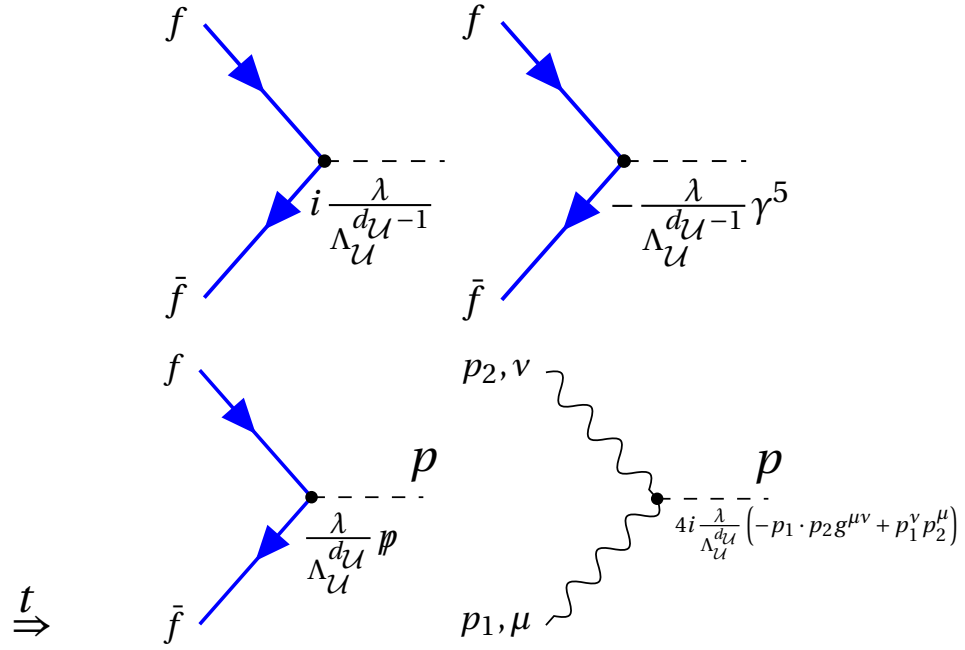
Figure 3.5: Vertices for the interactions of a scalar unparticle with the SM particles. The unparticle is indicated by a dashed line. A pair of fermions, a quark and an anti-quark for instance, couple to an unparticle (real emission) in the top diagrams and the bottom left diagram – this scenario is also considered in the present thesis. A gauge boson emits an unparticle in the scenario shown in the bottom right diagram.
