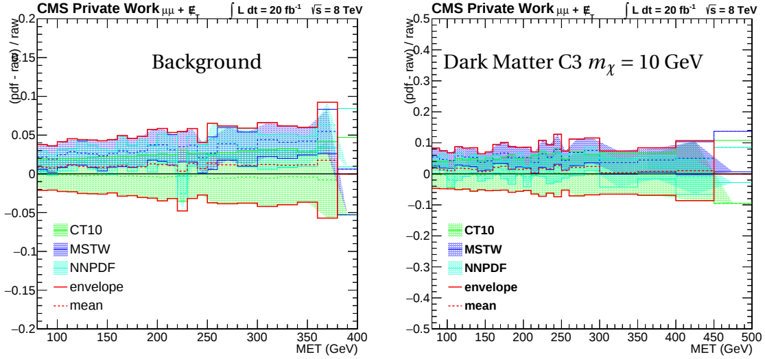
Figure 7.19: Relative uncertainty on the background prediction (left) and for C3 coupling with m_\chi = 10 GeV (right) for the final selection as a function of E_T^{\text{miss}} due PDF. The uncertainty tends to grow with increasing E_T^{\text{miss}} .
