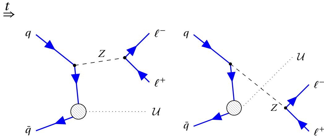
Figure 7.2: Feynman diagrams for unparticle \mathcal{U} production in association with a Z boson which subsequently decays into a pair of electrons or muons. The time axis is horizontal as indicated above the diagrams. The hatched circles indicate the interaction modeled with an effective field theory.
