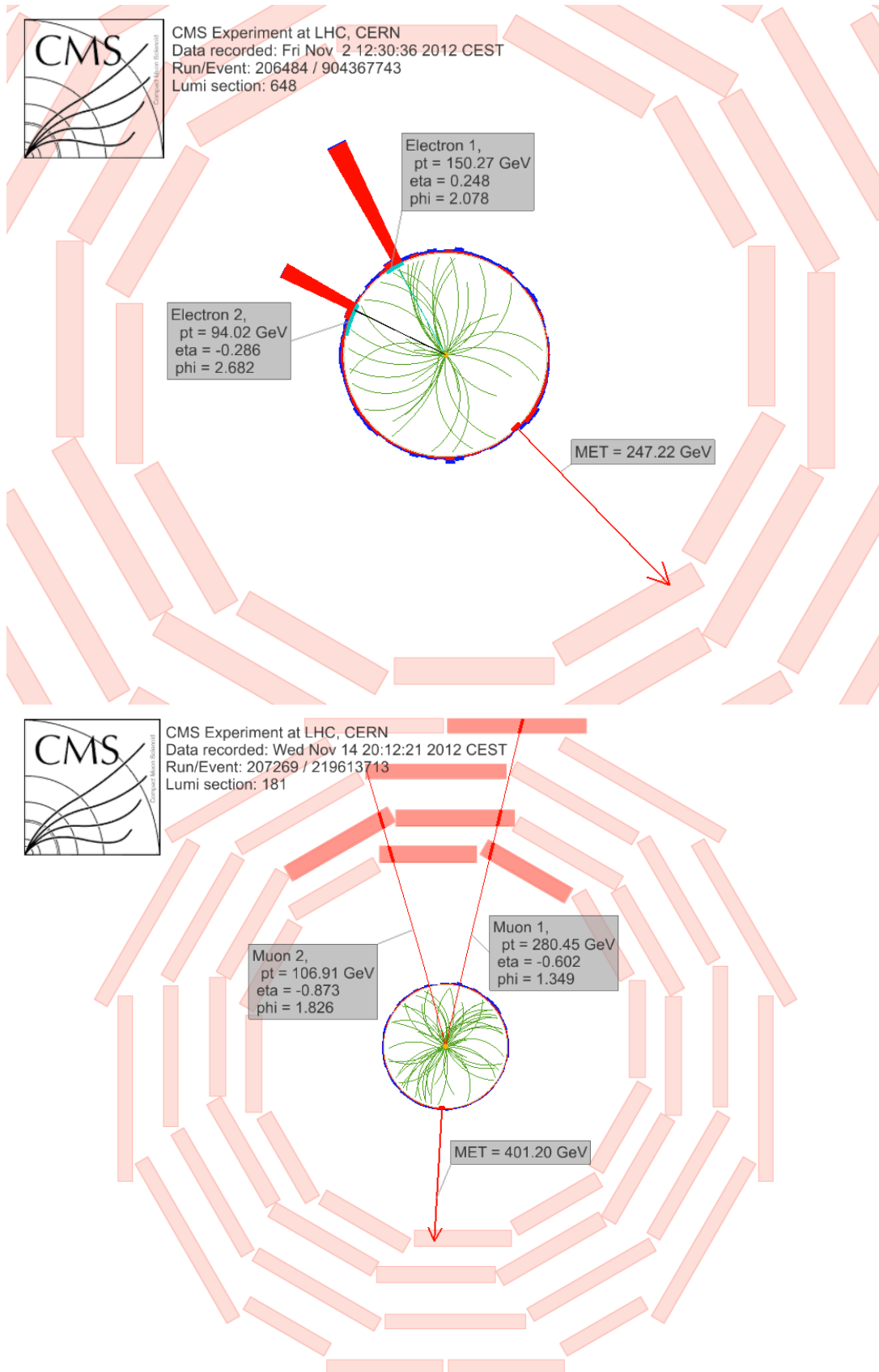
Figure 8.1: Event view for a high energetic dielectron+ E_T^{\text{miss}} (top) and a high energetic dimuon+ E_T^{\text{miss}} (bottom) events.
