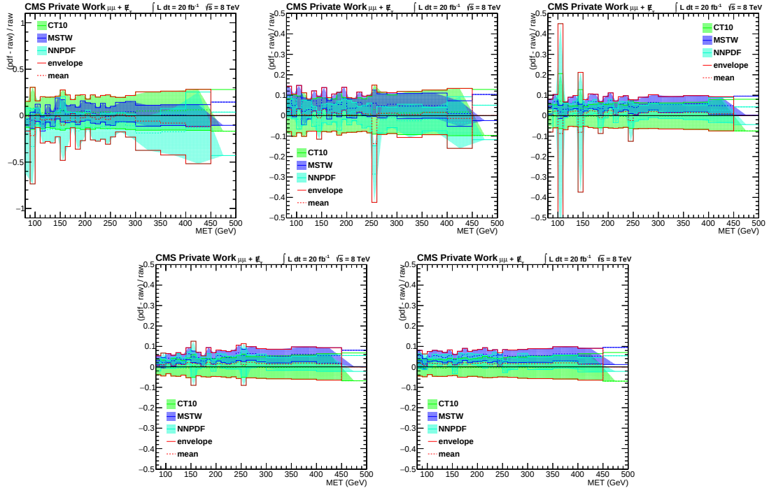
Figure 9.5: Signal PDF uncertainty for m_\chi = 1000, 500, 200, 10, 1\text{ GeV} with D9 coupling as function of E_T^{\text{miss}} (left to right, top to bottom)
