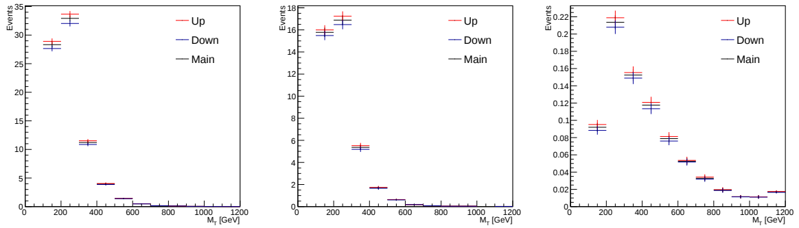
Figure 7.21: Shape uncertainties resulting from pileup for the ZZ (left), WZ (middle) and D8 with m_\chi = 100 \text{ GeV} (right).
