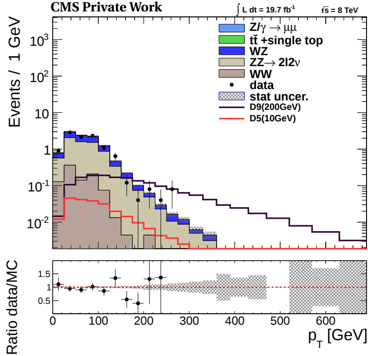
Figure 9.9: Muon p_T after all selection cuts.
