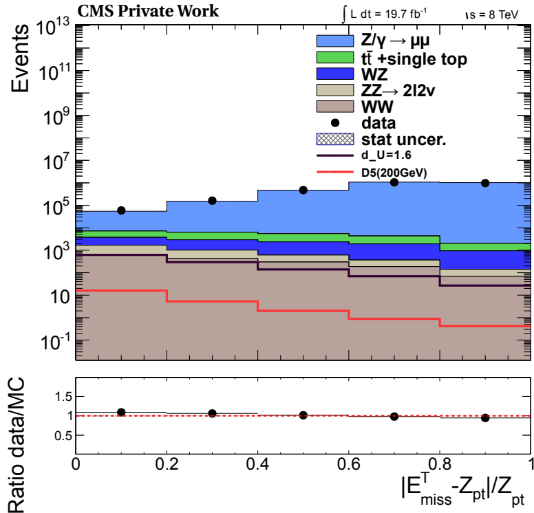
Figure 7.8: Distribution of the balance variable in the dimuon channel for the background samples and two signal hypotheses. The shape of the balance variable is different for the Drell-Yan background compared to signal hypotheses of dark matter and unparticle production allowing for an effective separation.
