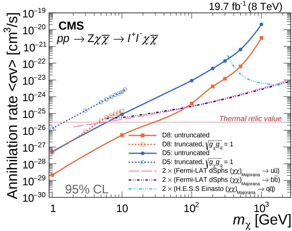
Figure 8.5: 95% CL upper exclusion limits on the dark matter annihilation rate \langle\sigma v\rangle for \chi\bar{\chi} \rightarrow q\bar{q} as a function of the DM particle mass m_\chi for vector coupling (D5) and axial-vector (D8) coupling. It is assumed that dark matter annihilates to quark with a 100% branching fraction. Experimental results from H.E.S.S [259] and Fermi-LAT [260] are also shown. Thermal relic value (the value which is required for dark matter in order to account for the relic abundance of dark matter) is shown as a red dotted line. Truncated limits with couplings set to \sqrt{g_q g_\chi} = 1 are denoted by dashed lines ([1], based on input from the present analysis).
