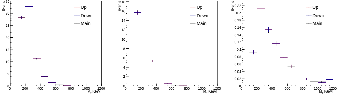
Figure 7.18: Shape uncertainties resulting from muon resolution variation for the ZZ (left), WZ (middle) and D8 with m_\chi = 100 GeV (right).
