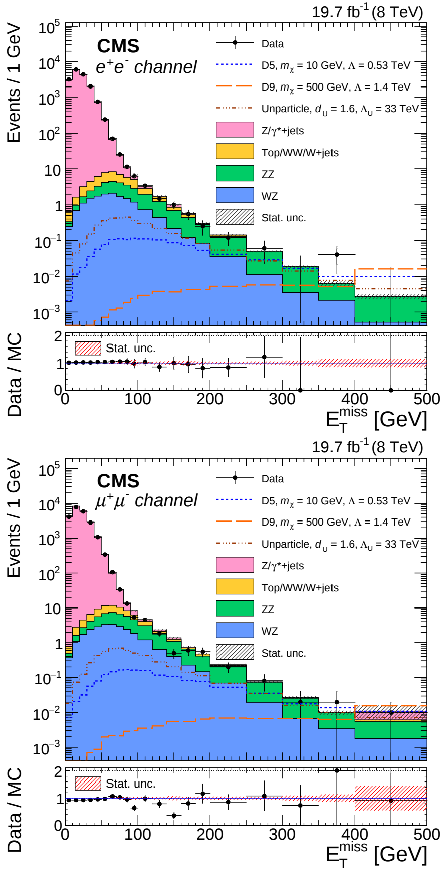
Figure 7.9: The distribution of E_T^{\text{miss}} after preselection for the Z \rightarrow ee (top, Northeastern) and Z \rightarrow \mu\mu (bottom, this thesis) channels. Several signal scenarios are shown for comparison. The statistical uncertainty is indicated by hatched regions. No scale factor from data-driven background estimation have been applied as these are only determined for the final selection step. The last bin of each distribution is the overflow bin containing all contributions above. Agreement is observed between the measurement and prediction whereby an outlier is visible for the dimuon side ([1], based on input from the present analysis).
