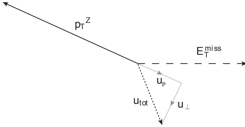
Figure 7.6: Geometrical construction of the response vector \vec{u}_{\text{tot}} . For processes in which the Z boson recoils against dark matter particles, one expects that the component u_p which is parallel to the axis of the p_T^Z be minimal due to the fact that the angle between the Z boson and missing energy E_T^{\text{miss}} is 180^\circ (back-to-back).
