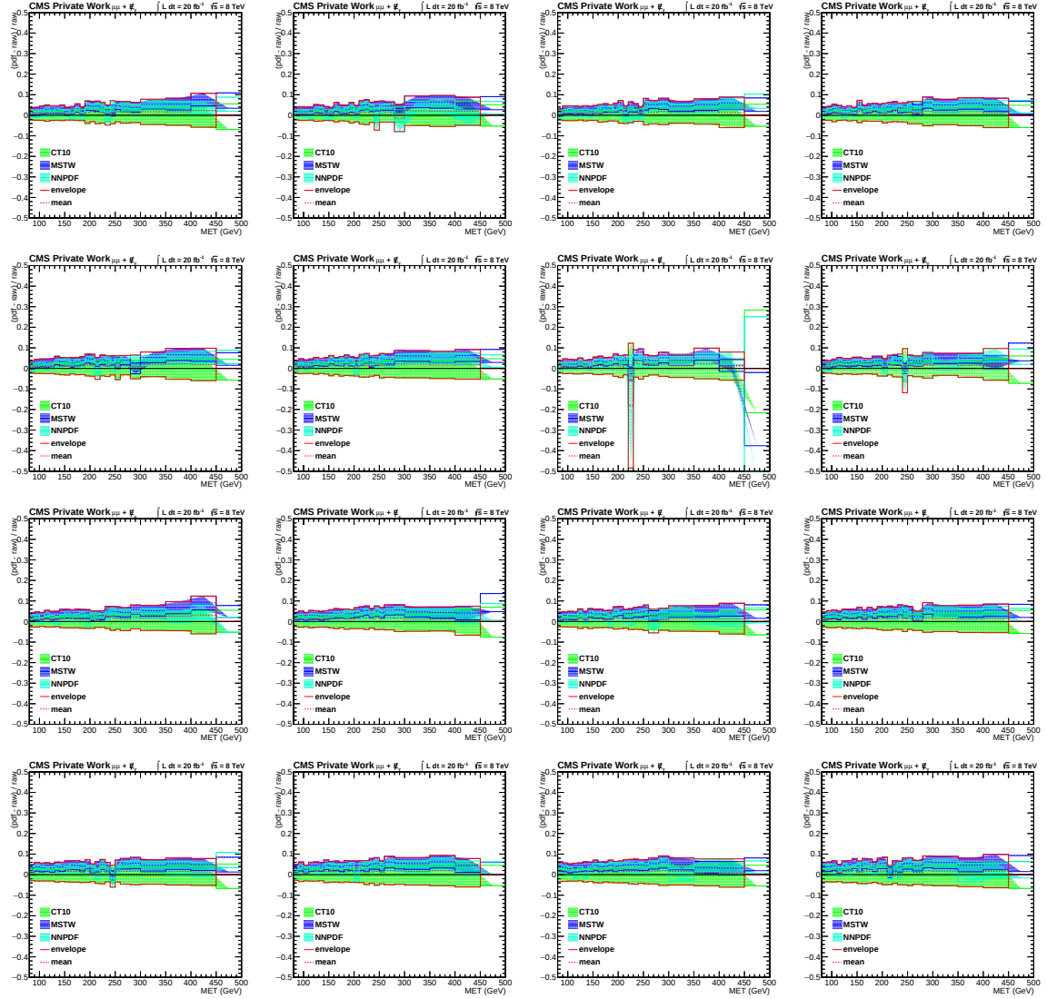
Figure 9.7: Signal PDF uncertainty for d_M = 1.01, 1.02, 1.04, 1.06, 1.09, 1.1, 1.2, 1.3, 1.4, 1.5, 1.6, 1.7, 1.8, 1.9, 2.0, 2.2 as function of E_T^{\text{miss}} (left to right, top to bottom)
