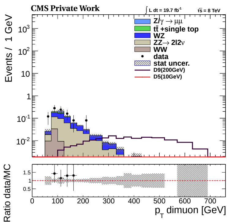
Figure 9.12: Vector sum of the dimuon p_T in the final event selection with one additional jet.
