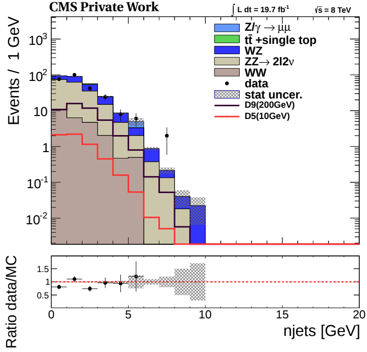
Figure 9.10: Number of jets in the final event selection excluding the jet veto in the dimuon channel.
