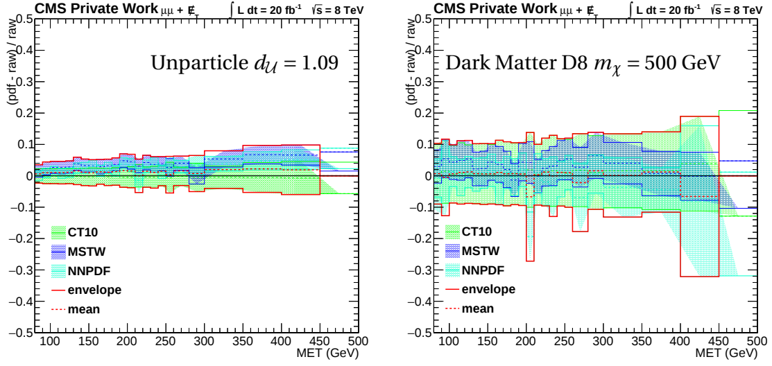
Figure 7.20: Relative uncertainty on the unparticle signal prediction with d_U = 1.09 (left) and for D8 coupling with m_\chi = 500 \text{ GeV} (right) for the final selection as a function of E_T^{\text{miss}} . The uncertainty increases rapidly for growing values of m_\chi .
