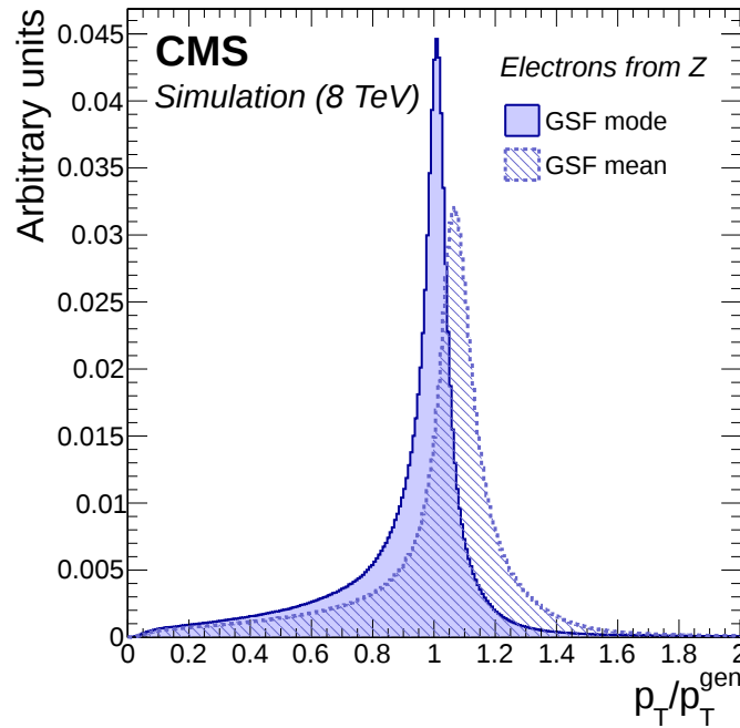
Figure 6.2: Ratio of reconstructed p_T of the electron and the generated p_T of the electron in simulation of Z \rightarrow ee events. Two reconstruction modes are shown – one using the most probable value of the GSF track component in solid and the weighted mean of the GSF fit in dashed [204].
