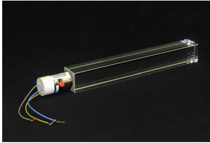
Figure 4.5: A picture of a ECAL scintillating \text{PbWO}_4 crystal from the endcap region [166].
