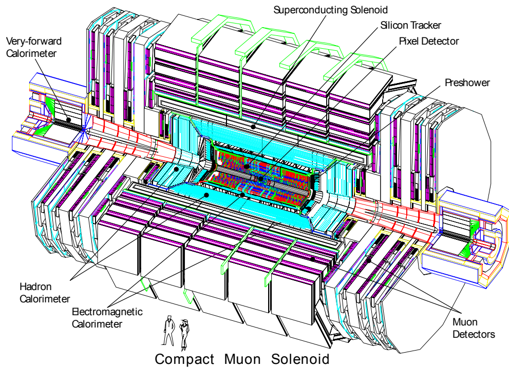
Figure 4.3: The CMS detector at CERN. The "onion"-like structure is shown and all subdetectors are indicated [166].
