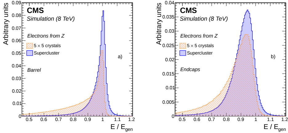
Figure 6.1: Distribution of the ratio of reconstructed and generated energy of a simulated electron arising from a Z \rightarrow ee decay for the barrel (left hand side) and endcaps (right hand side). The performance of the 5 \times 5 crystals versus the performance of superclusters is shown whereby no further corrections are applied. It is visible that the Supercluster approach performs better [204].
