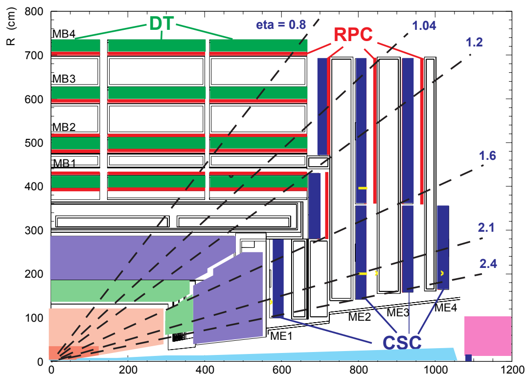
Figure 4.10: Muon detection system of CMS. The green detectors denote the drift tubes which are only installed in the barrel region, the resistive plate chambers in both the barrel and the end-cap regions are presented in red, the cathode strip chambers in the endcap are plotted in blue [166].
