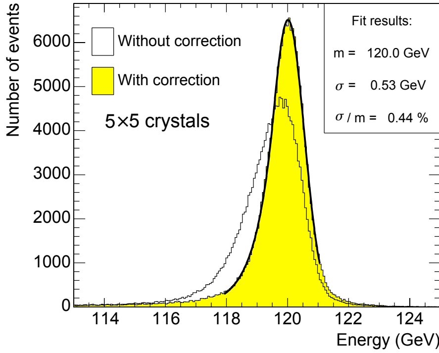
Figure 4.7: Distribution of energy reconstructed in a 5 \times 5 \text{PbWO}_4 crystal arrangement radiated with 120 GeV electrons over a 20 \times 20 \text{ mm}^2 , showing the results before and after correction for containment [166].
