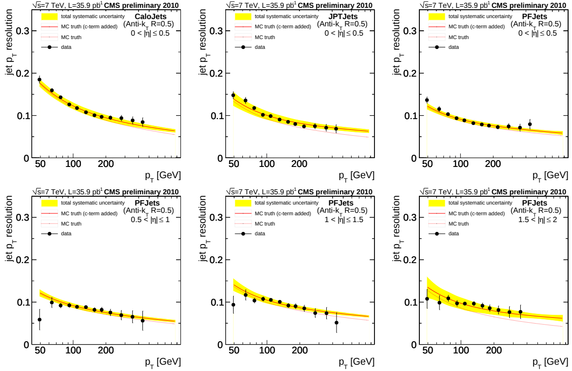
Figure 4.9: Top: Corrected jet p_T resolution in the 0 \leq |\eta| \leq 0.5 region for MC simulation and data before and after correction for the observed discrepancy. It is visible that p_T resolution improves with increasing p_T of the jet, whereby the PF reconstruction algorithm delivers best values. Bottom: Corrected jet p_T resolution for MC simulation and data before and after correction for higher values of |\eta| employing the PF algorithm [177].
