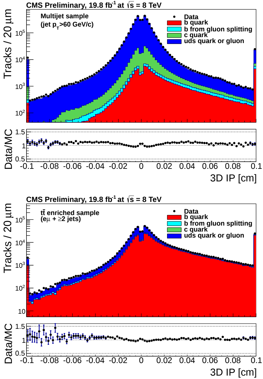
Figure 6.3: Distribution of the 3-dimensional impact parameter for a multijet (top) and t\bar{t} enriched sample measured with CMS in 2012. On the right (bottom) of each distribution, the contribution is added in one overflow (underflow) bin [224].
