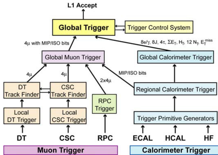
Figure 4.17: The structure of the level 1 trigger system of CMS. Information from calorimeters as well as from the muon system is employed for the decision making. [166].
