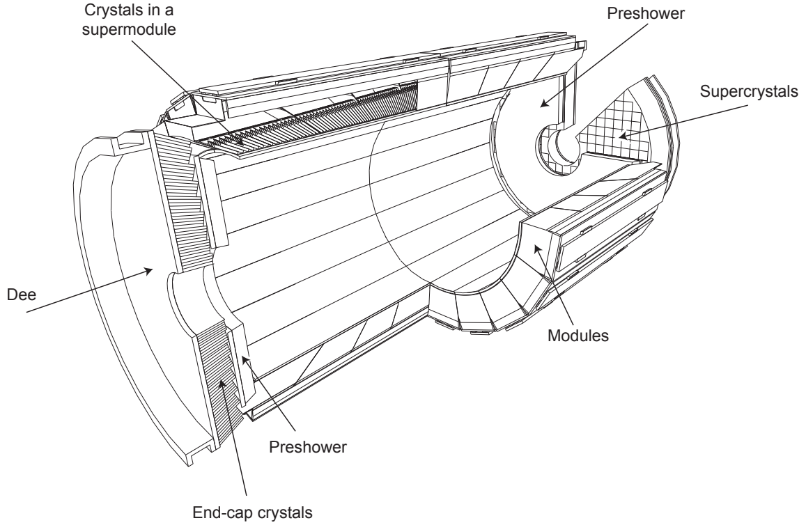
Figure 4.6: A schematic drawing of the electromagnetic calorimeter of CMS [166].
