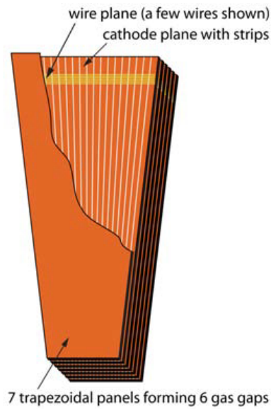
Figure 4.14: The structure of the cathode drift chambers of CMS. The strips are aligned radially. The largest chambers are 3.4 m long [166].
