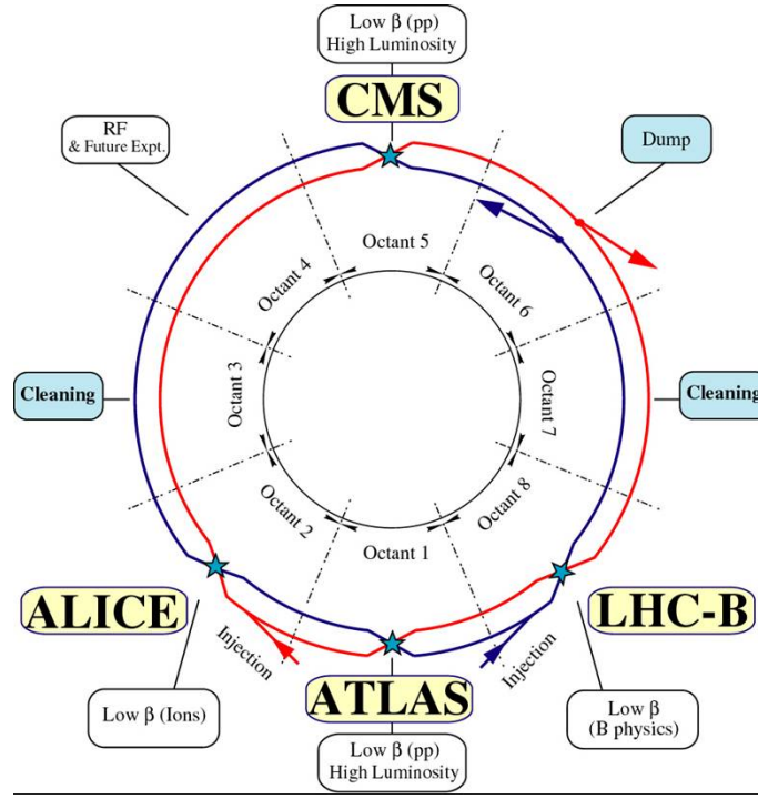
Figure 4.1: A schematic drawing of the LHC accelerator ring. Two accelerator vacuum tubes are shown as well as the four interaction points at which the detectors are located. The centers of the octants are often referred to as points – e.g. Point 5, for the CMS underground cavern [167].
