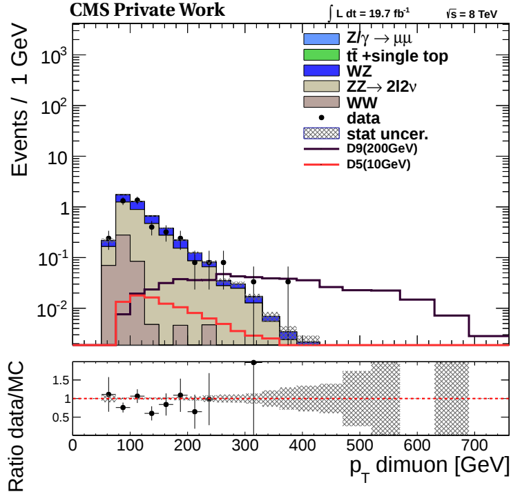
Figure 9.11: Vector sum of the dimuon p_T in the final event selection with no additional jets.
