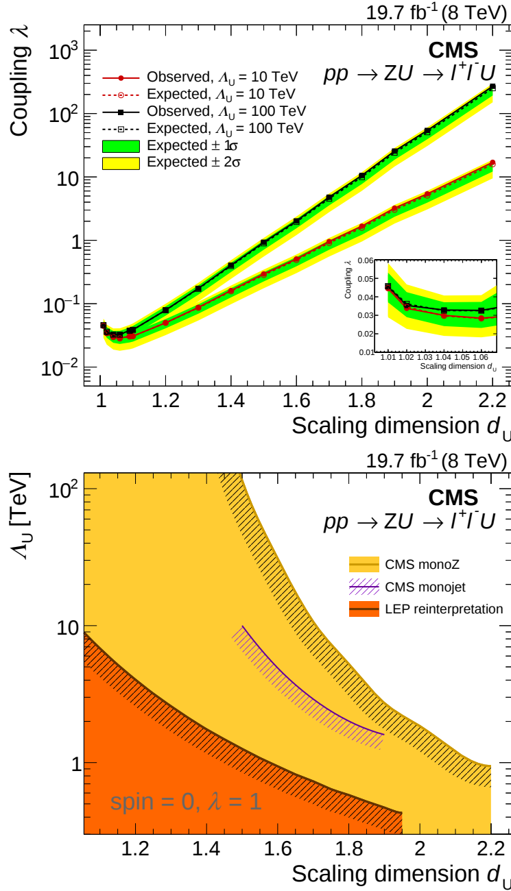
Figure 8.6: Top: 95% CL upper exclusion limits on the coupling \lambda of the unparticle to the standard model particles for two effective cutoff scale scenarios \Lambda_U = 10 and 100 TeV (left). An additional enhanced presentation is plotted for clarity. Bottom: 95% CL lower exclusion limits on unparticle effective cutoff scale \Lambda_U . Hereby, the coupling strength is fixed to \lambda = 1 . The results from CMS monojet search [16] along the reinterpretation of LEP searches [102] are shown for comparison. The shading indicates the excluded region of the parameter space ([1], based on input from the present analysis).
