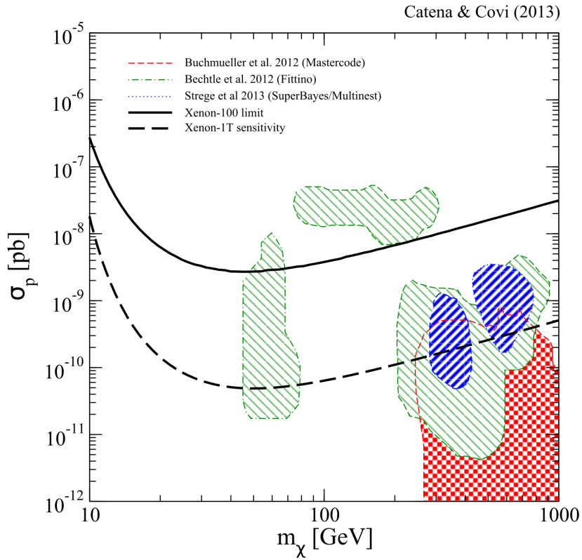
Figure 3.2: Regions in the plane of the dark matter mass m_\chi vs. the spin-independent dark matter nucleon scattering cross section \sigma_p which are found to be favored by independent global fits of the MSSM to variety of observations including LHC, cosmological limits, low energy observables and dark matter searches. The favored regions of the phase space are shown in hatched colors. Exclusion limits by the Xenon experiment as well as the estimated sensitivity of Xenon-1T experiment after one year data taking are shown for comparison [78].
