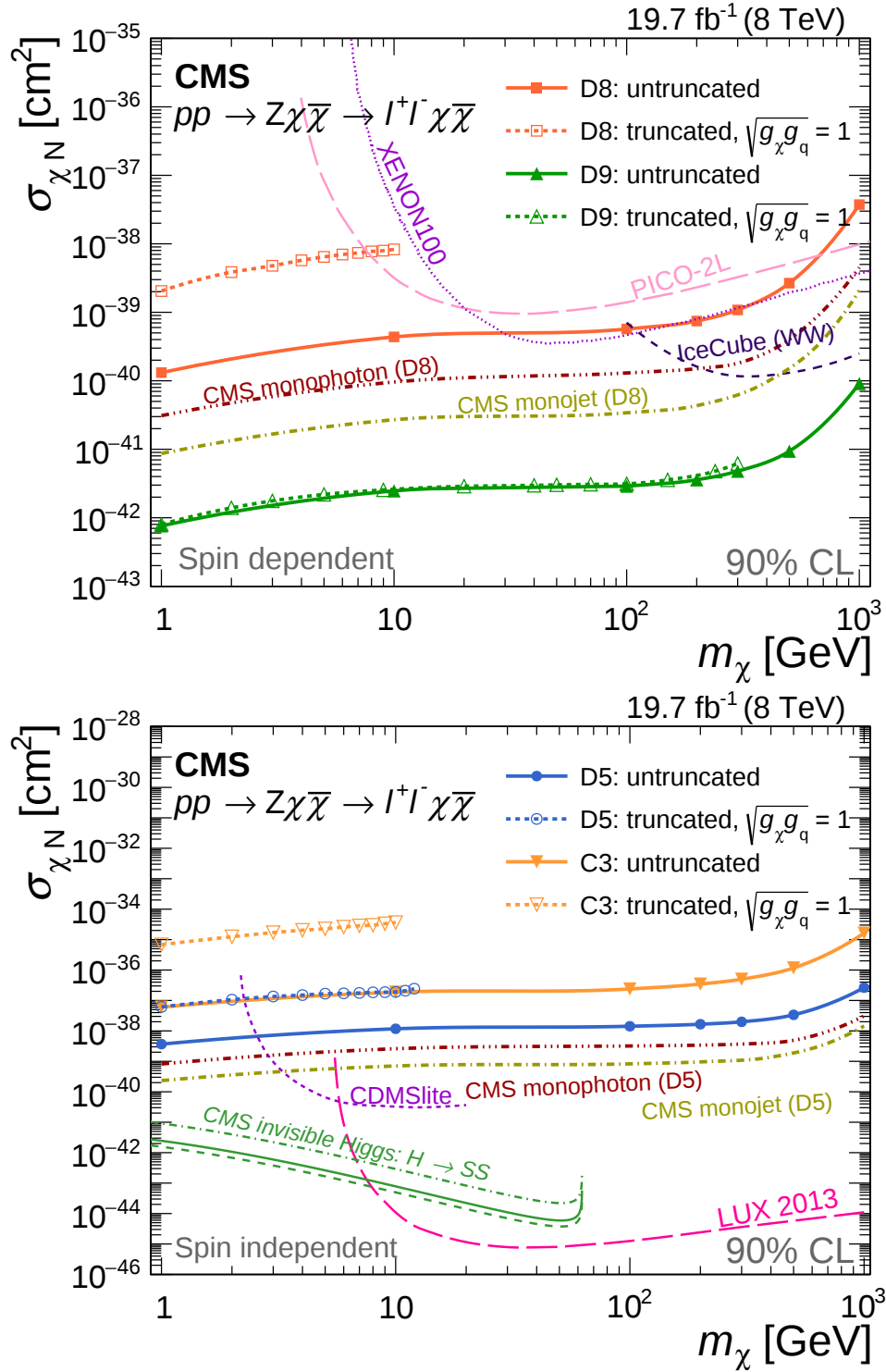
Figure 8.4: The 90% CL upper exclusion limits on the DM-nucleon cross section as a function of the dark matter particle mass m_\chi . Spin dependent exclusion limits for axial-vector D8 and tensor D9 couplings are shown on the top. For comparison, results from the PICO [254], XENON100 [255], and IceCube [9] collaborations are also shown. Spin independent exclusion limits for vector coupling operators C3 and D5 are shown on the bottom of the figure along results from CDMSlite [10], LUX [12], as well as Higgs-portal scalar DM results from CMS [258] with central (solid), minimum (dashed) and maximum (dot dashed) values of Higgs-nucleon couplings. Collider search results from CMS monojet [16] and monophoton [18] searches are included for comparison. Truncated exclusion limits with parameters \sqrt{g_q g_\chi} = 1 are denoted by dashed lines ([1], based on input from the present analysis).
