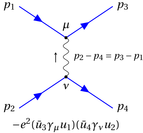
Figure 2.1: Electron-electron scattering described by the Feynman diagrams in leading order. The incoming electrons have the momenta p_1 and p_2 and interact at the vertices \mu and \nu exchanging a photon propagator. After the interaction, the exiting momenta are p_3 and p_4 . At all vertices, the four-dimensional momentum is conserved.
