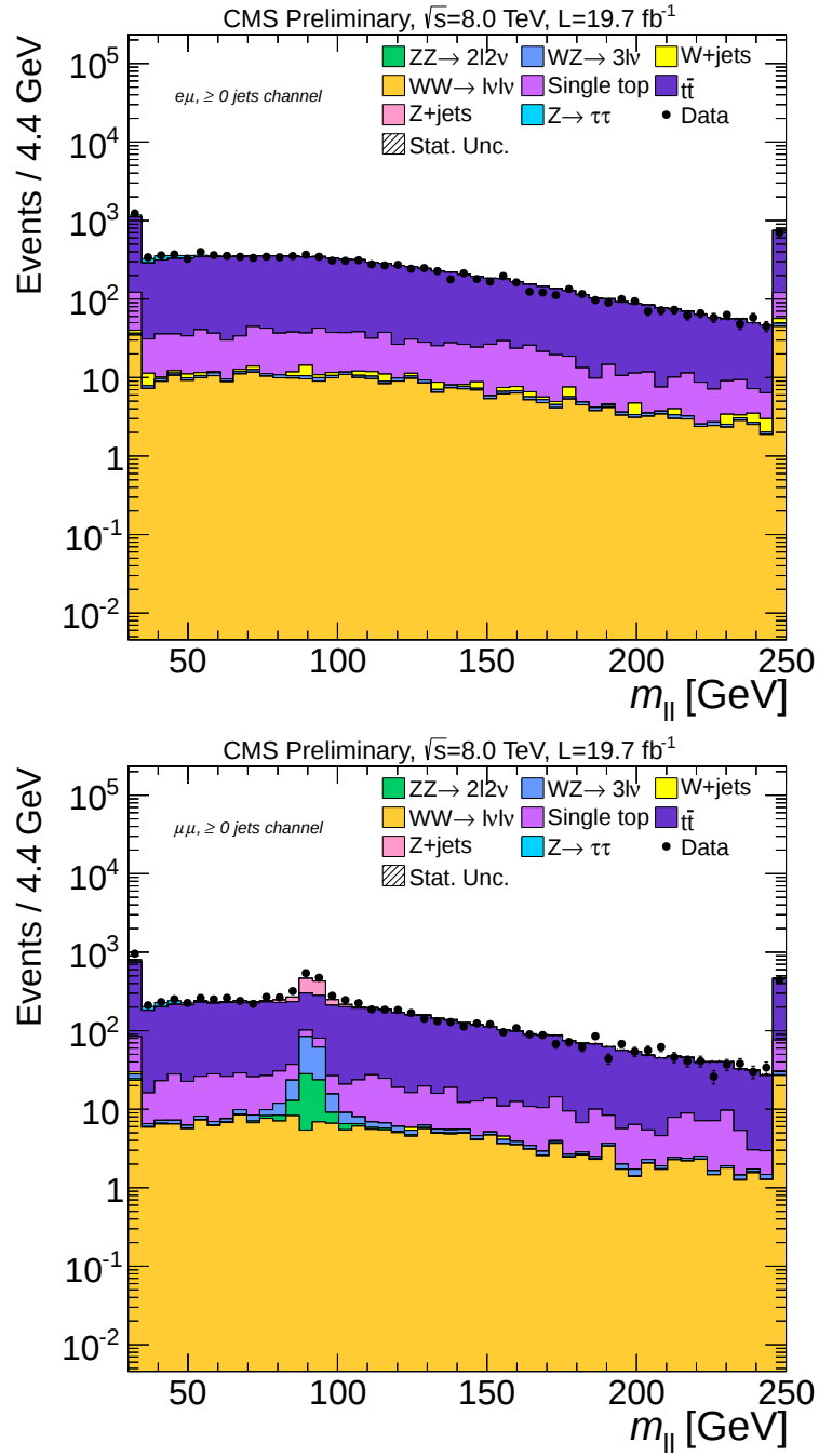
Figure 7.11: Distribution of dilepton invariant mass in e\mu (top) and \mu\mu (bottom) channel in the selected top-enriched sample. The region with 70 < m_{\ell\ell} < 110 GeV is excluded from the calculation of \alpha [232].
