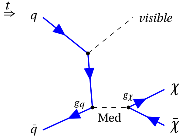
Figure 3.9: Collider production of dark matter in terms of a simplified model approach. Here, a pair quarks produces a particle which is detectable (marked by "visible" in the figure, e.g. Z boson) and also a heavy mediator, which is denoted by "Med". The mediator then decays into two dark matter particles \chi and \bar{\chi} . The coupling strength of dark matter to the mediator particle is denoted by g_\chi , the coupling strength of the mediator particle to the quarks is denoted by g_q . Further parameters are the mass of the mediator particle (typically denoted by m_{\text{Med}} ) and the mass of the dark matter particle m_\chi .
