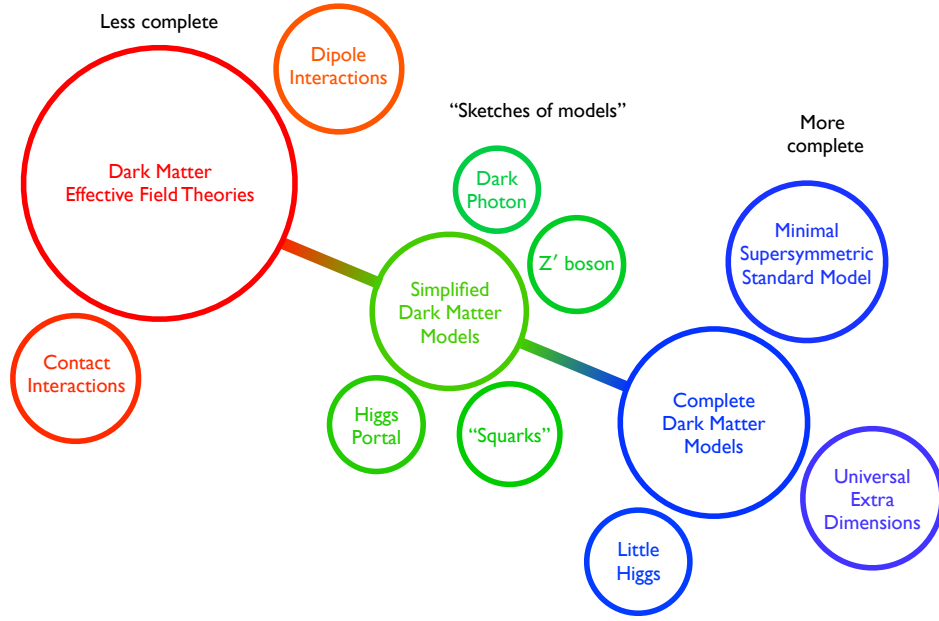
Figure 3.7: An artistic view of dark matter theories studied at particle colliders. The effective field theories (left) aim to explain the experimental effects of dark matter, whereas simplified models (middle) provide a more robust construct for the implementation of dark matter into theory. Theories like minimal supersymmetric SM (right) provide the most sophisticated explanation for dark matter from the theoretical point of view embedding it into a larger theory construction [117].
