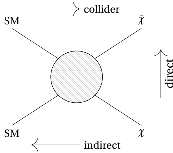
Figure 3.6: Three possible ways of detecting dark matter. Interaction of two standard model (SM) particles producing two dark matter particles is used in collider searches, whereby an additional standard model particle is needed (via initial or final state radiation) for observing (tagging) the interaction. Indirect detection relies on the annihilation of two dark matter particles producing two standard model particles which can be observed. Direct detection relies on the interaction of a dark matter particle with a standard model particle leading to a standard model particle which can be observed and a dark matter particle which escapes undetected.
