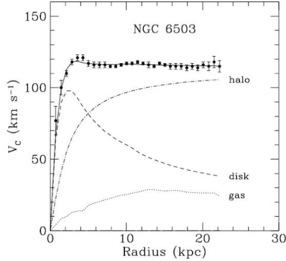
Figure 1.1: The measured rotation velocity of the spiral galaxy NGC 6503. The dashed and dotted lines represent the contribution by the visible matter and gas. The contribution of "halo" is attributed to the dark matter and is an assumption which can be used for explaining the observed curve [5].
