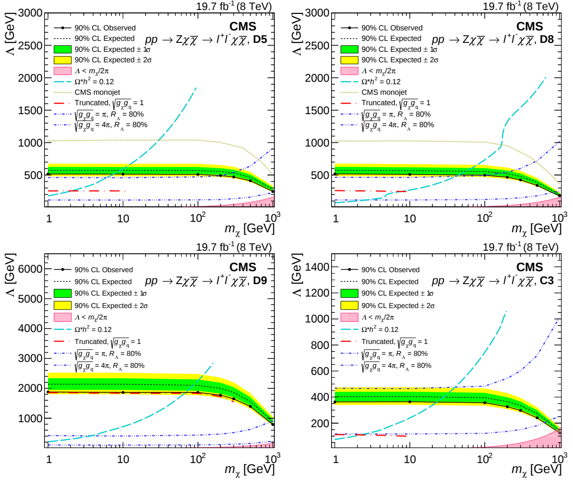
Figure 8.3: Expected and observed 90% CL lower exclusion limits on the EFT parameter \Lambda as a function of dark matter particle mass m_\chi . Couplings D5 (top left), D8 (top right), D9 (bottom left), and C3 (bottom right) are shown. The cyan long-dashed line is calculated by MadDM 1.0 [252] and indicates the relic density of cold non-baryonic dark matter: \Omega h^2 = 0.1198 \pm 0.0026 as measured by the Planck telescope [253]. The pink shaded area shows the lower bound with \Lambda > m_\chi/2\pi where the effective field theory approach is no longer valid. Results from CMS monojet search [16] is shown for D5 and D8 scenarios. Truncated limits with the requirement \sqrt{g_q g_\chi} = 1 are presented with red dot long-dashed lines. The blue triple-dot and double-dot dashed lines show the contours of truncated exclusion limits with R_\Lambda = 80\% for all considered operators. Hereby, the couplings are set to \sqrt{g_q g_\chi} = \pi and 4\pi ([1], based on input from the present analysis).
