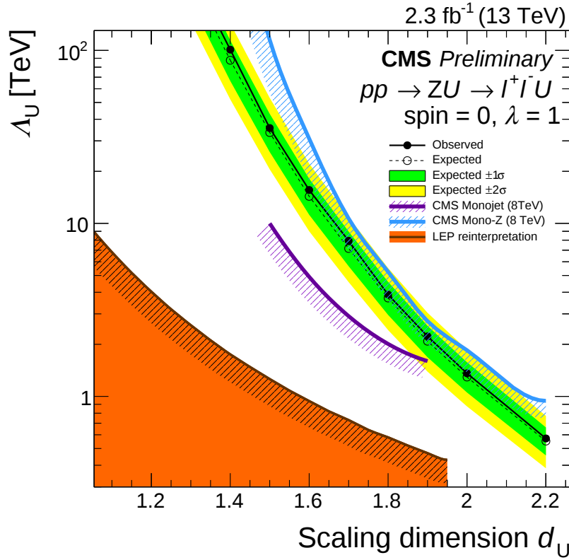
Figure 8.10: 95% CL lower exclusion limits on unparticle effective cutoff scale \Lambda_U assuming a fixed coupling \lambda = 1 obtained at \sqrt{s} = 13 TeV with an integrated luminosity of 2.3 \text{ fb}^{-1} . Results from the 8 TeV monojet search [16], the reinterpretation of LEP searches [102] as well as the result of the present dissertation (cf. Fig.8.6) are shown for comparison. The observed sensitivity is comparable to the one observed in the 8 TeV case albeit the much smaller dataset size [128].
