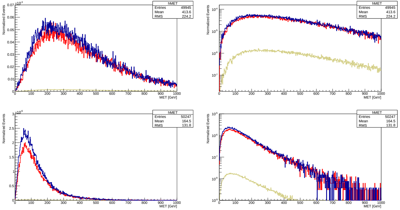
Figure 9.2: E_T^{\text{miss}} distributions for m_\chi = 10, 100, 1000 \text{ GeV} (blue, red and light-brown) for the tensor D9 coupling (upper row) and axial-vector C3 (bottom row) in linear and logarithmic scale. It is visible that the shape of D9 signal is significantly different from other three coupling operators. This also results in a harder p_T spectrum of the dilepton pair.
