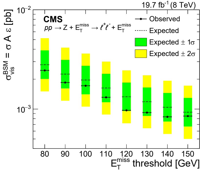
Figure 8.7: 95% CL model-independent upper limits on the visible cross section ( \sigma A \epsilon ) for production of events beyond the standard model as a function of E_T^{\text{miss}} cutoff threshold ([1], based on input from the present analysis).
