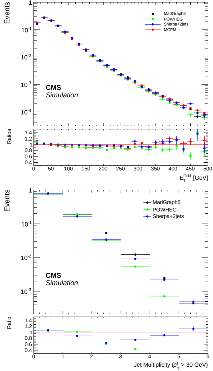
Figure 7.23: Distributions of E_T^{\text{miss}} (top) and jet multiplicity (bottom) at generator level for different generators employed for the estimation of the ZZ background uncertainty [232]. A deviation is visible which is interpreted as an uncertainty for the final ZZ background prediction.
