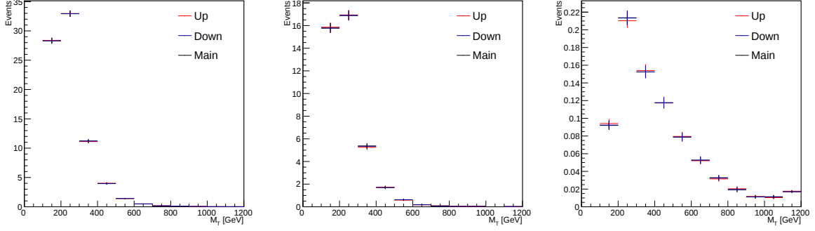
Figure 7.15: Shape uncertainties resulting from jet energy resolution variation for the ZZ (left), WZ (middle) and D8 with m_\chi = 100 GeV (right).
