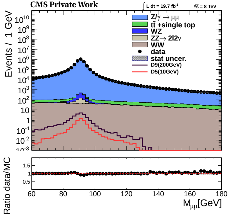
Figure 7.5: Invariant mass of dimuon pairs after the physics object selection requirement. Standard model prediction estimates from MC from different processes are shown stacked in different colors. Two signal hypotheses are plotted for clearness. Agreement between the prediction and measurement is observed. It is visible that both signal hypotheses have a clear peak around the Z mass. Only events with the invariant mass within m_Z \pm 10 \text{ GeV} are considered for further analysis.
