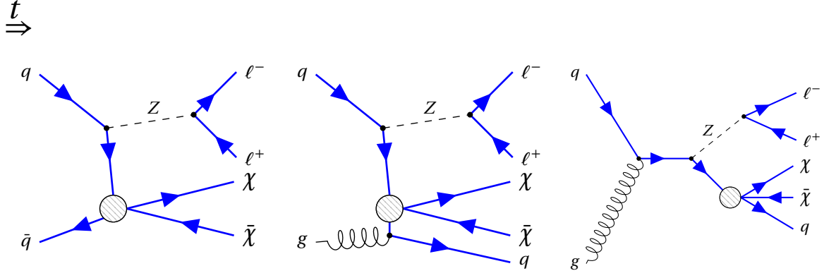
Figure 7.1: Dark matter signatures considered in the present thesis. The Z boson is produced in a proton-proton collision and recoils against two undetectable dark matter particles \chi subsequently decaying into a pair of electrons or muons. Also scenarios with radiation of one jet are studied. The time axis is horizontal as indicated above the diagrams. The dashed circle represents the interaction modeled by the effective field theory.
