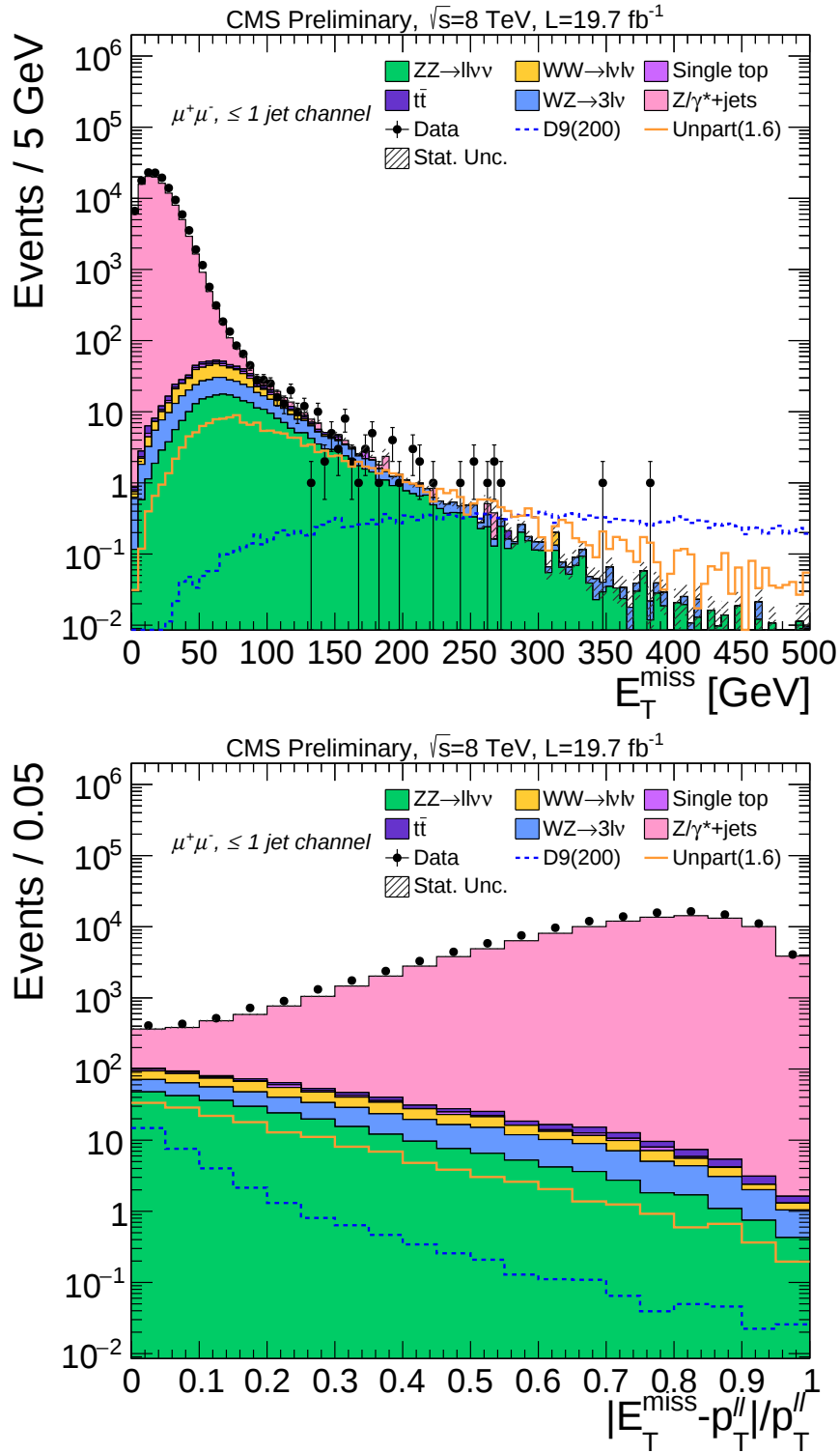
Figure 7.10: Distributions of E_T^{\text{miss}} (top) and balance b (bottom) employed for the derivation of the Drell-Yan scale factors in the control regions (before the application of scale factors). The full selection except E_T^{\text{miss}} , balance b and \Delta\phi requirements is applied [232].
