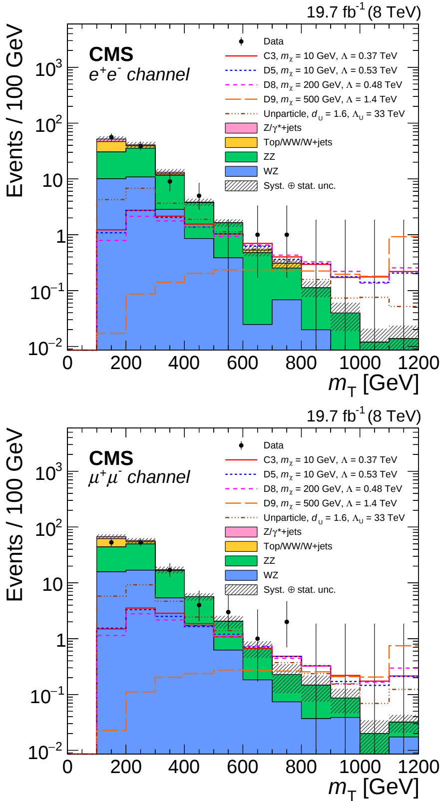
Figure 8.2: Distributions of the transverse mass m_T for the final selection in the electron (top, Northeastern) and muon (bottom, this thesis) channels. Sample distributions of m_T for several dark matter and unparticle signal hypotheses are shown. Examples of expected signal distributions are shown for DM production and unparticle production. The total statistical and systematic uncertainty in the overall background is shown as a hatched region. Overflow events are integrated in the last bin. Agreement is observed between the standard model prediction and the data measurement ([1], based on input from the present analysis).
