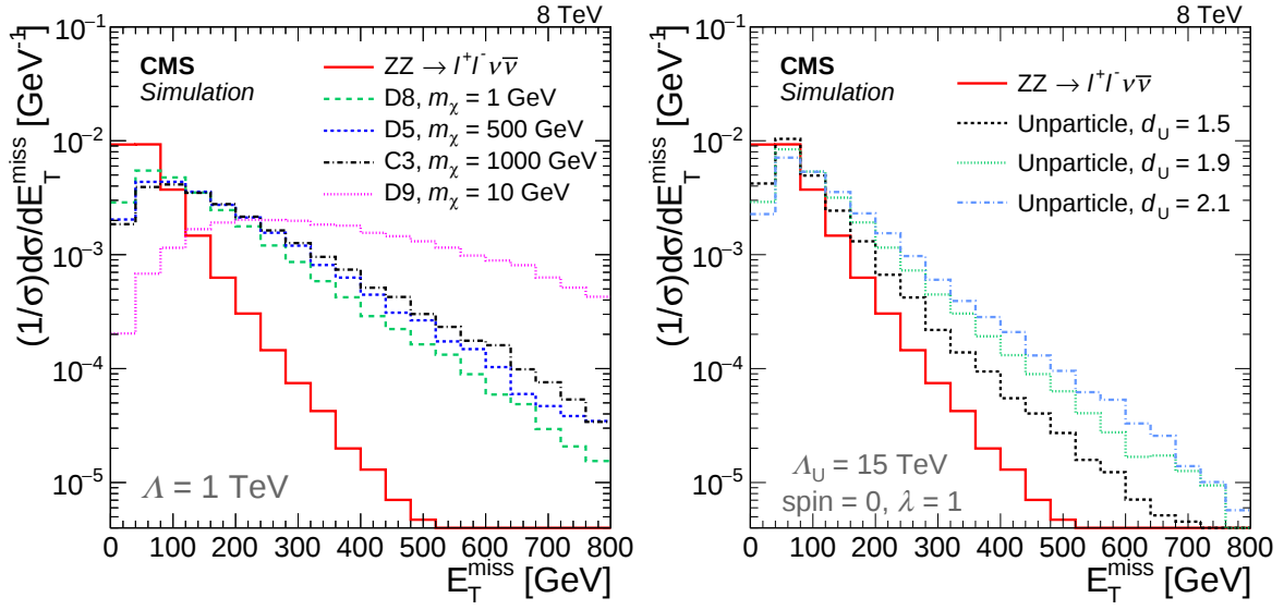
Figure 7.3: The normalized distribution in E_T^{\text{miss}} at the generator level, for DM (left) and unparticle (right) scenarios. The DM curves are shown for different m_\chi with vector (D5), axial-vector (D8), and tensor (D9) coupling for Dirac fermions, and vector (C3) coupling for complex scalar particles. The scaling dimension d_U ranges from 1.5 to 2.1. The SM background ZZ \rightarrow \ell^- \ell^+ \nu \bar{\nu} is shown as a red solid curve [1].
