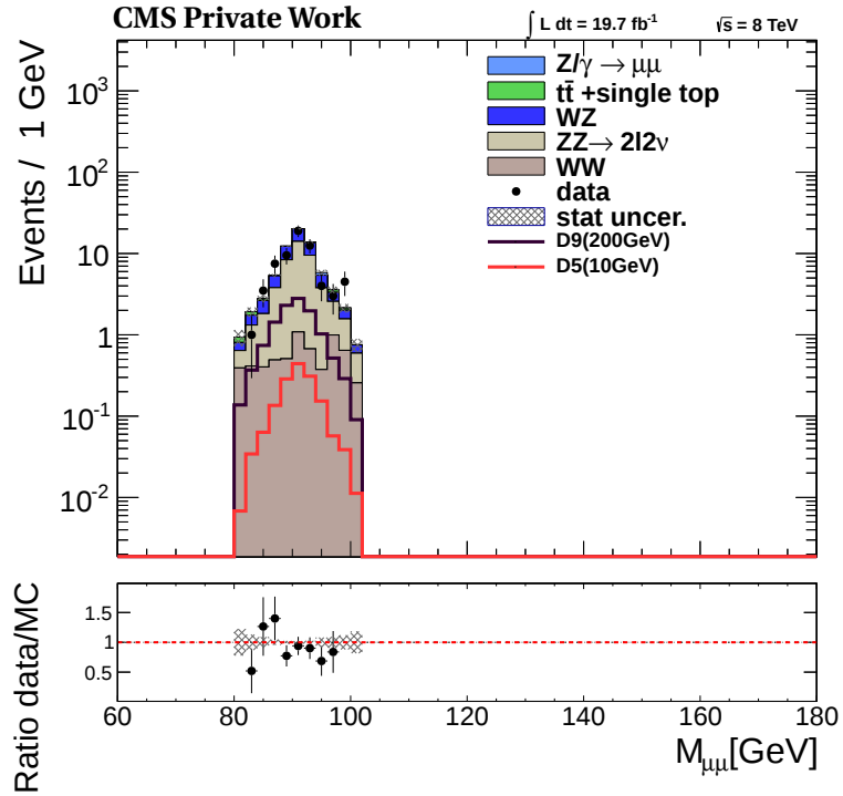
Figure 9.8: Mass of the dimuon system after all selection cuts.
