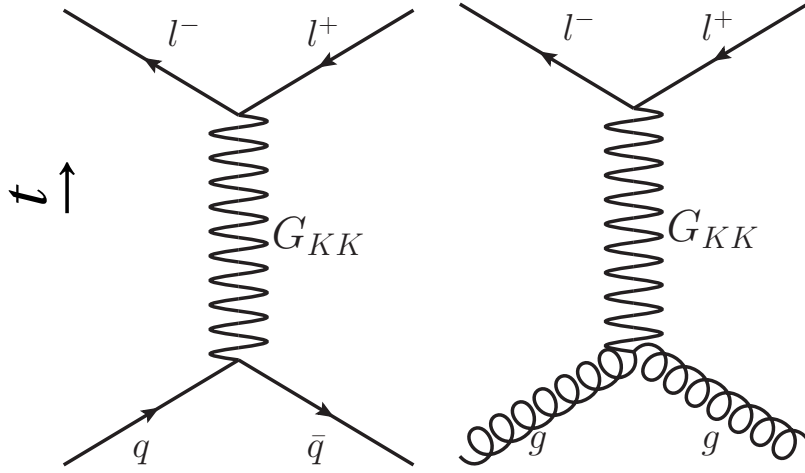
Figure 3.3: Virtual exchange of a Kaluza-Klein graviton G_{KK} at the LHC in the ADD theory with the subsequent decay into a lepton pair.
