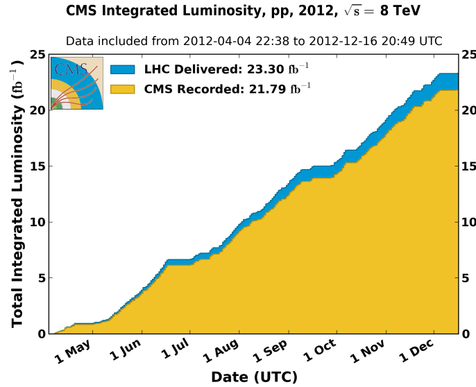
Figure 4.2: Total integrated luminosity delivered by the LHC and recorded by the CMS detector as a function of date in 2012 [172].
