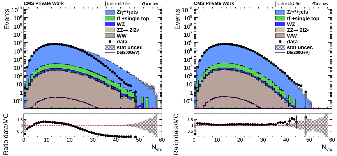
Figure 7.14: Distribution of the number of vertices N_{vtx} after a basic muon pair identification selection requirement before (left) and after (right) the pileup reweighting procedure. It is visible that the reweighting procedure leads to a much better agreement between the simulated and the measured distributions of N_{vtx} .
