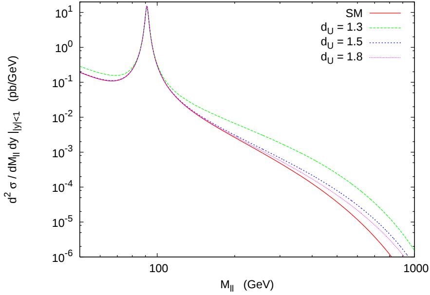
Figure 3.4: Simulated distribution of the invariant mass of a lepton pairs produced in p\bar{p} collisions at the Tevatron collider ( \sqrt{s} = 1.96 TeV) with possible scenarios of virtual unparticle production. The standard model contribution (Drell-Yan process) is shown in red. Scenarios of enhancement through the virtual unparticle exchange with d_U = 1.3; 1.5; 1.8 are shown for comparison. It is visible that a non-resonant excess of events in the tail of the distribution (high values of m_{\text{inv}}^{\ell\ell} ) can be interpreted as a hint for the existence of unparticles [95].
