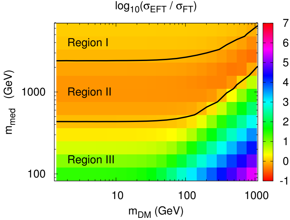
Figure 3.10: Ratio of the cross sections for a monojet final state computed with EFT and the simplified model approach (FT for Full Theory) as a function of m_{\text{med}} and m_{\chi} . Couplings are assumed to be g_q = g_{\chi} = 1 and the requirement p_T > 110 \text{ GeV} for the jet is introduced [131].
