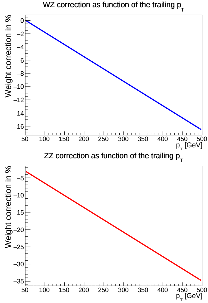
Figure 7.13: Electroweak corrections of the diboson background for WZ (top) and ZZ (bottom) as a function of the p_T of the trailing boson.
