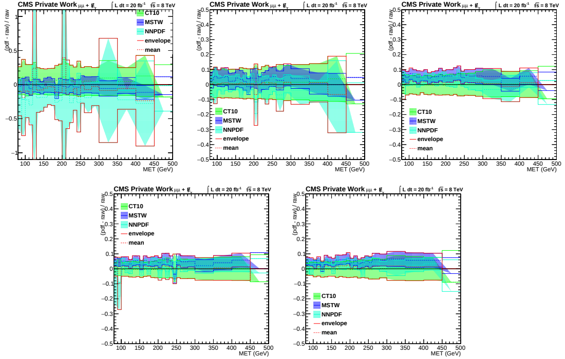
Figure 9.3: Signal PDF uncertainty for m_\chi = 1000, 500, 200, 10, 1\text{GeV} with D5 coupling as function of E_T^{\text{miss}} (left to right, top to bottom)
