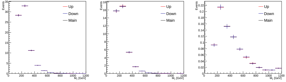
Figure 7.16: Shape uncertainties resulting from jet energy scale variation for the ZZ (left), WZ (middle) and D8 with m_\chi = 100 GeV (right).
