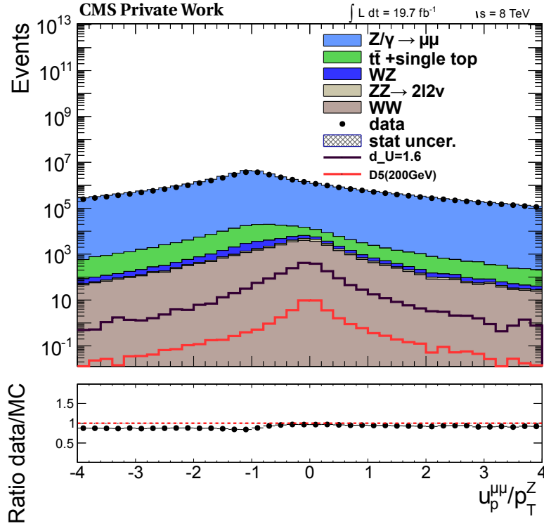
Figure 7.7: Distribution of the response variable u in the dimuon channel for the background samples and two signal hypotheses. It is visible that both signal assumptions peak around 0 whilst Z and top background peak around -1 .
