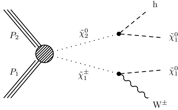
Figure 3.1: Event diagram for the production of the LSP in a MSSM scenario at the LHC. The pair of colliding protons produces a chargino \tilde{\chi}_1^\pm and a neutralino \tilde{\chi}_2^0 which both decay into a detectable particle (the Higgs boson and the W boson) and the lightest neutralino, the LSP [77].
