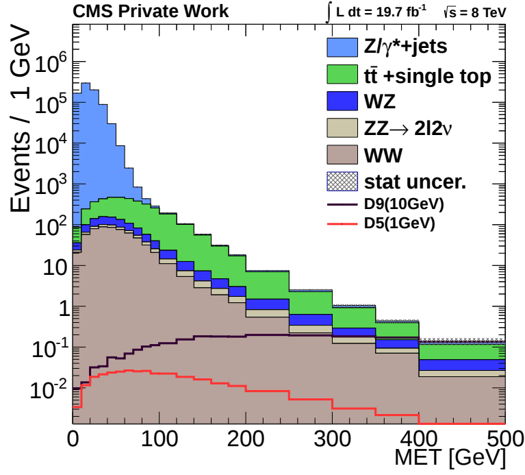
Figure 7.4: Simulated E_T^{\text{miss}} distribution of background contributions for a basic dimuon selection. One can see that the Drell-Yan contribution leads in the low E_T^{\text{miss}} region whilst top quark production is dominant in the high E_T^{\text{miss}} region. One scenario for D9 coupling with m_\chi = 10 GeV and a scenario for D5 coupling with m_\chi = 1 GeV are shown. The value of \Lambda is set to 1000 GeV.
