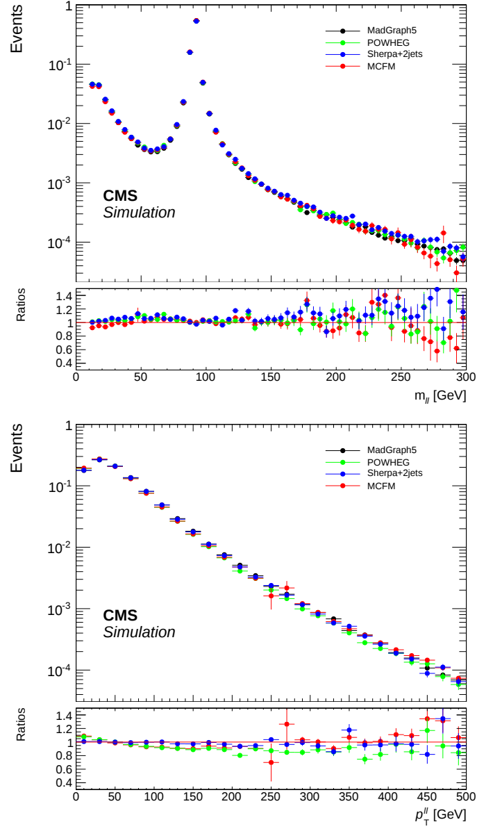
Figure 7.22: Distributions of dilepton mass (top) and dilepton p_T (bottom) at generator level for different generators employed for the estimation of the ZZ background uncertainty [232]. A deviation is visible which is interpreted as an uncertainty for the final ZZ background prediction.
