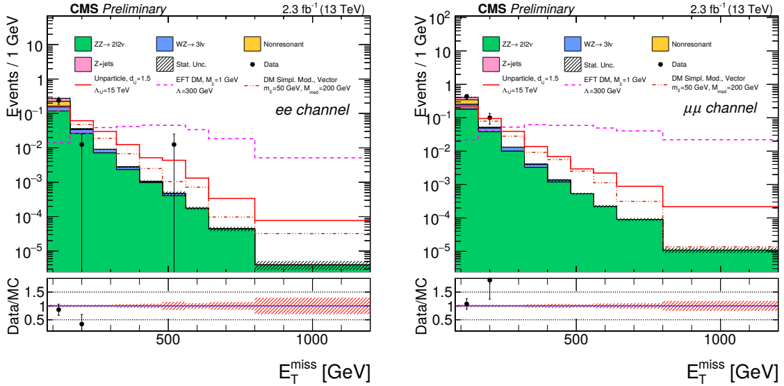
Figure 8.8: The distribution of E_T^{\text{miss}} after for the final selection for the Z \rightarrow ee (left) and Z \rightarrow \mu\mu (right) channels of the 13 TeV analysis. Expected signal distributions are shown for the simplified model of DM production with vector couplings, the EFT scenario of DM production, and unparticles. Agreement is observed between the measurement and background prediction [128].
