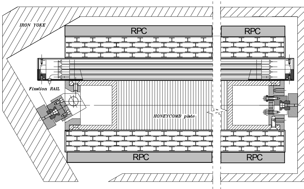
Figure 4.12: Drift tube chambers of CMS shown in the r - \phi plane. The two superlayers are visible, each containing 4 layers of rectangular drift cells, which are shifted by half a cell length with respect to each other. The resistive plate chamber are only indicated, the structure is not shown [166].
