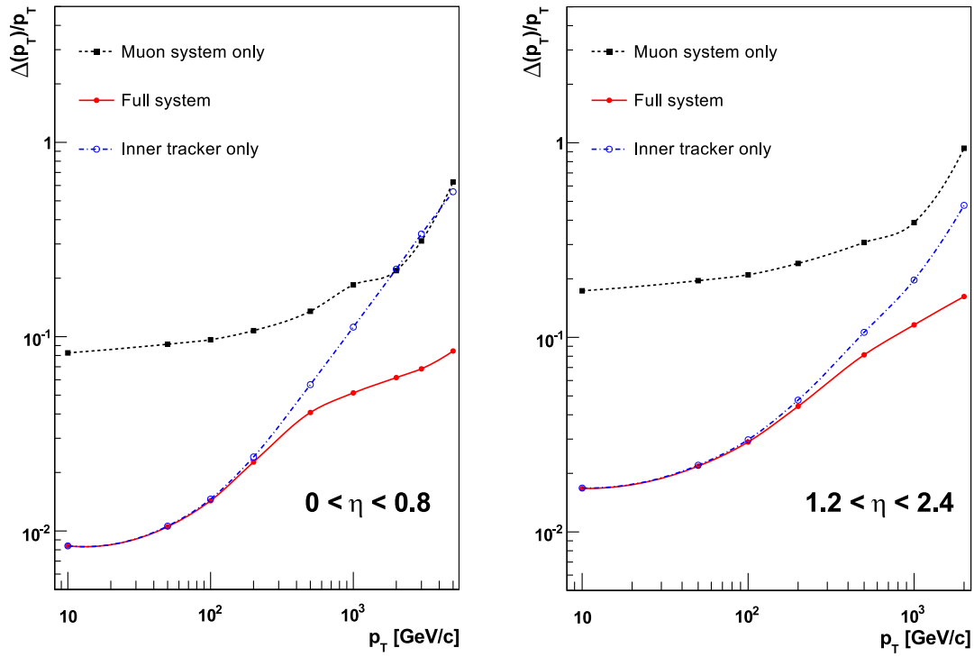
Figure 4.11: The relative muon momentum resolution as a function of muon p_T for two regions in |\eta| measured by the muon system only, the inner tracking system only and employing both systems at once [166].
