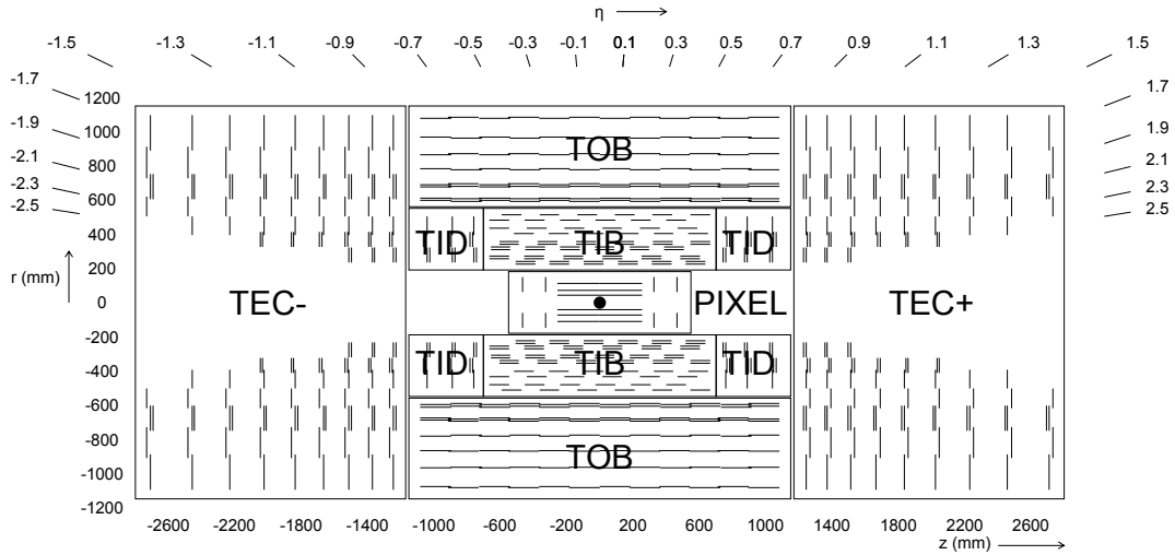
Figure 4.4: A schematic cross section of the CMS inner tracker system. TIB stands for Tracker Inner Barrel and TID stands Tracker Inner disks. TOB corresponds to Tracker Outer Barrel and TEC stands for Tracker EndCaps [166].
