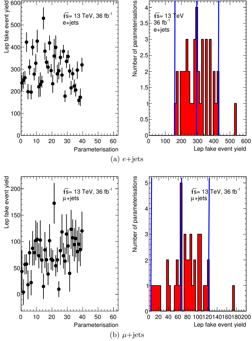
Figure 5.5.: The fake lepton yields for each parameterisation with the y -axis projection displayed on the right. The blue lines indicate the mean (the nominal weight) and the up/down systematic variations which form the extremes of the histogram.
