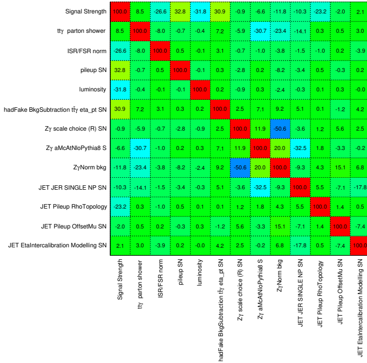
Figure 8.21.: Correlations for the single-lepton and dilepton channel for each nuisance parameter and the signal strength. Only NPs with at least one correlation above 15% are shown.
