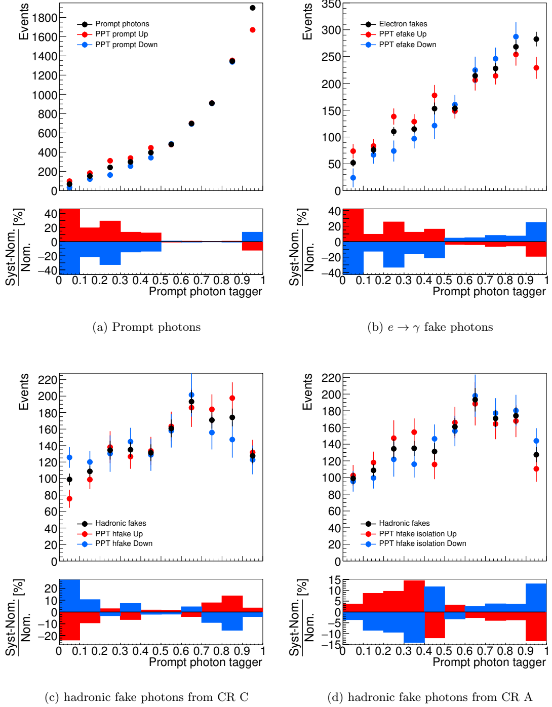
Figure 6.4.: The relative sizes of the PPT scale factors/systematic uncertainties for prompt, e \rightarrow \gamma fake and hadronic fake photons (for the two sources of uncertainties). “Up” and “down” labels are arbitrary.
