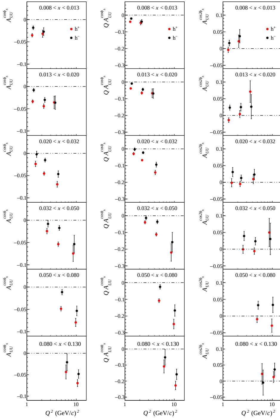
FIGURE 5.30: A_{UU}^{\cos\phi_h} , QA_{UU}^{\cos\phi_h} and A_{UU}^{\cos 2\phi_h} as extracted in the 1D approach, for positive (red) and negative hadrons (black) as a function of Q^2 in six bins of x .
