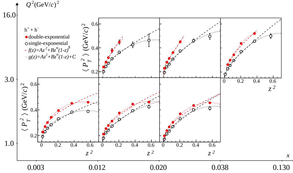
FIGURE 4.19: \langle P_T^2 \rangle versus z^2 as derived from the double-exponential (closed markers) and from the single-exponential fit (open markers) of the P_T^2 -distributions, measured in seven z bins and summing over the hadron charge, with the indication of the two fit functions.
