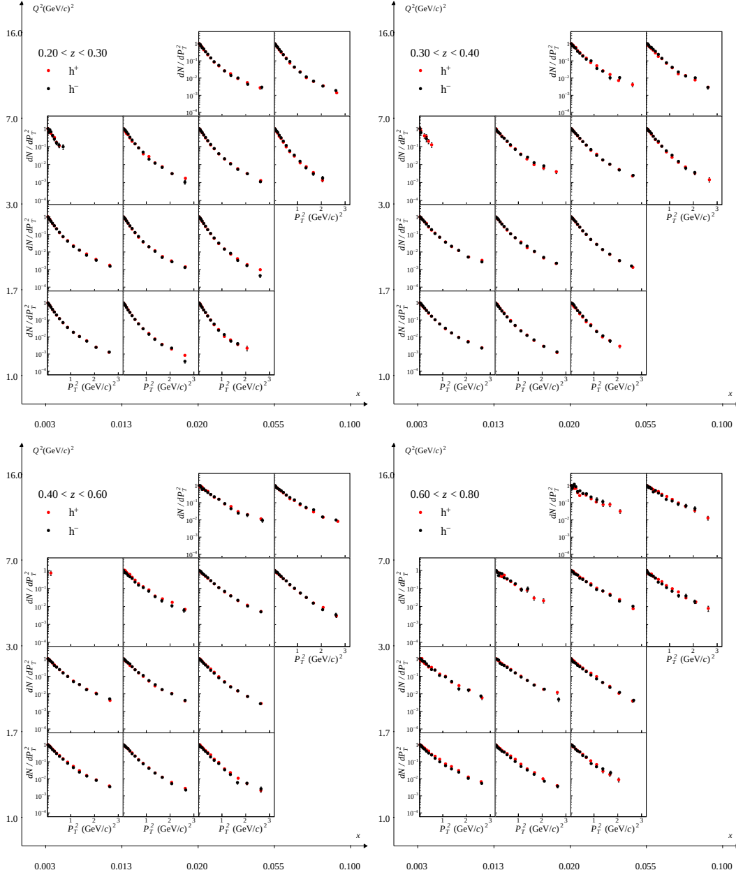
FIGURE 4.24: P_T^2 -distributions for positive (red) and negative hadrons (black) in bins of x (horizontal axis) and Q^2 (vertical axis), in the four z bins.
