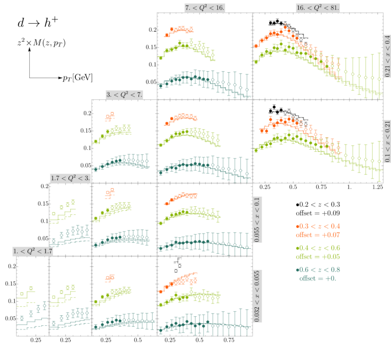
FIGURE 1.10: COMPASS unpolarized multiplicities, multiplied by z^2 and in bins of x , Q^2 , z and P_T , for positive hadrons produced in SIDIS off a deuteron target. The closed (open) points have been included (not included) in the phenomenological analysis. Solid and dashed lines correspond to the theory predictions at different approximation levels: NNLO and N3LO [102].
