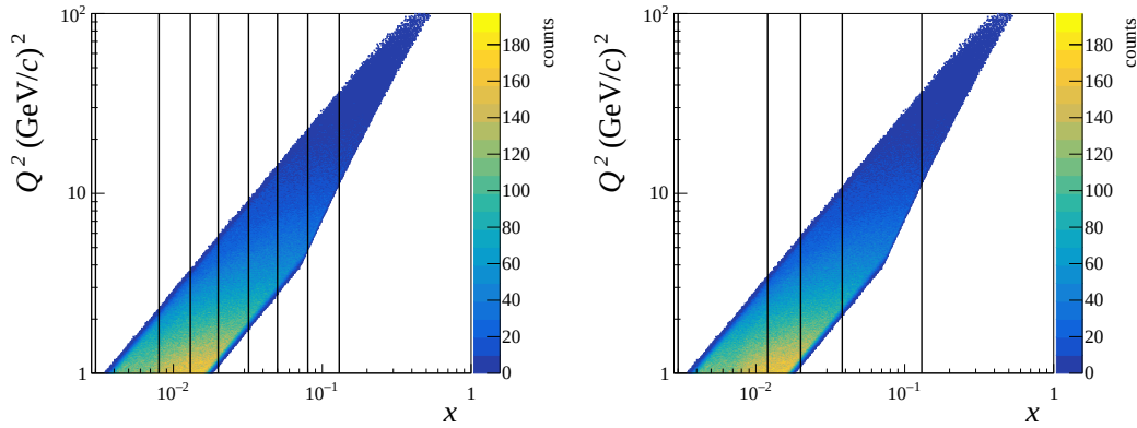
FIGURE 5.1: Drawn on top of the x - Q^2 correlation plot are: the standard binning used for the measurement of the azimuthal asymmetries in 1D (left) and in 3D (right).
