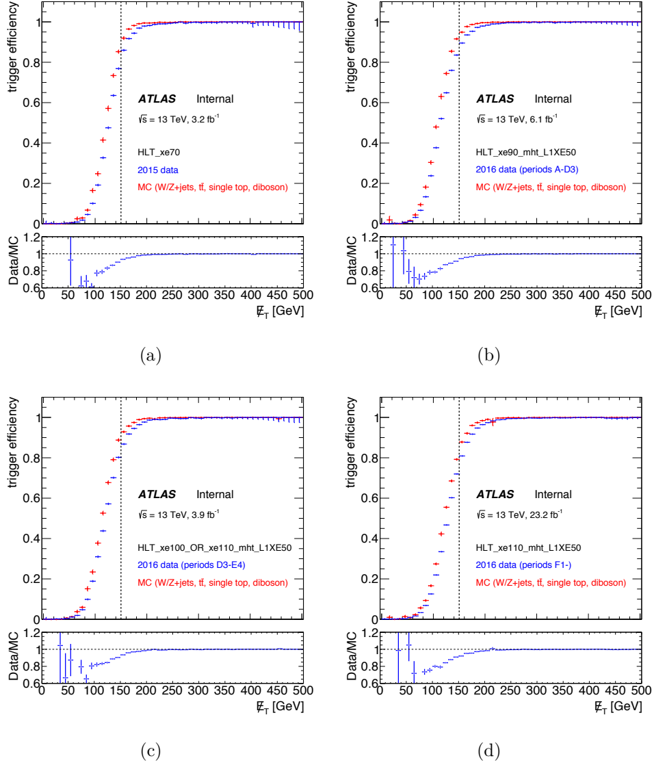
Figure 6.3 – Measured E_T^{\text{miss}} trigger efficiencies and scale factors as function of offline E_T^{\text{miss}} in data and Monte-Carlo simulation for 6.3(a) HLT_xe70, 6.3(b) HLT_xe90_mht_L1XE50, and 6.3(c) HLT_xe100_mht_L1XE50 OR HLT_xe110_mht_L1XE50, and 6.3(d) HLT_xe110_mht_L1XE50 triggers are shown. The plots are shown for 0,1 and 2 tags together. The MC is dominated by W +jet and t\bar{t} events [233].
