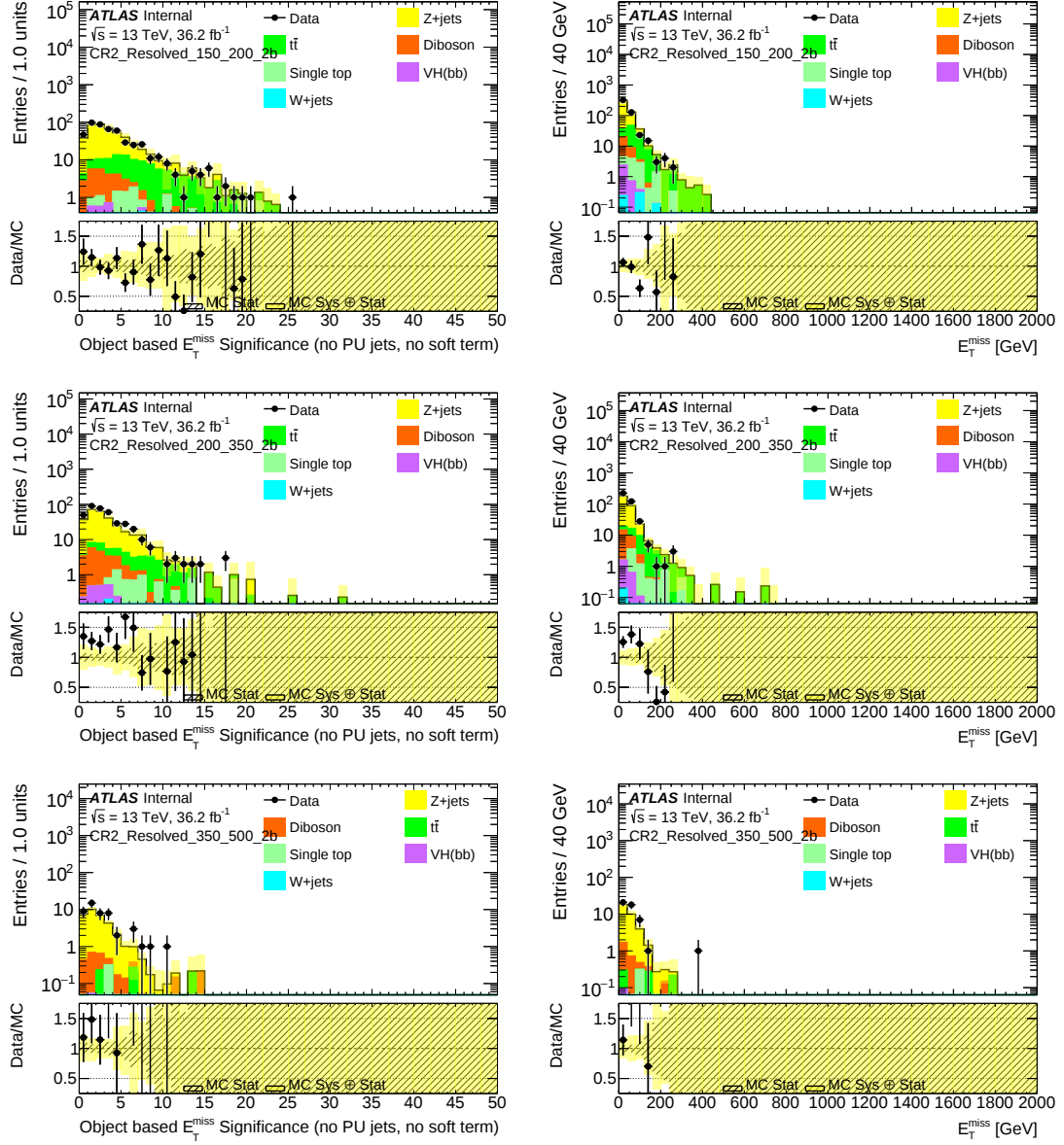
Figure 8.18 – Object-based E_T^{\text{miss}} significance (left) and E_T^{\text{miss}} (right) distributions for data and MC simulation in the 2 lepton control region, without the event-based E_T^{\text{miss}} significance applied in event selection, for events with 2 b-tagged jets in different E_T^{\text{miss}} categories in the resolved regime. Band of the bottom panels includes both systematic and statistical uncertainties. The mismodeling at low E_T^{\text{miss}} values is due to a missing Z(\mu\mu) + \text{jets} MC sample.
