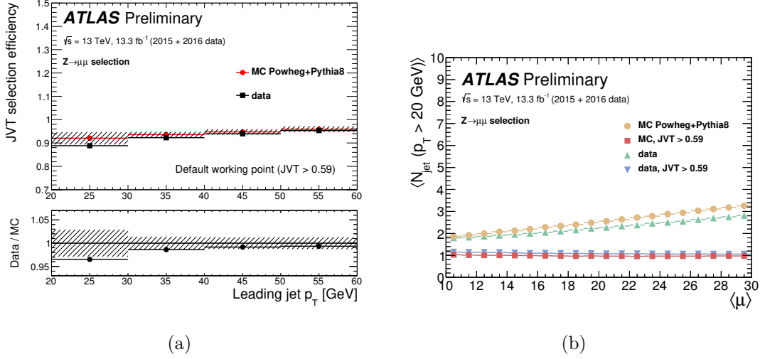
Figure 4.3 – Medium JVT working point. 4.3(a) Hard-scatter jet selection efficiency, in Powheg+Pythia8 MC and in 2015+2016 data, of a \text{JVT} > 0.59 cut on a jet balanced against a Z boson decaying to muons. The uncertainties shown are the statistical uncertainty summed in quadrature with the systematic uncertainty, evaluated varying the residual contamination from pileup jets by 20%. 4.3(b) The average number of jets with p_T > 20 \text{ GeV} in Powheg+Pythia8 MC and in 2015+2016 data before and after a cut of \text{JVT} > 0.59 , as a function of the average number of interactions per bunch crossing.
