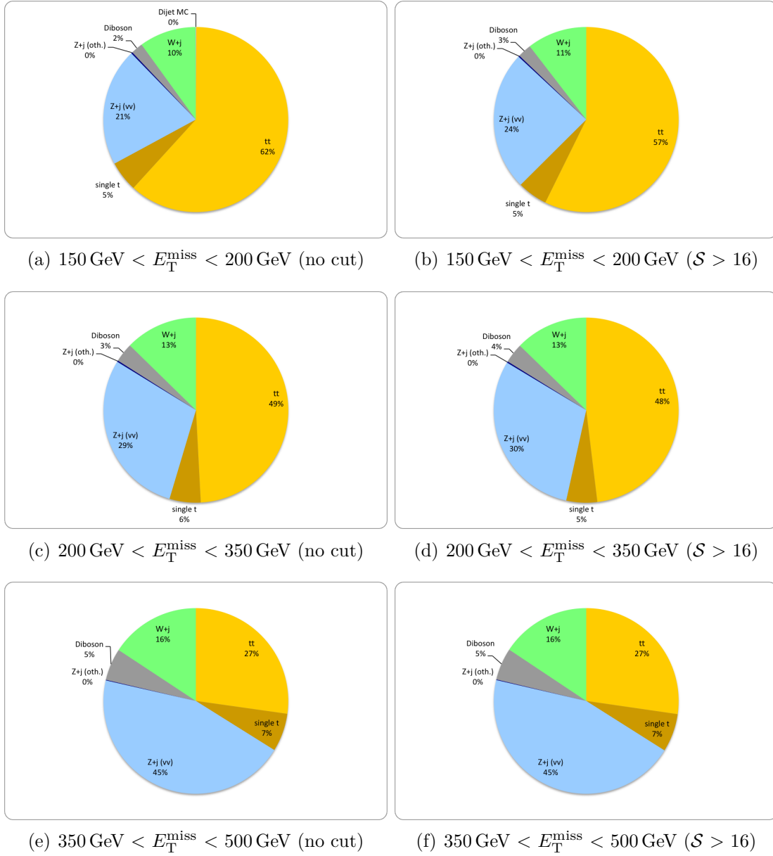
Figure 8.17 – Background composition in the three resolved event selection E_T^{\text{miss}} bins for events with 2 b-tagged jets, without (left) and with E_T^{\text{miss}} significance > 16 requirement (right) in the signal region.
