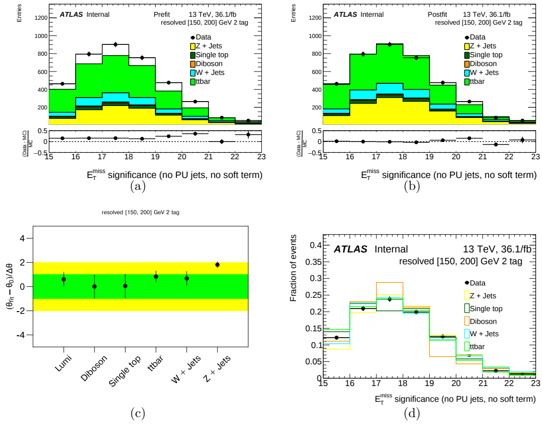
Figure G.6 – Fit results for the 150 GeV < E_T^{\text{miss}} < 200 GeV, 2-btag region (a) Pre-fit distribution (b) Post-fit distribution (c) Pulls and constraints for background normalisations (d) Comparison of shapes for different simulated backgrounds
