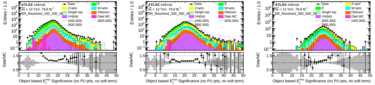
Figure 8.9 – E_T^{\text{miss}} significance distribution for events with 2 b -tagged jets in the regions with 150\text{ GeV} < E_T^{\text{miss}} < 200\text{ GeV} (left), 200\text{ GeV} < E_T^{\text{miss}} < 350\text{ GeV} (middle), 350\text{ GeV} < E_T^{\text{miss}} < 500\text{ GeV} (right). Only statistical uncertainties are taken into account for displaying the uncertainty bands. The signal distributions overlayed are normalised to 1 pb.
