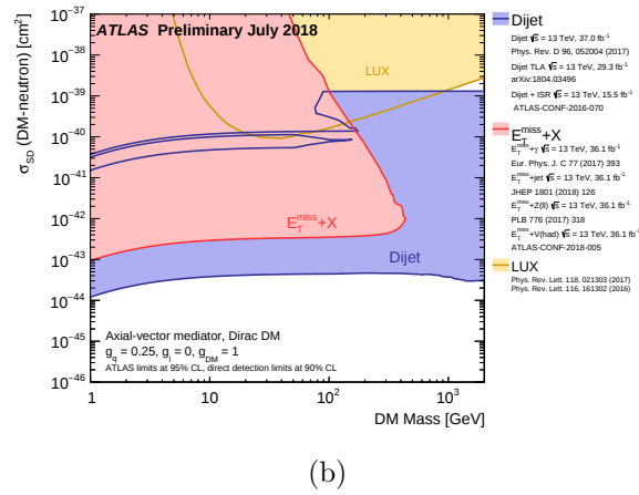
Figure 2.9 – Comparison of the inferred limits to the constraints from direct detection experiments on the spin-dependent WIMP-neutron scattering cross section for the 2.9(a) vector mediator and the 2.9(b) axial-vector mediator. LHC limits are shown at 95% CL and direct detection limits at 90% CL. The comparison is valid solely in the context of these models with the shown specific couplings. LHC searches and direct detection experiments exclude the shaded areas.
