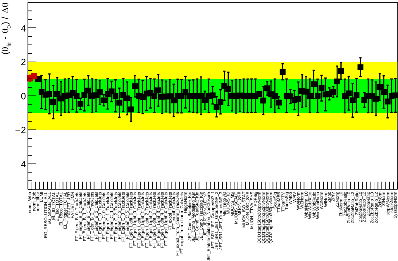
Figure 7.3 – The nuisance parameter pulls for the fit to the observed data in the sidebands of the discriminating variable, assuming \mu = 0 . The major background normalisations are summarized in Table 7.3 [233].
