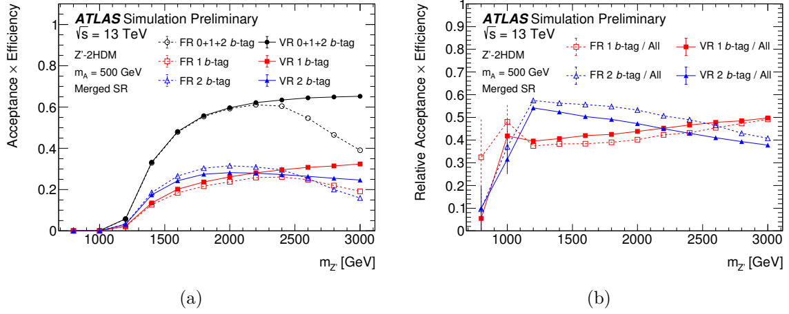
Figure 8.5 – (a) Acceptance \times efficiency ( A \times \epsilon ) for different b -tag multiplicities as a function of m_{Z'} in a Z' -2HDM model with m_A = 500 GeV, \tan \beta = 1.0 , g_Z = 0.8 , m_\chi = 100 GeV, and m_H = m_{H^\pm} = 300 GeV, for events with E_T^{\text{miss}} > 500 GeV (merged SR) when using FR track jets (open symbols, dashed lines) and VR track jets (filled symbols, solid lines). The selection includes a requirement to have at least two track jets associated to the large- R jet, and requires a minimum angular separation of the two leading track jets, as described in Appendix E. The combined A \times \epsilon for events with either 0, 1 or 2 b -tagged jets is drawn with circular markers, while triangular and square markers correspond to the individual A \times \epsilon for 1 and 2 b -tag(s), respectively. (b) Relative A \times \epsilon for different b -tag multiplicities with the same Z' -2HDM model and selections. The A \times \epsilon for 1 b -tagged and 2 b -tagged events are normalised to the sum of events with either 0, 1 or 2 b -tagged jets (“All”), as obtained for each track jet choice individually [259].
