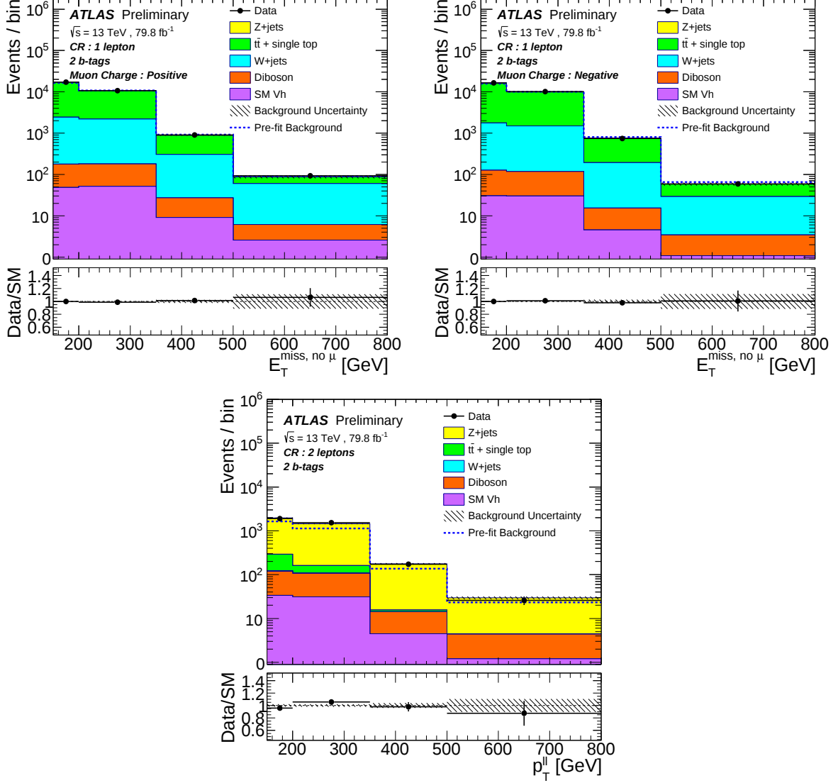
Figure 8.21 – Distributions of E_{T,\text{no}\mu}^{\text{miss}} in the 1\mu -CR (top) and p_T^{\ell\ell} in the 2\ell -CR (bottom). The distribution of the 1\mu -CR is shown for events with positively (left) and negatively (right) charged muons separately. The distributions in the the 1\mu -CR are separated by the muon charge because the fit uses the muon charge as the discriminating variable to separate the t\bar{t} process from the W + \text{jets} process. The upper panels show a comparison of data to the SM expectation before (dashed lines) and after the background-only fit (solid histograms). The bottom panel displays the ratio of data to SM expectations after the background-only fit, with its systematic uncertainty considering correlations between individual contributions indicated by the hatched band. The rightmost bin includes overflows [5].
