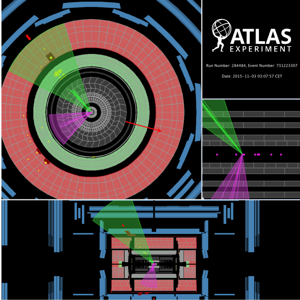
Figure 6.1 – An event display of a signal event in the resolved signal region. This event is characterized by E_T^{\text{miss}} = 213 GeV, red arrow, and two b-tagged small-R calorimeter jets, green and purple cones, that form a dijet system with m_{jj} = 120 GeV.
