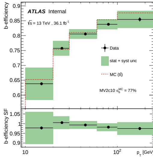
Figure E.1 – b -tagging efficiency (top) estimated in data (black symbols) and a t\bar{t} simulation (dashed red line) and the resulting b -tagging scale factors (bottom) obtained for the 77% efficiency working point. The error band (green) includes both statistical and systematic uncertainty.
