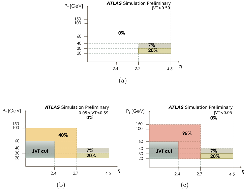
Figure 5.1 – Scheme of the regions in p_T and \eta of the jet with the corresponding percentage representing the fraction of jets originating from pile-up interactions. The regions shown are for (a) \text{JVT} > 0.59 , (b) 0.05 \leq \text{JVT} \leq 0.59 , and for (c) \text{JVT} < 0.05 . Bin values are used as-is with no interpolation performed across boundaries.
