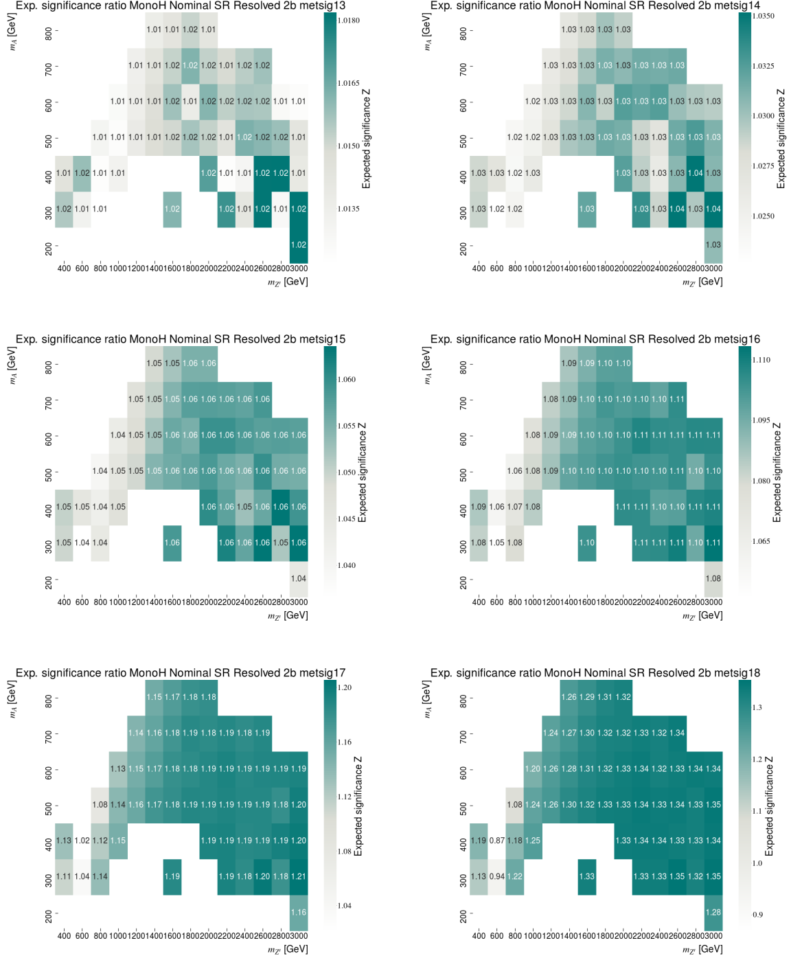
Figure 8.12 – Ratio of expected signal significance (taking into account the limited background MC statistics) with \mathbf{E}_T^{\text{miss}} significance cut varied from 13 to 18 with respect to no cut for events with 2 b-tagged jets.
