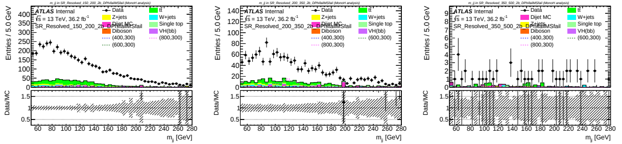
Figure 8.22 – Higgs boson candidate mass distribution for data recorded during 2015 and 2016 and MC simulation in the QCDCR. Selected events has exactly 2 b-tagged jets and 150 \text{ GeV} < E_T^{\text{miss}} < 200 \text{ GeV} (left), 200 \text{ GeV} < E_T^{\text{miss}} < 350 \text{ GeV} (middle), and 350 \text{ GeV} < E_T^{\text{miss}} < 500 \text{ GeV} (right) in the QCDCR.
