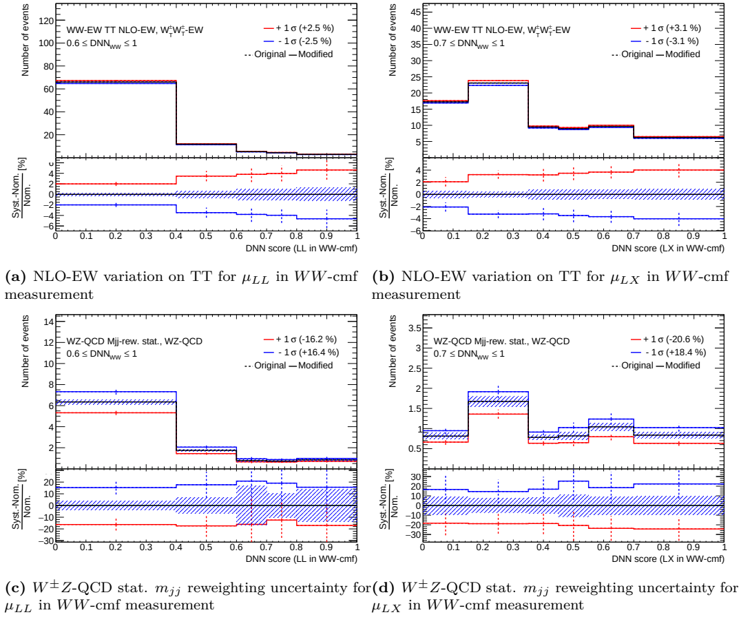
Figure 12.15: The systematic uncertainty of the NLO-EW correction on the TT polarization state and the statistical uncertainty of the m_{jj} reweighting of the W^\pm Z -QCD background. The variations are shown in the signal region histogram with 0.6 < \text{DNN}_{W^\pm W^\pm}\text{-score} \leq 1 for the LL measurement and 0.7 < \text{DNN}_{W^\pm W^\pm}\text{-score} \leq 1 for the LX measurement.
