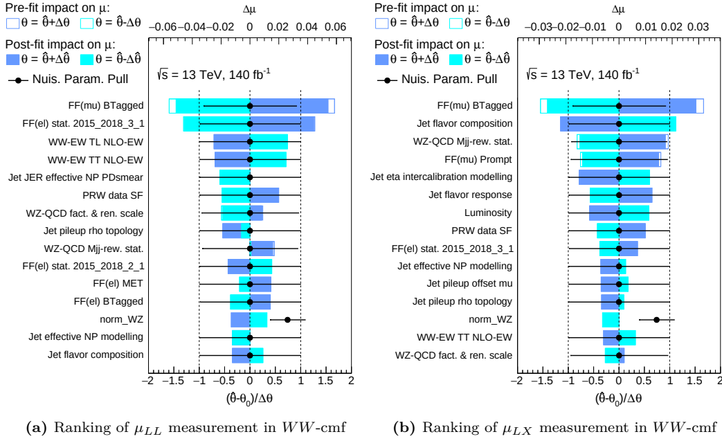
Figure 12.16: The ranking plots of the partially unblinded fiducial cross-section fits in the WW -cmf. The fit is derived for measured data in the W^\pm Z control region and Asimov data in the signal and Low- m_{jj} control region. The W^\pm Z -QCD contribution in the Asimov data is scaled by 0.74.
