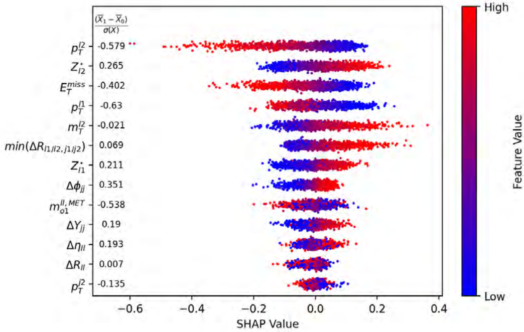
Figure 10.11: The SHAP values of the polarization DNNs trained in pp-cmf are plotted with a color encoding the value of the corresponding feature. In addition, it is also listed how much the mean values of the features in LL/LX-polarization \bar{x}_1 and TX/TT-polarization \bar{x}_0 differ.
