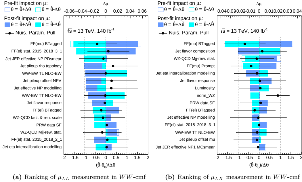
Figure 12.24: The ranking plots for the measured fiducial cross-section fits in the WW -cmf.
