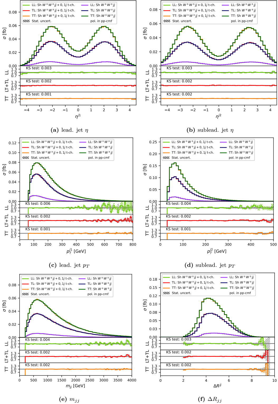
Figure B.12: Comparison of the polarization in pp-cmf simulated by SHERPA W^\pm W^\pm jj and W^\pm W^\pm jj (t-ch.) in jet kinematic on particle-level in the combined signal and Low- m_{jj} region defined in table 8.2. The SHERPA W^\pm W^\pm jj is corrected by the DNN_{0,1j}^{pol} . To avoid a bias the networks are applied in the k-fold method to the corresponding validation data used during their training.
