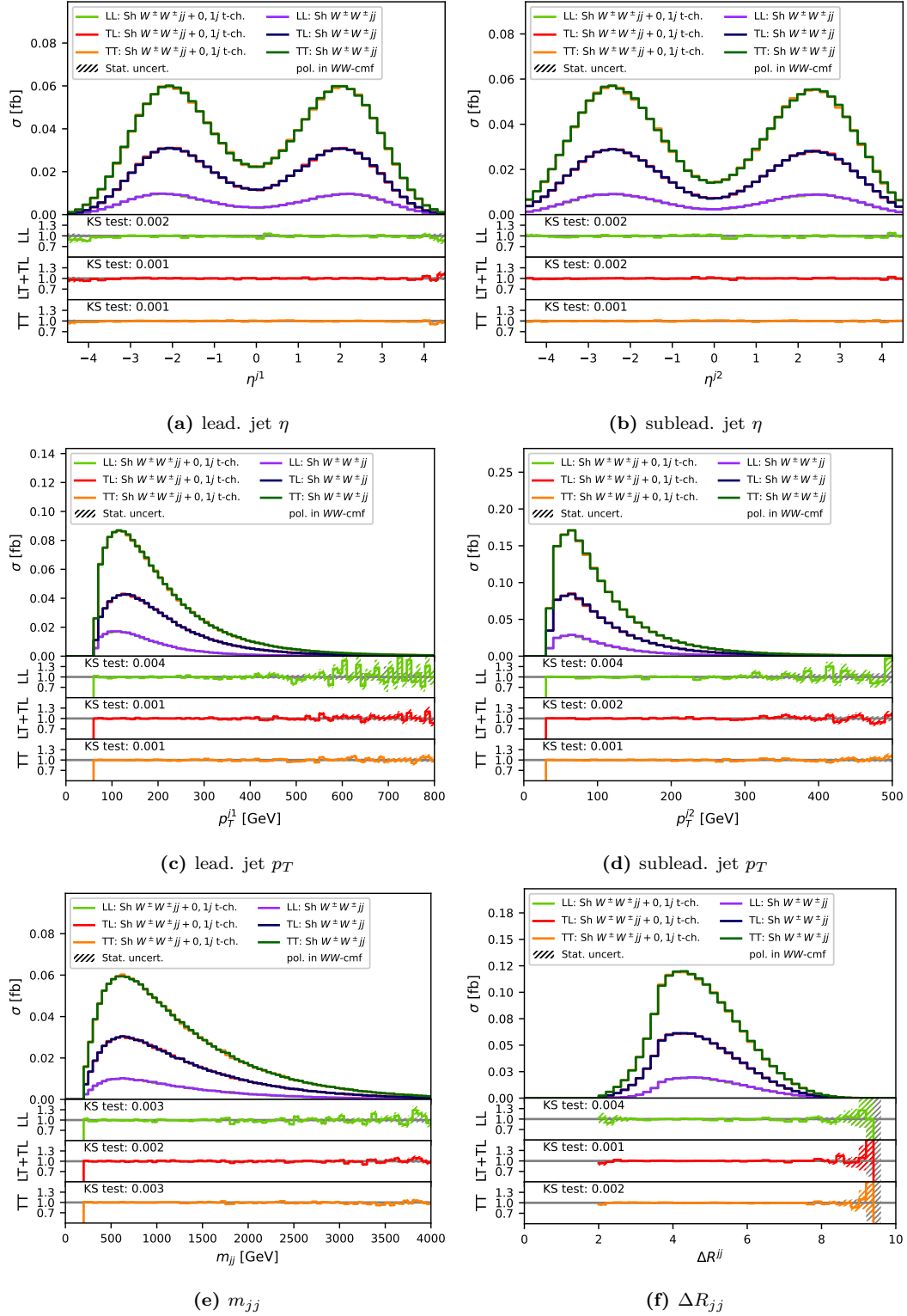
Figure B.10: Comparison of the polarization in WW-cmf simulated by SHERPA W^\pm W^\pm jj and W^\pm W^\pm jj (t-ch.) in jet kinematic on particle-level in the combined signal and Low- m_{jj} region defined in table 8.2. The SHERPA W^\pm W^\pm jj is corrected by the DNN _{0,1j}^{poll} . To avoid a bias the networks are applied in the k-fold method to the corresponding validation data used during their training.
