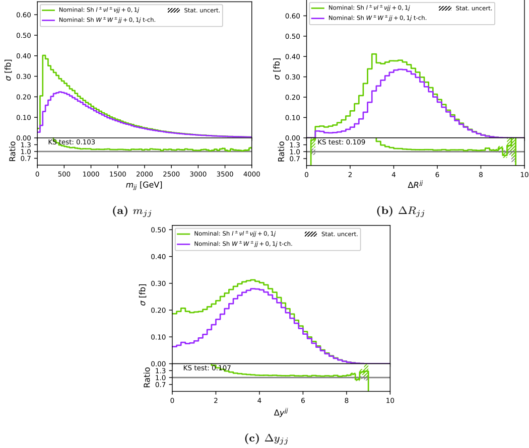
Figure 8.6: Comparison of the differential cross-sections simulated by SHERPA W^\pm W^\pm jj + 0, 1j (t-ch.) and l^\pm l^\pm \nu jj + 0, 1j on particle-level in the phase space defined in table 8.4.
