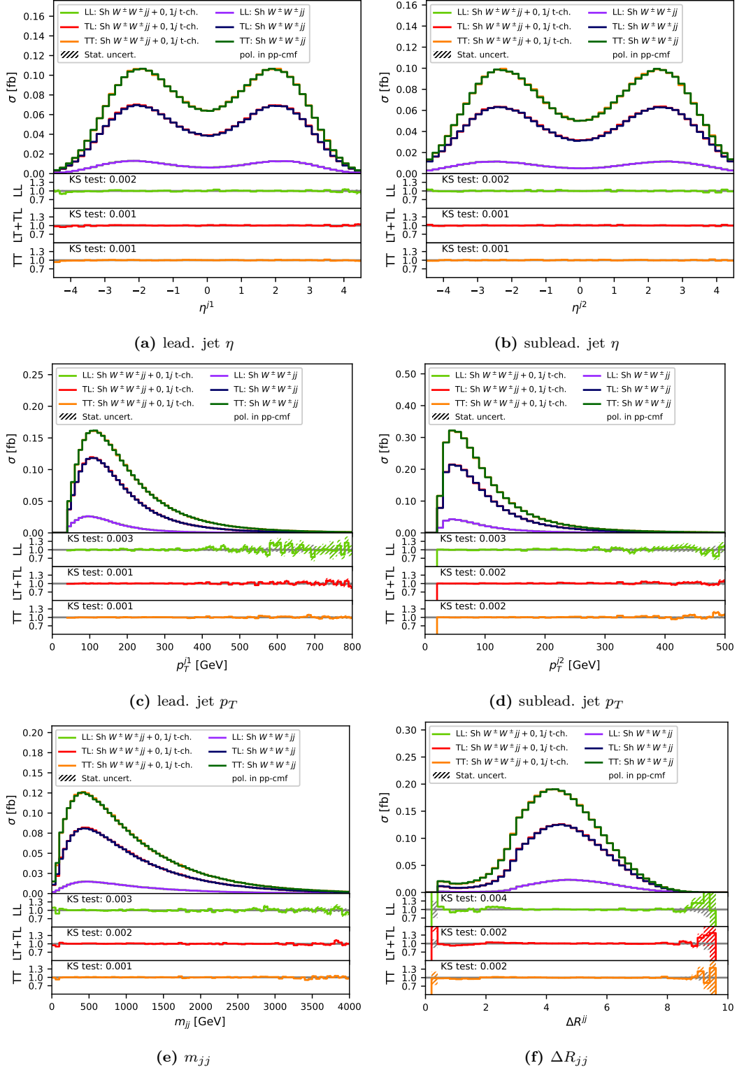
Figure B.6: Comparison of the polarization in pp-cmf simulated by SHERPA W^\pm W^\pm jj and W^\pm W^\pm jj (t-ch.) on particle-level in the phase space defined in table 8.4. The SHERPA W^\pm W^\pm jj is corrected by the DNN_{0,1j}^{poll} . To avoid a bias the networks are applied in the k-fold method to the corresponding validation data used during their training.
