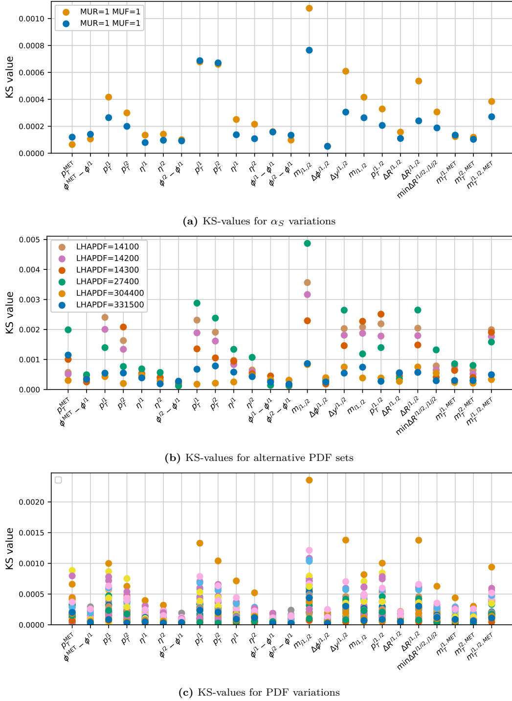
Figure F.1: Kolmogorov Smirnov test between the nominal SHERPA l^\pm \nu l^\pm \nu jj + 0, 1j sample and the corresponding \alpha_S , PDF set, and internal PDF variations. The kinematic distributions are derived on particle-level in the combined signal and Low- m_{jj} region defined in table 8.2.
