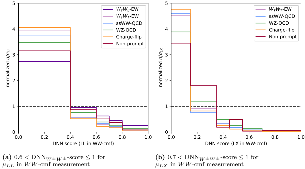
Figure 12.14: The shape of the W^\pm W^\pm jj -QCD, W^\pm Z -QCD, charge-flip, and non-prompt background compared to the LL/LX signal of the polarization measurement in the WW-cmf. The shape differences are evaluated in the signal region histogram with the highest \text{DNN}_{W^\pm W^\pm} score.
