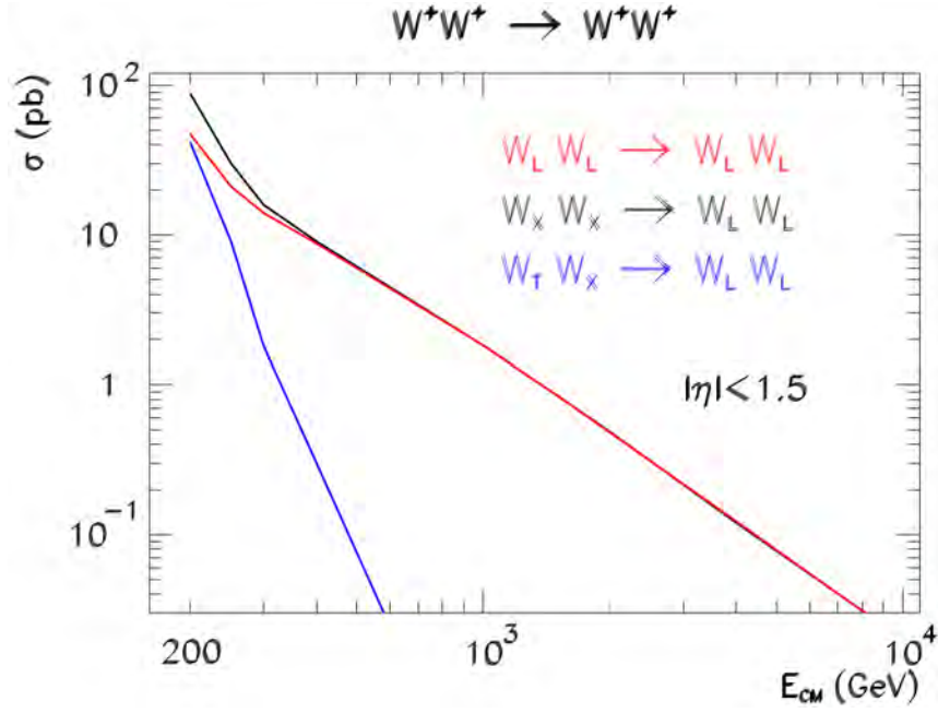
Figure 3.3: "Total W^+W^+ \rightarrow W_L^+W_L^+ scattering cross-sections in the SM as a function of the center-of-mass energy. Shown are the individual contributions of different initial polarization states to the final state consisting of purely longitudinal W_L^+W_L^+ pairs. Subscript X denotes any polarization ( T or L ). Assumed are two on-shell, unpolarized, colliding W^+ beams. A cut on the scattering angle that corresponds to pseudorapidity of \pm 1.5 with respect to the incoming W direction was applied. Results of MadGraph calculations." [43]
