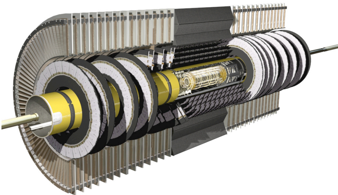
Figure 4.10: 3D schematic of the ATLAS inner detector. Taken from [75].
