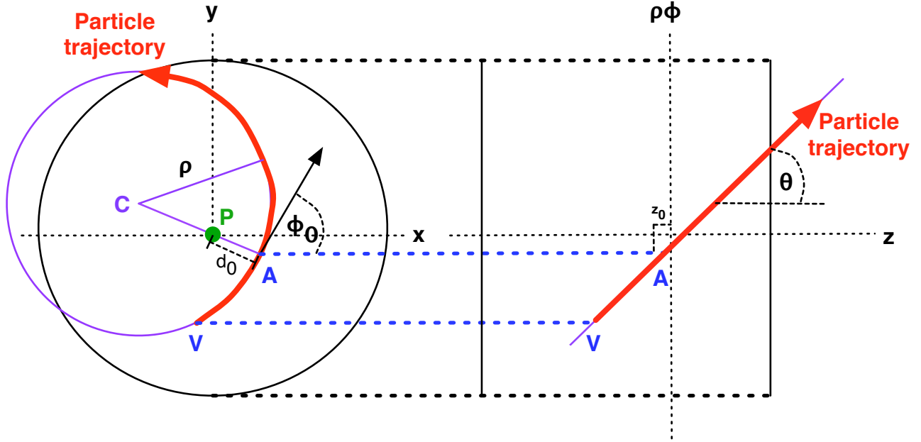
Figure 5.8: The ATLAS track helix parameters. Based on [65].
