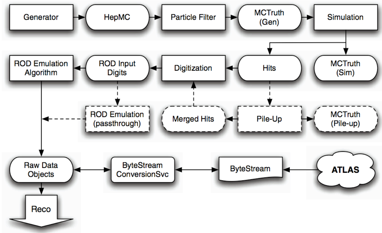
Figure 5.9: The ATLAS simulation chain from event generation to reconstruction. Sharp-cornered boxes indicate processing steps; round-cornered boxes represent data object types. The detector itself is also represented. Taken from [29].
