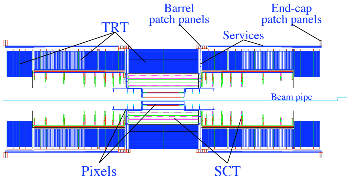
Figure 4.8: 2D schematic of the ATLAS inner detector, rz projection. Taken from [72].
