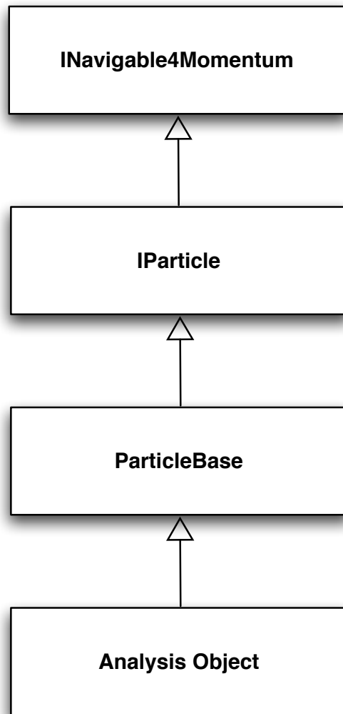
Figure 5.10: The AOD class inheritance diagram
