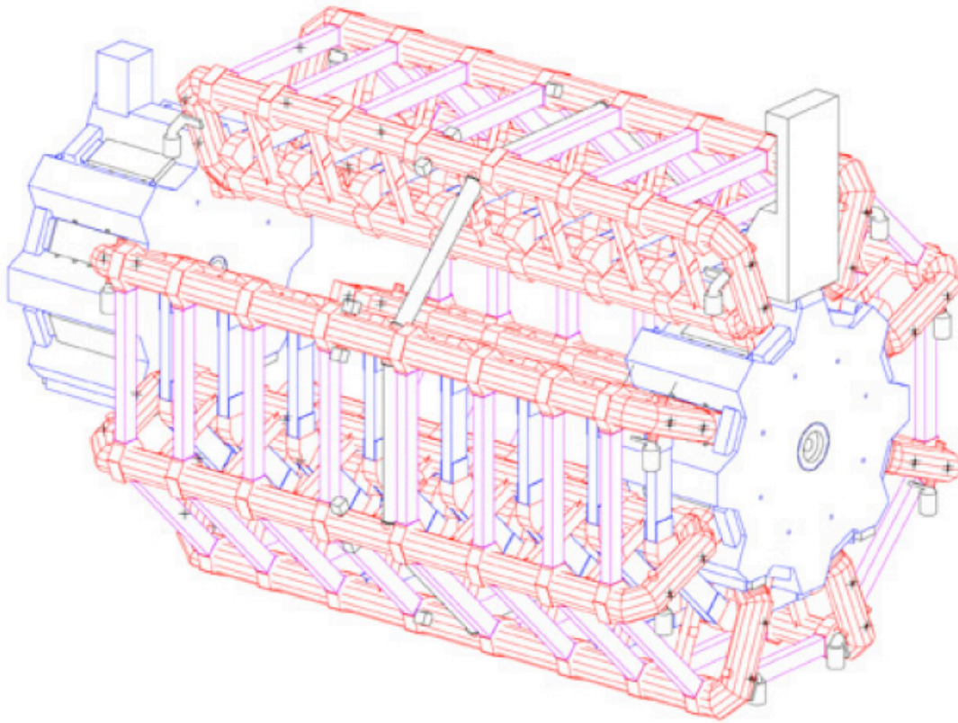
Figure 4.7: The toroid magnet system. Taken from [75]
