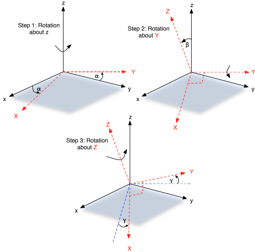
Figure 3.1: Construction of an arbitrary rotation through three successive rotations
