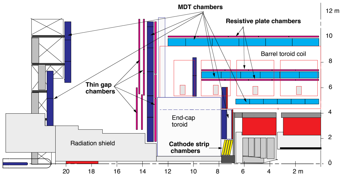
Figure 4.12: View of a single quadrant of the muon spectrometer in the rz projection. Taken from [74].
