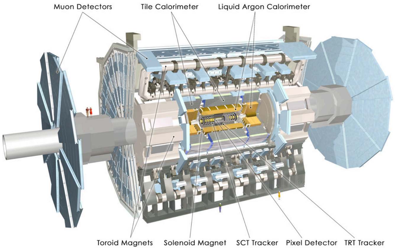
Figure 4.6: The ATLAS detector. Taken from [75]
