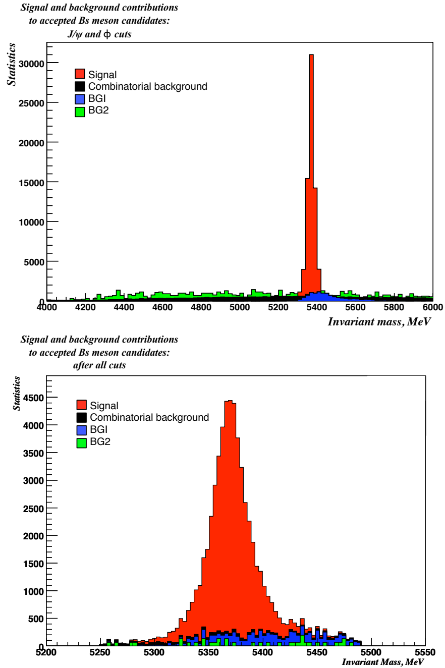
Figure 7.7: Contributions to the B_s^0 candidates from the signal and background, after the \phi and B_s^0 cuts (the J/\psi cuts are implicit). Note that the real backgrounds have been scaled up according to cross section, for illustrative purposes. The final histogram is a stack of the different contributions, as opposed to the others which are overlaid.
