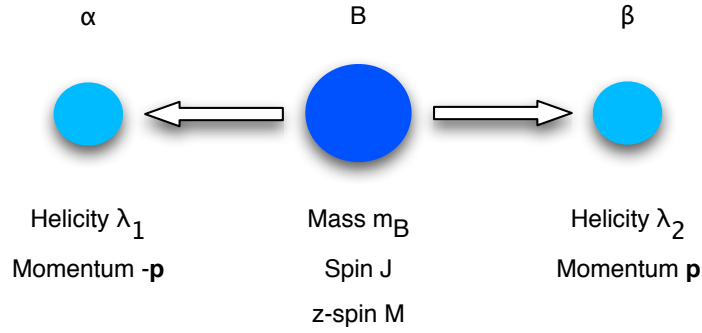
Figure 3.3: Two-body decay
