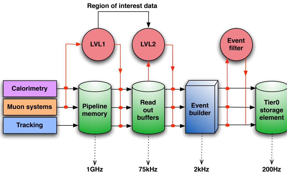
Figure 4.15: Simplified flow diagram for the ATLAS trigger
