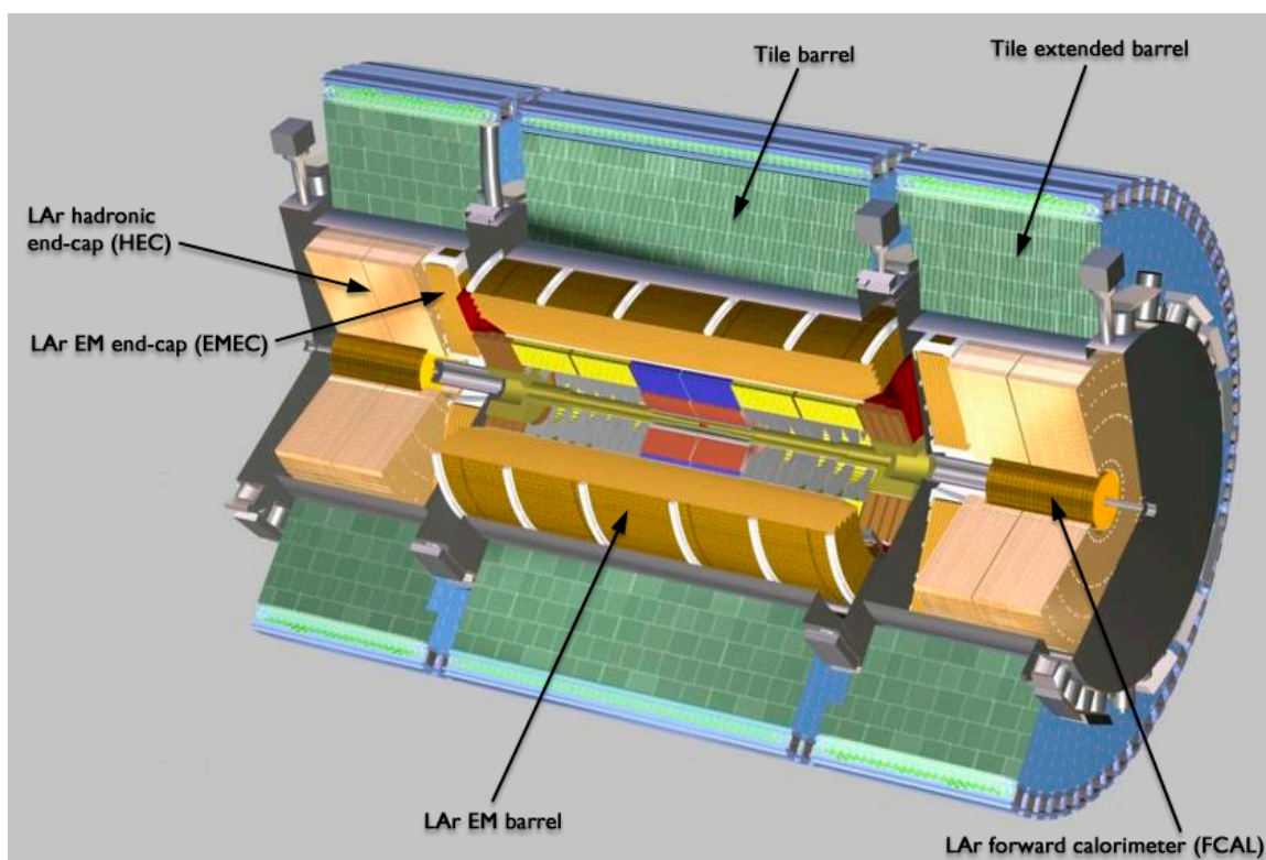
Figure 4.11: 3D schematic of the ATLAS calorimetry. Taken from [75].
