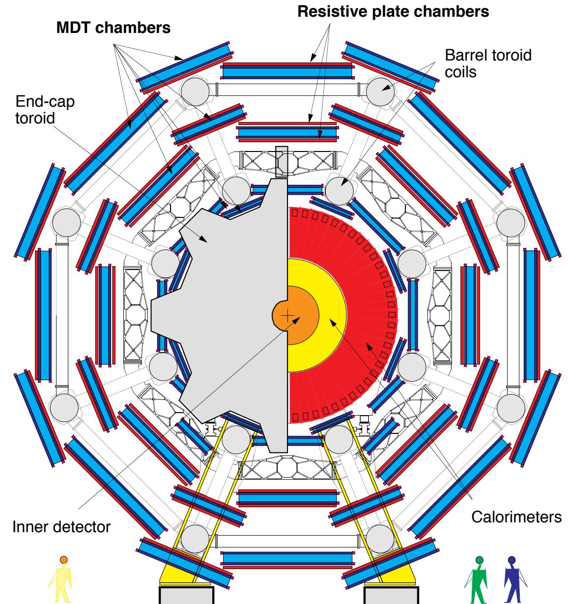
Figure 4.13: View of the muon spectrometer in the xy projection. Taken from [74].
