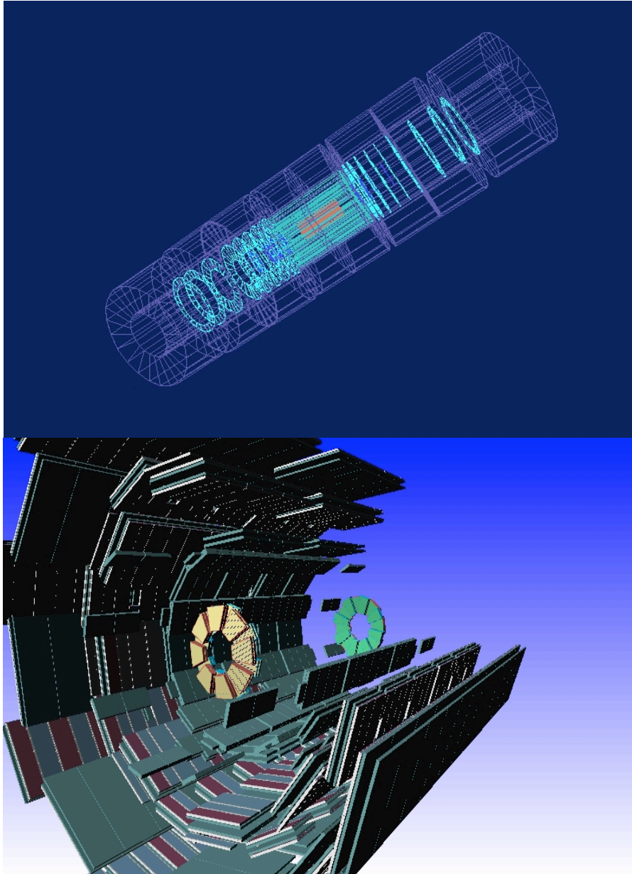
Figure 5.7: Examples of Geant4 visualization technology, showing the ATLAS inner detector and muon systems. Taken from [61].
