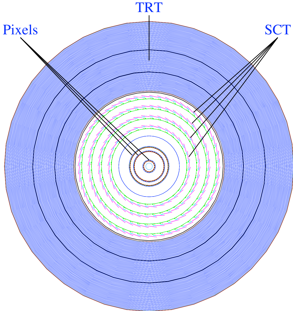
Figure 4.9: 2D schematic of the ATLAS inner detector, r\phi projection. Taken from [72].
