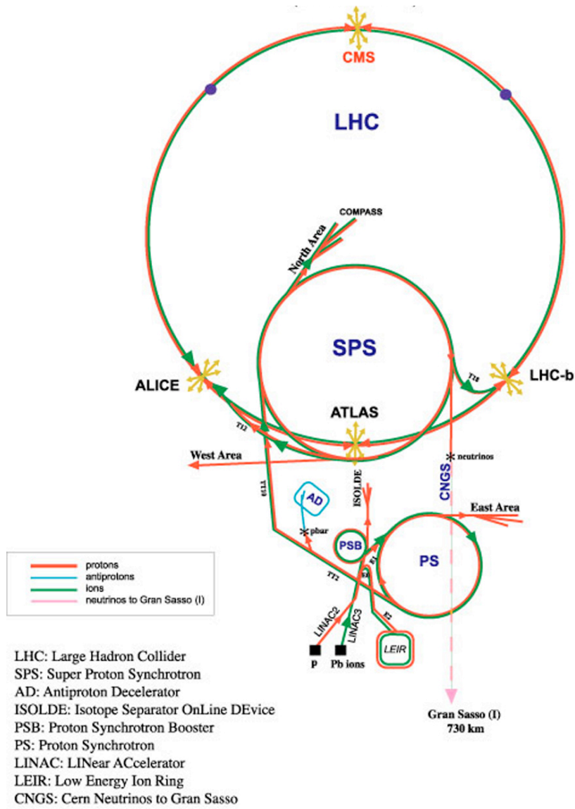
Figure 4.1: The CERN accelerator complex - taken from [75]
