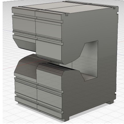
Fig. 1.1b The magnetic blocks (iron yokes) of the PS. This consists of a “closed” followed by an “open” combined function magnet. Taken from [13].
