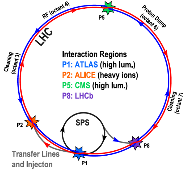
Figure 2.1: Layout of the CERN Large Hadron Collider, showing the interaction regions of the four main LHC experiments and the twin-ring design of the collider, and the accelerator chain. The CMS experiment cave is located beyond access point 5, in Cessy (France).
