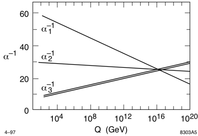
Figure 1.6: Evolution of the SU(3) \times SU(2) \times U(1) gauge couplings as a function of the momentum transfer Q of the scattering process in the MSSM. Prediction obtained using the 1-loop RG equations of the SM. The double line for \alpha_3 is the current experimental error in this quantity, not visible for \alpha_1 and \alpha_2 since it is too small.
