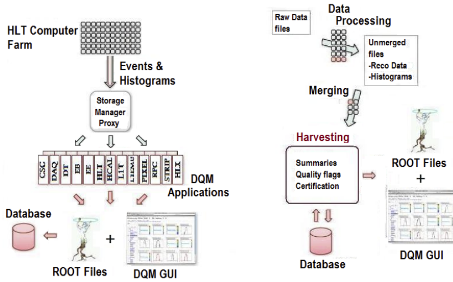
Figure 3.15: DQM workflows for online (left) and offline (right).
