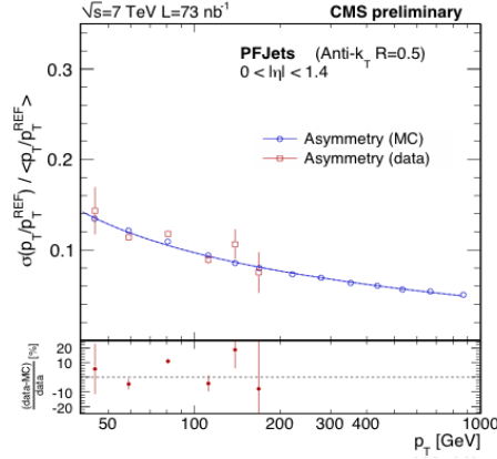
Figure 4.1: Particle-flow jet p_T resolution for jet reconstructed using the anti- k_T algorithm in the region 0 \lesssim \eta \lesssim 1.4 . The asymmetry method is used, for both data (red) and MC (blue).
