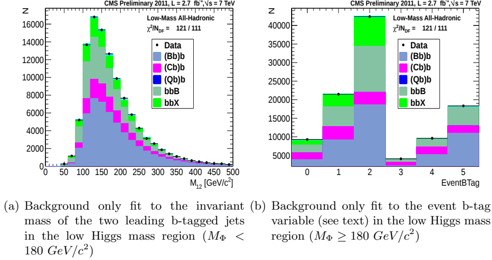
Figure 7.1: Results of the background only fit in data (black dots) using only the background templates (full distributions). The fit is performed in the two dimensional space defined by the invariant mass of the two leading b-tagged jets and the event b-tag variable (see text). The projection of the fit in each variable is shown in the plots. Each background template is indicated in the legend with the corresponding category name, bbx/bxb/xbx (see text), with x = Q, B, C depending on the true flavor assumed for the not b-tagged jet ( Q = \text{light quark/gluon} , B = b - \text{quark} and C = c - \text{quark} ). The bbX template results from the combination of the bbQ and bbC templates.
