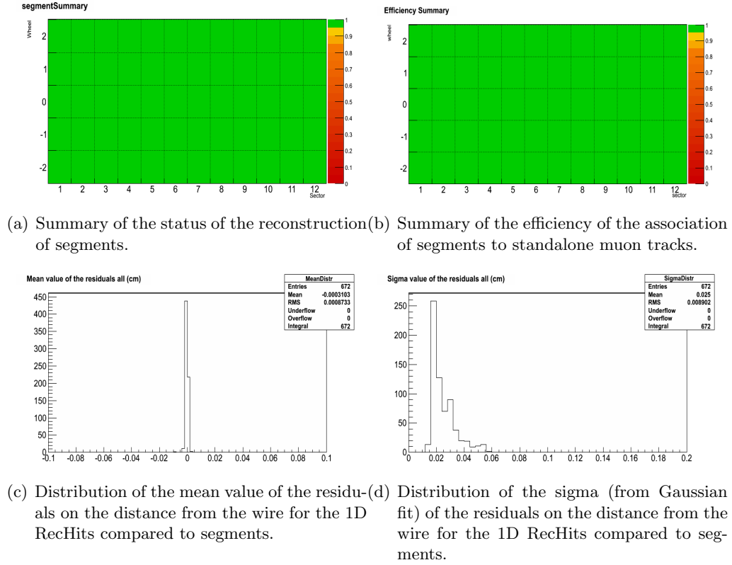
Figure 3.17: Offline monitoring objects showing the summary of the DT subsystem status for a reference run with high statistics taken during 2012 data-taking period. They are two 2D distributions, with the wheel number in the vertical axis and the sector number in the horizontal axis, and two 1D distributions.
