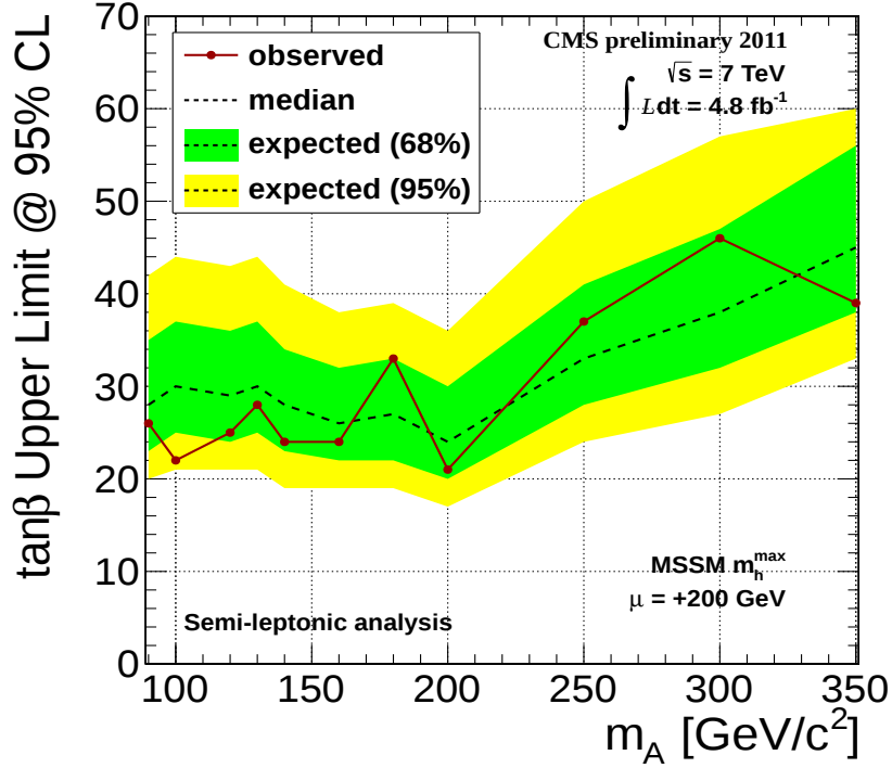
Figure 6.4: The 95% CL upper limits on the \tan\beta , as a function of the pseudo-scalar A mass, in the pp \rightarrow b + \Phi , \Phi \rightarrow b\bar{b} channel, with \Phi = h, H, A . The m_h^{max} is considered as benchmark scenario. These limits correspond to a total amount of data of \mathcal{L} = 4.8 \text{ fb}^{-1} . The red line corresponds to the observed limit in the data. The dashed line is the median expected limit for the background only hypothesis. The green (yellow) band is the range that is expected to contain 68% (95%) of all the observed limit excursions from the median.
