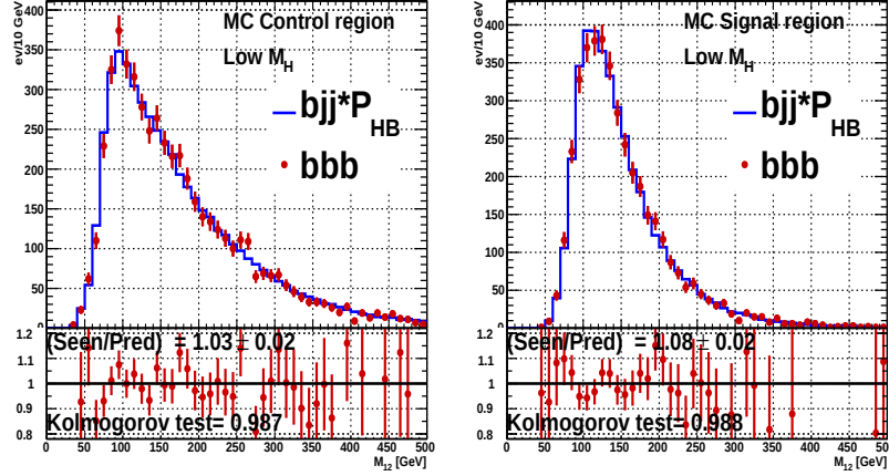
Figure 5.30: Invariant mass of the two leading jets as predicted by the Hyperball method (blue line) compared to the observed distribution (red dots) in QCD Monte Carlo simulated events. The results are shown for low Higgs mass region ( M_H < 200 \text{ GeV}/c^2 ) in control (left) and signal (right) region. The predicted and observed distributions are normalized to the same area, and the ratio between the true events is shown on the bottom of the distributions together with the Kolmogorov test result.
