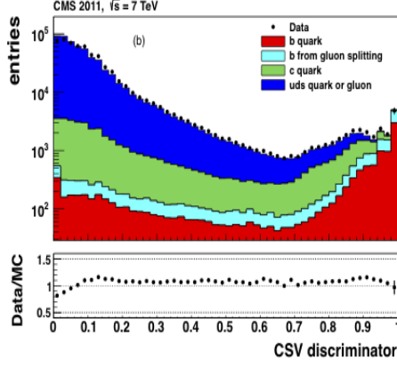
Figure 4.3: Distribution of the CSV b-tagging discrimination variable. The data are compared with the Monte Carlo simulated events split for the different flavor component.
