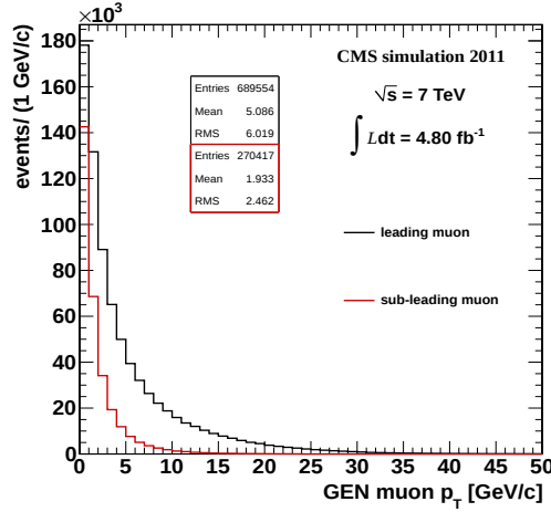
Figure 5.3: Distribution of the p_T for the leading and sub-leading muon from b-quark semi-leptonic decay at generation level.
