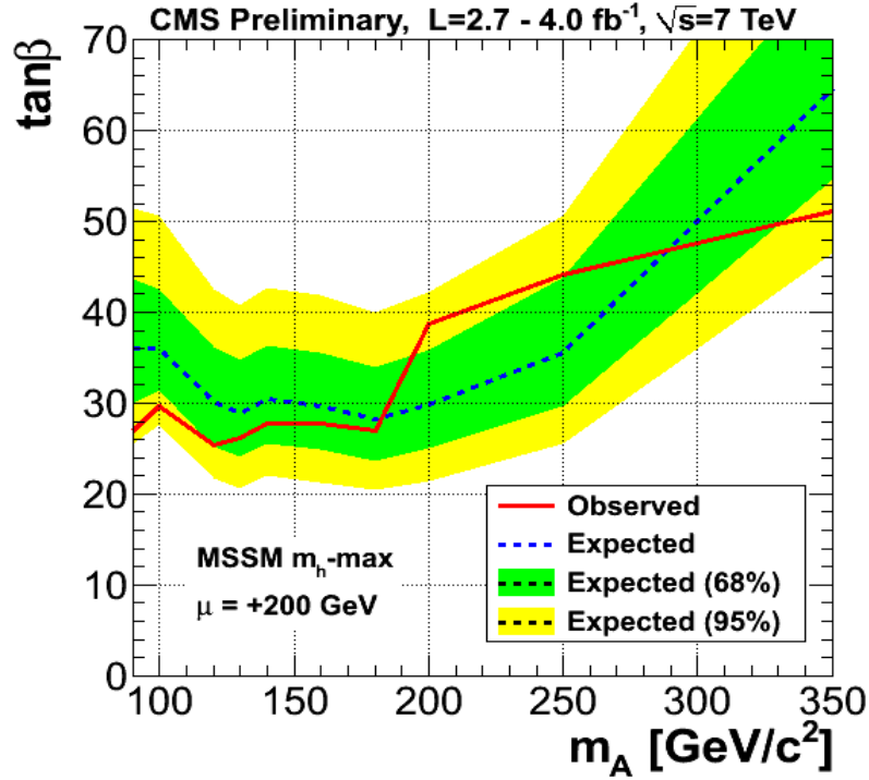
Figure 7.3: The 95% CL upper limits on the \tan\beta , as a function of the pseudo-scalar A mass, in the pp \rightarrow b + \Phi , \Phi \rightarrow b\bar{b} channel ( \Phi = h, H, A ) in the all-hadronic search in the m_h^{max} benchmark scenario. These limits correspond to a total amount of data of \mathcal{L} = 2.7 \text{ fb}^{-1} in the low Higgs mass region and \mathcal{L} = 4 \text{ fb}^{-1} in the medium mass region. The red line corresponds to the observed limit on data. The dashed line is the median expected limit for the background only hypothesis. The green (yellow) band is the range that is expected to contain 68% (95%) of all the observed limit excursions from the median.
