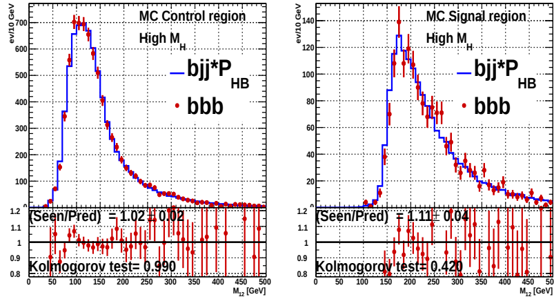
Figure 5.31: Invariant mass of the two leading jets as predicted by the Hyperball method (blue line) compared to the observed distribution (red dots) in QCD Monte Carlo simulated events. The results are shown for high Higgs mass region ( M_H \geq 200 \text{ GeV}/c^2 ) in control (left) and signal (right) region. The predicted and observed distributions are normalized to the same area, and the ratio between the true events is shown on the bottom of the distributions together with the Kolmogorov test result.
