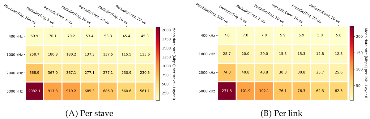
FIGURE H.1: Average data rate per stave/RU (A) and per link (B), simulated for pp in layer 0 of the ITS.
