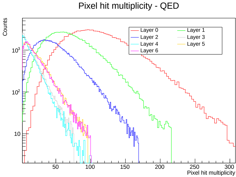
FIGURE D.2: Pixel hit multiplicity of QED event pool for ITS simulations.
