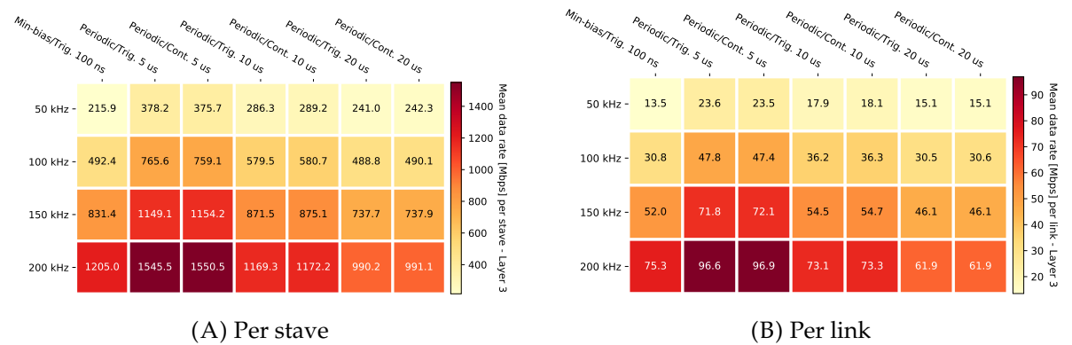
FIGURE 7.14: Simulated data rates for Pb–Pb in layer 3 of the ITS.
