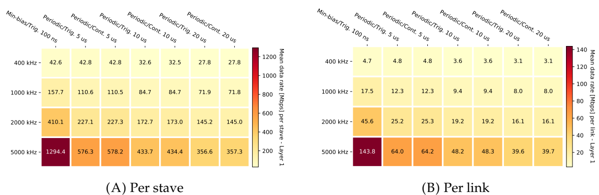
FIGURE H.2: Average data rate per stave/RU (A) and per link (B), simulated for pp in layer 1 of the ITS.
