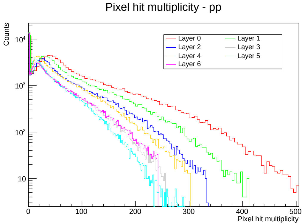
FIGURE D.3: Pixel hit multiplicity of pp event pool for ITS simulations.
