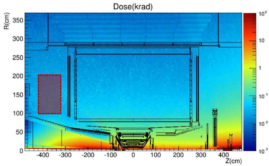
FIGURE 2.15: TID in ALICE for Run 3. The beam-line runs parallel to the Z -axis at R = 0 , and R is the distance from the beam-line. The red box with the dashed lines was added to indicate the position of the crate for the RUs. Source: [32].
