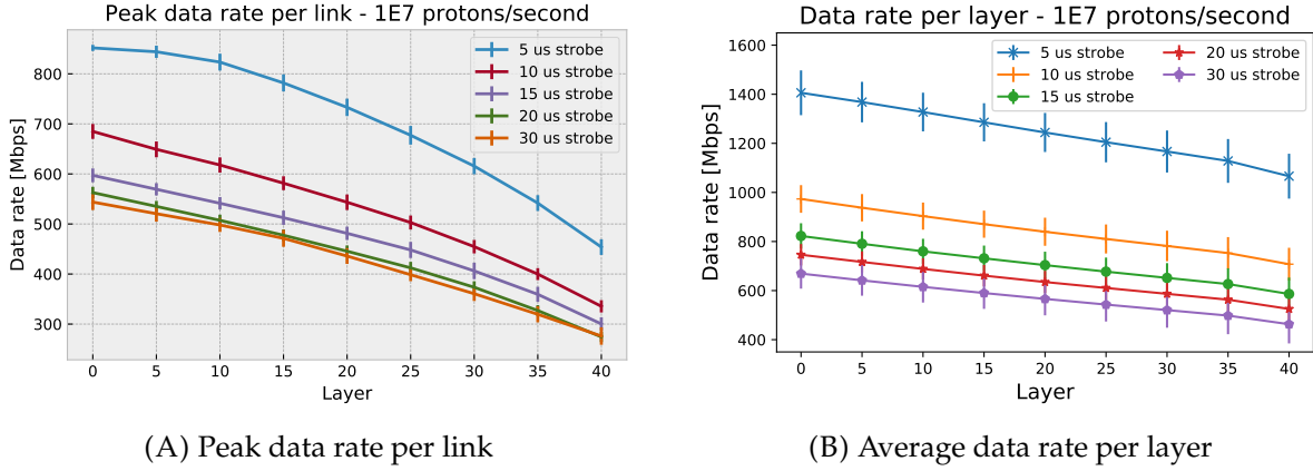
FIGURE 7.21: Simulated data rates for the pCT detector in continuous mode. The peak data rate (A) is the highest rate during a 10 \mu s interval, and the average rate (B) is the average for the whole duration of the simulation. In both cases, the average of all links in a layer is shown, with the error bar indicating the spread in values among the links. Note: The y-axis has been truncated. [36]
