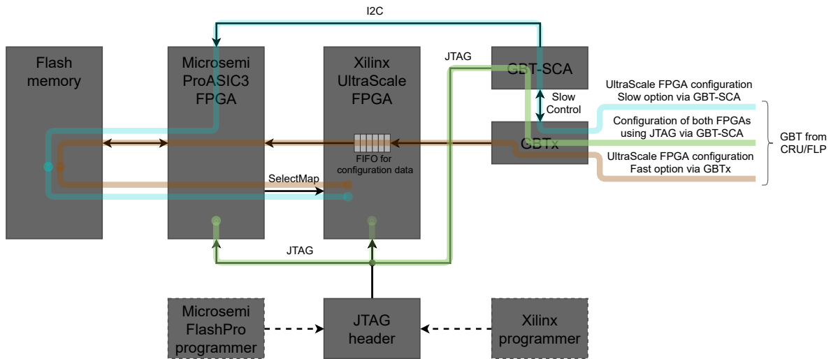
FIGURE 2.19: Readout Unit Configuration Paths for the FPGAs.
