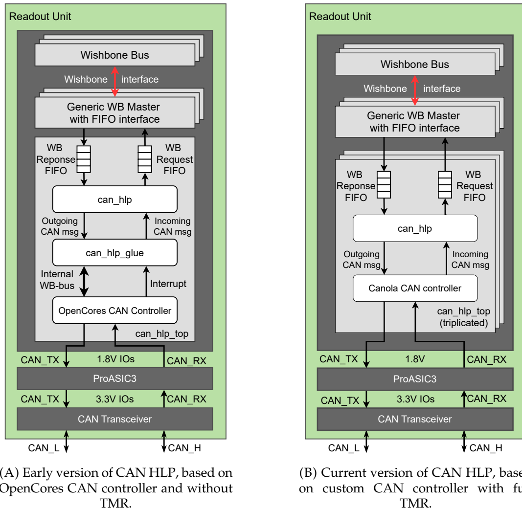
FIGURE 3.7: Implementation of CAN-based interface to the WB bus for DCS.
