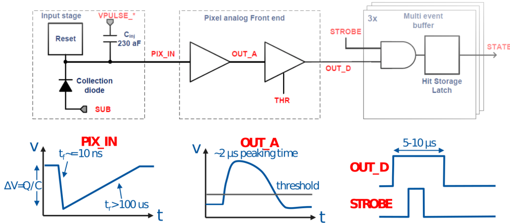
FIGURE B.1: Block diagram of ALPIDE pixel cell [26].
