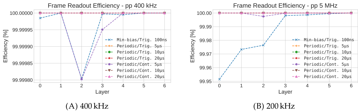
FIGURE 7.6: Frame readout efficiency for ITS in pp simulations [103].
