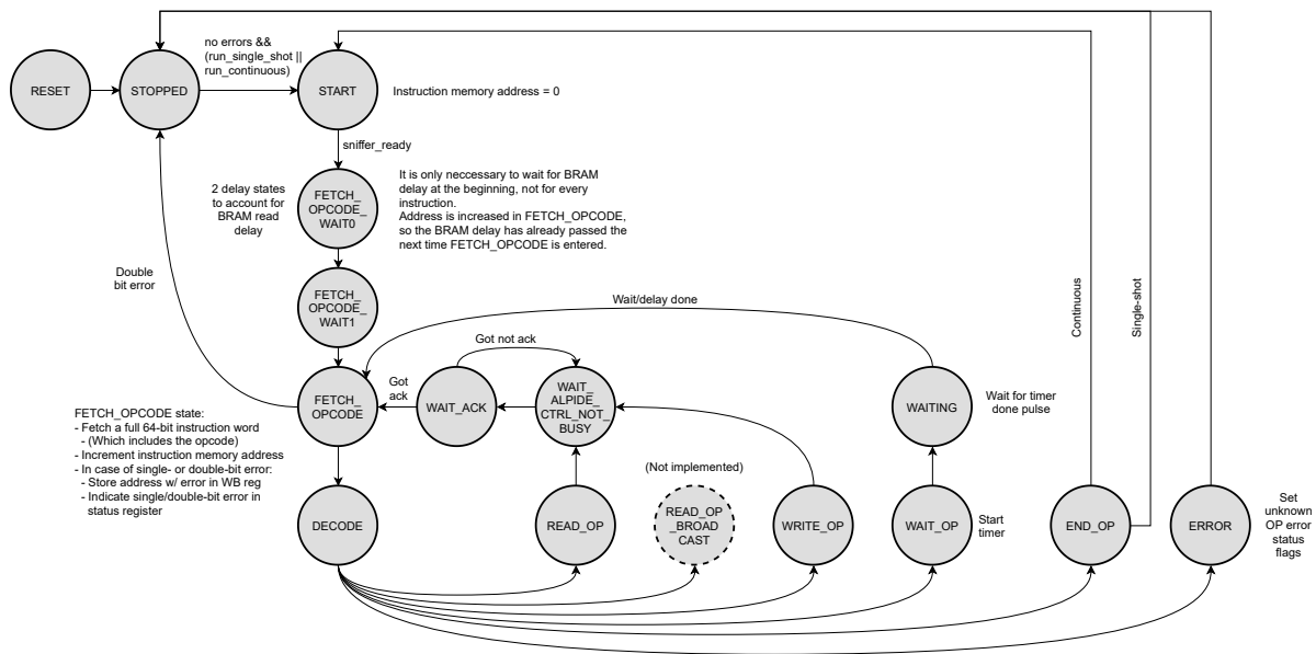
FIGURE 3.10: Alpide Monitor Sequencer FSM Diagram.
