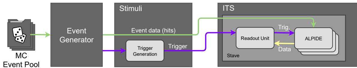
FIGURE 6.4: Overview of SystemC simulation model for ITS.
