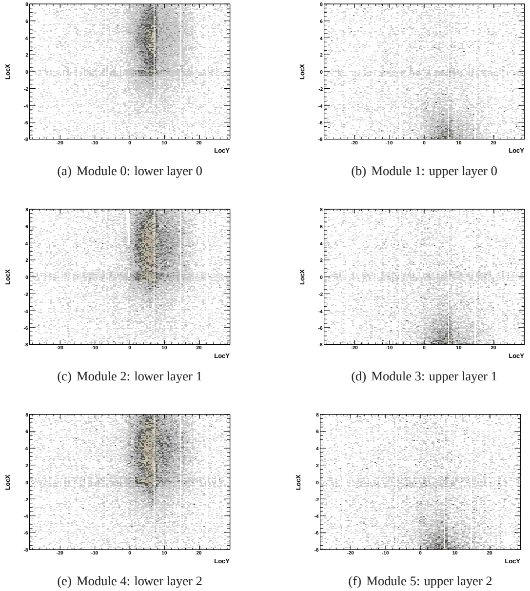
Figure 7.3: Hit maps of the modules using a delay setting of 22 ns. LocX gives the short side of the module in mm and LocY the long side in mm. There was an overlap of 0.2 mm in LocX
