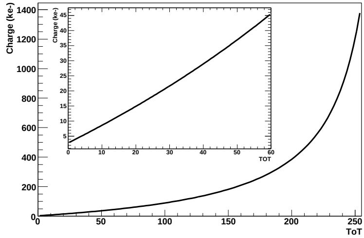
Figure 7.13: A typical relation between the charge and the TOT value.
