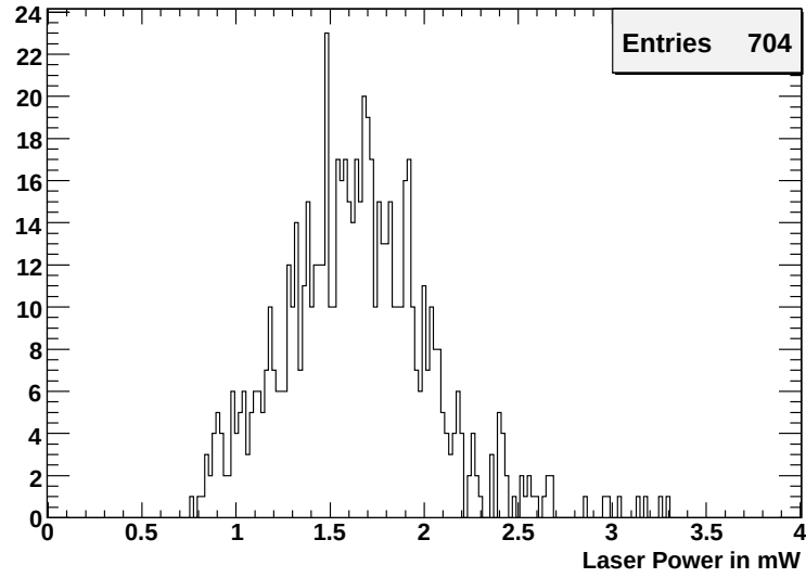
Figure 5.5: Distribution of averaged optical power generated by the TX-plugin VCSEL's at the highest possible laser current. The signal sent was a clock like signal, so the measured power value is about half of the signal amplitude. The mean averaged power is 1.64 mW with an RMS of 0.39 mW. The lower limit is 750 \mu W. 88 TX-plugins have been measured.
