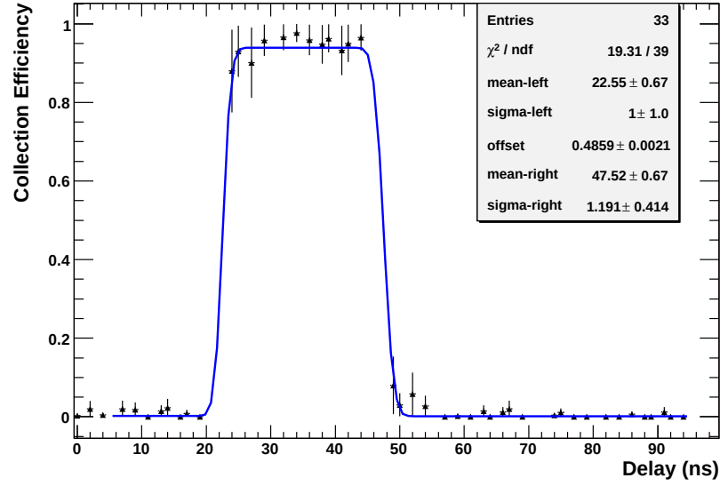
Figure 7.11: Collection efficiency versus the delay for hits with TOT=30.
