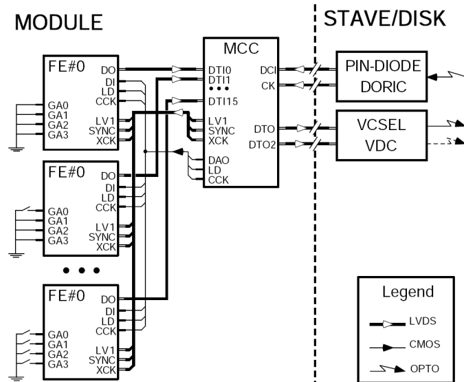
Figure 3.16: Sketch of the MCC to module communication [33].
