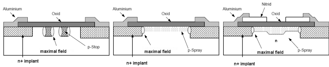
Figure 3.9: Cross sections of pixel isolation: on the left the traditional p-stop technique, in the middle the p-spray technique, and on the right the modified p-spray technique [26].
