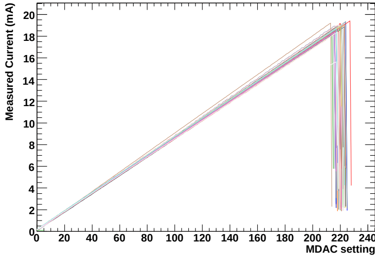
Figure 5.2: During the PiN-current test generated currents against the MDAC settings. At around 18 mA an overcurrent has to be observed to control the overcurrent safety option. The mean slope of the curves is s = (0.0855 \pm 0.0015) mA/steps, see Figure 5.4.
