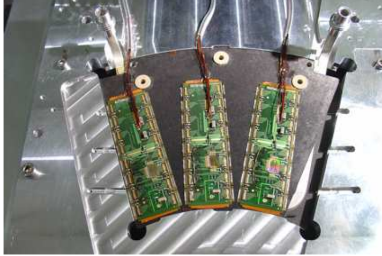
Figure 3.3: A sector on a test station. The sector is the smallest mechanical unit of a disk. A sector carries 6 module, 3 on the front and 3 on the back side.
