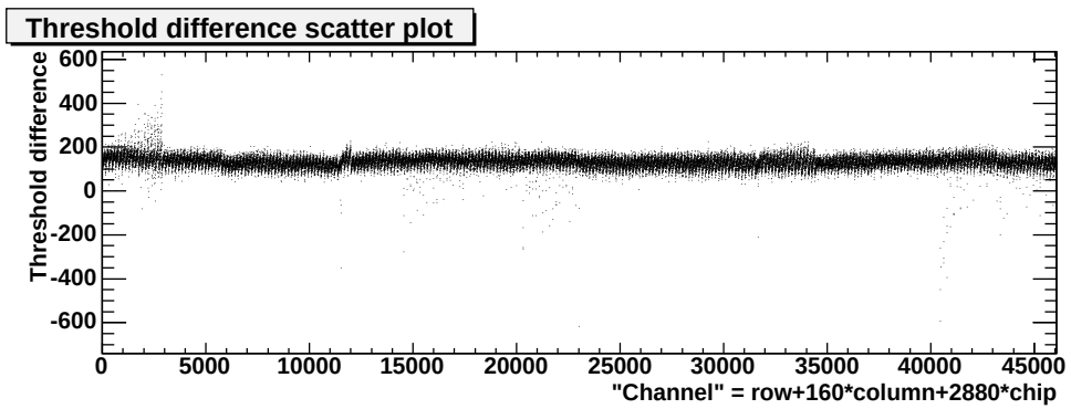
(c) Scatter plot of the threshold differences.
