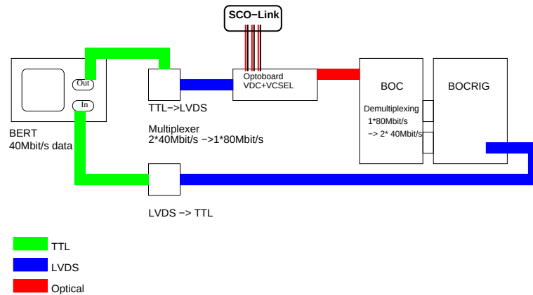
(b) Schematical overview of the setup for the bit error rate measurement.
