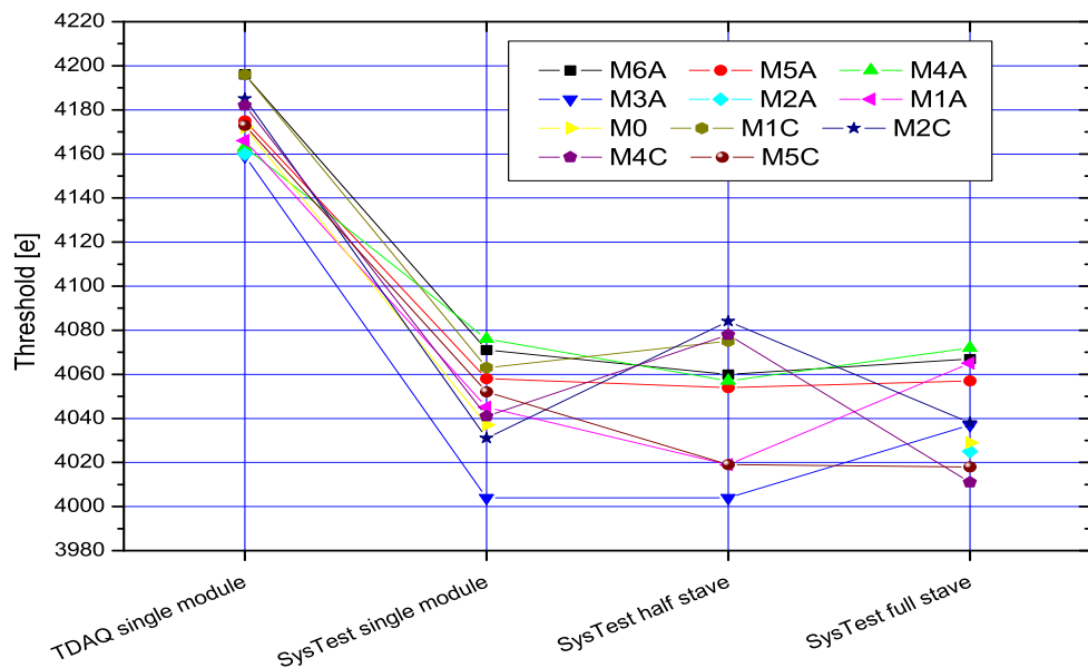
Figure 6.7: Mean threshold results for the modules on the system test stave 4008. The measurements were performed for different configurations of the powering and readout.
