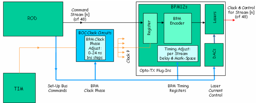
Figure 4.4: Schematic view of the command stream model in the Back of Crate card [40].
