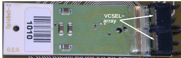
Figure 3.20: The optoboard. A B-Layer board is shown with two VCSEL-arrays. The dimensions are 2 \times 6.5 \text{ cm}^2 .
