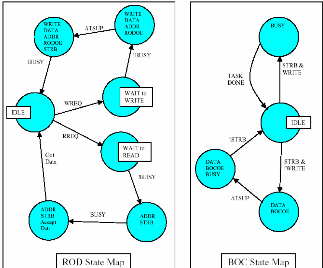
Figure 4.3: State map of the setup bus protocol [40]. The communication between the ROD and the BOC card is performed using this protocol.
