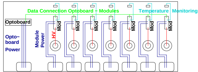
Figure 6.3: Schematic view of the PP0.
