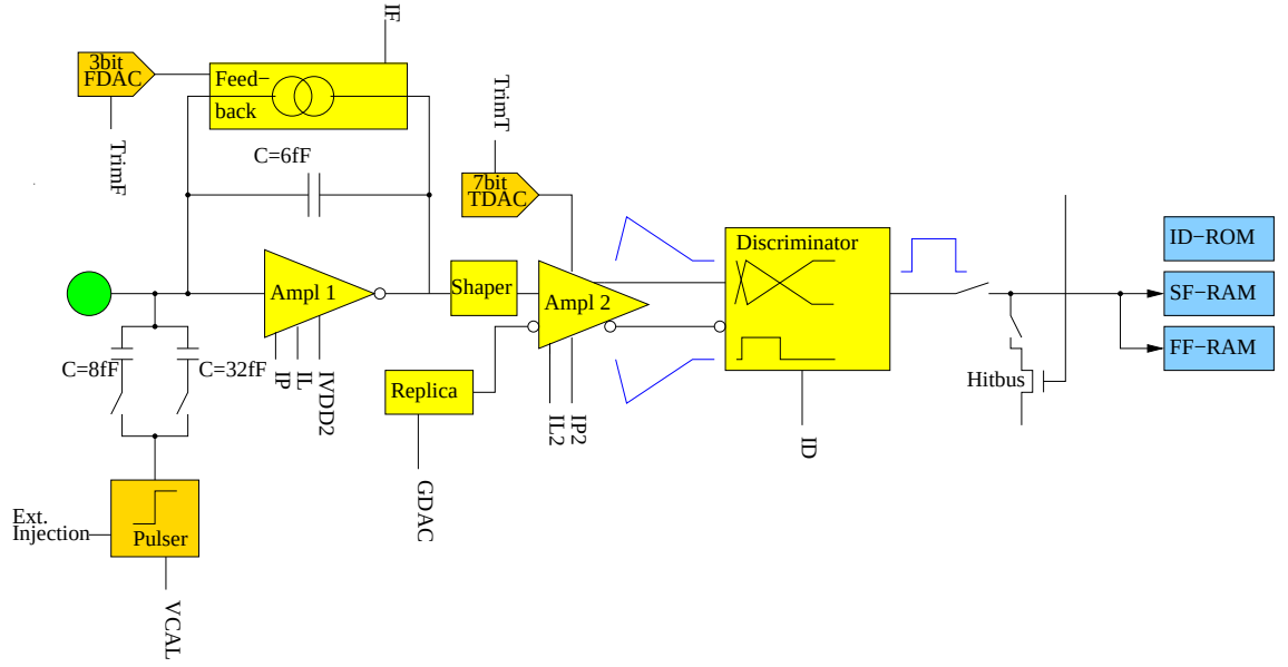
Figure 3.10: Schematic of the pixel unit cell.
