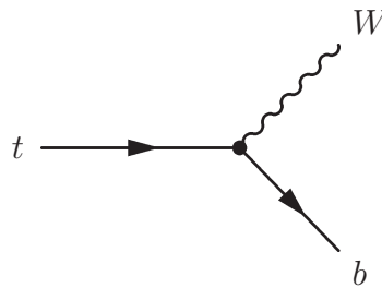
Figure 1.5: Main top decay mode: t \rightarrow W + b
