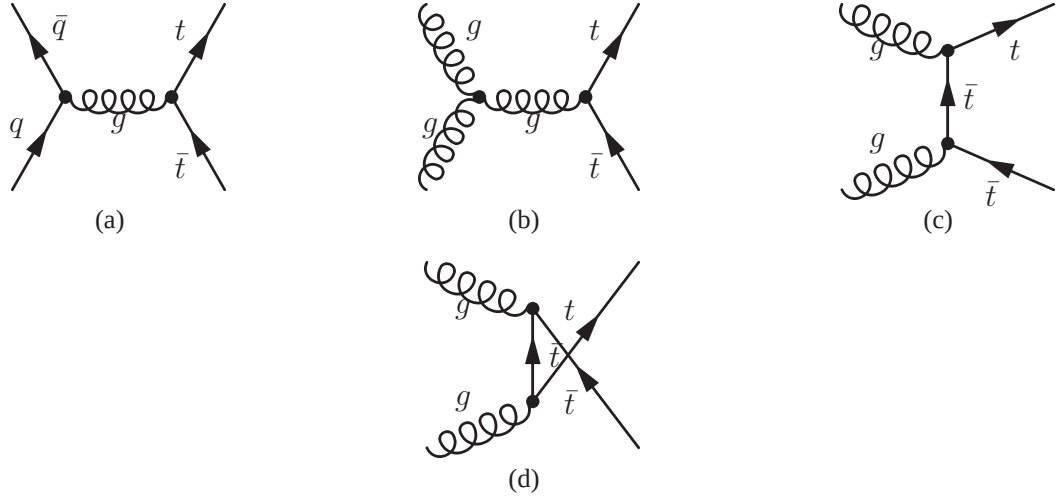
Figure 1.4: Main top quark production processes via strong interaction.
