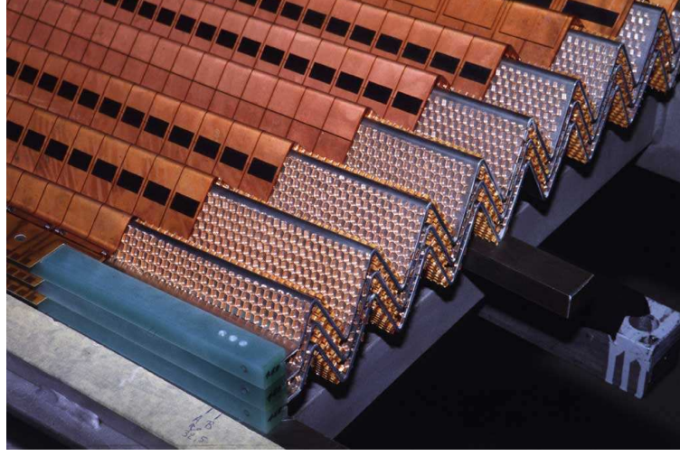
Figure 2.6: Liquid Argon Calorimeter in accordion structure
