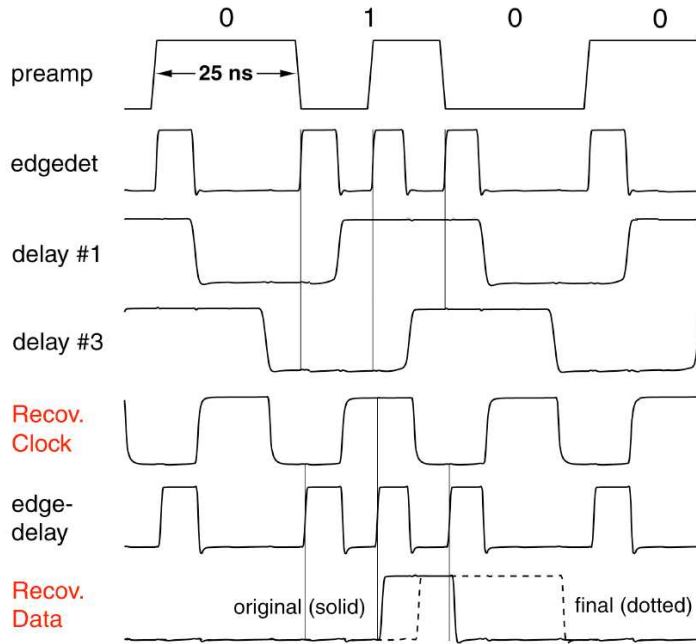
Figure 3.21: Biphasic mark (BPM) decoding [35].
