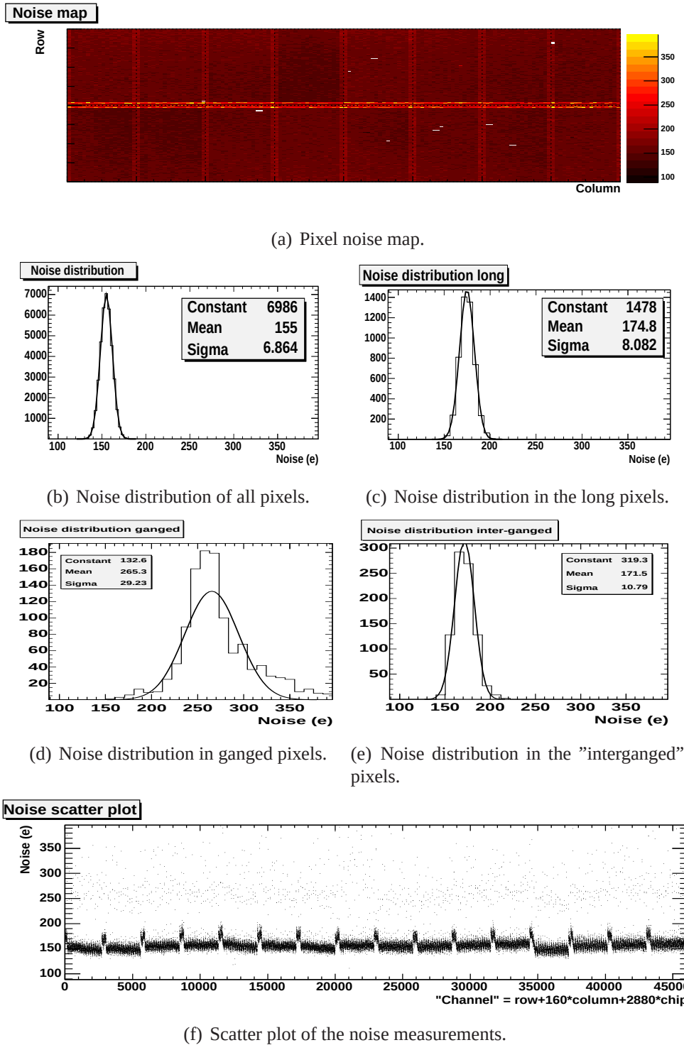
Figure 6.6: Typical result for a noise measurement. Here the result for the separately powered module M510868 is shown. The mean noise value is 155 e^- .
