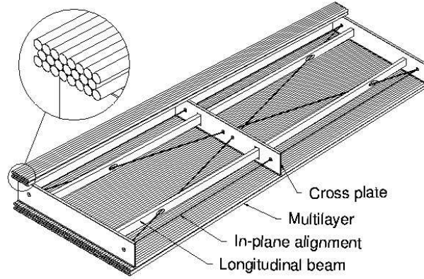
Figure 2.5: Monitored Drift Tube of the ATLAS muon System.
