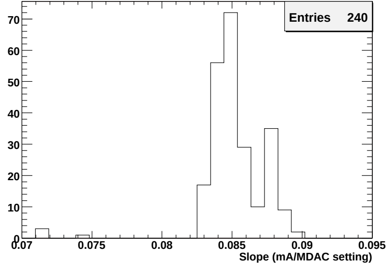
Figure 5.4: Slope of the current curves. The mean slope of the curves is s = (0.0855 \pm 0.0015) mA/steps. The slope limits are 0.080 < s < 0.095 mA/steps. 240 RX-sites have been measured.
