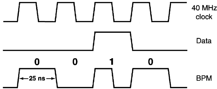
Figure 3.19: The principle of the bi phase mark encoding. The clock and the data signal are encoded into a BPM-signal
