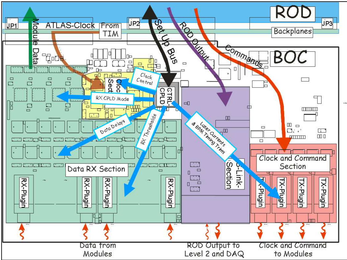
Figure 4.2: Schematical view of the Back of Crate card [40].
