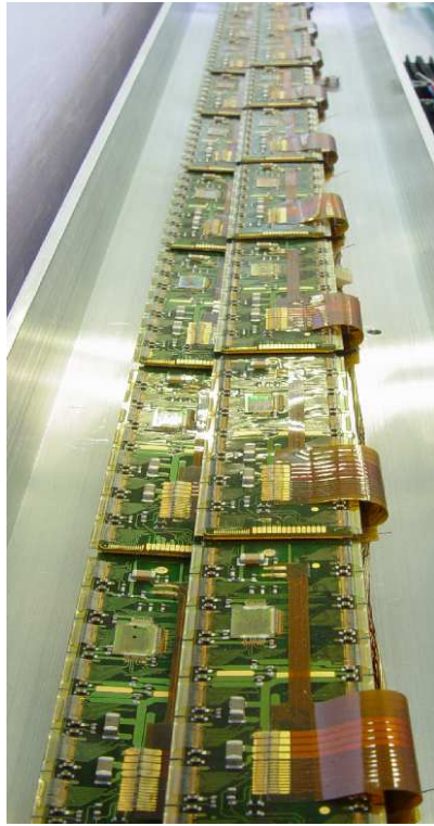
Figure 6.2: Bi-stave used as device under test in the Wuppertal system test.
