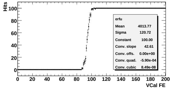
Figure 6.4: Result of a threshold scan for a pixel.
