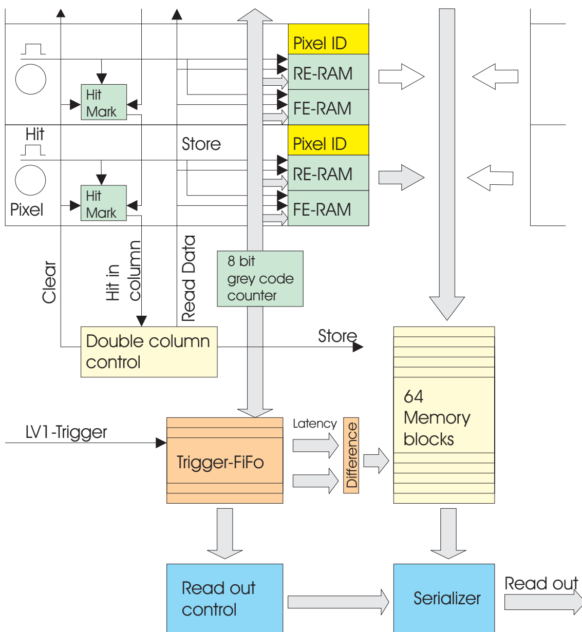
Figure 3.11: Schematic overview of the readout of hits from a pixel cell.
