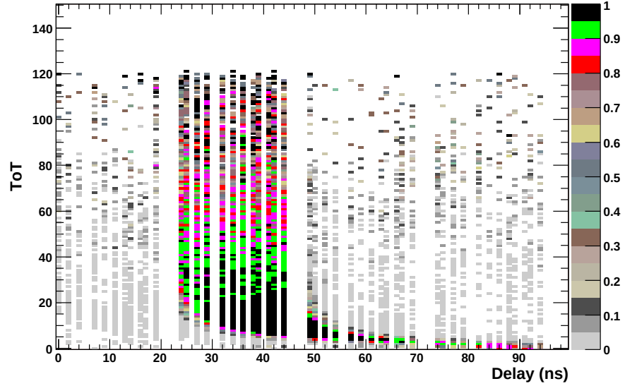
Figure 7.9: Collection efficiency. The colour represents the efficiency for the given TOT - delay setting, 2 dimensional visualisation. The plot shows the 12 delay setting for the 4 LV1 bins of interest, resulting in 48 delay settings in total.
