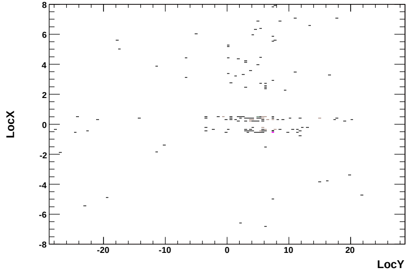
Figure 7.16: Hit map of hits with TOT < 5 , taken with a delay setting of 22 ns. LocX and LocY are representing the module dimensions in mm.
