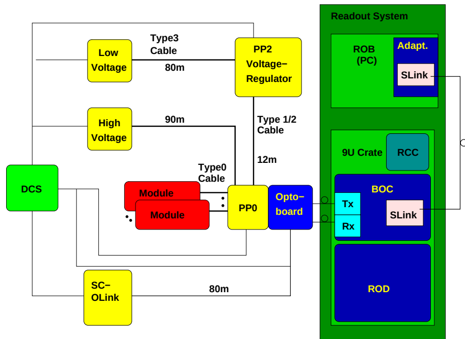
Figure 6.1: Readout scheme of the system test [45]. The parts of the power supply system are yellow, the readout system green and blue. This work will mainly focus on the readout system.
