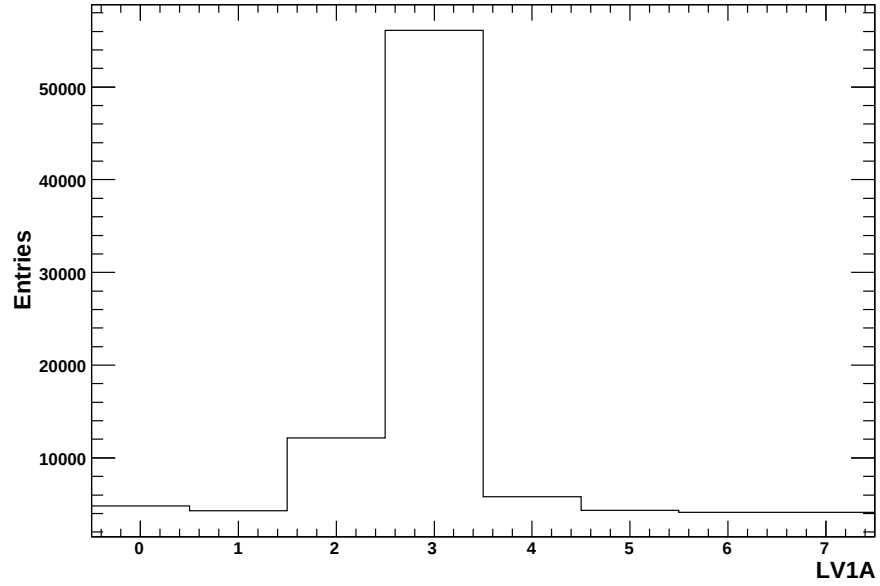
Figure 7.6: LV1 distribution for all TOT values for hits assigned to a track.
