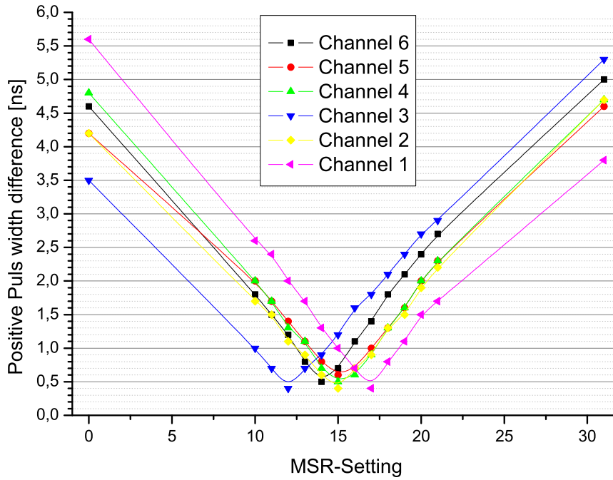
Figure 6.13: Scan of the clock edge "hopping" in dependence of the mark space ratio (MSR) setting.
