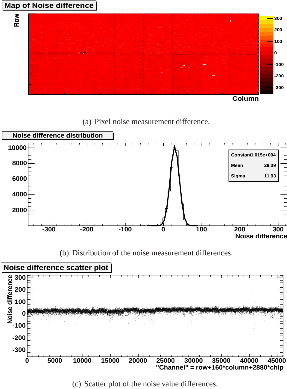
Figure 6.10: The calculated difference of the pixel noise values measured with the TurboDAQ system and the optical system for module 510868 on the test stave is shown.
