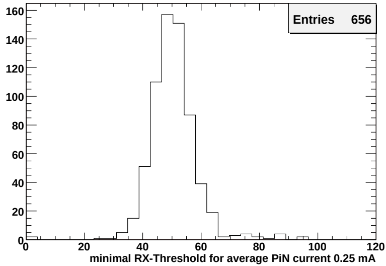
Figure 5.6: Distribution of the minimal RX-threshold for receiving the data correctly at a mean PiN current of 250 \mu\text{A} . The mean RX-threshold value is 50.14 with an RMS of 8.69. The minimal RX-threshold must be below 160. 82 RX-plugins have been measured.
