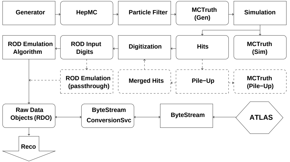
Figure 7.4: Overview of the Athena framework for the offline software development [57]. The upper three lines are showing the Monte Carlo generation being formatted into an RDO. The lower line is representing the detector data being formatted into an RDO.
