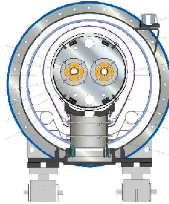
Figure 2.3: Cross section of the vacuum pipes inside a quadrupole magnet [14].
