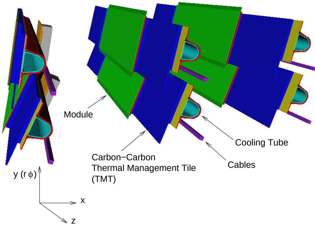
Figure 7.2: GEANT simulation of the pixel detector in the Combined Test Beam setup.
