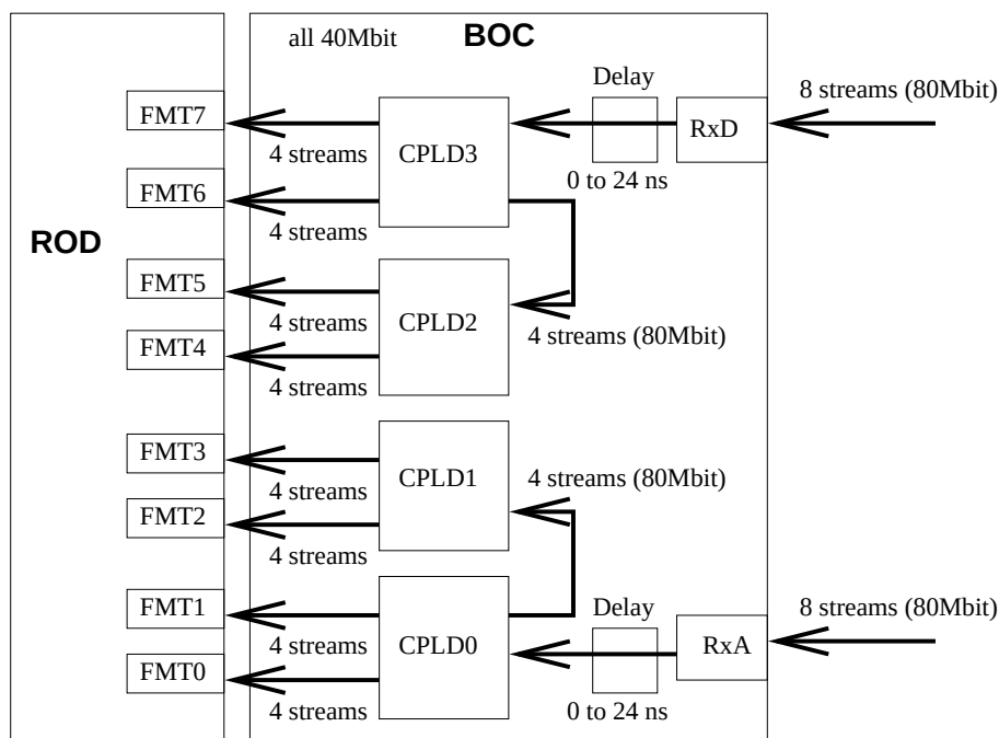
Figure 4.10: Data flow through the BOC card in 80 Mb/s or 160 Mb/s operation.
