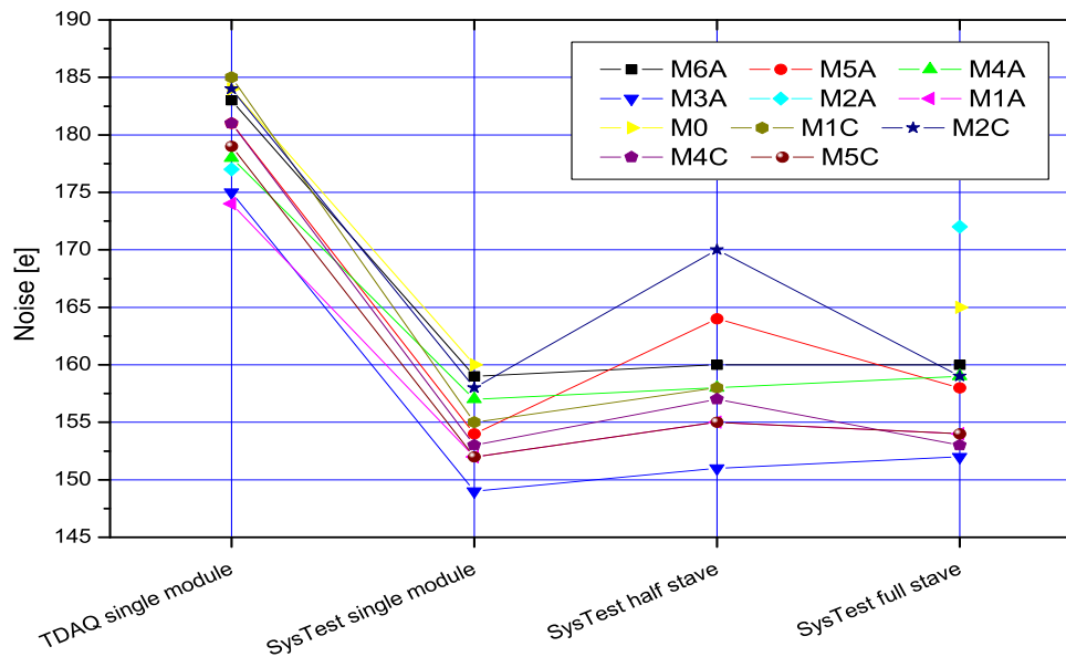
Figure 6.9: Noise measurement results for the modules on the system test stave 4008. The measurements were performed for different configurations of the powering and readout.
