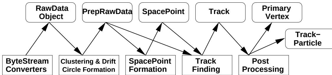
Figure 7.5: Overview of track reconstruction. The data object (top) are processed through algorithms (bottom) [57].
