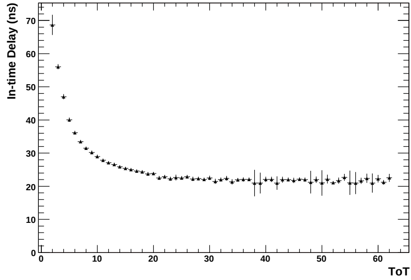
Figure 7.12: Delay setting for in-time registering versus the TOT.
