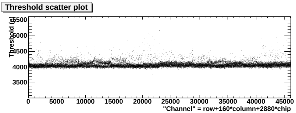
(c) Scatter plot of the pixel thresholds.
