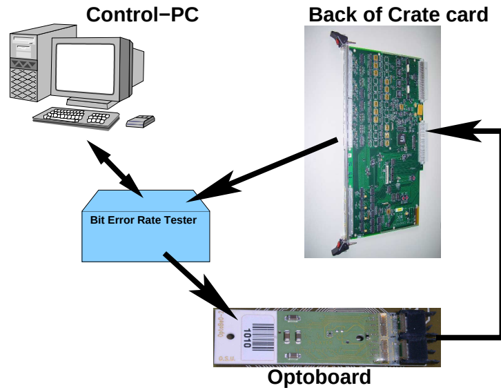
(a) Components of the bit error rate measurement.
