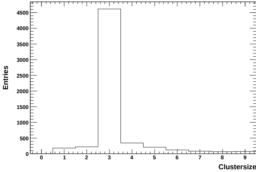
Figure 7.15: Cluster size of the hits with TOT < 5 clock cycles.
