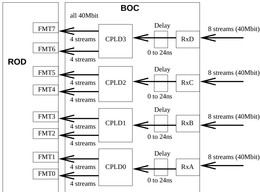
Figure 4.9: Data flow through the BOC card in 40 Mb/s operation.
