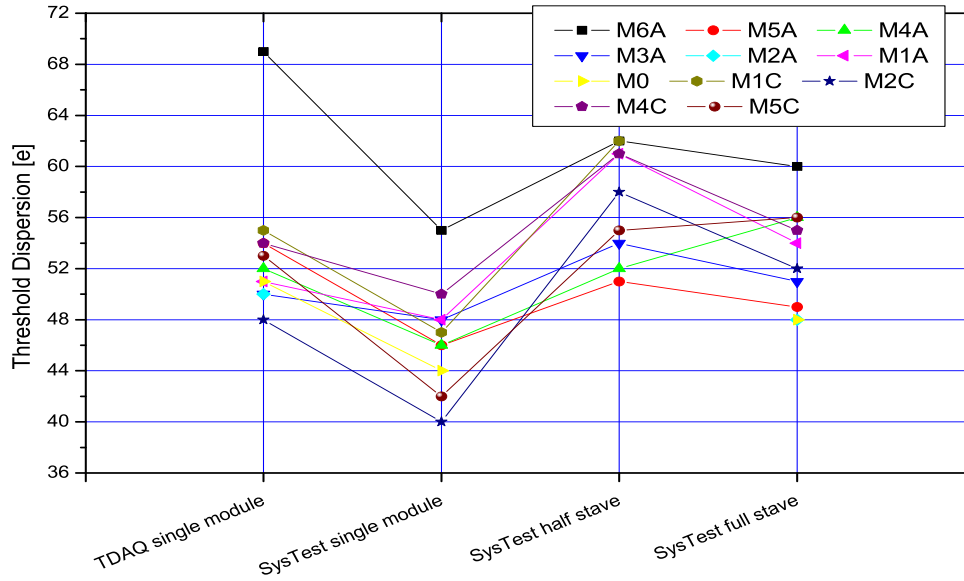
Figure 6.8: Threshold dispersion results for the modules on the system test stave 4008. The measurements were performed for different configurations of the powering and readout.
