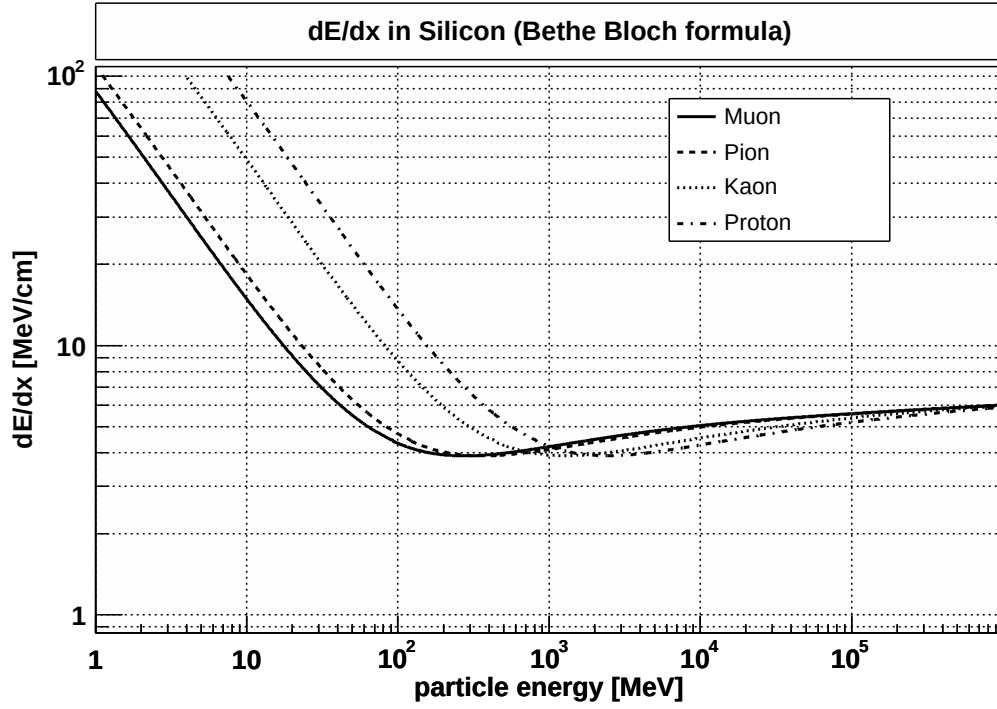
Figure 3.5: Energy loss of different types of particles according to the Bethe-Bloch equation, calculated for particles traversing 250 \mu\text{m} thick silicon [23].
