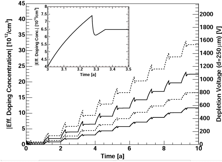
Figure 3.7: Sensor full depletion voltage under irradiation and annealing for the 10 years of ATLAS. The dashed lines are for pure silicon, the solid lines show the oxygen enriched silicon, which is used for the pixel detector. The upper two lines are for the B-Layer, the lower two lines are for Layer1 [27].
