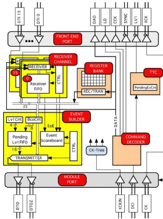
Figure 3.15: Block diagram of the MCC logic [33].
