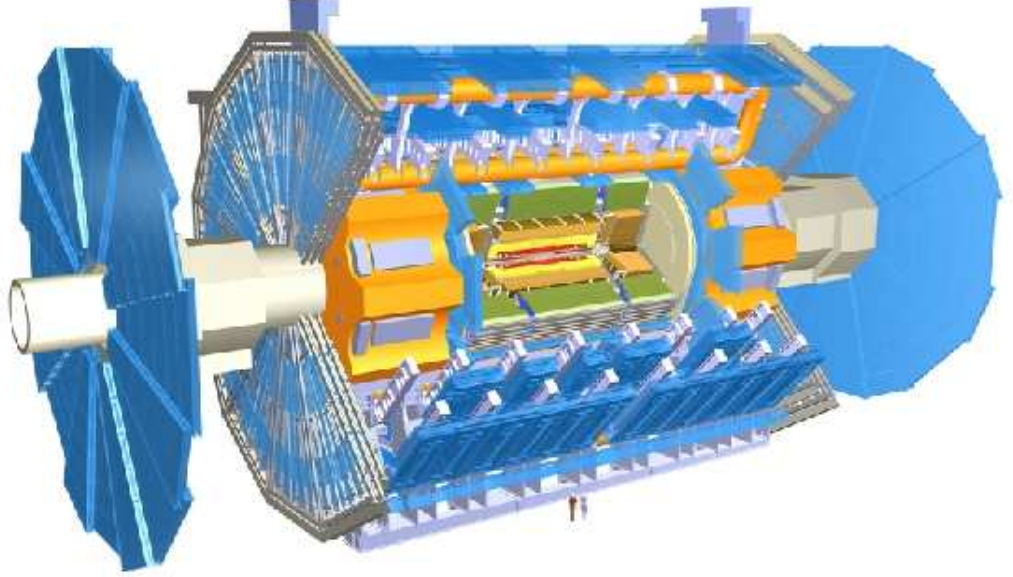
Figure 2.4: Schematic of the ATLAS experiment [14].
