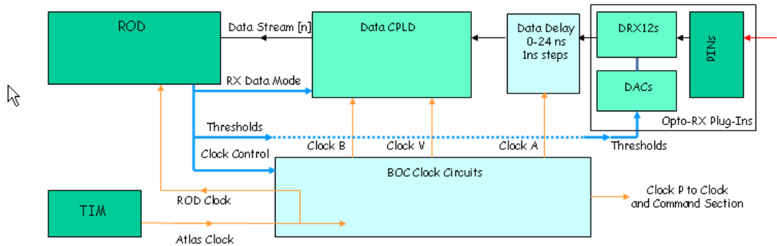
Figure 4.6: Schematic view of the data recovery circuit in the Back of Crate card [40]. The V-Clock is used for 80 Mb/s operation only.
