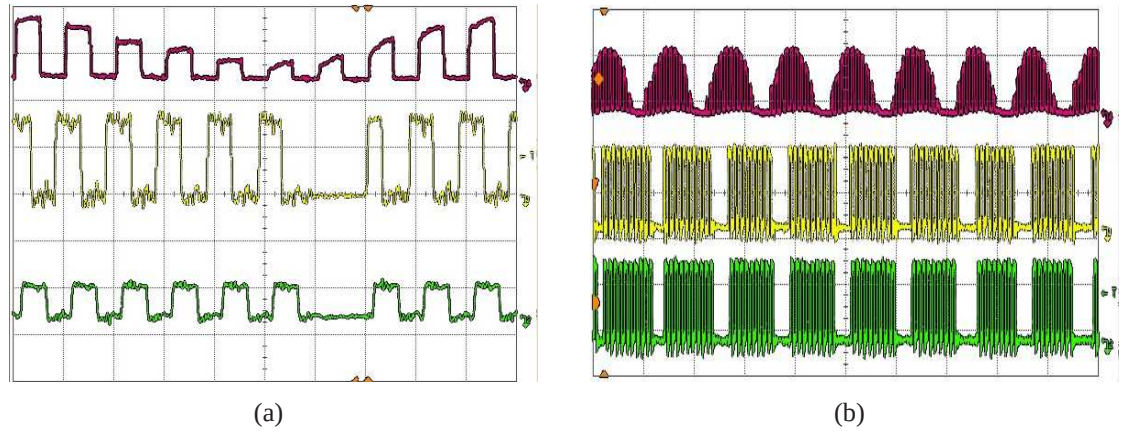
Figure 6.16: Signals transmitted by the optoboard in case of induced errors. Scoped are the optical signal (purple) of channel 1 and the received signal (yellow and green) on the BOC for channel 2. The yellow line shows the signal before sampling (RX-plugin output), the green line shows the sampled signal.
