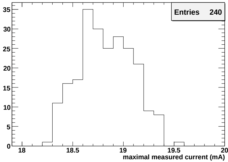
Figure 5.3: The maximal generated current before breakdown. The mean value is 18.83 mA with an RMS of 0.26 mA. The limits are 18 \text{ mA} < I < 20 \text{ mA} . 240 RX-sites have been measured.
