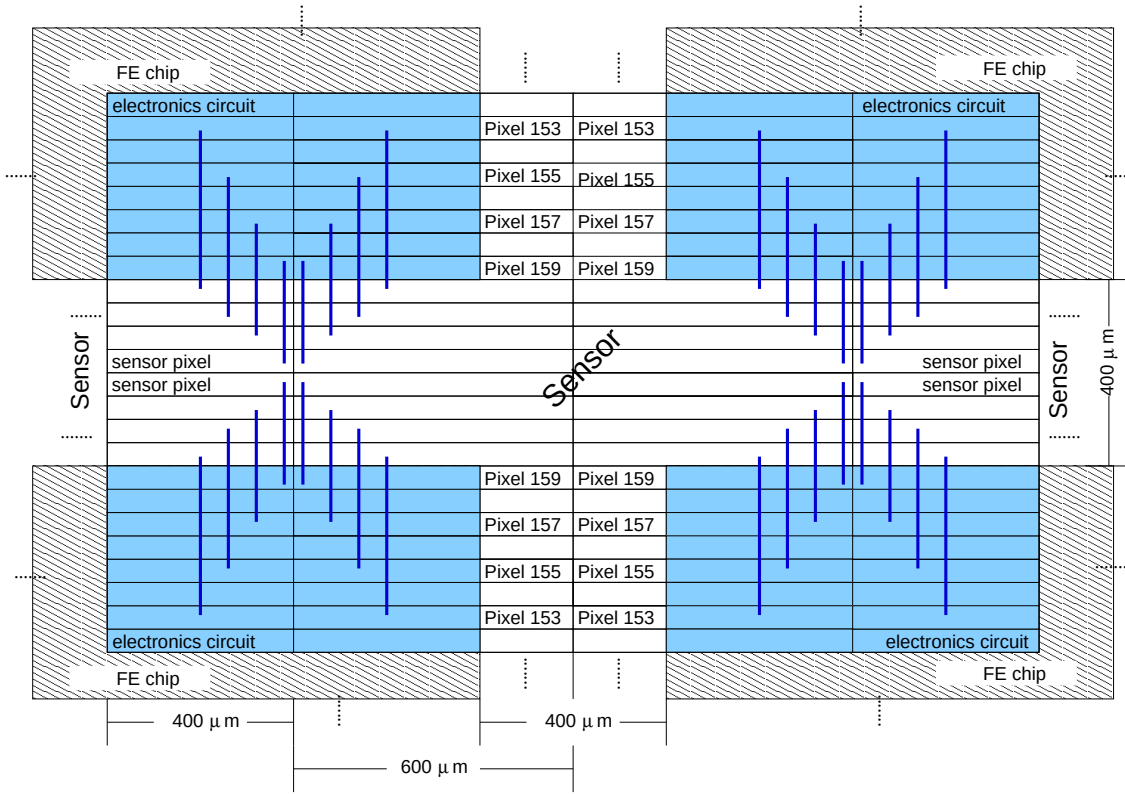
Figure 3.8: Ganged sensor pixels as view on the sensor top side. The pixels are the long horizontal structures. The vertical junctions are the connections of two pixel. The edges of the read out chips are sketches. A double connected cell always alternates with a single connected cell.
