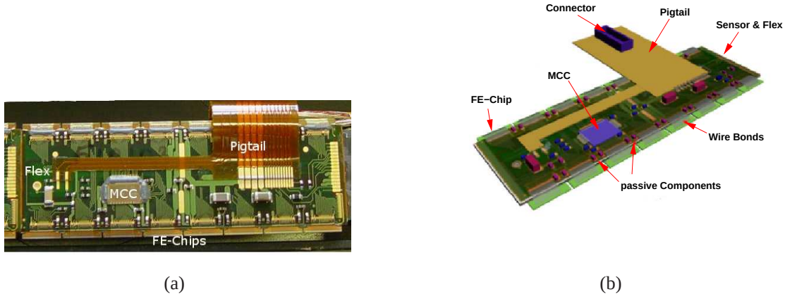
Figure 3.4: A pixel module. The 16 Front End (FE) chips are underneath as shown in the illustration. A flexible capton foil provides the interconnections between the FE chips and the module control chip (MCC) on top.
