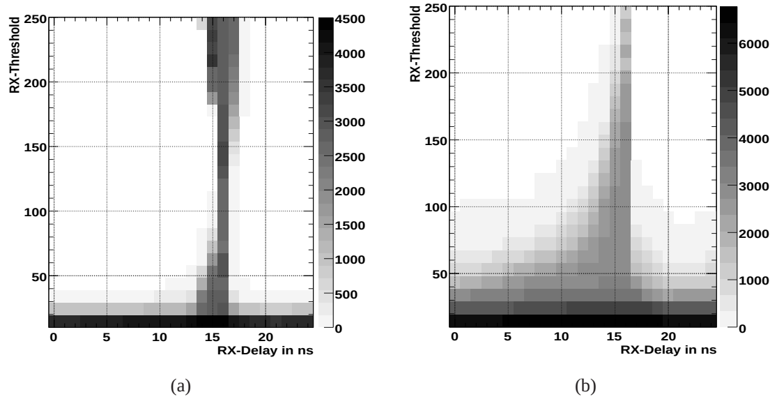
Figure 6.14: Result of a 2-dimensional scan of the RX threshold versus the RX data delay. The gray scale give the bit errors in the transmission. The different behaviour depends on the light power emitted by the optoboard VCSEL. Plot a) shows the result for an optimised light power. Plot b) shows the scan result for a higher light power. The working range has shrunk.
