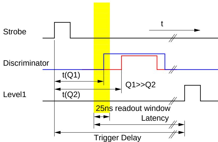
Figure 3.13: Principle of timewalk measurement [26]. The read out window (yellow) is shifted by the latency setting. Pulses of different height are illustrated (see Figure 3.12).
