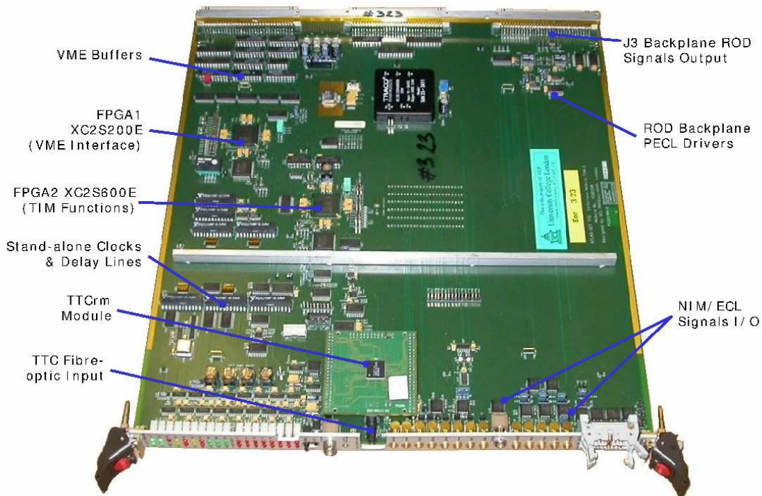
Figure 3.24: The TIM (TTC Interface Module) [39].
