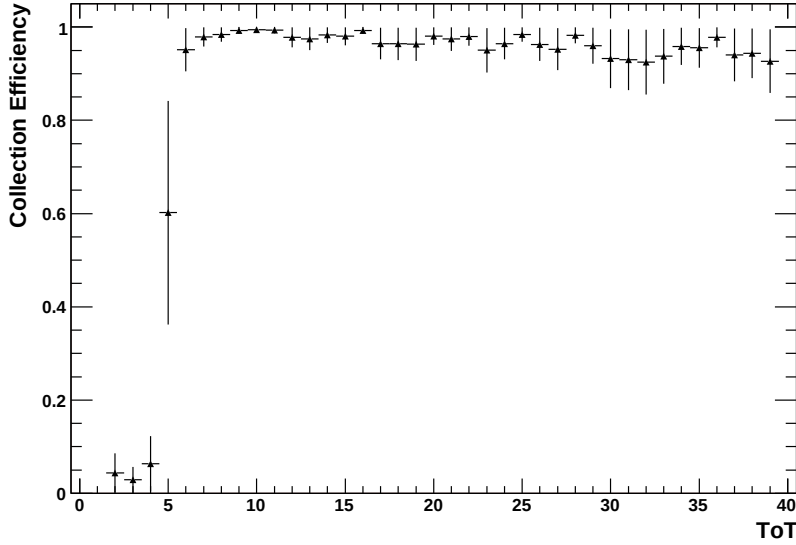
Figure 7.14: Collection efficiency as a function of the TOT for the optimised delay setting of 22 ns. Hits with a TOT lower than 5 clock cycles are not registered in the readout window.
