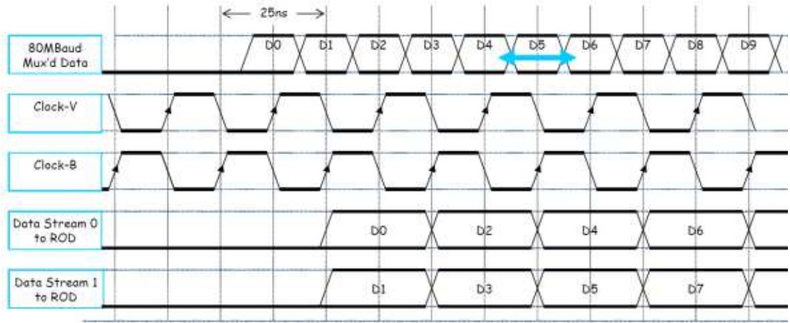
Figure 4.8: Demultiplexing of an 80 Mb/s stream into two 40 Mb/s streams [41].
