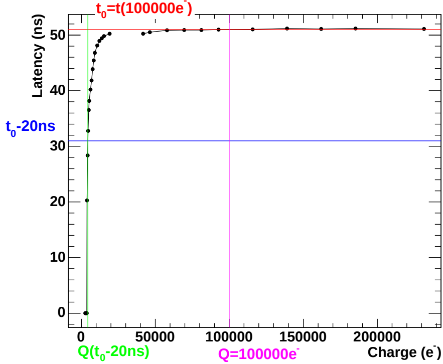
Figure 3.14: Measured timewalk of a single pixel with low and high injection capacity. The data reflects the latency at which 50% of the hits generating the given charge are registered.
