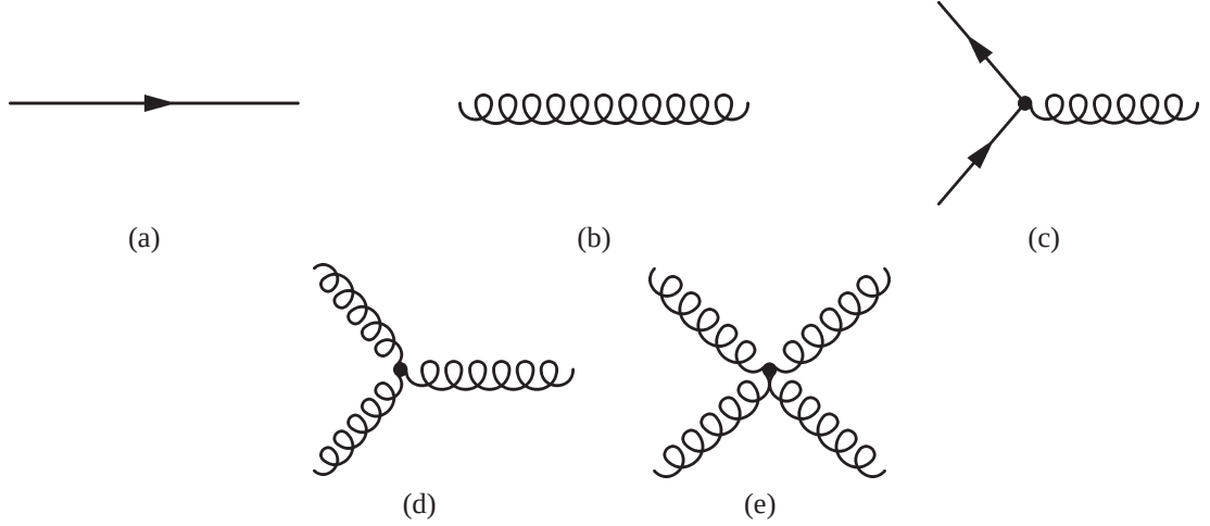
Figure 1.2: Fundamental Feynman graphs of QCD: a) Quark propagator, b) Gluon propagator, c) Interaction vertex, d) and e) Gluon self-coupling
