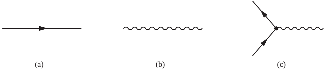
Figure 1.1: Fundamental Feynman graphs of QED: a) Fermion propagator, b) Photon propagator, c) Interaction vertex
