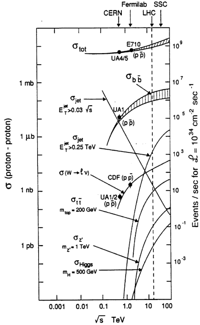
Figure 1.3: Energy dependence of some characteristic cross-sections from present colliders to the LHC [10].
