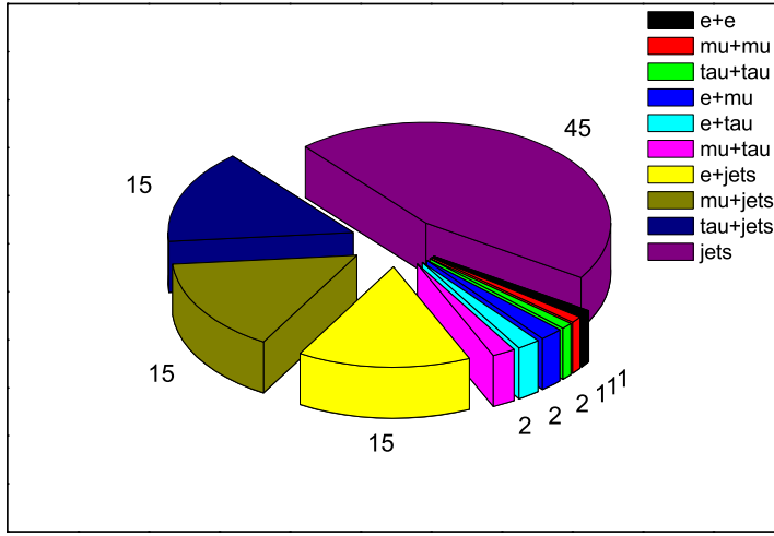
Figure 1.6: Branching ratios for the decay of the t\bar{t} pair [12].
