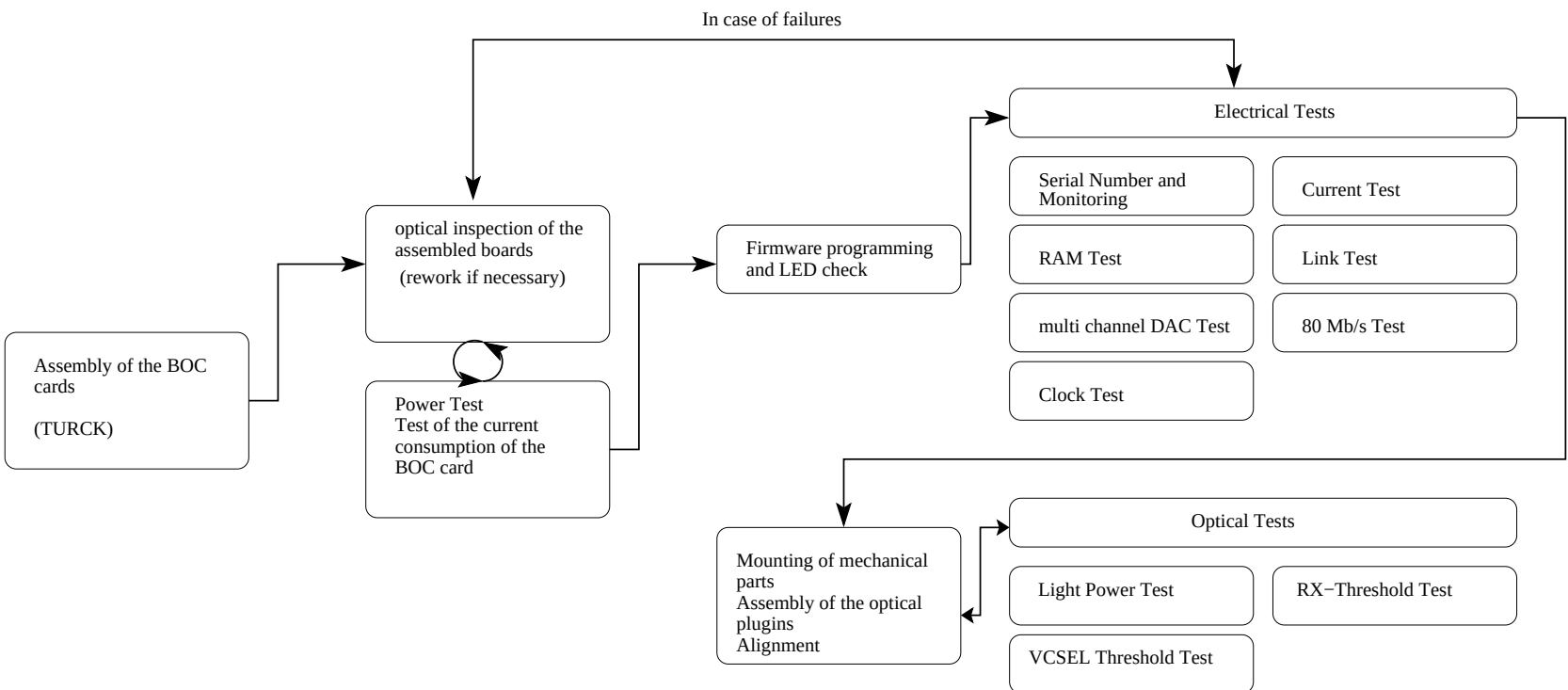
Figure 5.1: Production and test flow for the BOC card.
