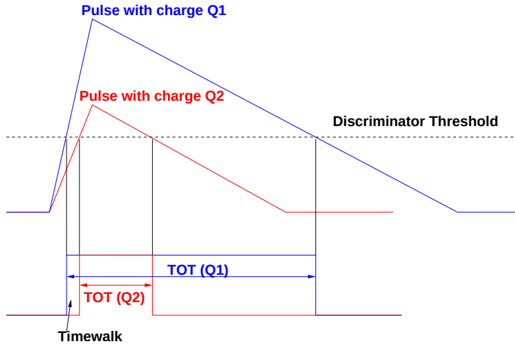
Figure 3.12: Schematic of hits with different energy deposition in the detector.
