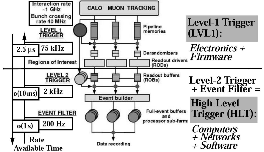
Figure 2.7: The overview of the ATLAS trigger and data acquisition system [18].
