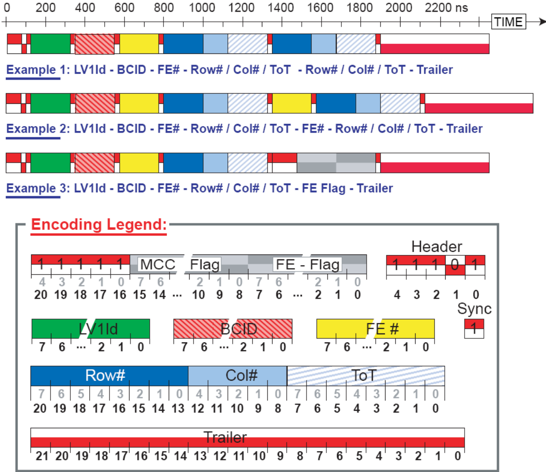
Figure 3.17: Data flow in the module control chip [32].
