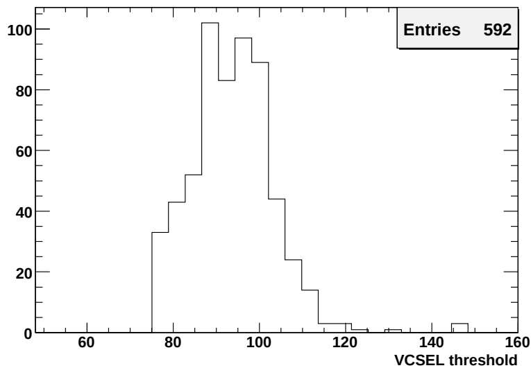
Figure 5.7: Distribution of VCSEL thresholds for generating a PiN-current of 0.2 mA.
